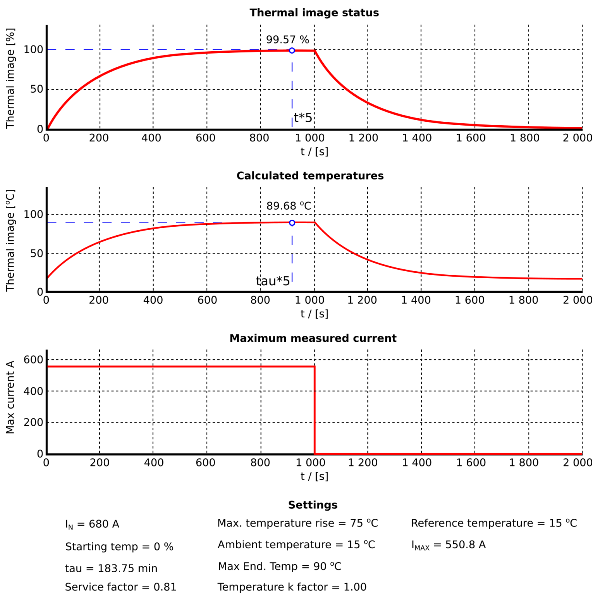
Figure. 5.4.7 - 98. Thermal response with k SF factor correctly set.
