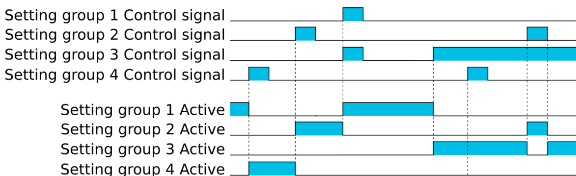
Figure. 5.5.1 - 101. Example sequences of group changing (control with pulse only, or with both pulses and static signals).
