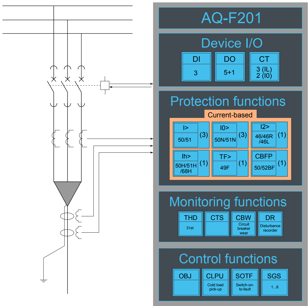
Figure. 7.1 - 139. AQ-F201 application example with function block diagram.
