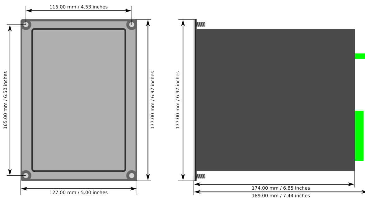
Figure. 8.4 - 150. Device dimensions.
