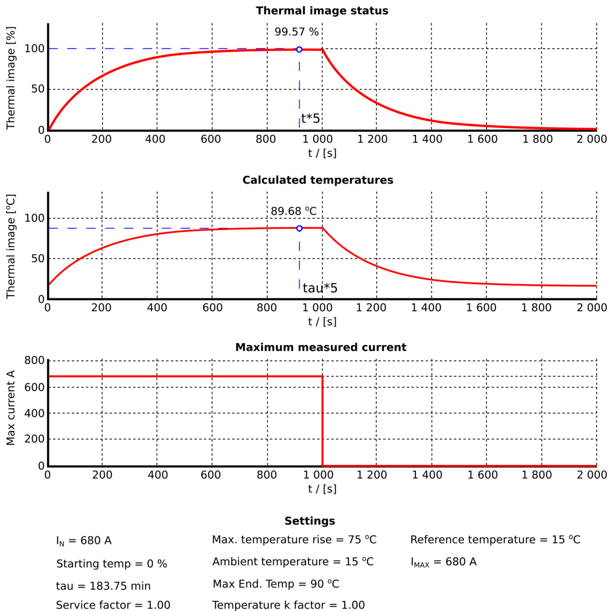
Figure. 5.4.7 - 96. Thermal image response with maximum load (installation according to presumptions).
