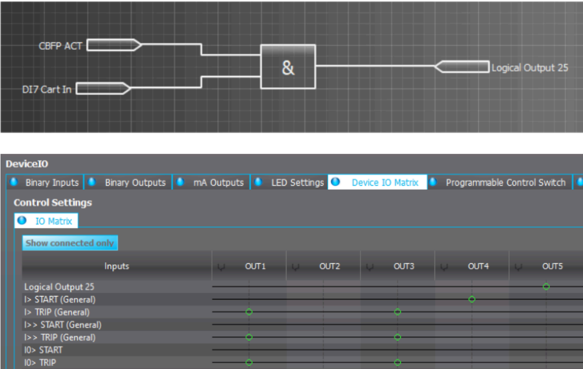
Figure. 5.5.7 - 116. Logic output example. Logical output is connected to an output relay in matrix.
