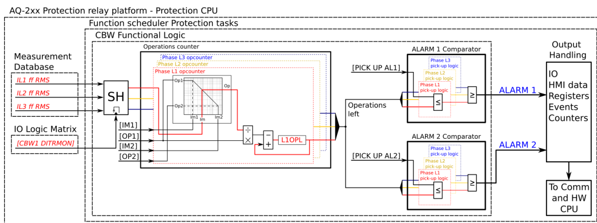
Figure. 5.6.2 - 131. Simplified function block diagram of the circuit breaker wear function.
