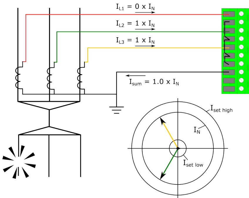
Figure. 5.6.1 - 123. Primary circuit fault in phase L1 wiring.
