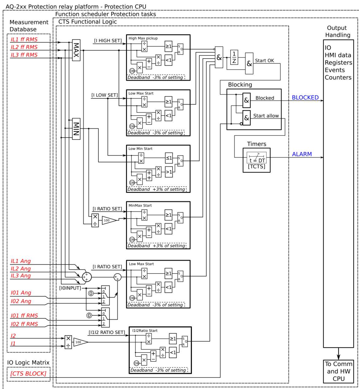
Figure. 5.6.1 - 120. Simplified function block diagram of the CTS function.
