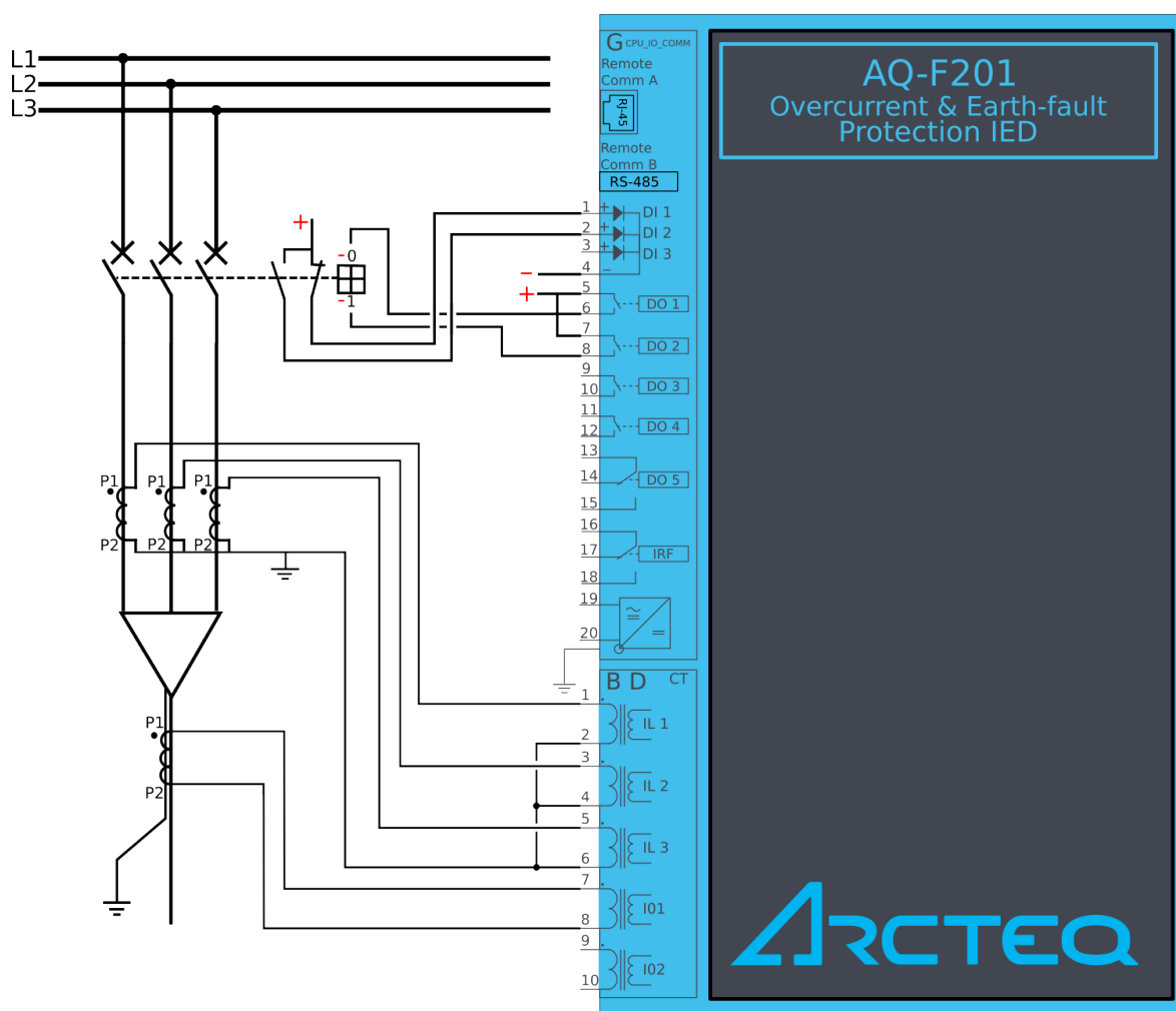
Figure. 7.2 - 140. Application example and its connections.
