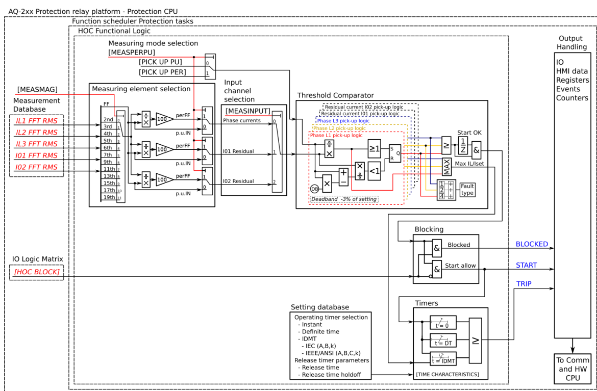
Figure. 5.4.5 - 75. Simplified function block diagram of the I_h > function.
