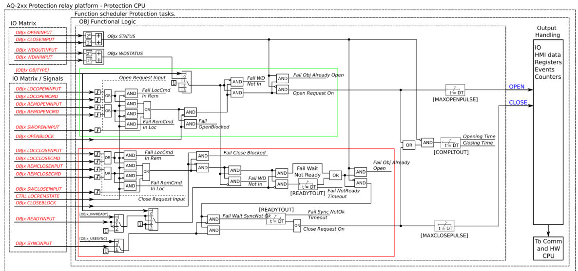
Figure. 5.5.2 - 106. Simplified function block diagram of the object control and monitoring function.
