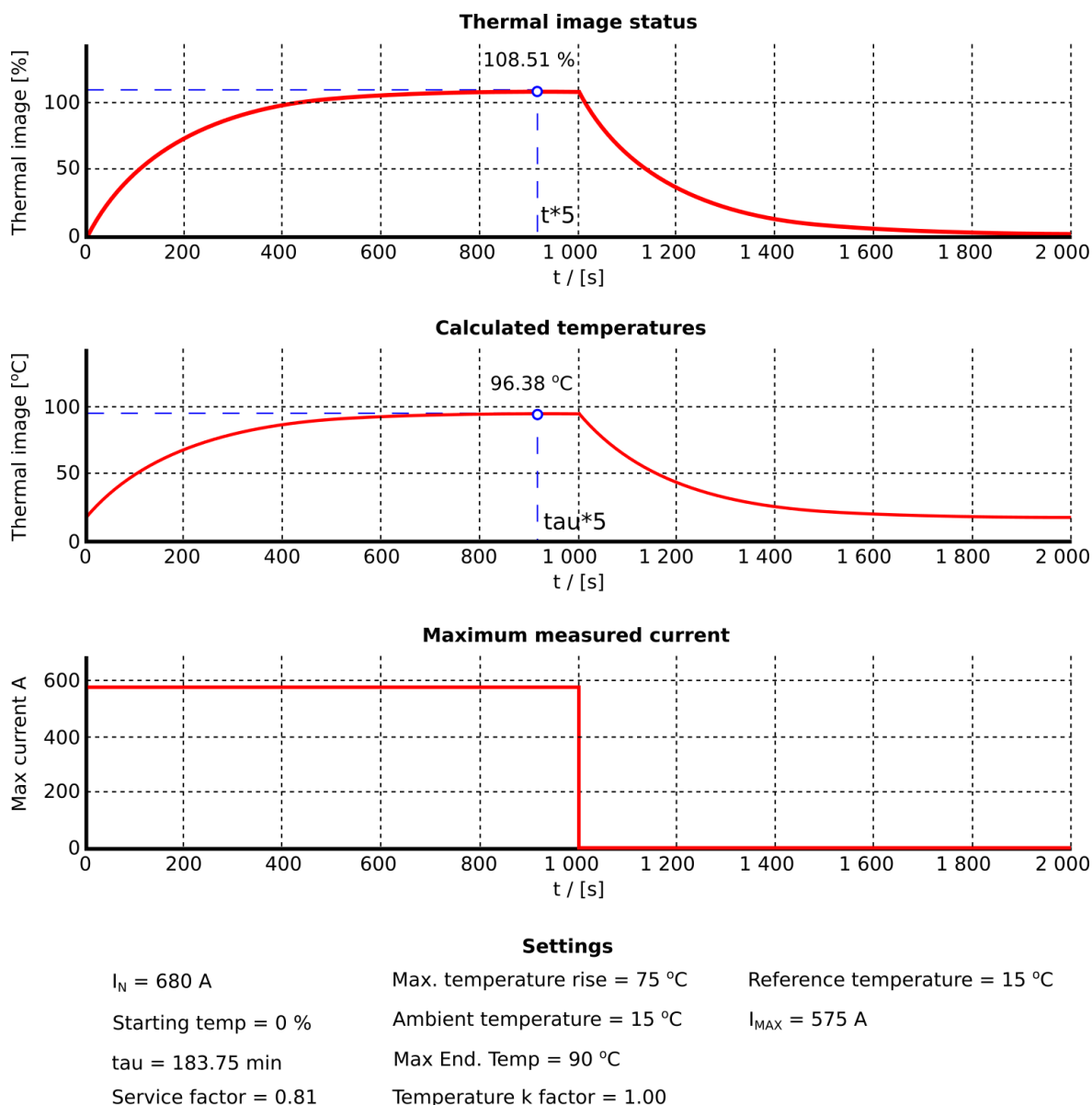
Figure. 5.4.7 - 97. Thermal image response with nominal currents and fine-tuned k_{\text{SF}} correction factor.
