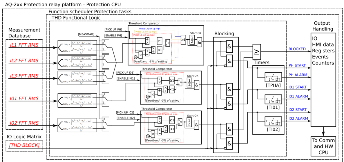
Figure. 5.6.3 - 133. Simplified function block diagram of the total harmonic distortion monitor function.
