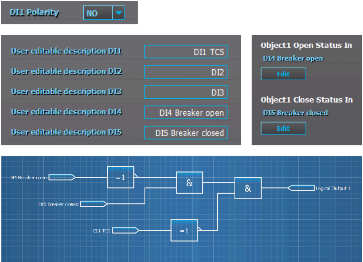
Figure. 7.4 - 146. Example block scheme.
