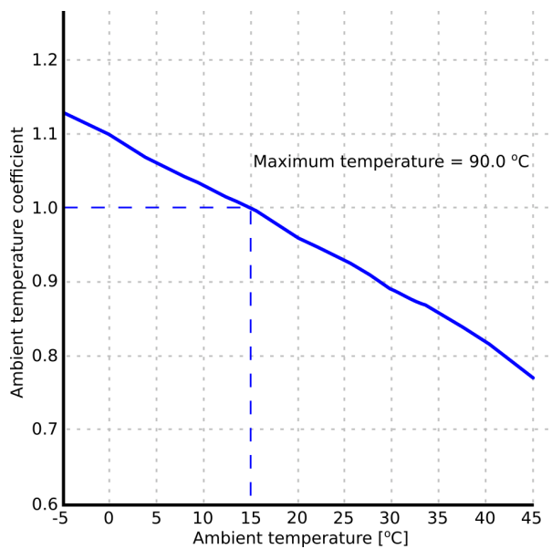
Figure. 5.4.7 - 91. Set correction curve for ambient temperature.
