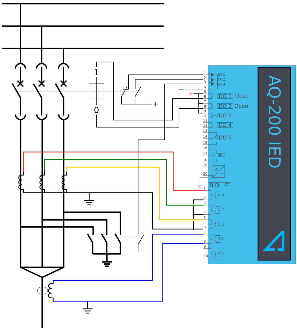
Figure. 5.5.2 - 107. Example of an interlock application.
