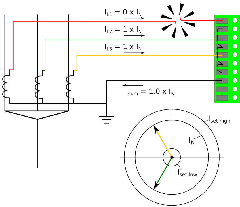
Figure. 5.6.1 - 122. Secondary circuit fault in phase L1 wiring.
