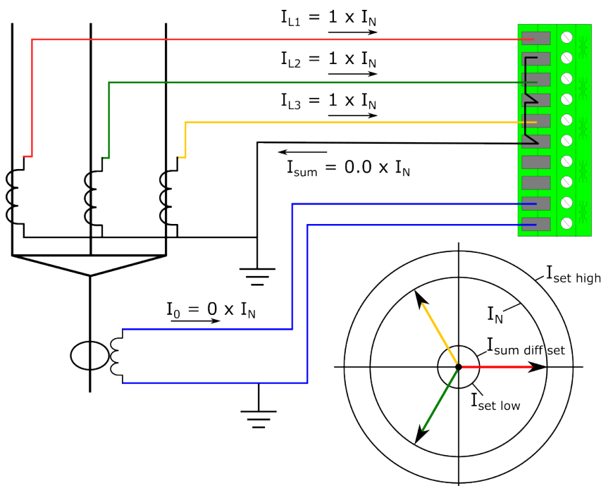
Figure. 5.6.1 - 126. Normal situation, residual current also measured.
