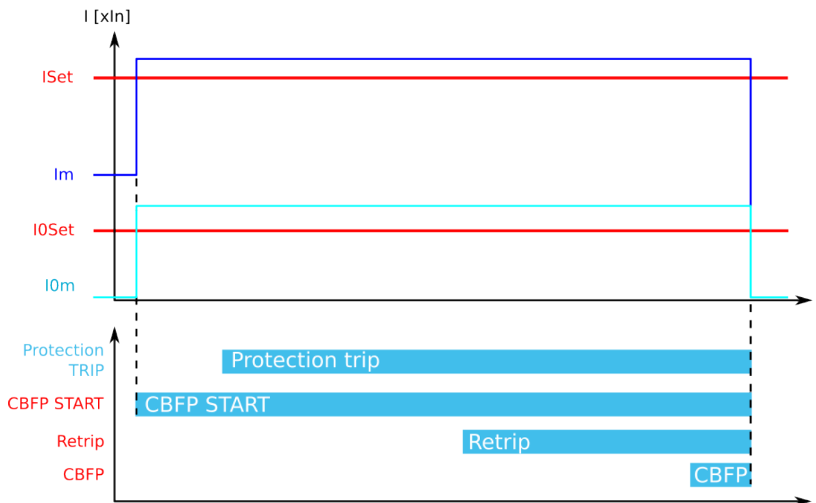
Figure. 5.4.6 - 78. Retrip and CBFP when "Current" is the selected criterion.
