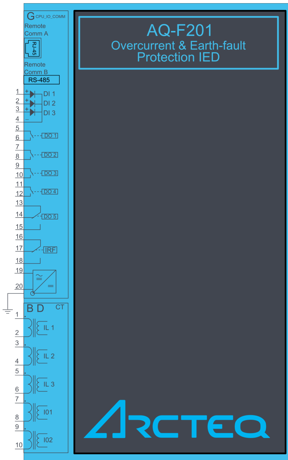
Figure. 7.1 - 138. AQ-F201 hardware.
