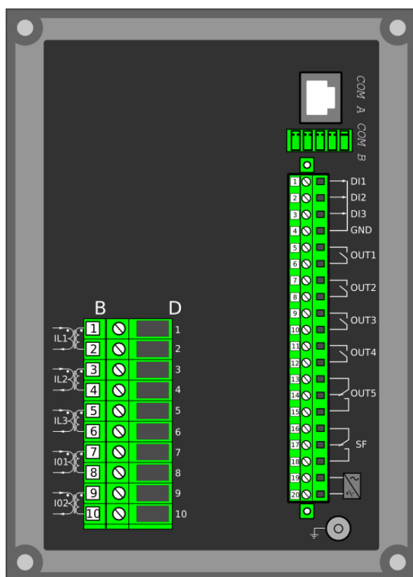
Figure. 8.1 - 147. Connections and modules in AQ-F201.
