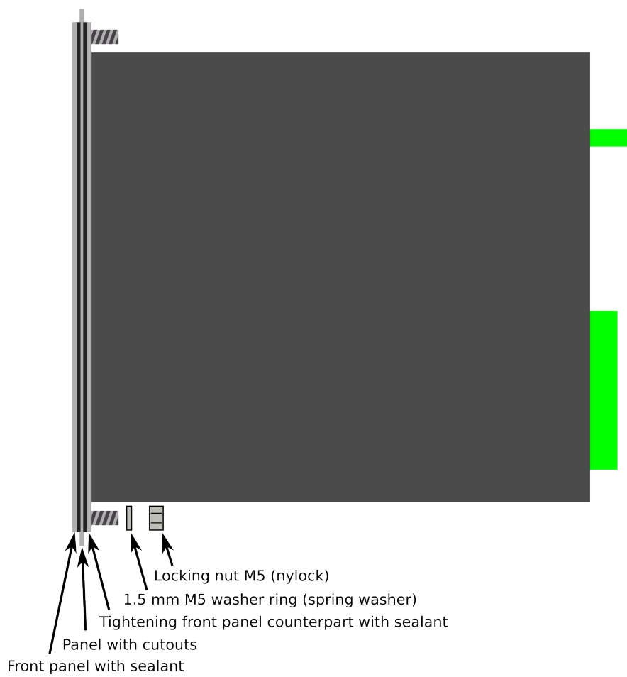
Figure. 8.4 - 151. Device installation.
