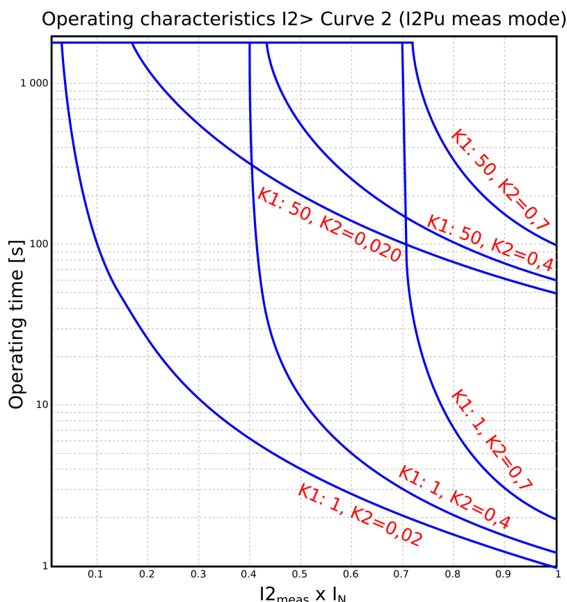
Figure. 5.4.4 - 74. Operation characteristics curve for I_2 > \text{Curve2} .
