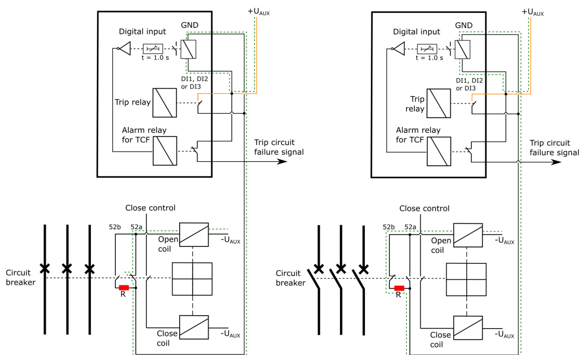
Figure. 7.4 - 142. Trip circuit supervision with one DI and one non-latched trip output.
