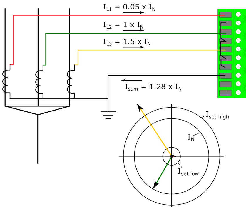
Figure. 5.6.1 - 124. No wiring fault but heavy unbalance.
