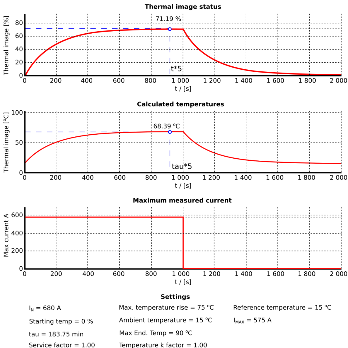
Figure. 5.4.7 - 95. Thermal image response with nominal load (installation according to presumptions).
