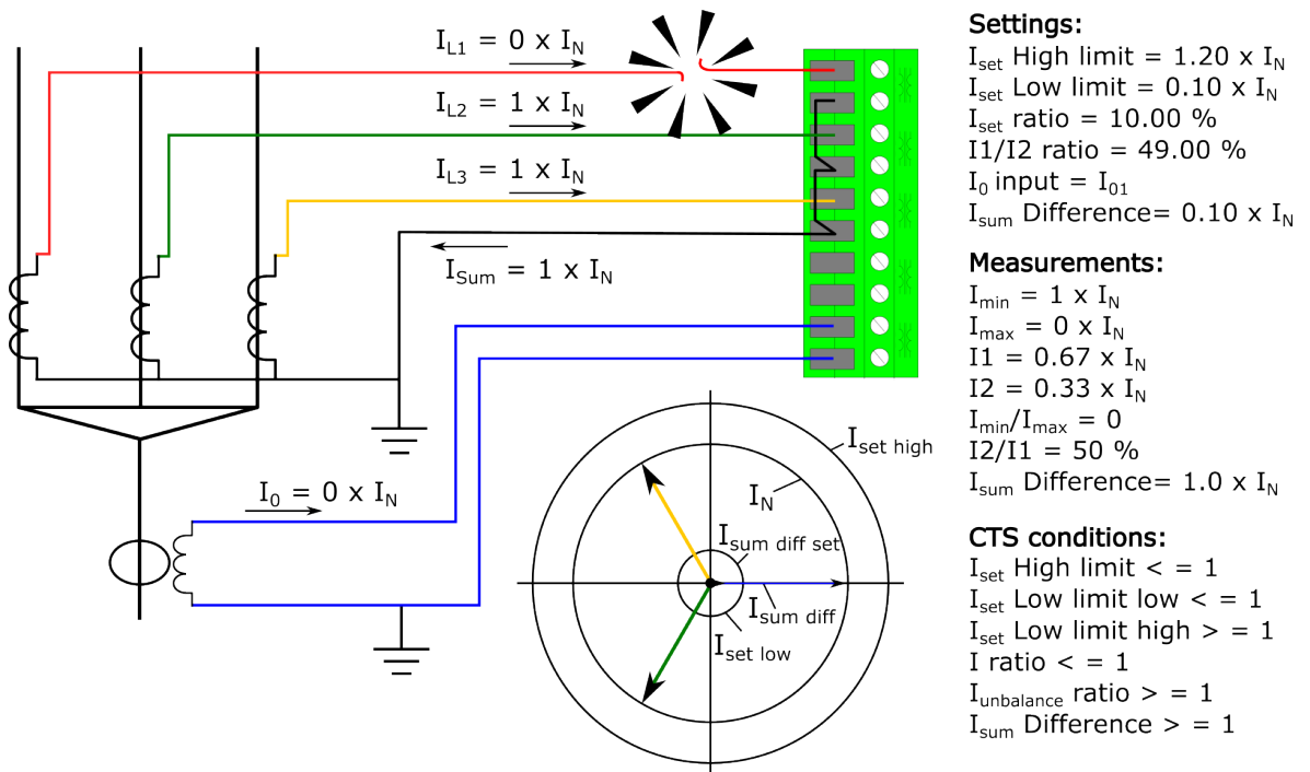
Figure. 5.6.1 - 127. Broken secondary phase current wiring.
