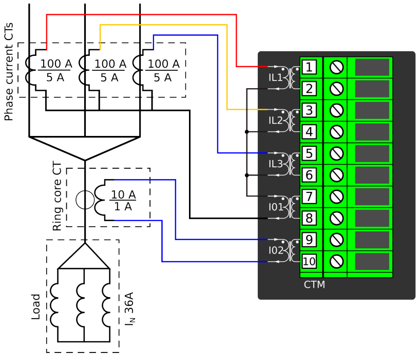
Figure. 5.2.1 - 52. Connections.
