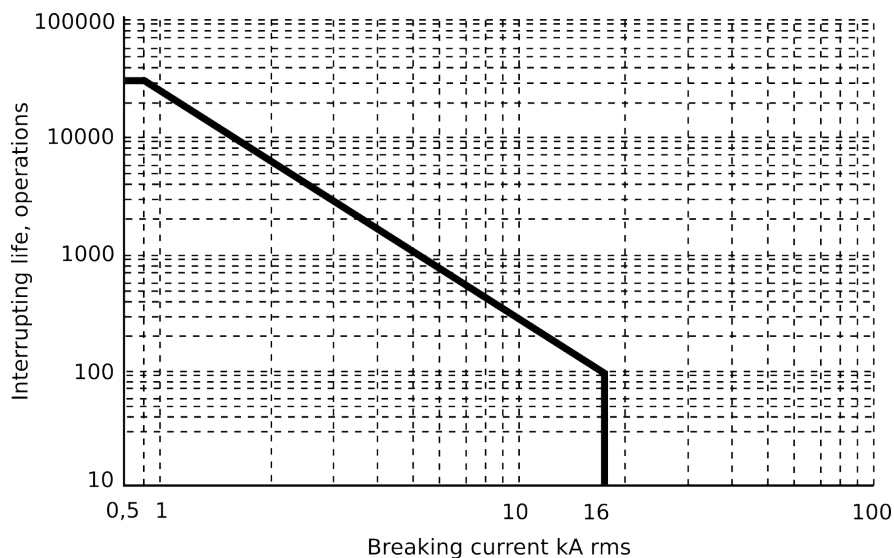
Figure. 5.6.2 - 130. Example of the circuit breaker interrupting life operations.
