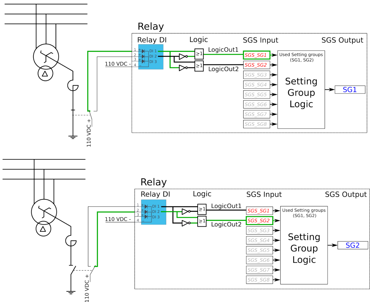
Figure. 5.5.1 - 104. Setting group control – two-wire connection from Petersen coil status with additional logic.
