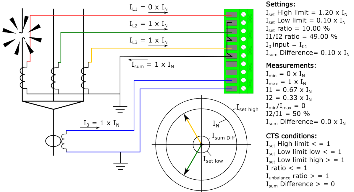
Figure. 5.6.1 - 128. Broken primary phase current wiring.
