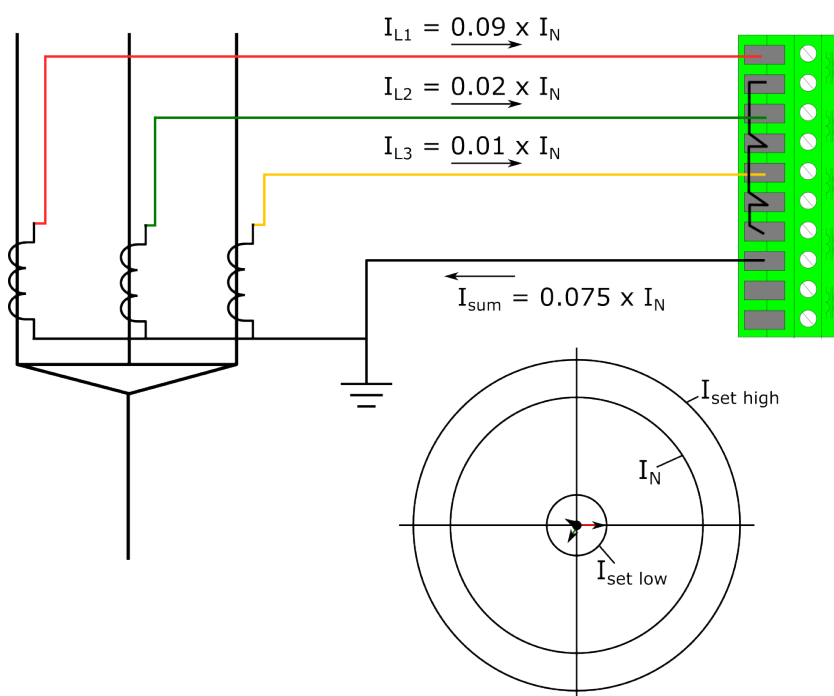
Figure. 5.6.1 - 125. Low current and heavy unbalance.
