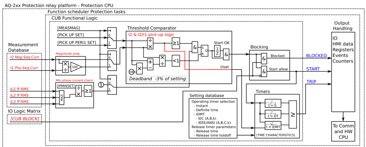
Figure. 5.4.4 - 73. Simplified function block diagram of the CUB function.
