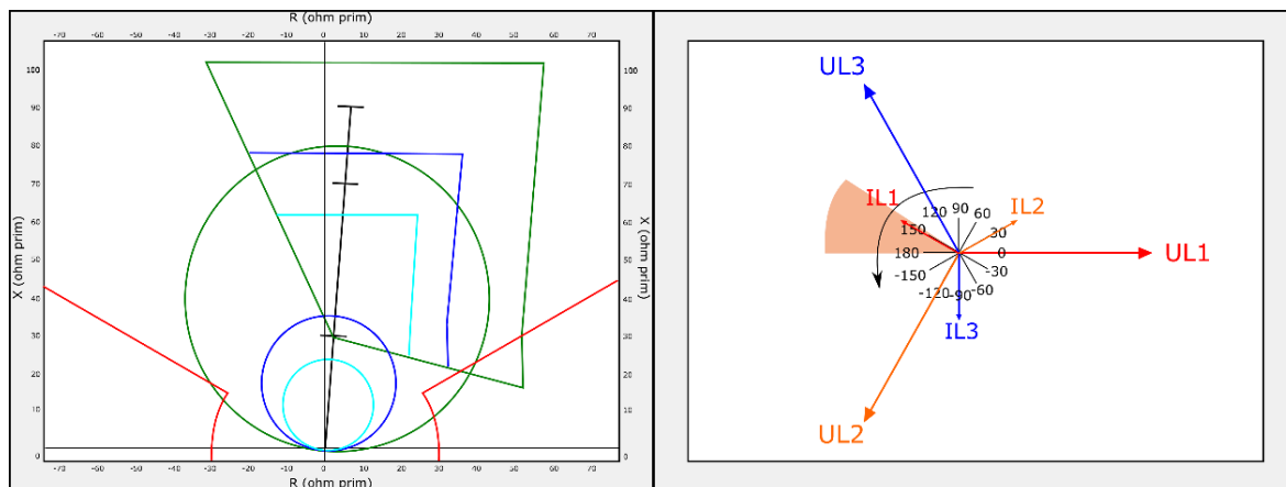
Figure. 5.4.22 - 164. Distance protection characteristics and directional overcurrent.
