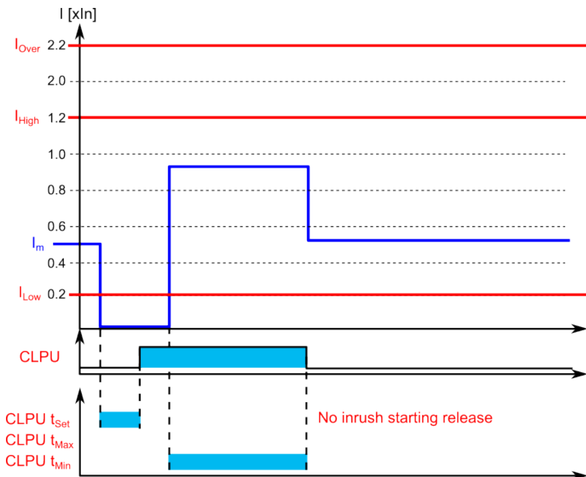
Figure. 5.5.6 - 198. Example of timers and pick-up parameters (no inrush current detected in the starting).
