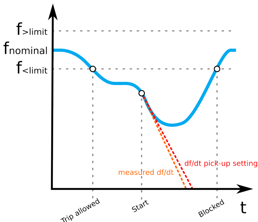
Figure. 5.4.15 - 138. Operation of the df/dt > / < function when the frequency starts but doesn't trip.
