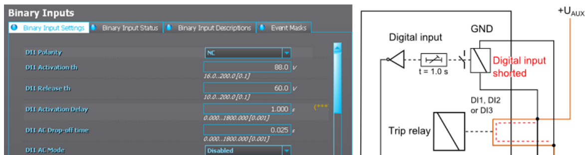
Figure. 7.4 - 235. Settings for a digital input used for trip circuit supervision.
