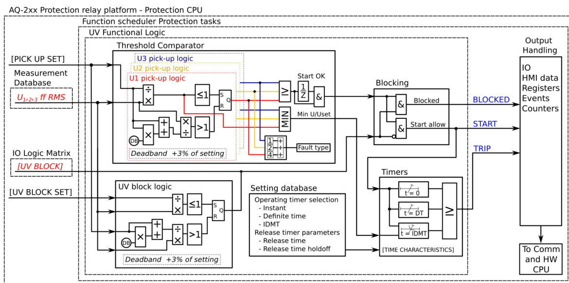
Figure. 5.4.11 - 122. Simplified function block diagram of the U&lt; function.
