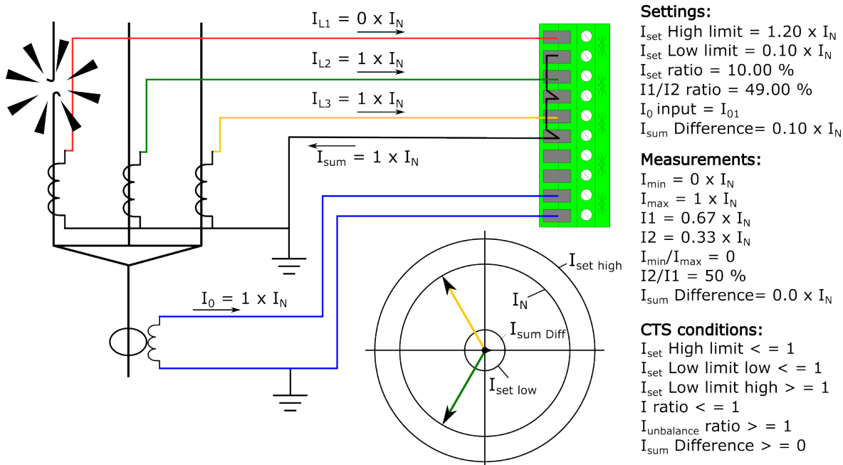
Figure. 5.6.1 - 217. Broken primary phase current wiring.
