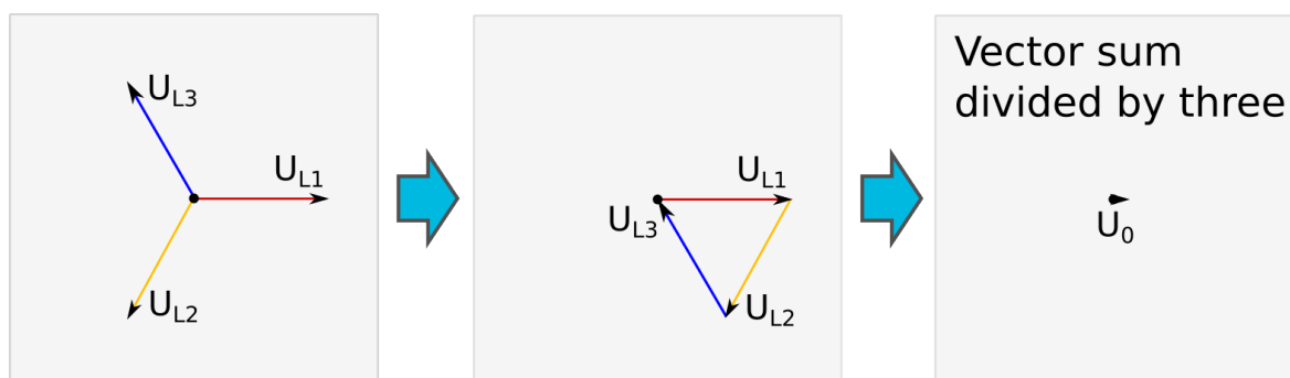
Figure. 5.4.12 - 125. Earth fault in isolated network.
