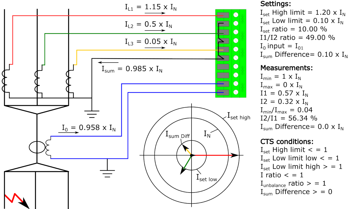
Figure. 5.6.1 - 218. Primary side high-impedance earth fault.
