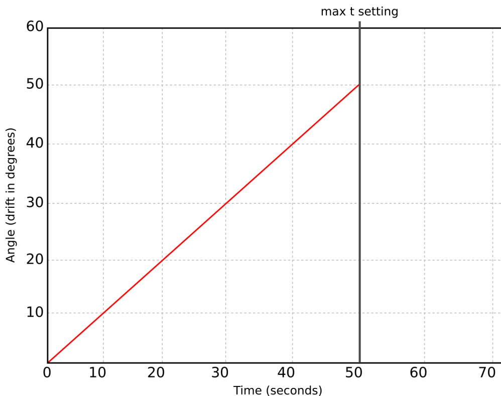
Figure. 5.4.22 - 165. Voltage angle drift.
