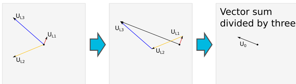
Figure. 5.4.12 - 126. Close-distance short-circuit between phases 1 and 3.
