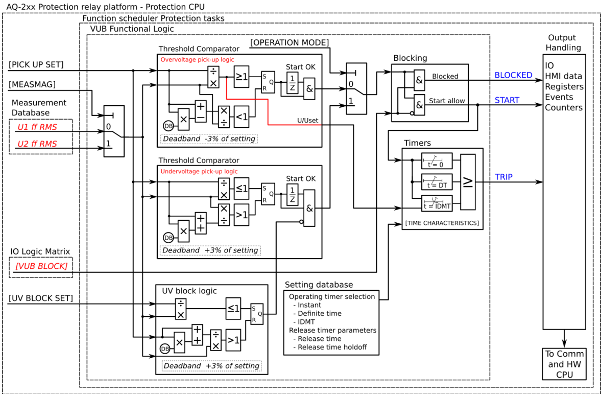
Figure. 5.4.13 - 134. Simplified function block diagram of the U1/U2>/< function.
