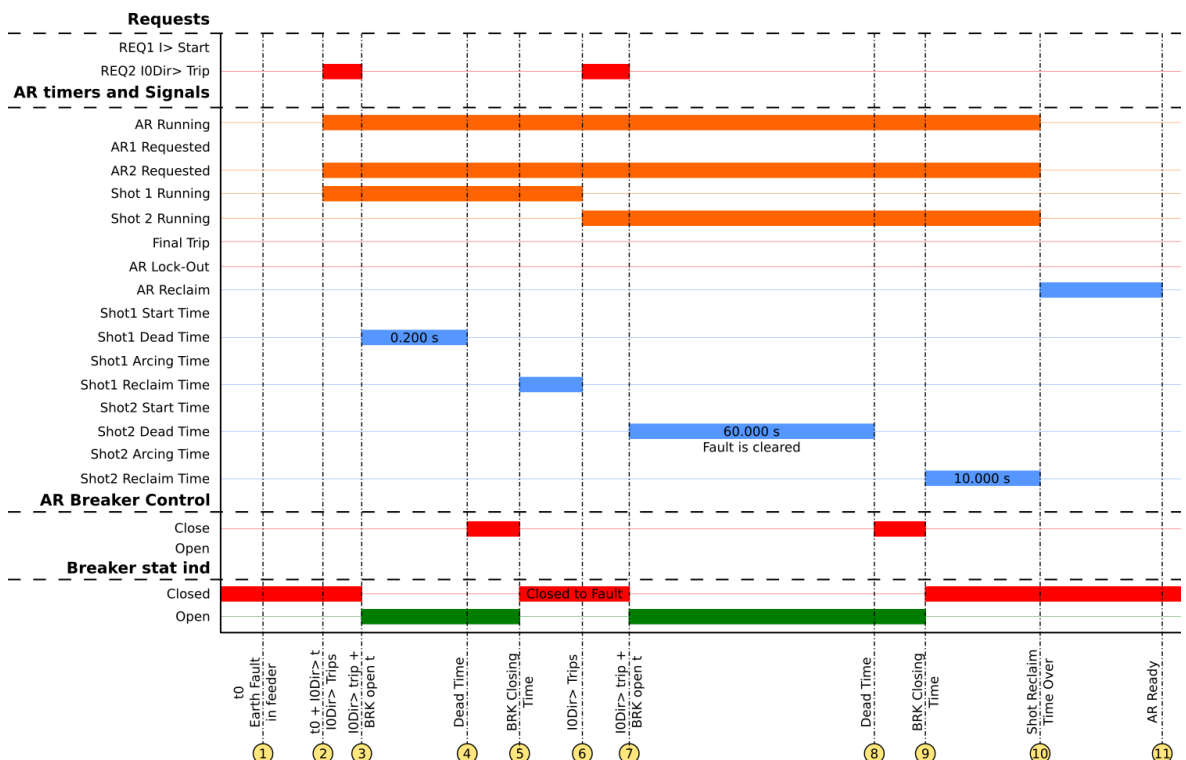
Figure. 5.5.5 - 181. Signal status graph of the semi-permanent earth fault auto-recloser cycle.
