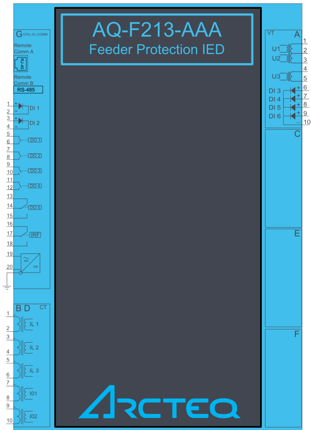
Figure. 7.1 - 229. AQ-F213 variant without add-on modules.
