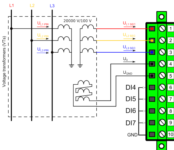
Figure. 5.2.2 - 66. Connections.
