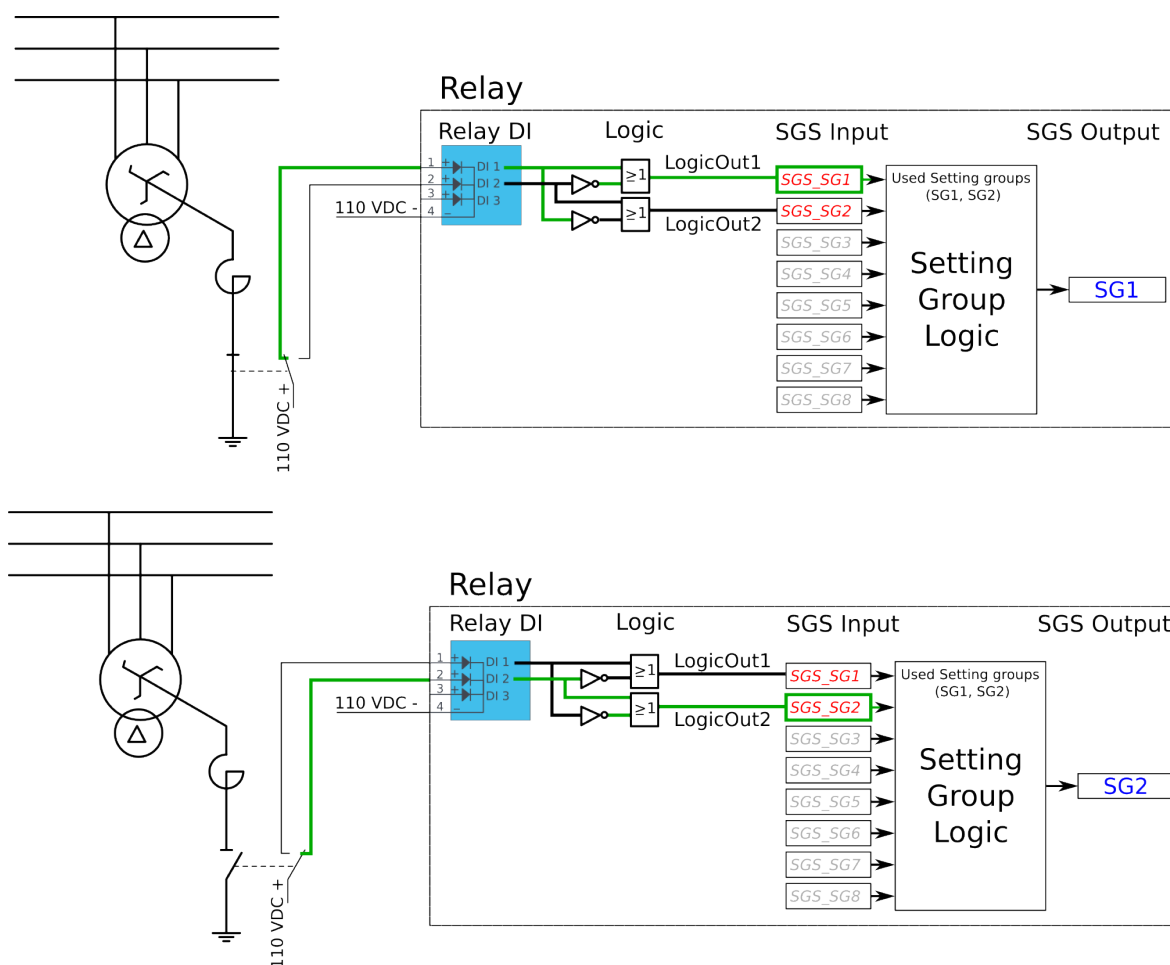
Figure. 5.5.2 - 171. Setting group control – two-wire connection from Petersen coil status with additional logic.
