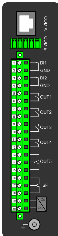
Figure. 8.2 - 241. CPU module.
