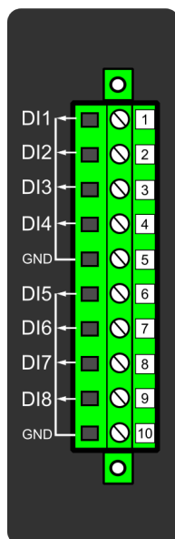
Figure. 8.5 - 244. Digital input module (DI8) with eight add-on digital inputs.
