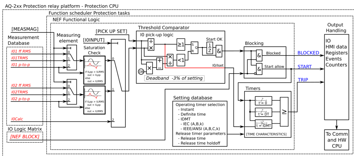
Figure. 5.4.3 - 87. Simplified function block diagram of the I0> fucntion.
