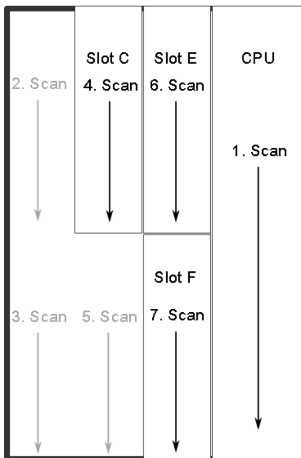
Figure. 8.1 - 240. AQ-X213 hardware scanning and I/O naming principles.
