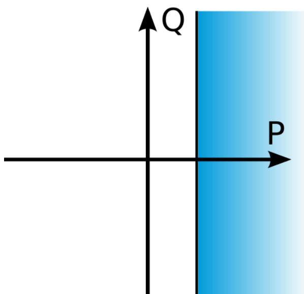
Figure. 5.4.16 - 140. Operating characteristics of overpower protection.
