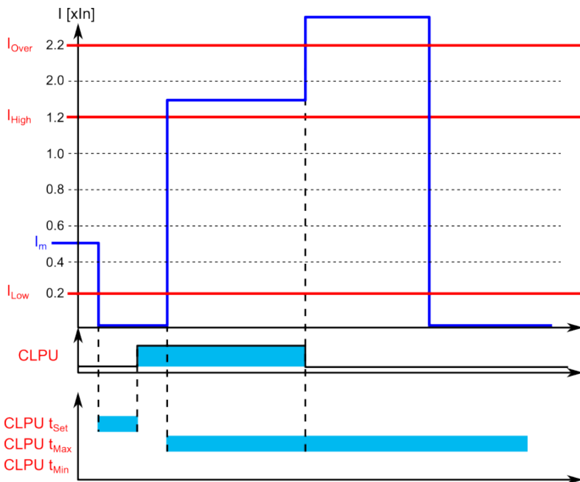
Figure. 5.5.6 - 196. Example of timers and pick-up parameters (activated pick-up and instant release due to overcurrent).
