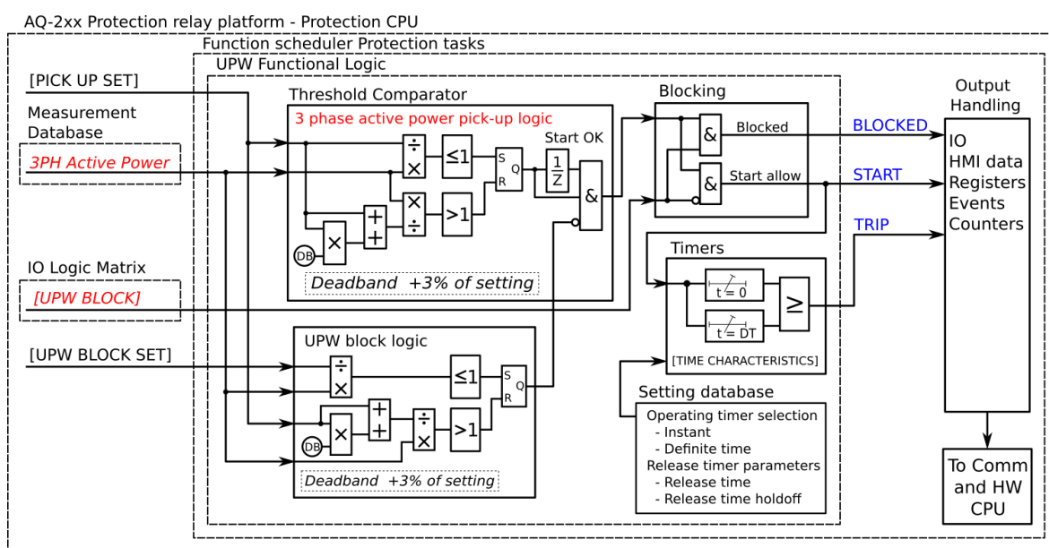
Figure. 5.4.17 - 143. Simplified function block diagram of the P< function.
