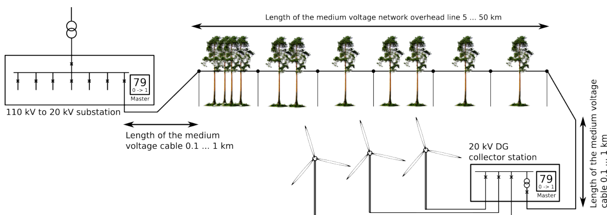
Figure. 5.5.5 - 190. Auto-reclosing with distributed generation in the line.
