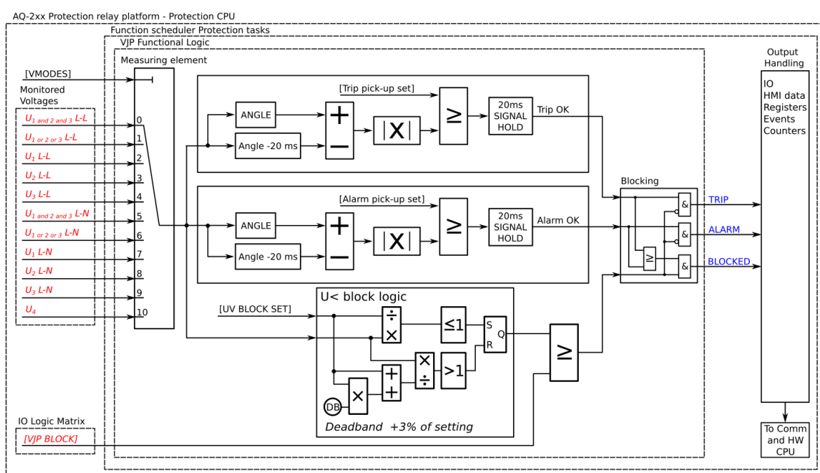
Figure. 5.5.9 - 202. Simplified function block diagram of the \Delta\phi function.
