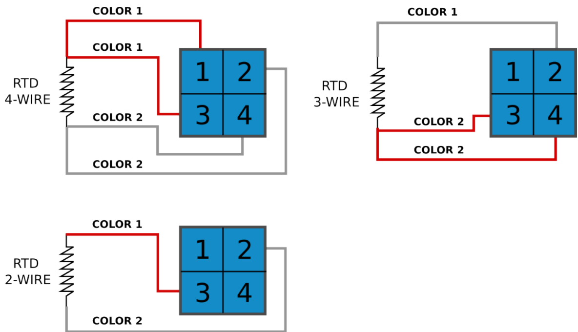
Figure. 8.8 - 249. RTD sensor connection types.
