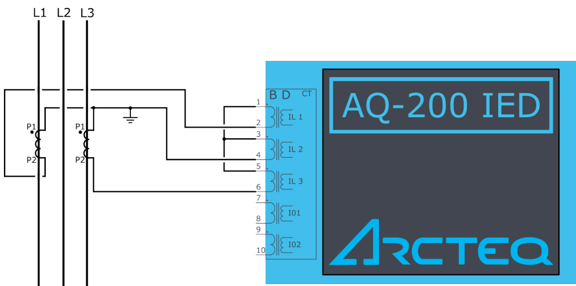
Figure. 7.3 - 233. ARON connection.
