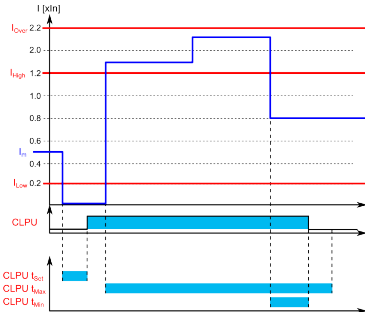
Figure. 5.5.6 - 194. Example of timers and pick-up parameters (normal CLPU situation).
