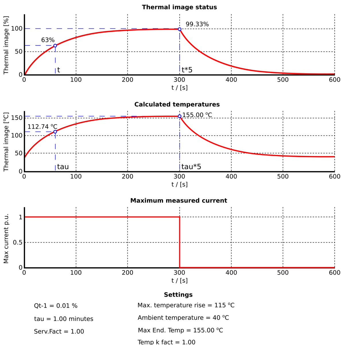
Figure. 5.4.19 - 147. Example of thermal image calculation with nominal conditions.
