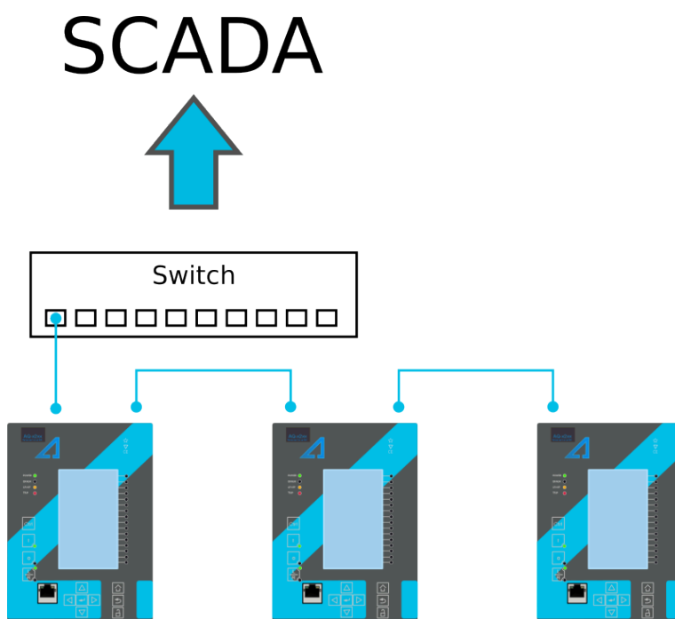
Figure. 8.12 - 256. Example of a multidrop configuration.
