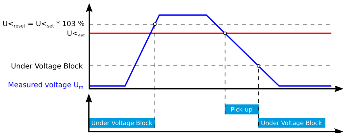
Figure. 5.4.11 - 123. Example of the block setting operation.
