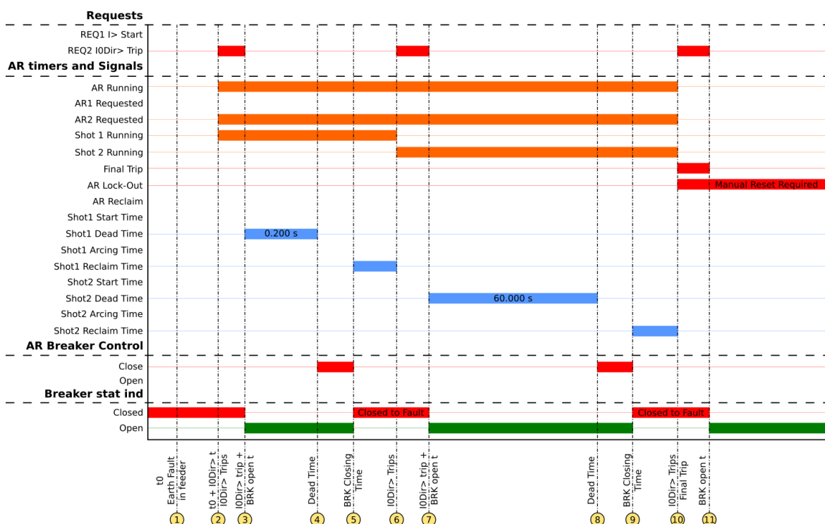
Figure. 5.5.5 - 179. Signal status graph of the permanent earth fault auto-recloser cycle.
