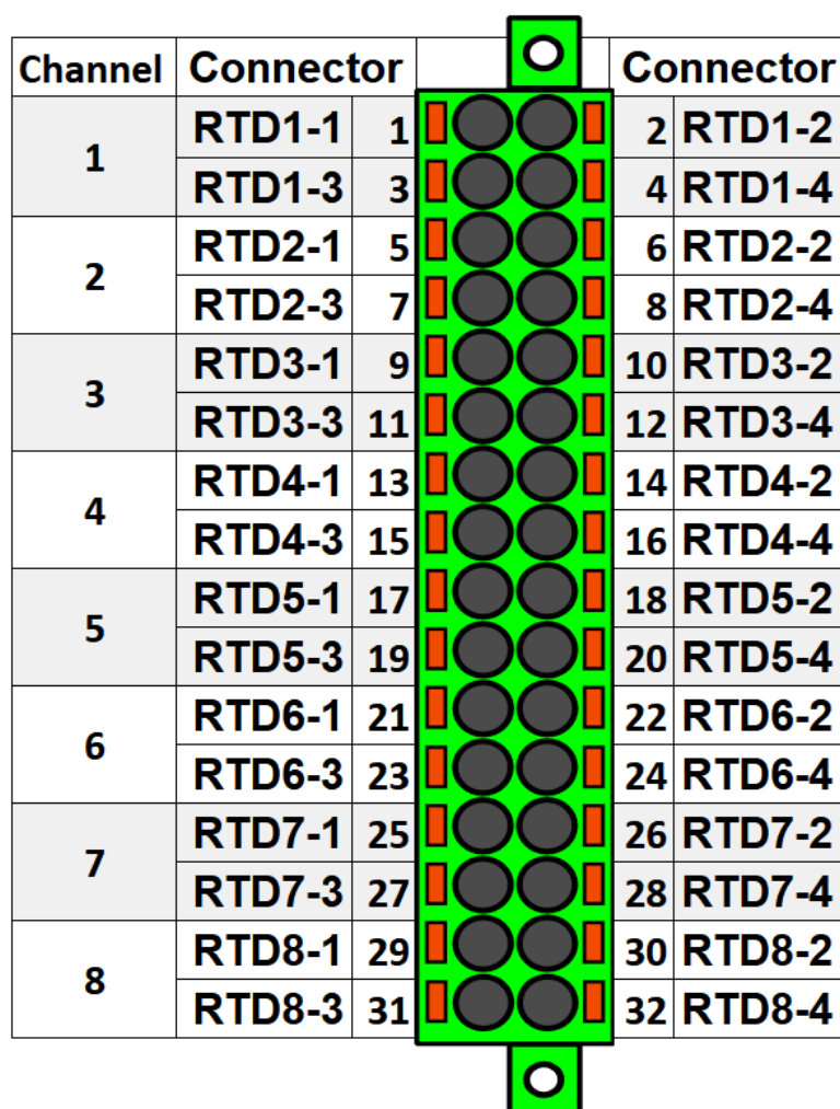
Figure. 8.8 - 248. RTD input module connectors.
