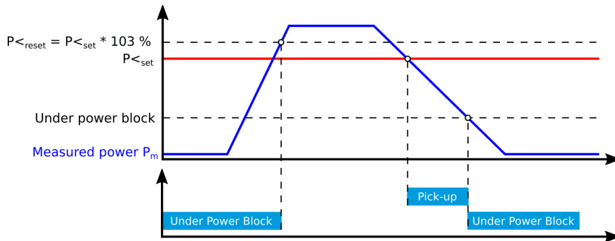
Figure. 5.4.17 - 144. Activation and deactivation characteristics of low power blocking.
