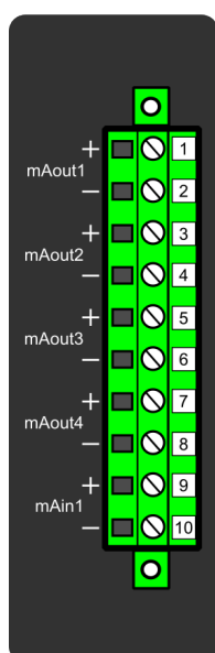
Figure. 8.13 - 257. Milliampere (mA) I/O module connections.
