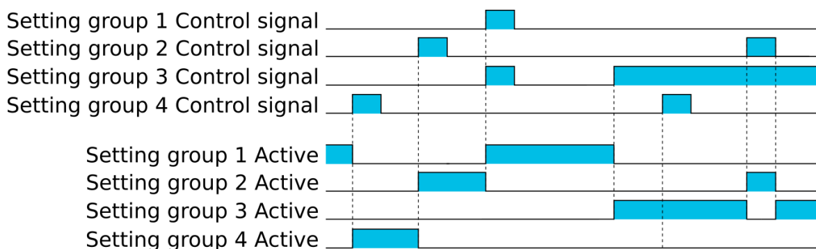
Figure. 5.5.2 - 168. Example sequences of group changing (control with pulse only, or with both pulses and static signals).
