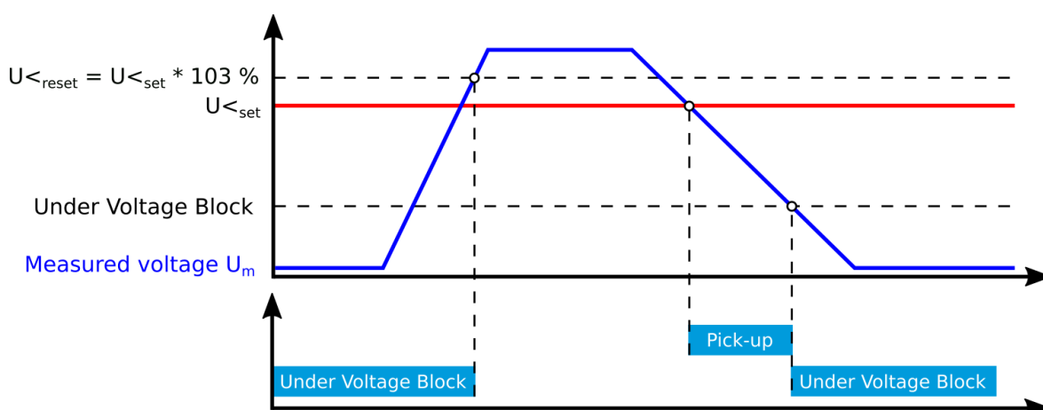
Figure. 5.4.13 - 135. Example of the block setting operation.
