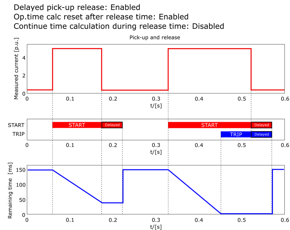
Figure. 5.4.1 - 84. Delayed pick-up release, delay counter value is held during the release time.
