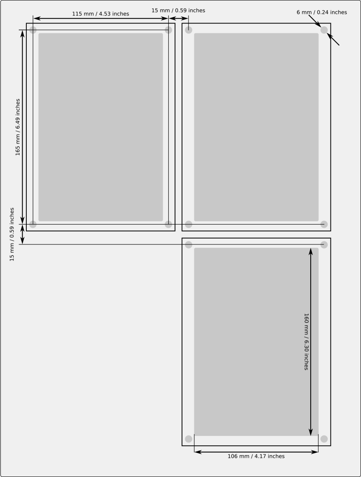
Figure. 8.14 - 260. Panel cutout dimensions and device spacing.
