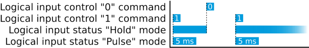
Figure. 5.5.13 - 206. Operation of logical input in "Hold" and "Pulse" modes.
