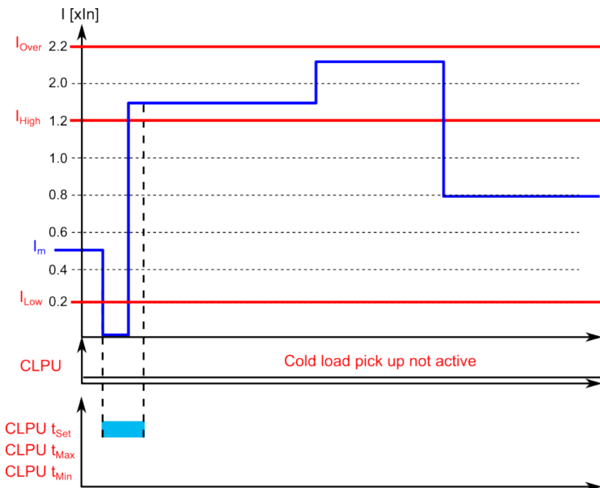
Figure. 5.5.6 - 195. Example of timers and pick-up parameters (no cold load pick-up, I_{low} too short).
