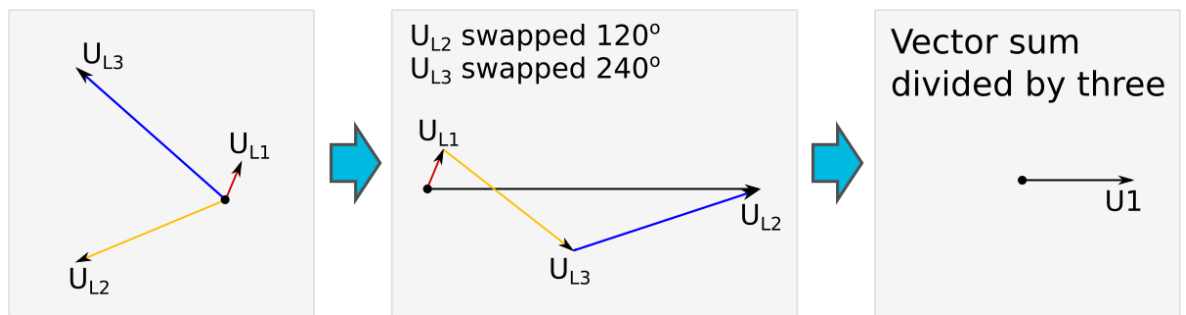
Figure. 5.4.13 - 130. Close-distance short-circuit between phases 1 and 3.
