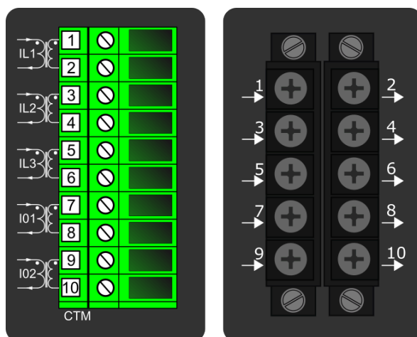
Figure. 8.3 - 242. Module connections with standard and ring lug terminals.
