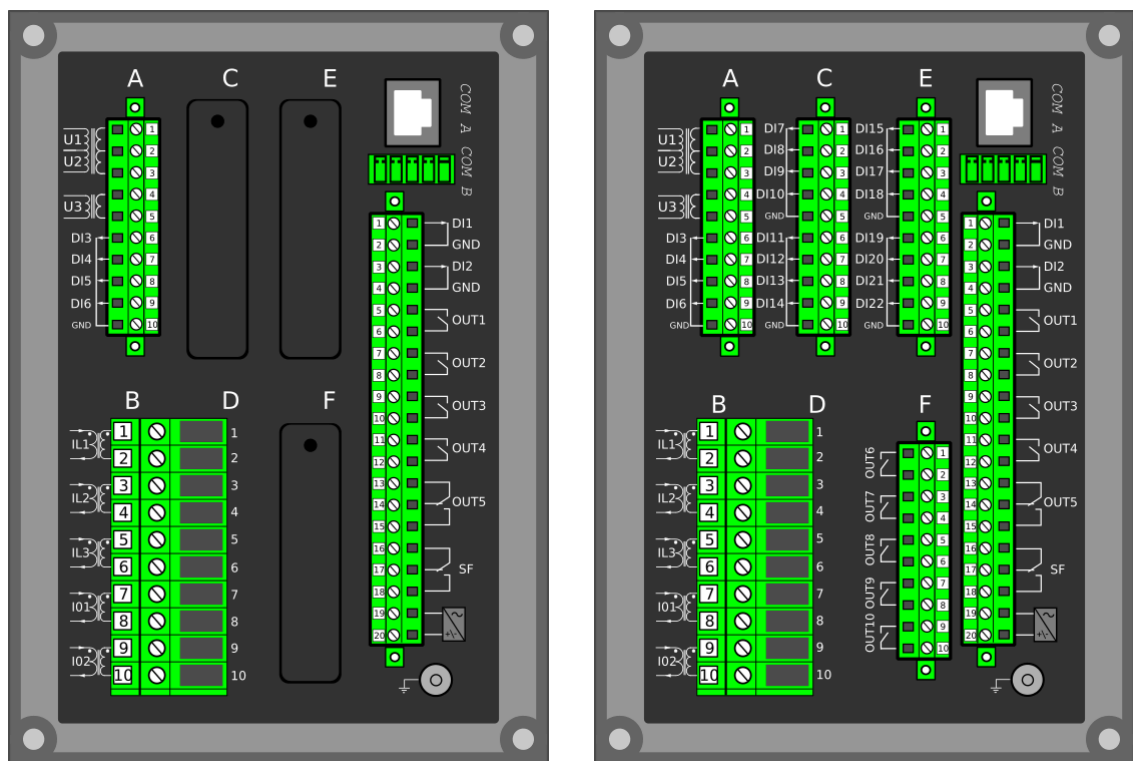
Figure. 8.1 - 239. Modular construction of AQ-X213.
