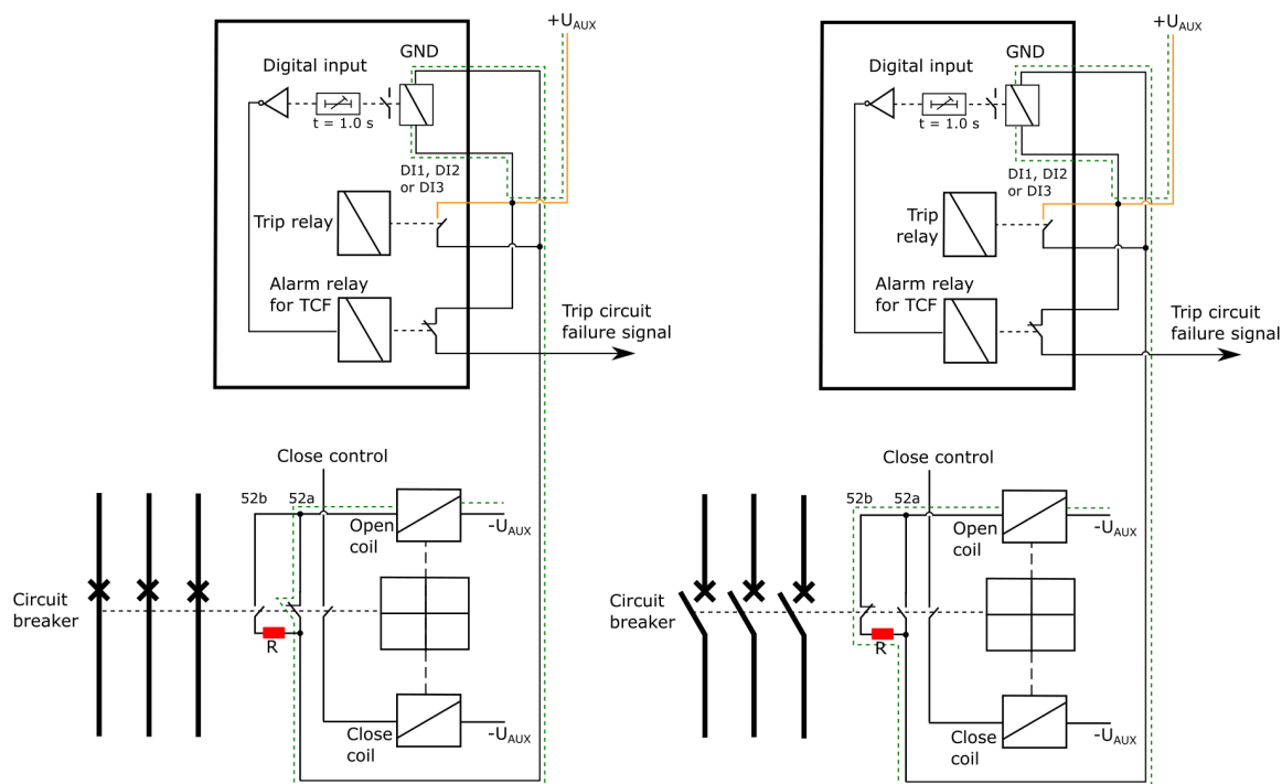
Figure. 7.4 - 234. Trip circuit supervision with one DI and one non-latched trip output.
