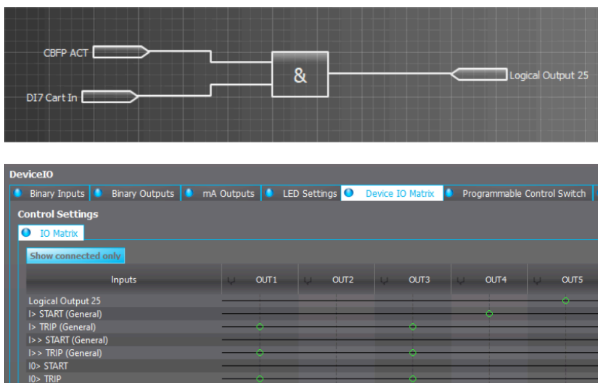
Figure. 5.5.12 - 205. Logic output example. Logical output is connected to an output relay in matrix.
