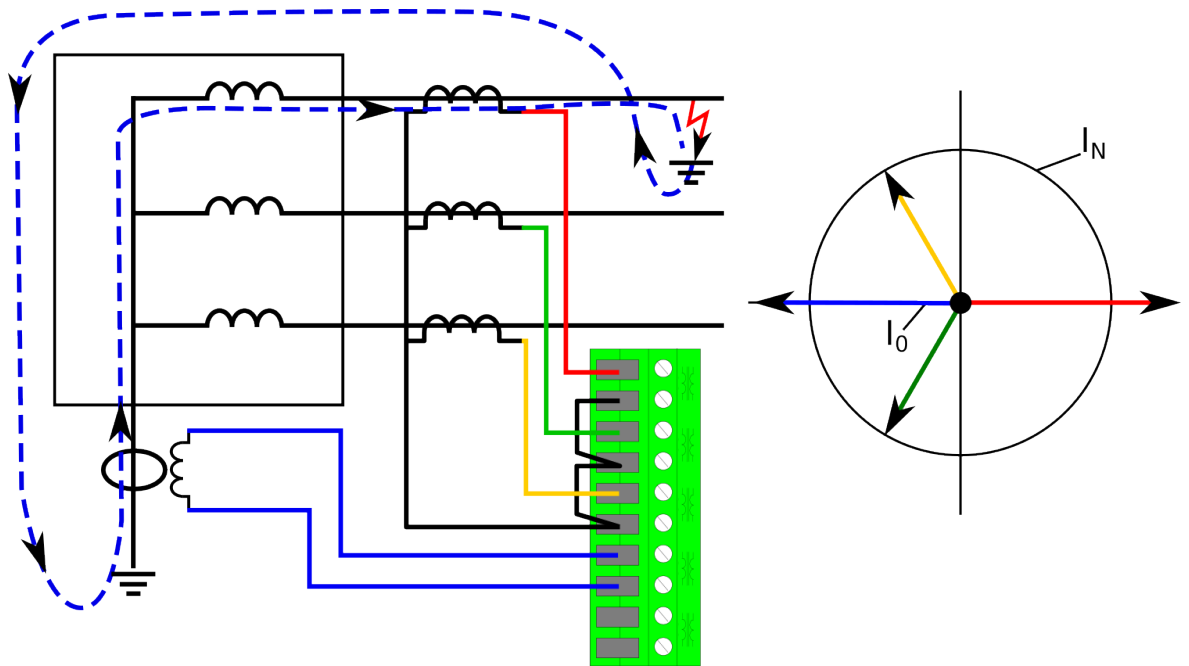
Figure. 5.4.9 - 119. Restricted earth fault outside a Y winding transformer.
