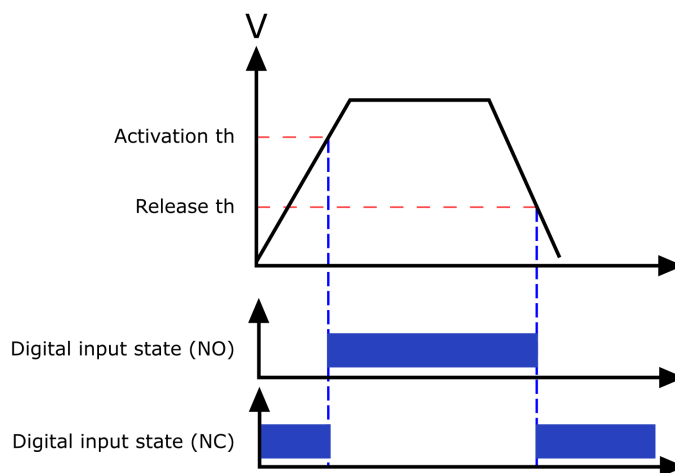
Figure. 8.5 - 245. Digital input state when energizing and de-energizing the digital input channels.
