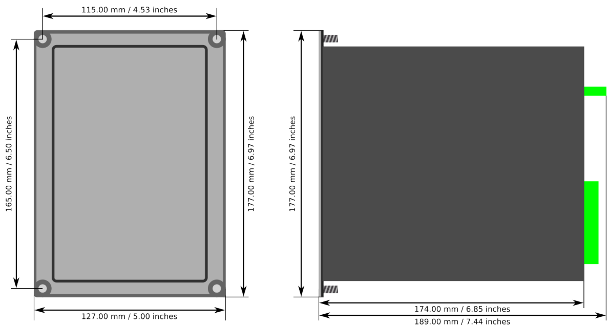
Figure. 8.14 - 258. Device dimensions.
