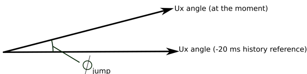
Figure. 5.5.9 - 204. Vector jump from the relay's point of view.
