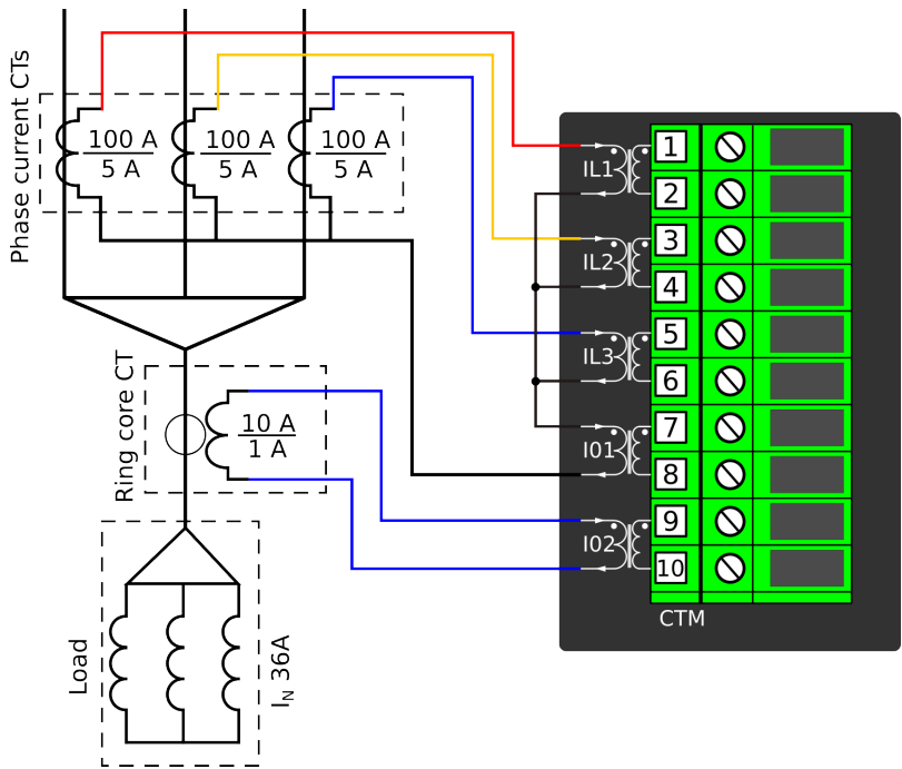
Figure. 5.2.1 - 55. Connections.
