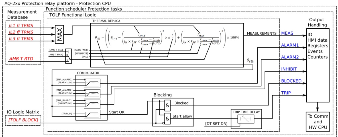
Figure. 5.4.19 - 159. Simplified function block diagram of the TF> function.
