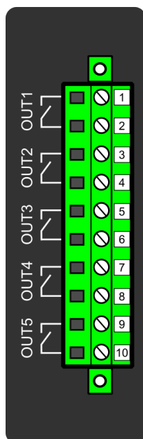
Figure. 8.6 - 246. Digital output module (DO5) with five add-on digital outputs.
