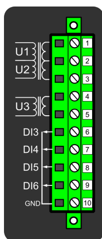
Figure. 8.4 - 243. Voltage measurement module.
