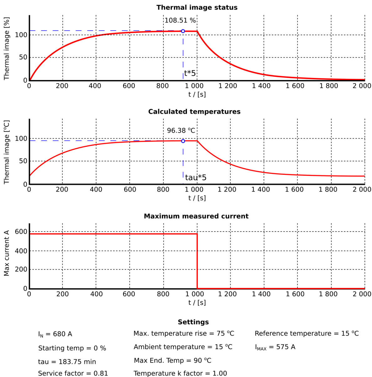
Figure. 5.4.19 - 157. Thermal image response with nominal currents and fine-tuned k_{\text{SF}} correction factor.
