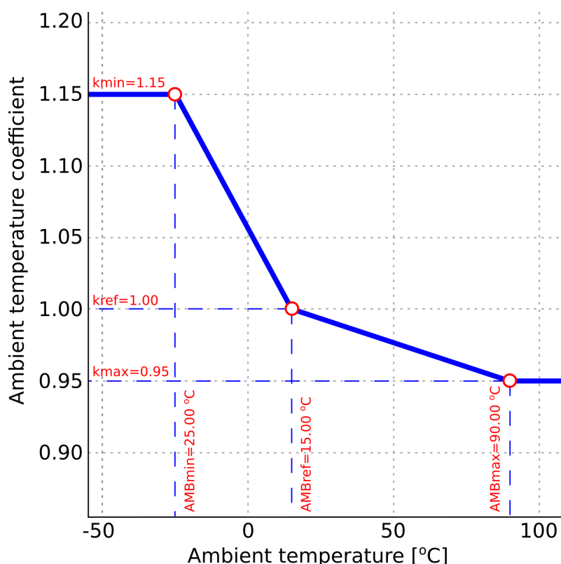
Figure. 5.4.21 - 160. Ambient temperature coefficient calculation (a three-point linear approximation and a settable correction curve).
