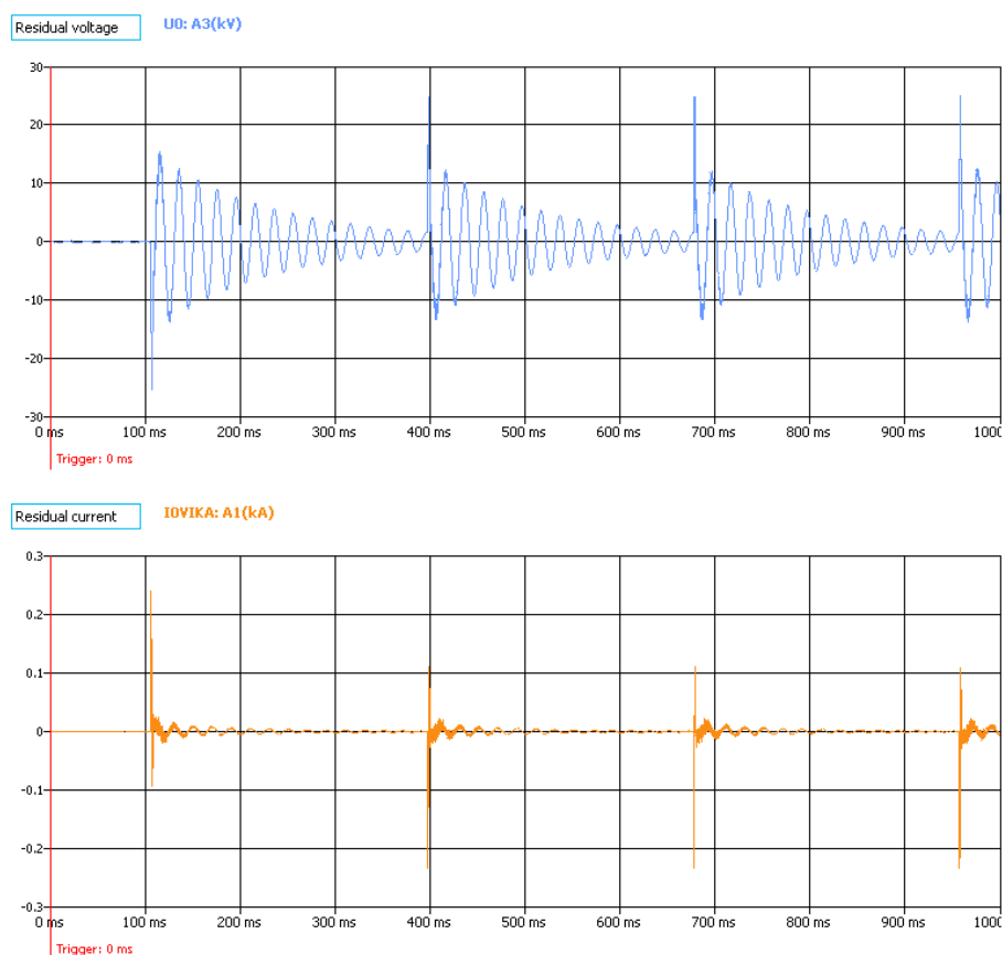
Figure. 5.4.6 - 98. An intermittent earth fault in a medium size network tuned close to resonance, as seen by a faulty feeder relay.
