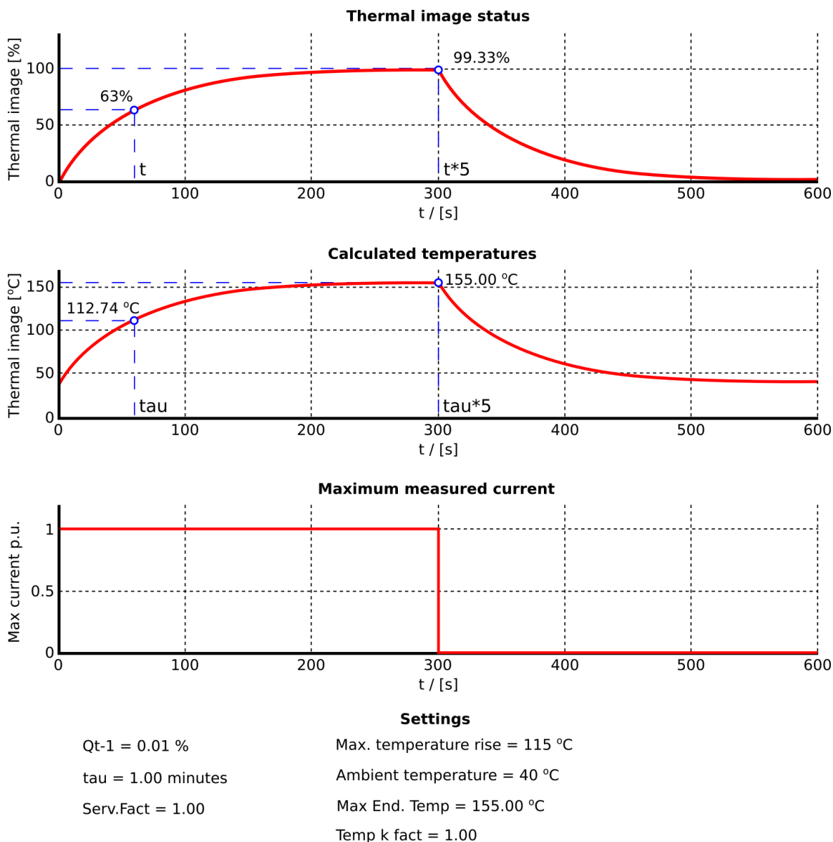
Figure. 5.4.21 - 159. Example of thermal image calculation with nominal conditions.
