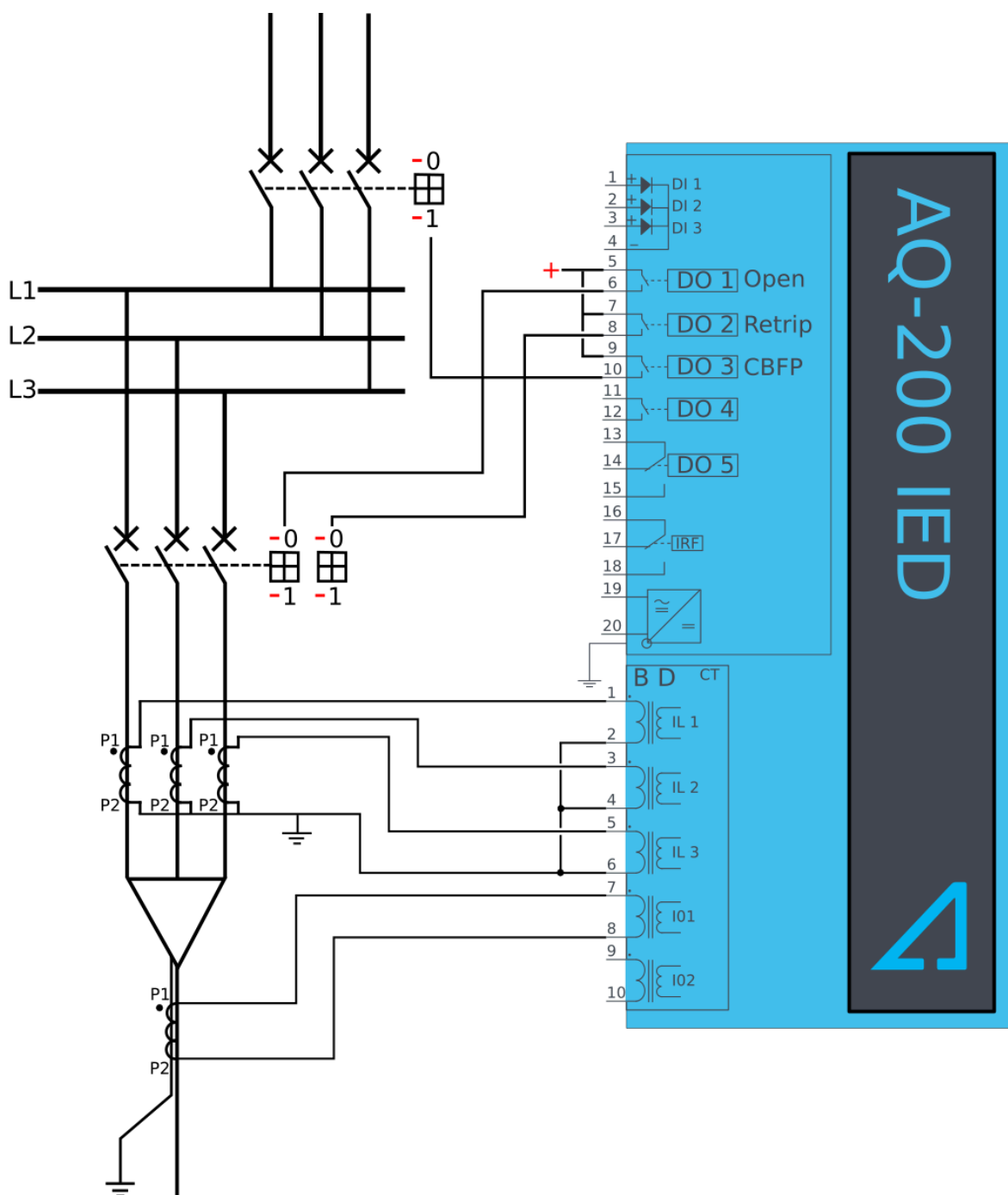
Figure. 5.4.9 - 106. Wiring diagram when Trip, Retrip and CBFP are configured to the device.
