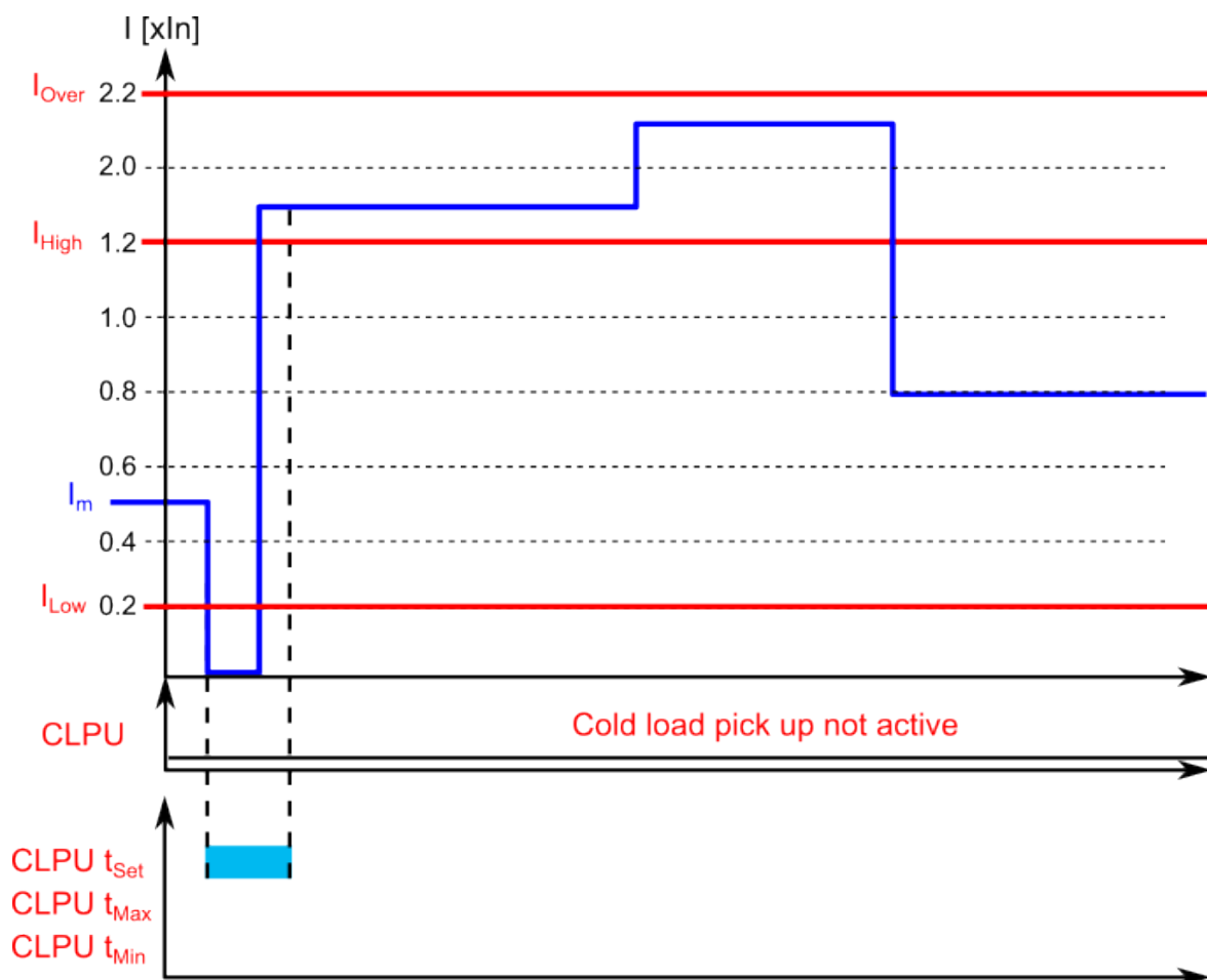
Figure. 5.5.7 - 208. Example of timers and pick-up parameters (no cold load pick-up, I_{low} too short).
