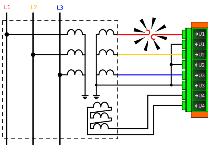
Figure. 5.6.2 - 242. Secondary circuit fault in phase L1 wiring.
