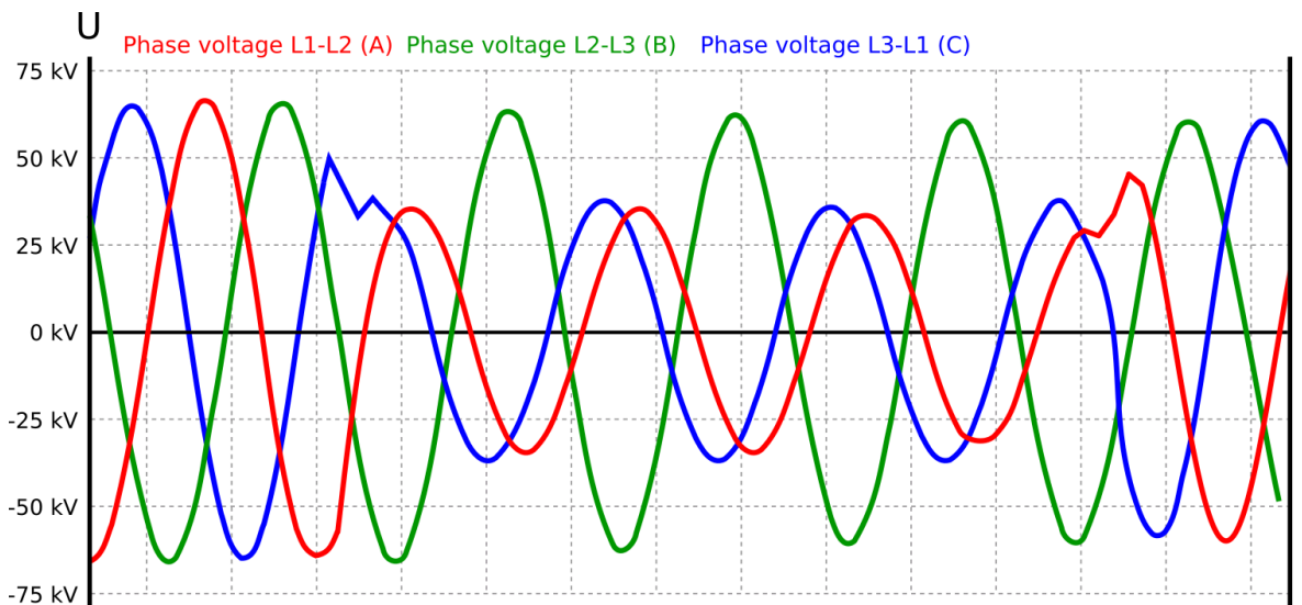
Figure. 5.5.11 - 226. Generator islanding.
