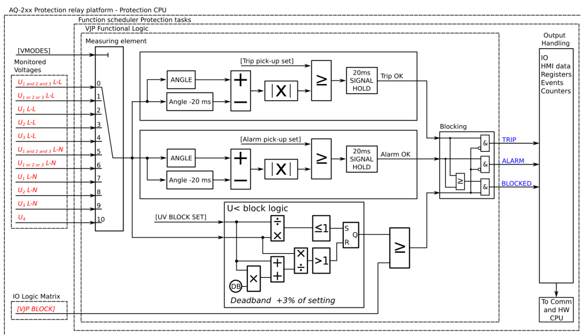
Figure. 5.5.11 - 225. Simplified function block diagram of the \Delta\phi function.
