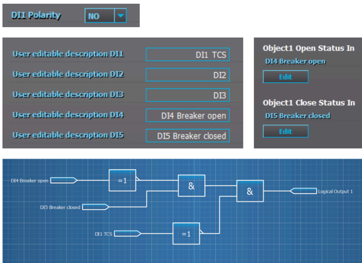
Figure. 7.4 - 261. Example block scheme.
