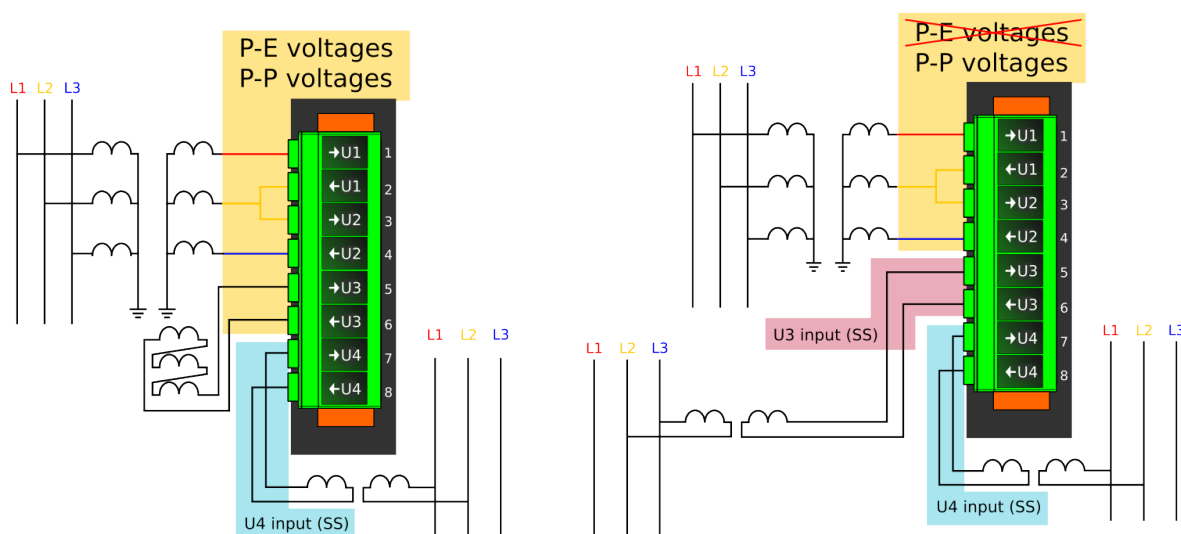
Figure. 5.4.11 - 128. Selectable measurement magnitudes with 2LL+U3+U4 VT connection (P-E voltages not available without residual voltage).
