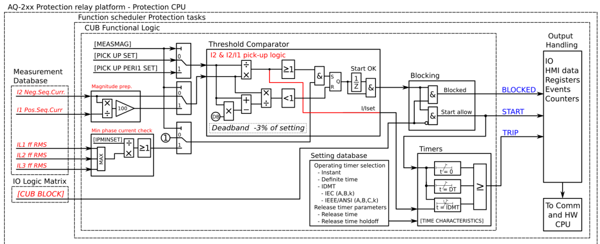
Figure. 5.4.7 - 102. Simplified function block diagram of the I2> function.
