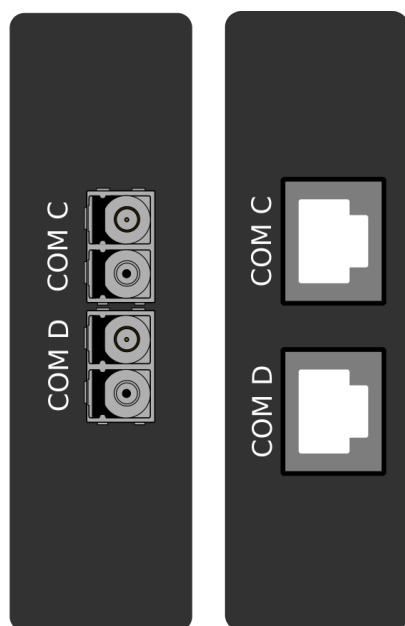
Figure. 8.10 - 274. LC and RJ45 100 Mbps Ethernet module connectors.
