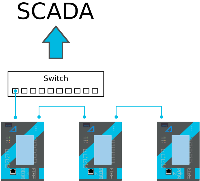
Figure. 8.12 - 279. Example of a multidrop configuration.
