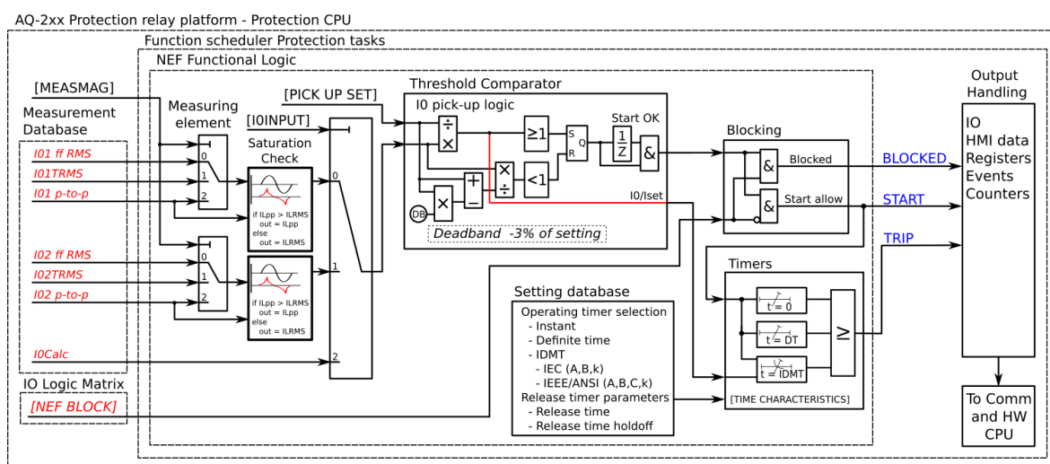
Figure. 5.4.3 - 87. Simplified function block diagram of the I0> function.
