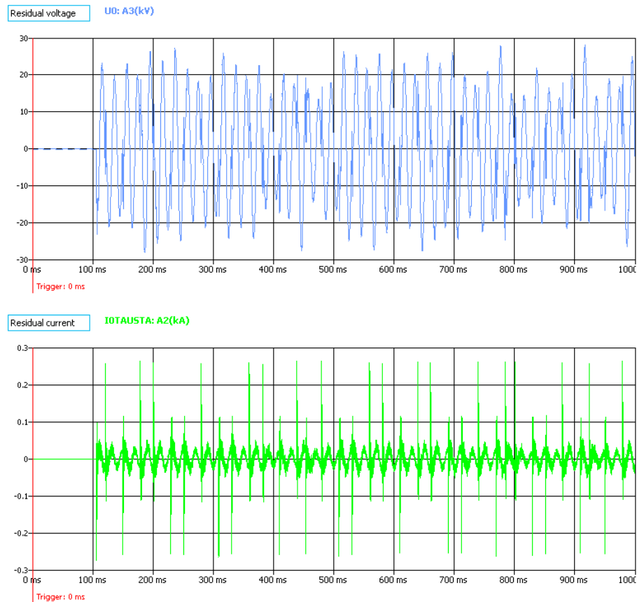
Figure. 5.4.6 - 101. Undercompensated medium size network intermittent earth fault seen by healthy feeder relay.
