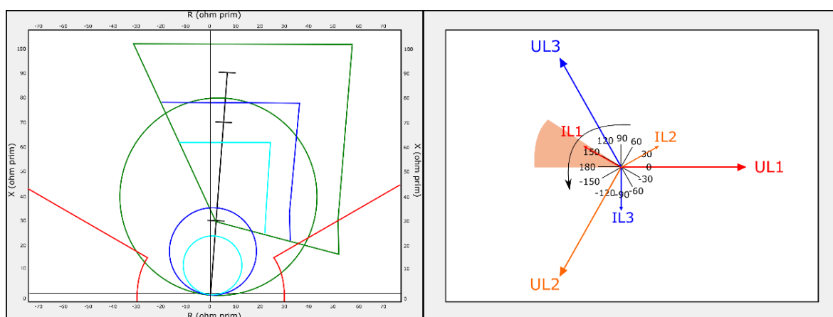
Figure. 5.4.24 - 176. Distance protection characteristics and directional overcurrent.
