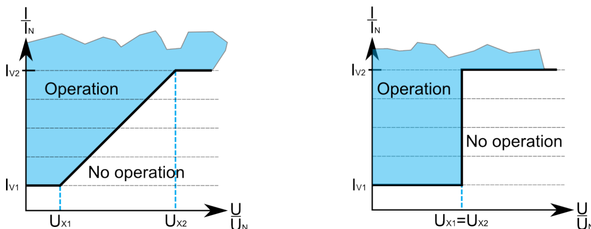
Figure. 5.4.20 - 157. Pick-up levels in the two modes.
