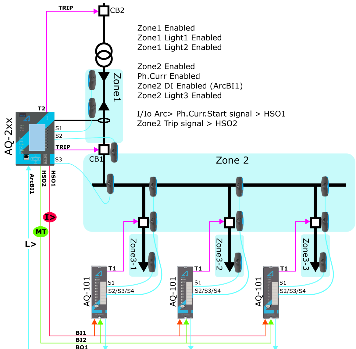
Figure. 5.4.23 - 174. Scheme IA1 (with AQ-101 arc protection relays).
