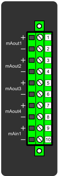
Figure. 8.13 - 280. Milliampere (mA) I/O module connections.
