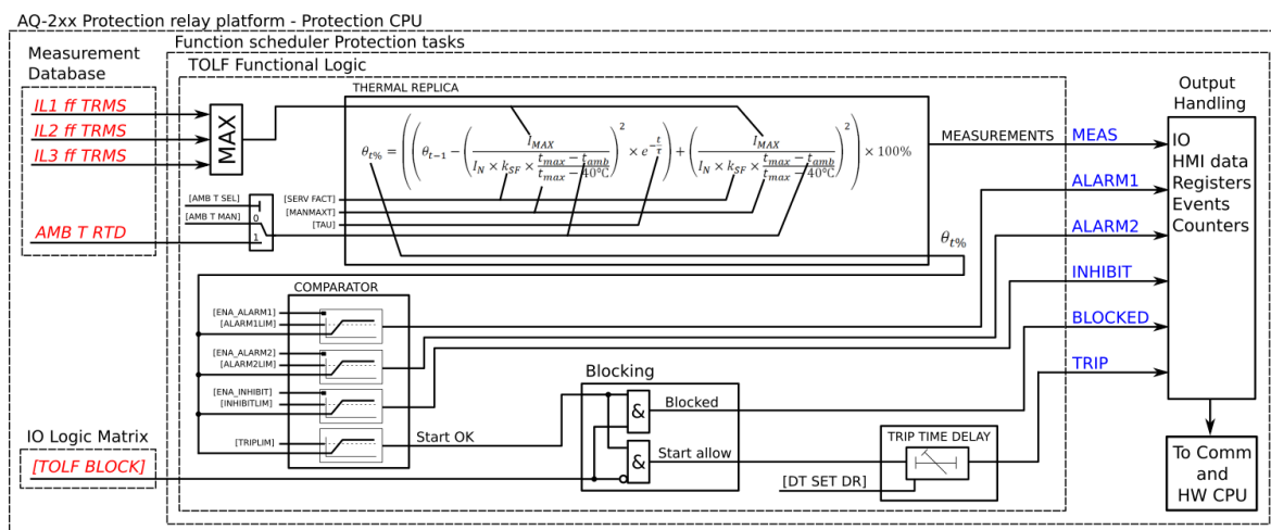
Figure. 5.4.21 - 171. Simplified function block diagram of the TF> function.
