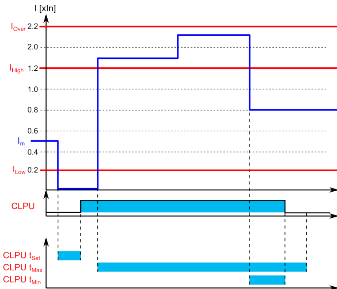
Figure. 5.5.7 - 207. Example of timers and pick-up parameters (normal CLPU situation).
