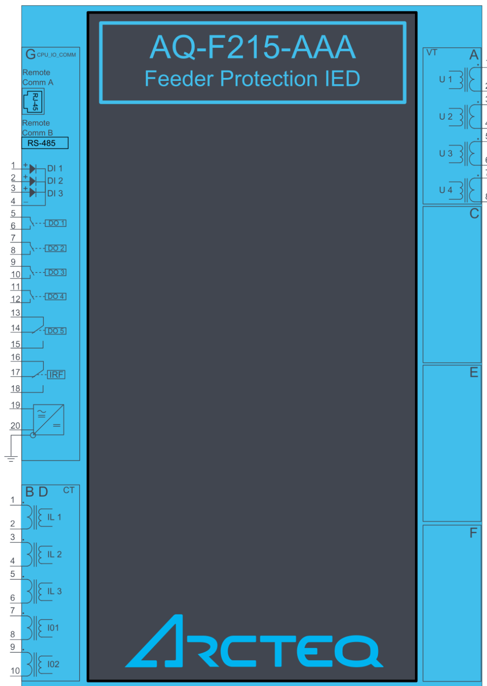
Figure. 7.1 - 252. AQ-F215 variant without add-on modules.
