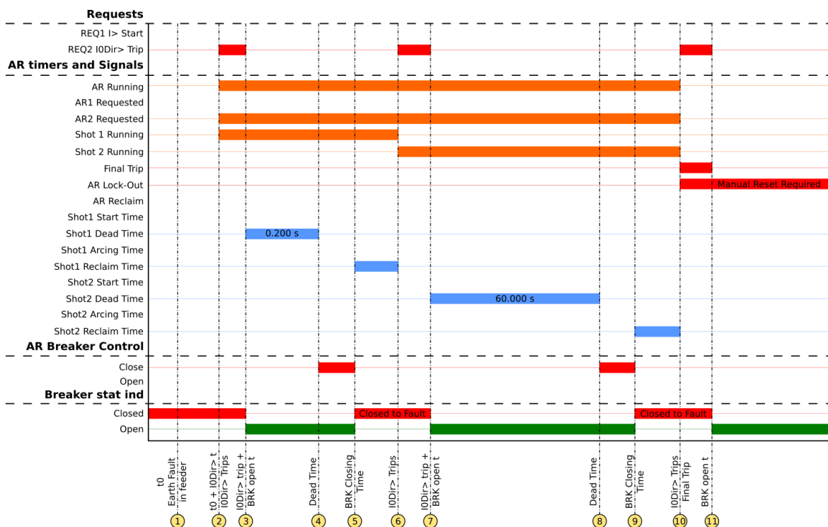
Figure. 5.5.5 - 191. Signal status graph of the permanent earth fault auto-recloser cycle.
