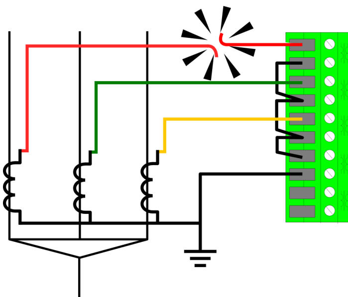
Figure. 5.6.1 - 231. Secondary circuit fault in phase L1 wiring.
