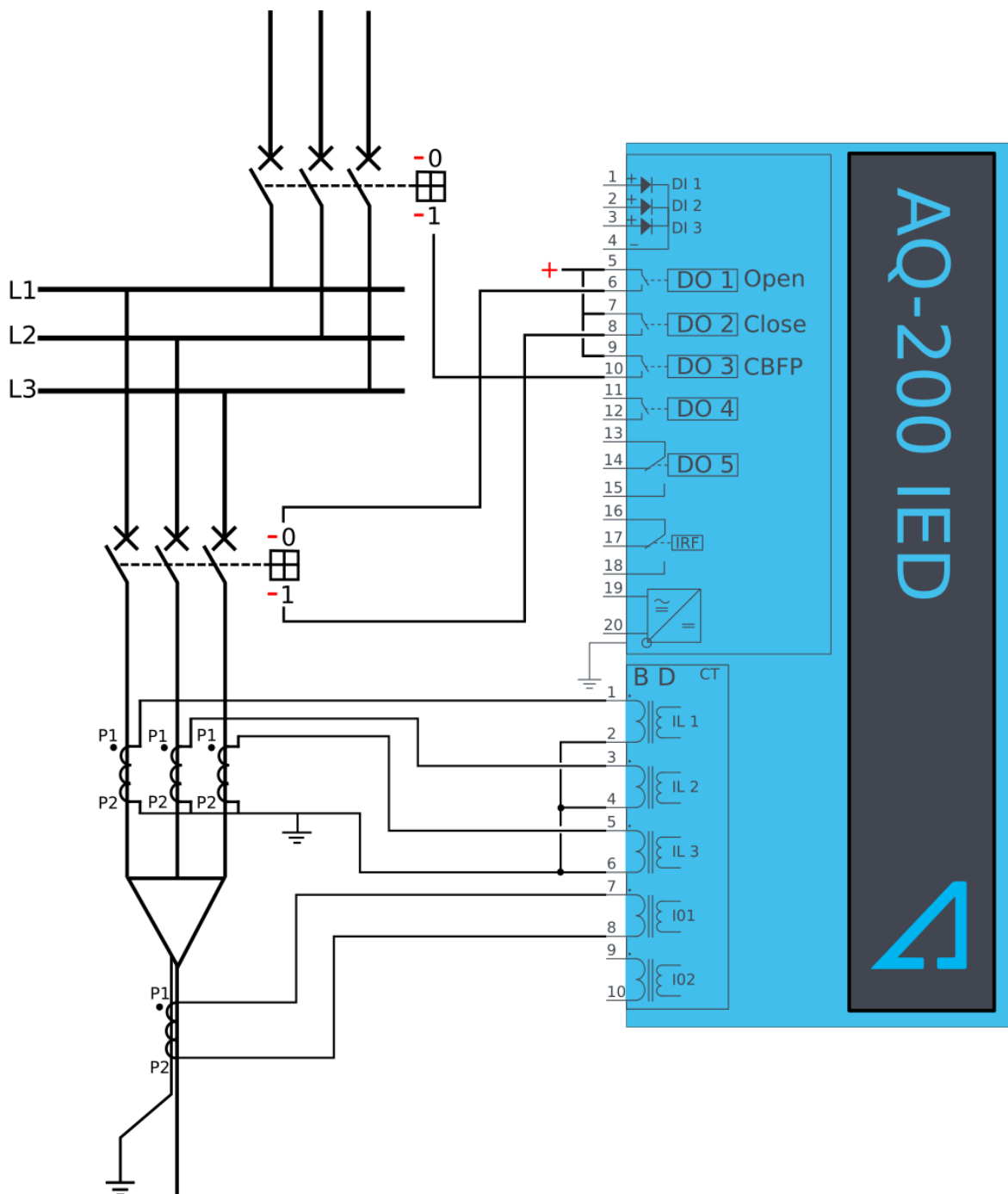
Figure. 5.4.9 - 110. Wiring diagram when Trip and CBFP are configured to the device.
