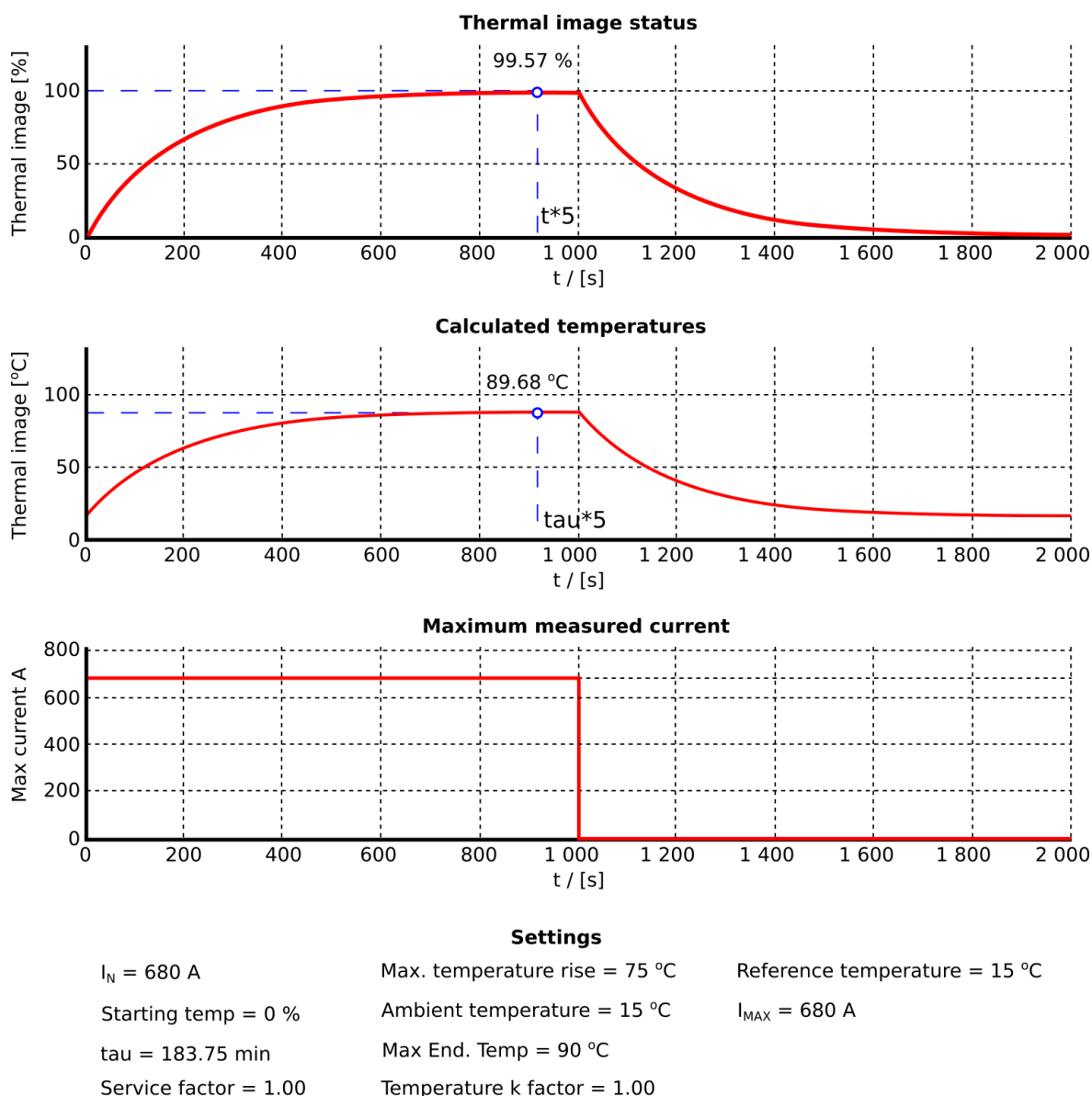
Figure. 5.4.21 - 168. Thermal image response with maximum load (installation according presumptions).
