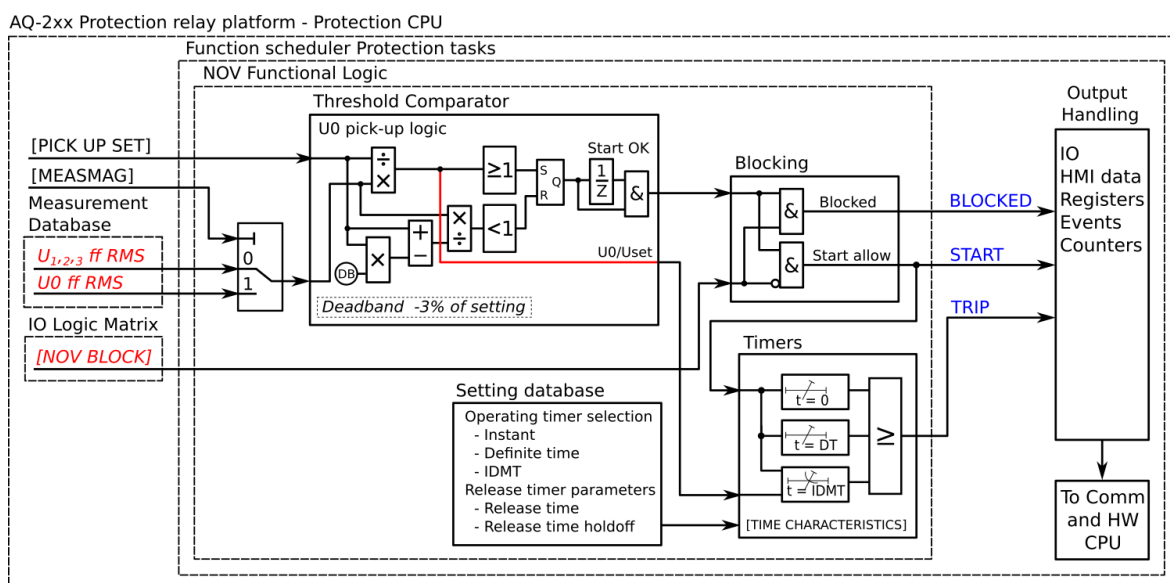
Figure. 5.4.13 - 137. Simplified function block diagram of the U0> function.
