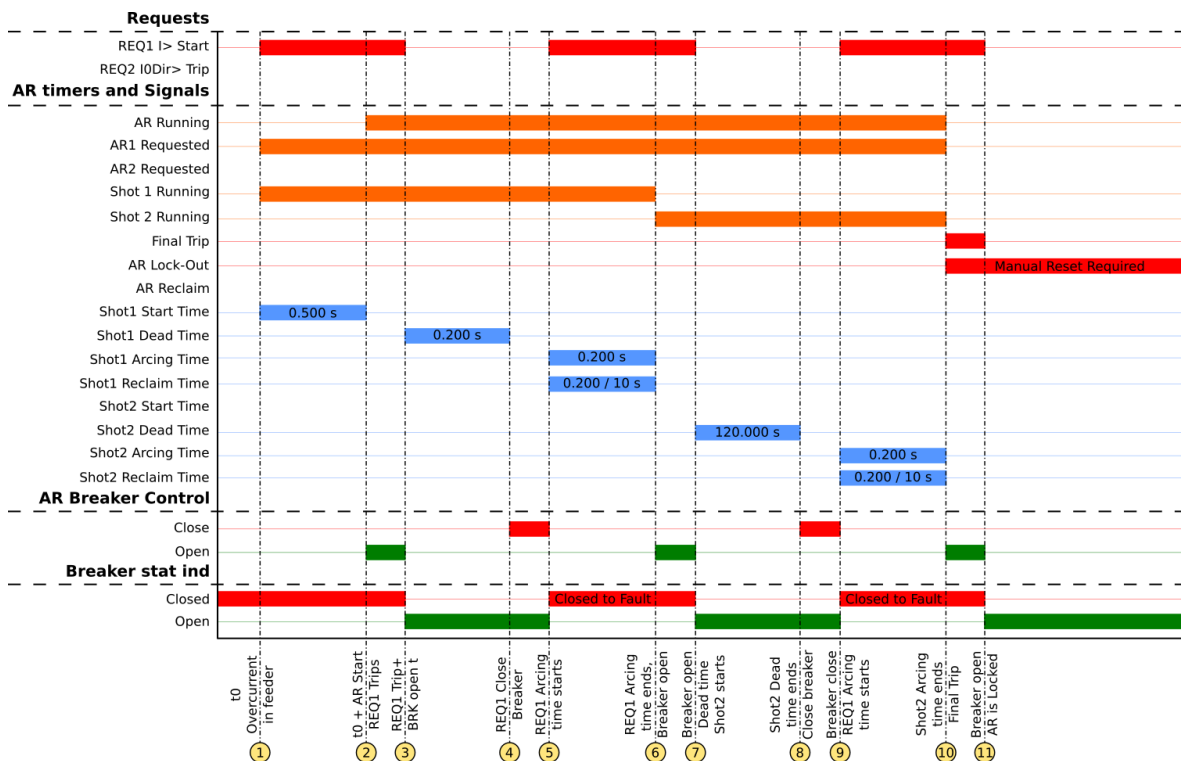
Figure. 5.5.5 - 197. Signal status graph of the permanent overcurrent auto-recloser cycle.
