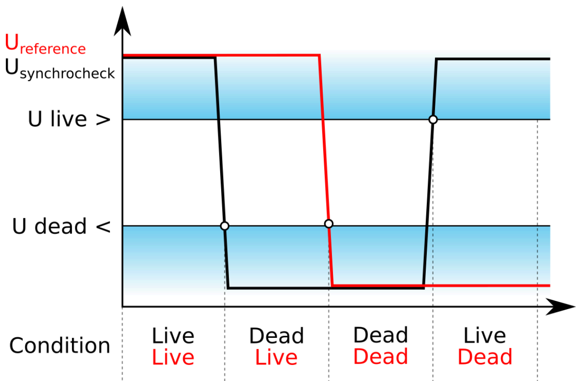
Figure. 5.5.9 - 221. System states.
