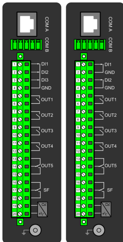
Figure. 8.2 - 264. CPU module.
