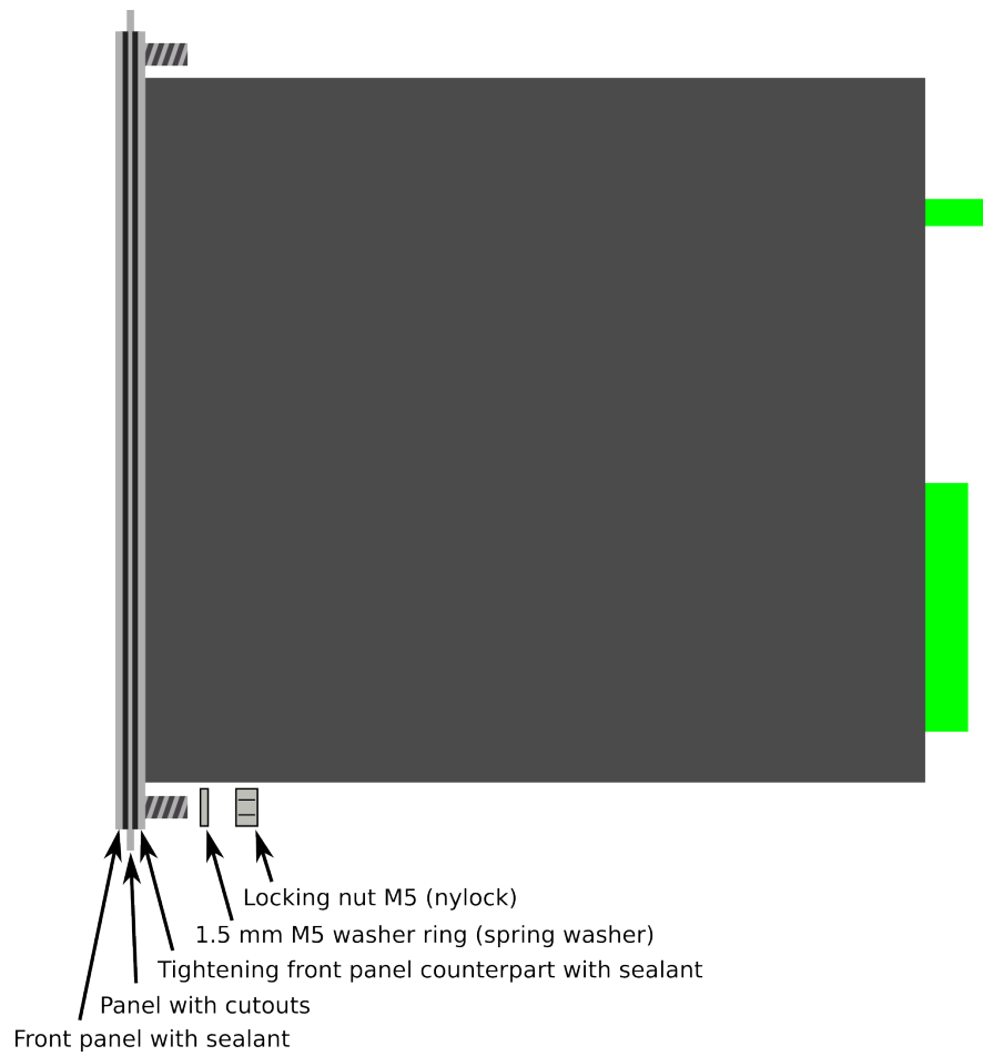
Figure. 8.14 - 282. Device installation.
