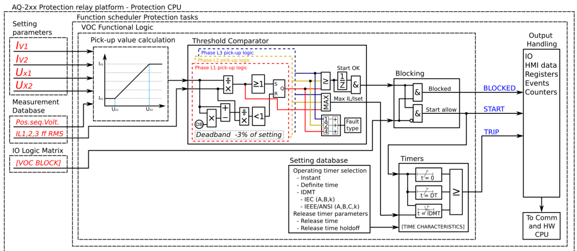
Figure. 5.4.20 - 158. Simplified function block diagram of the I_v > function.
