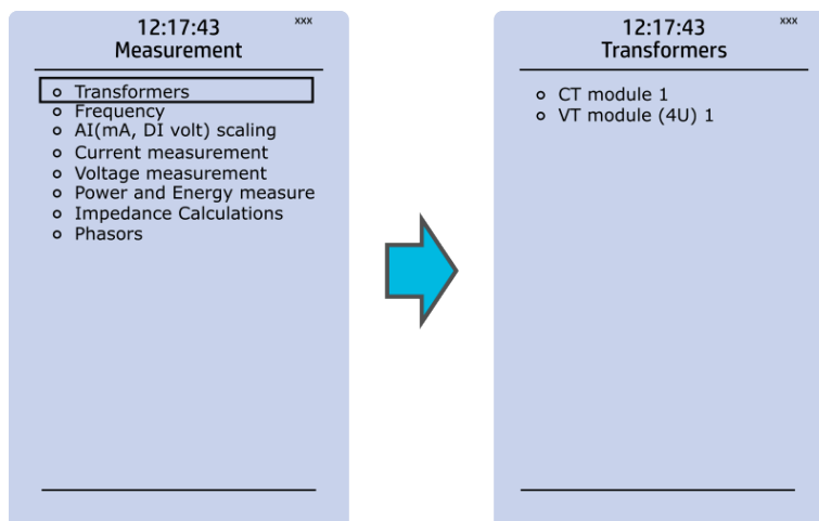
Figure. 4.7 - 41. Transformers section.
