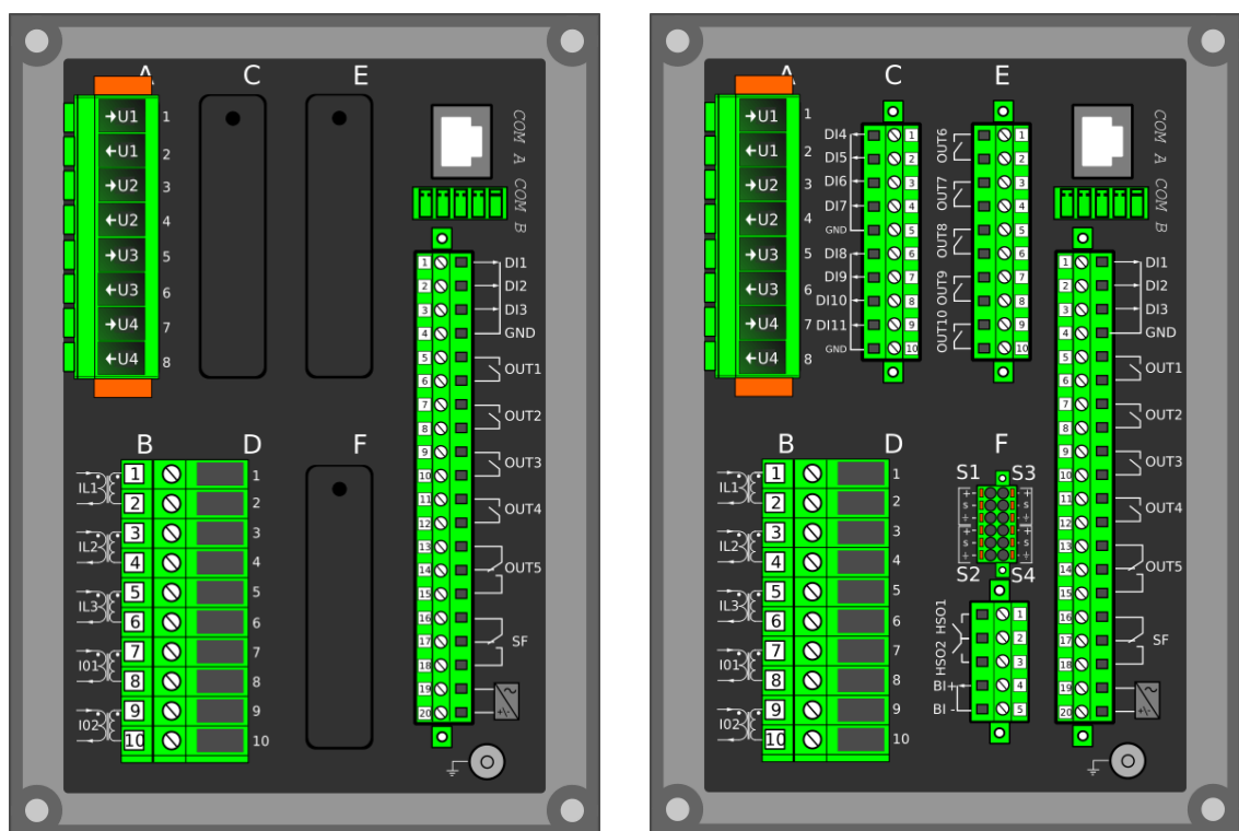
Figure. 8.1 - 262. Modular construction of AQ-X215.
