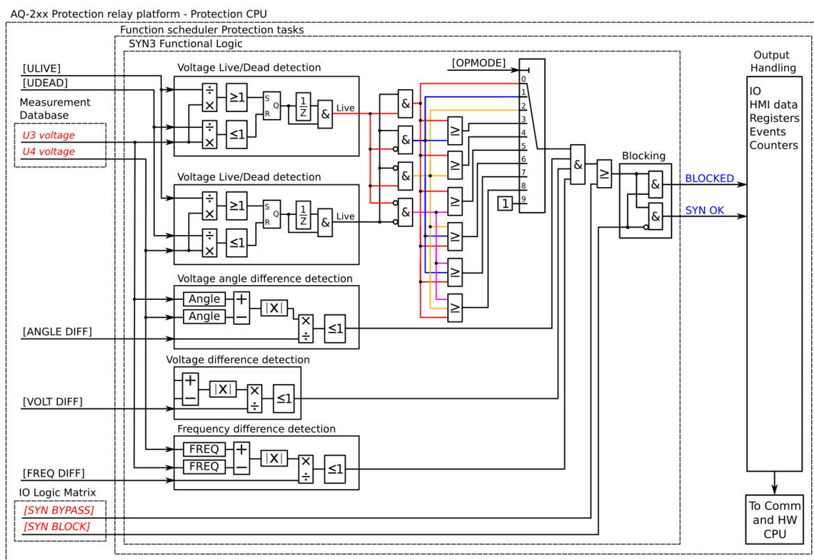
Figure. 5.5.9 - 223. Simplified function block diagram of the SYN3 function.
