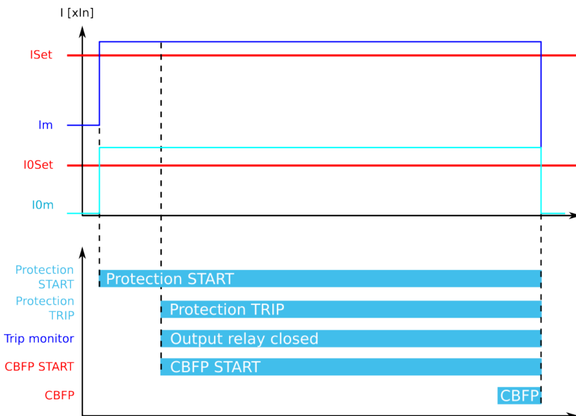
Figure. 5.4.9 - 112. CBFP when "Current and DO" is the selected criterion.
