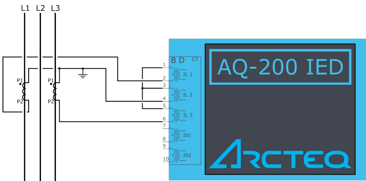
Figure. 7.3 - 256. ARON connection.
