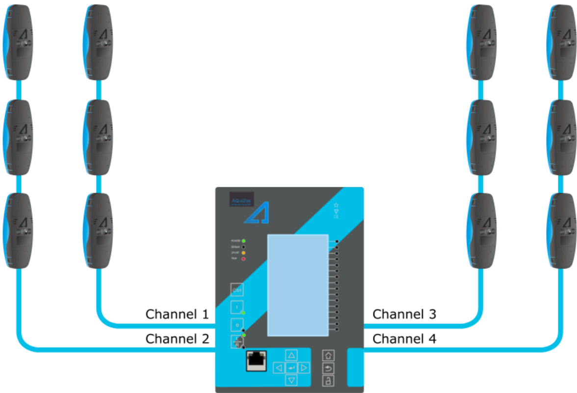
Figure. 5.4.23 - 173. IED equipped with arc protection.
