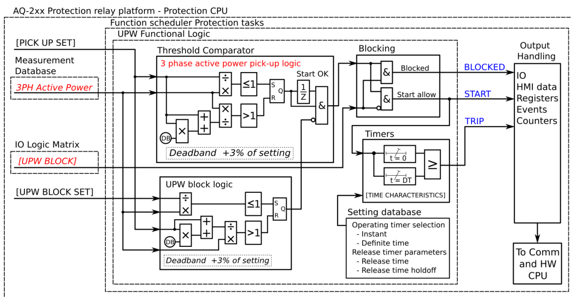
Figure. 5.4.18 - 153. Simplified function block diagram of the P< function.
