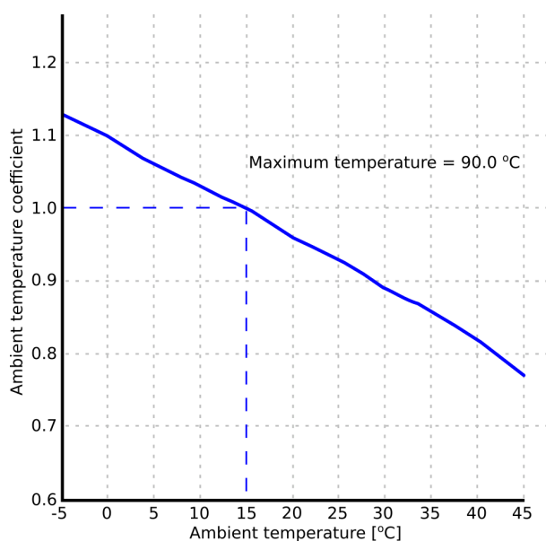
Figure. 5.4.21 - 163. Set correction curve for ambient temperature.
