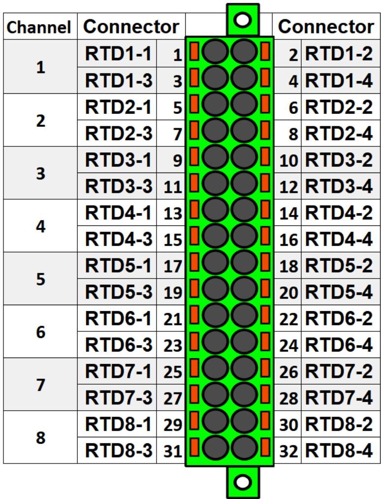
Figure. 8.8 - 271. RTD input module connectors.
