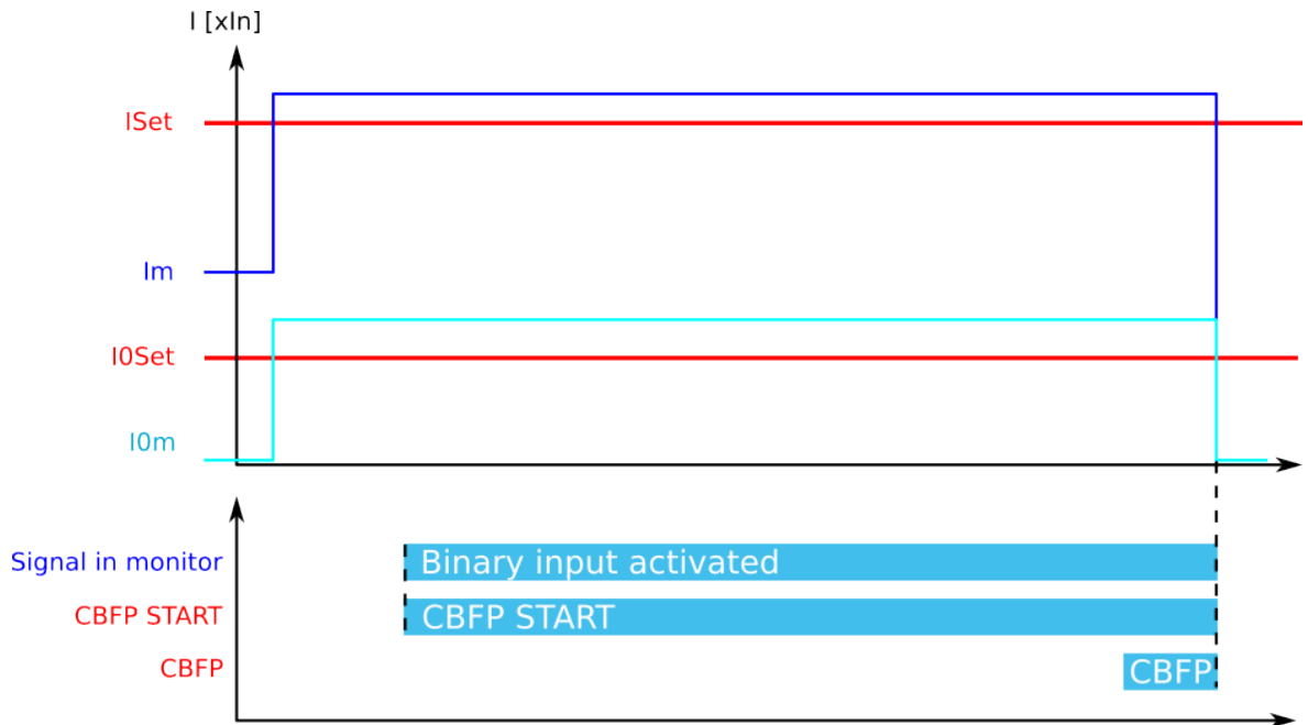
Figure. 5.4.9 - 115. Dedicated CBFP operation from digital input signal.
