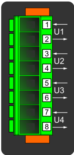
Figure. 8.4 - 266. Voltage measurement module.
