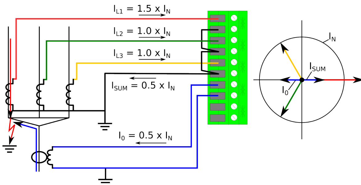
Figure. 5.4.10 - 122. Cable end differential when a fault occurs.
