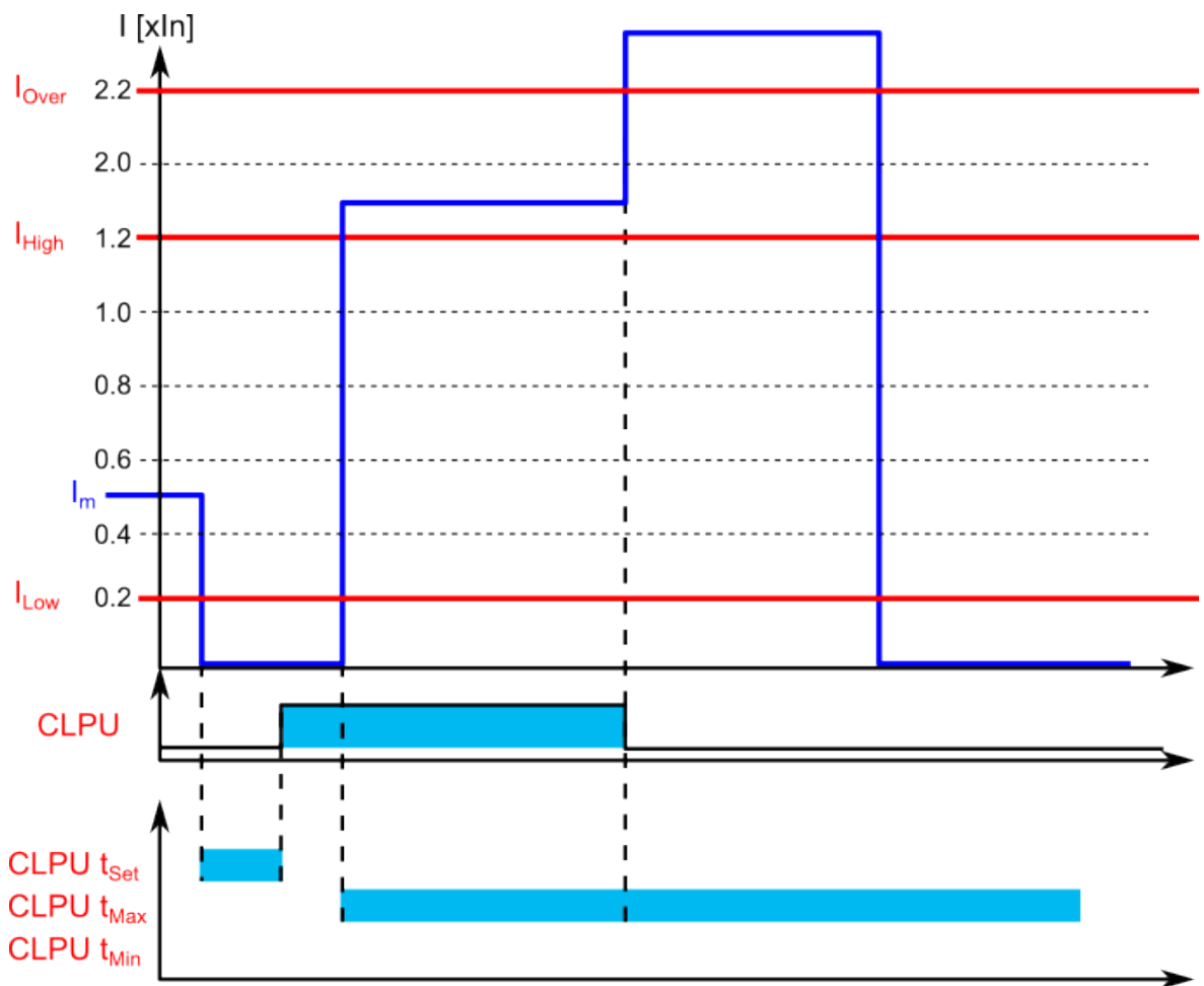
Figure. 5.5.7 - 209. Example of timers and pick-up parameters (activated pick-up and instant release due to overcurrent).
