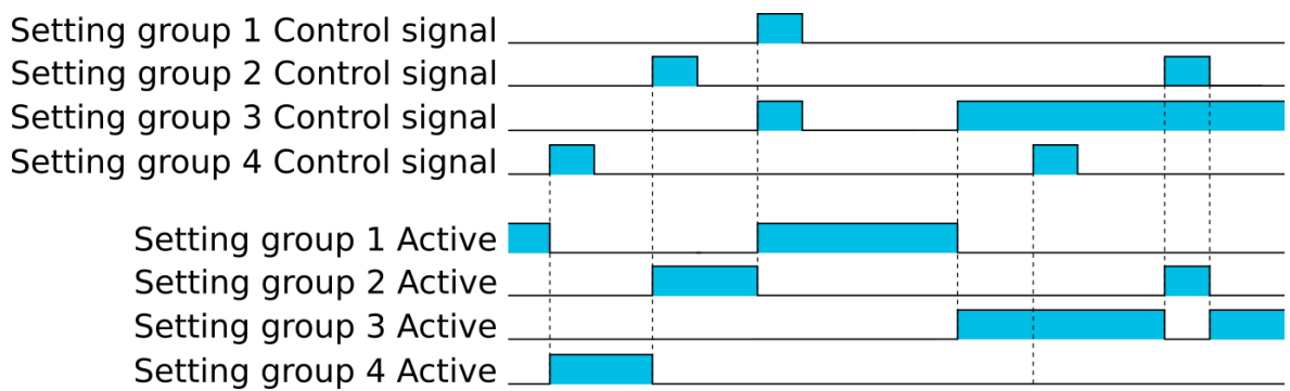
Figure. 5.5.2 - 180. Example sequences of group changing (control with pulse only, or with both pulses and static signals).
