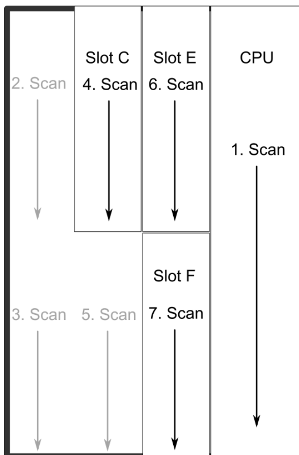
Figure. 8.1 - 263. AQ-X215 hardware scanning and I/O naming principles.
