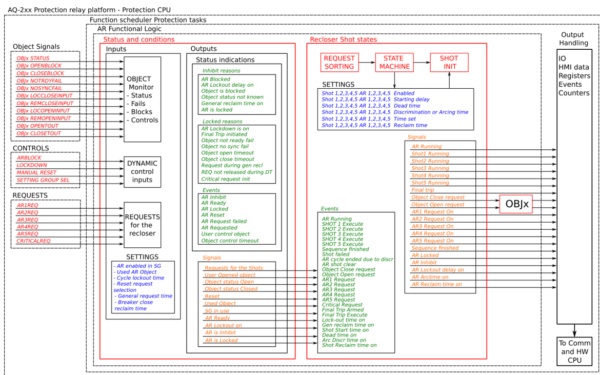
Figure. 5.5.5 - 203. Simplified function block diagram of the auto-recloser function.
