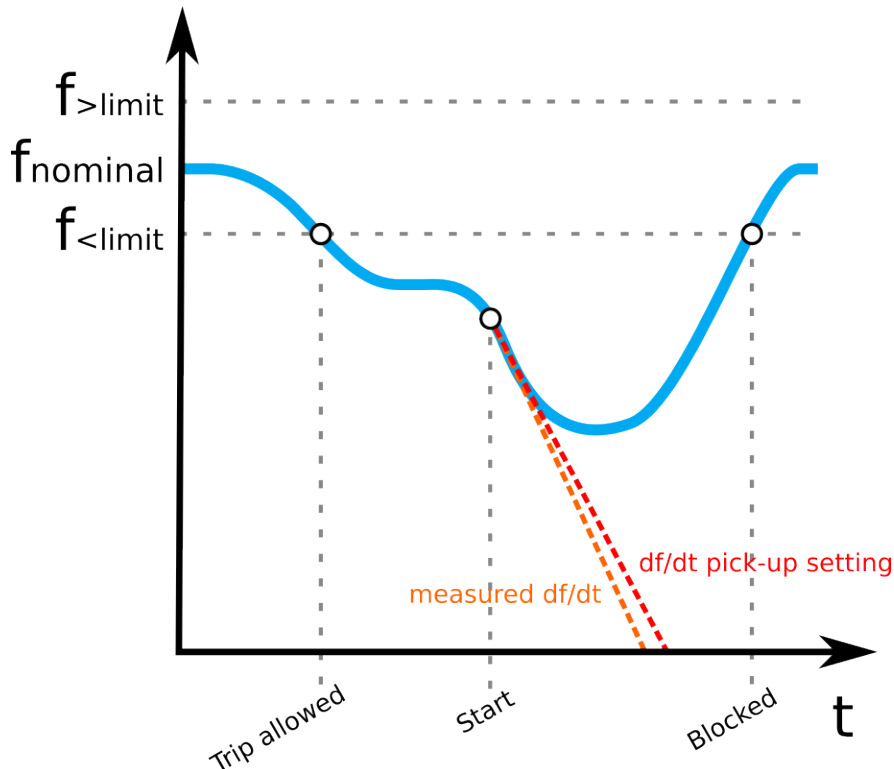
Figure. 5.4.16 - 148. Operation of the df/dt >/< function when the frequency starts but doesn't trip.
