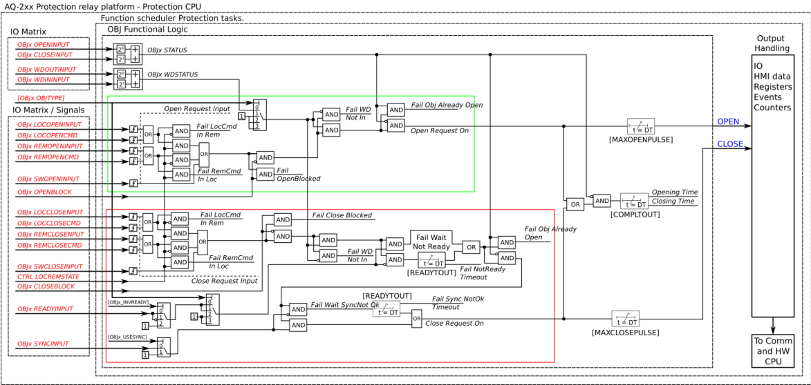
Figure. 5.5.3 - 185. Simplified function block diagram of the object control and monitoring function.
