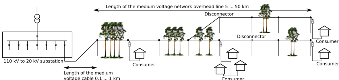
Figure. 5.5.5 - 187. Diagram of a typical radial medium-voltage network in rural areas.
