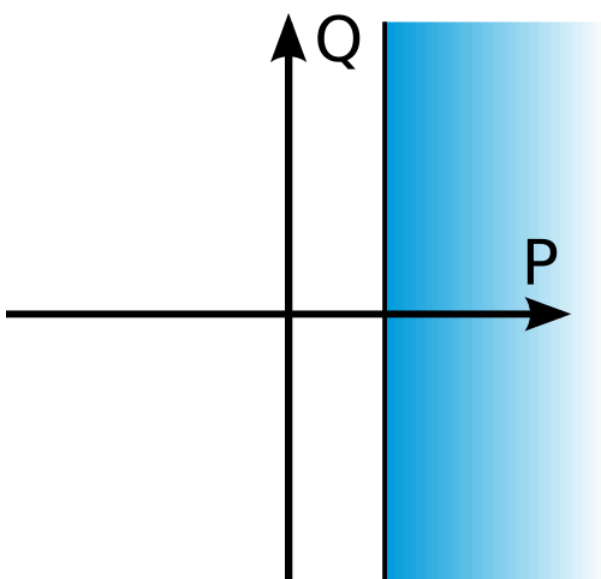
Figure. 5.4.17 - 150. Operating characteristics of overpower protection.
