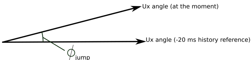
Figure. 5.5.11 - 227. Vector jump from the relay's point of view.
