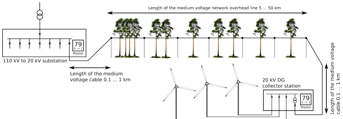
Figure. 5.5.5 - 202. Auto-reclosing with distributed generation in the line.
