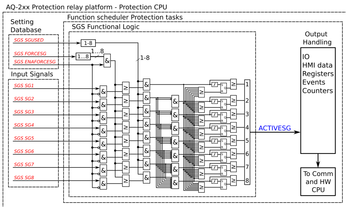
Figure. 5.5.2 - 179. Simplified function block diagram of the setting group selection function.
