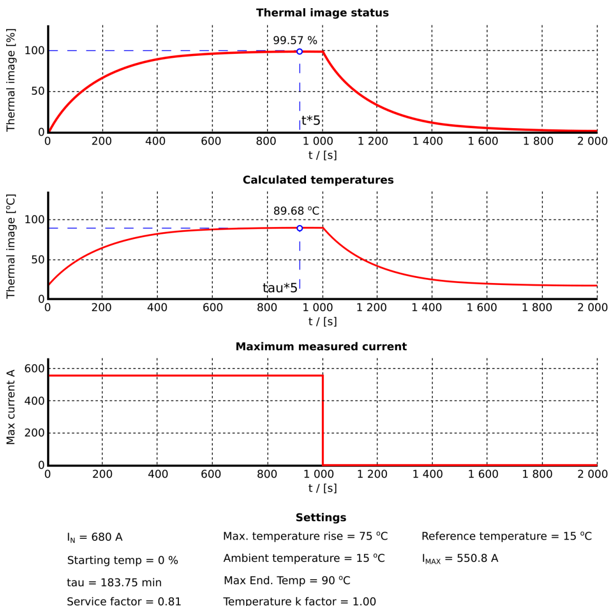
Figure. 5.4.21 - 170. Thermal response with k sf factor correctly set.
