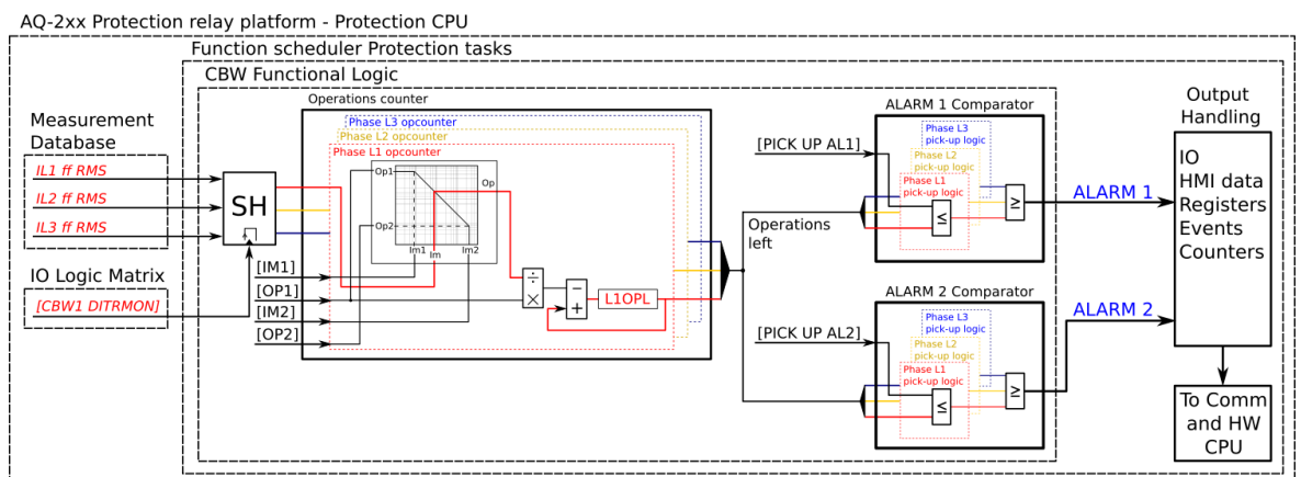
Figure. 5.6.3 - 245. Simplified function block diagram of the circuit breaker wear function.
