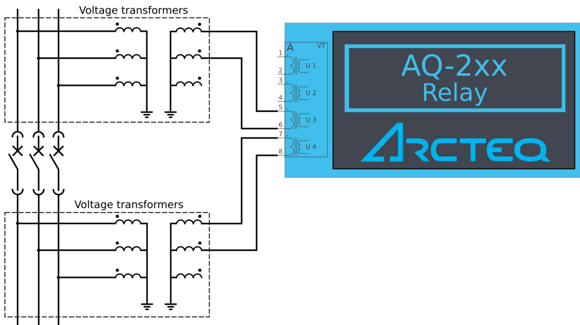
Figure. 5.5.9 - 216. Example connection of the synchrocheck function (2LL+U3+U4 mode, SYN3 in use, UL12 as reference voltage).
