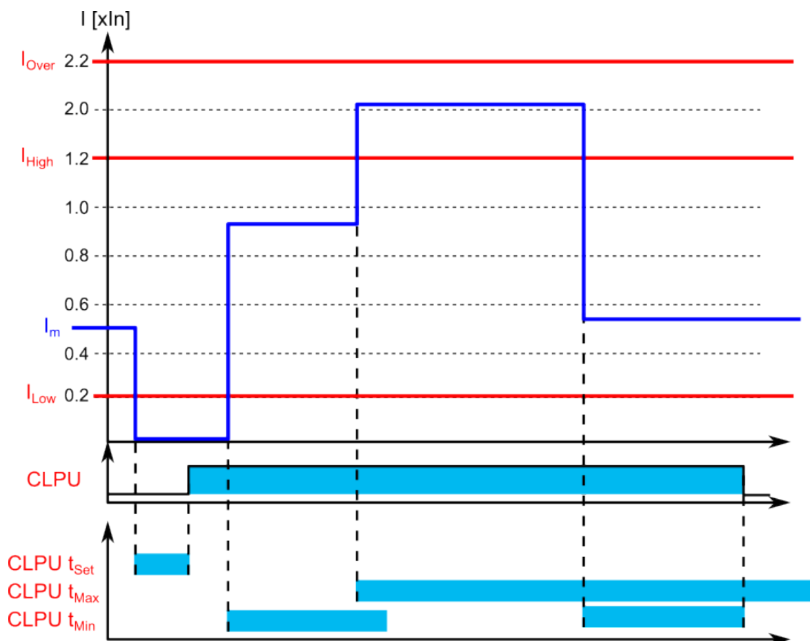
Figure. 5.5.7 - 212. Example of timers and pick-up parameters (an inrush current detected during T_{min} time).
