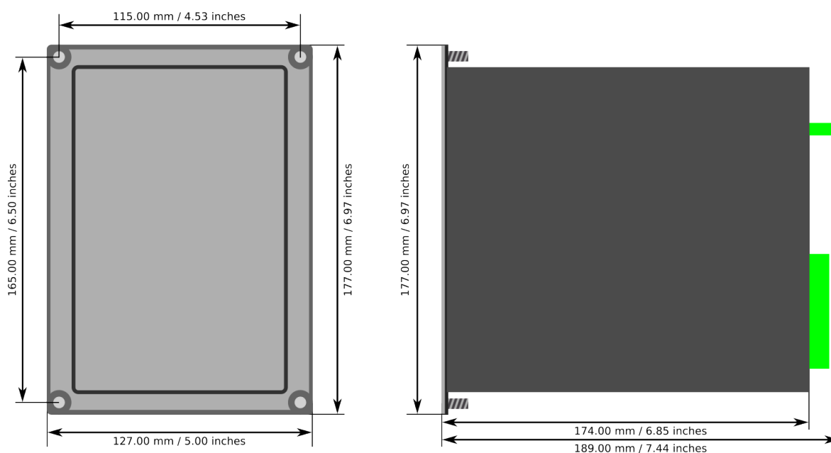
Figure. 8.14 - 281. Device dimensions.
