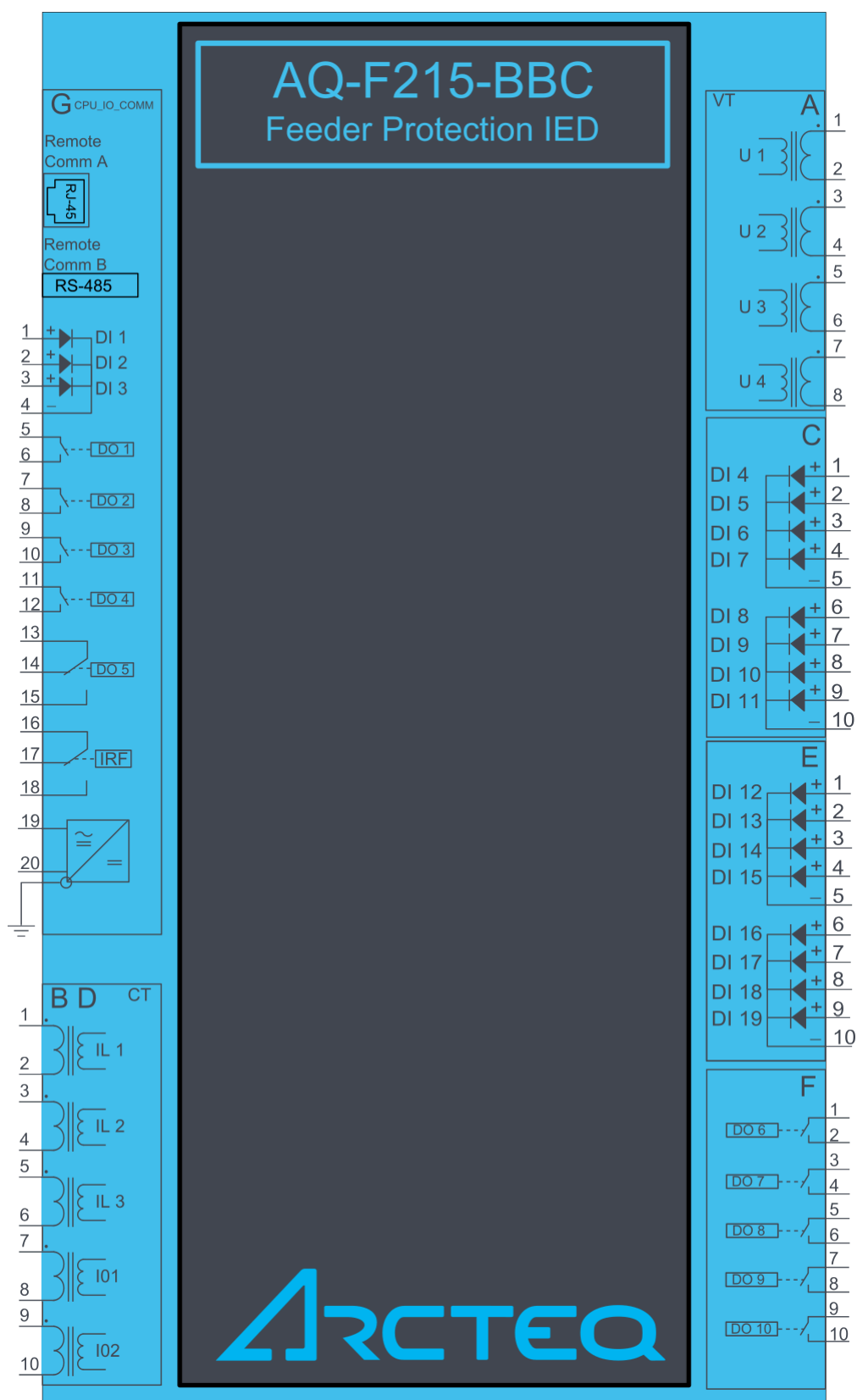
Figure. 7.1 - 253. AQ-F215 variant with digital input and output modules.
