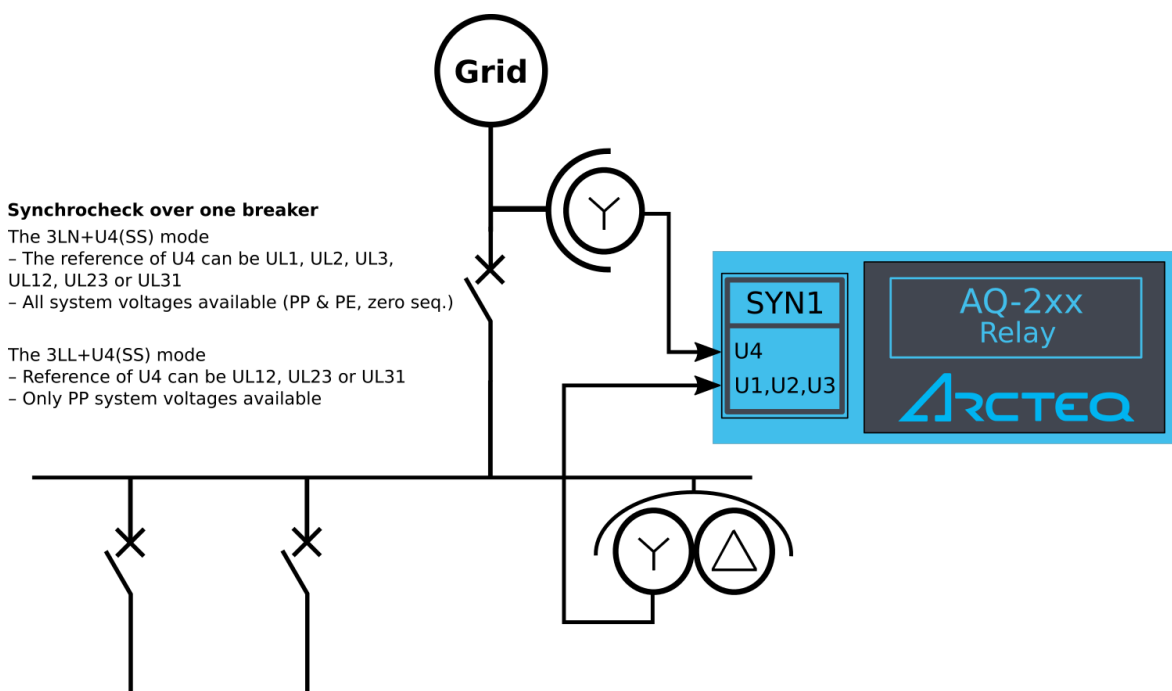
Figure. 5.5.9 - 218. Example application (synchrocheck over one breaker, with 2LL VT connection).
