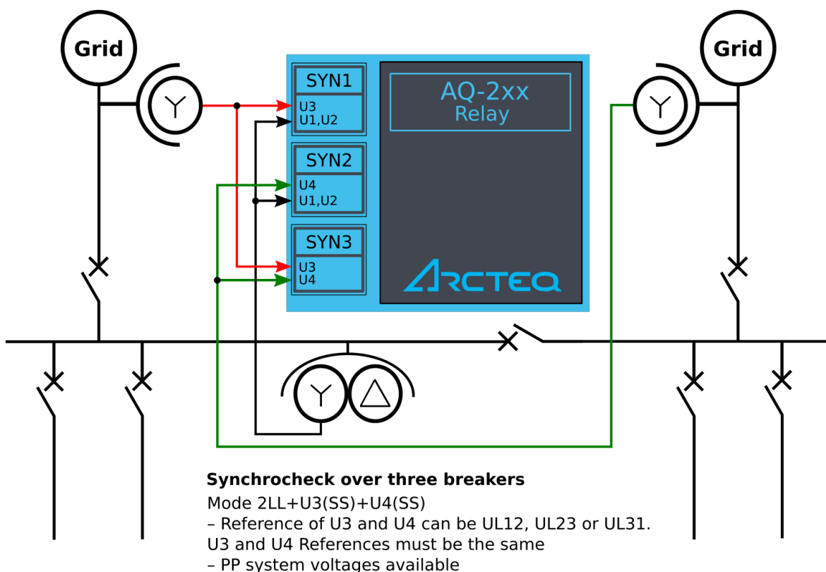
Figure. 5.5.9 - 220. Example application (synchrocheck over three breakers, with 2LL+U3+U4 connection).
