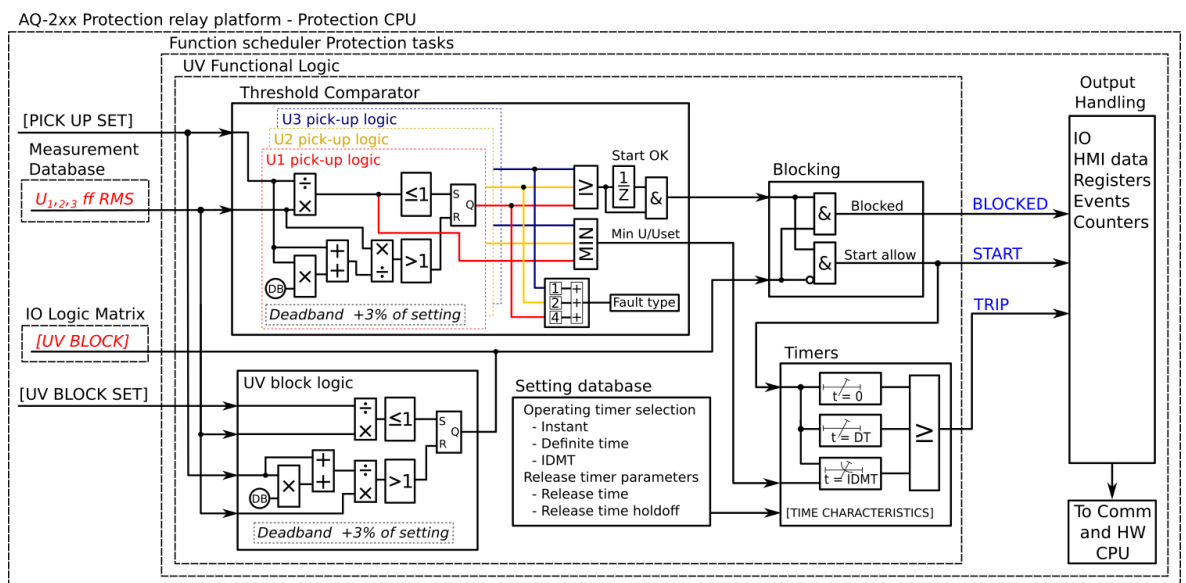
Figure. 5.4.12 - 129. Simplified function block diagram of the U< function.
