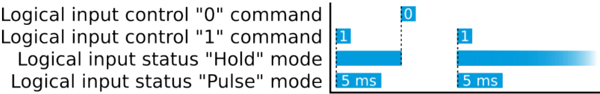
Figure. 5.5.15 - 229. Operation of logical input in "Hold" and "Pulse" modes.
