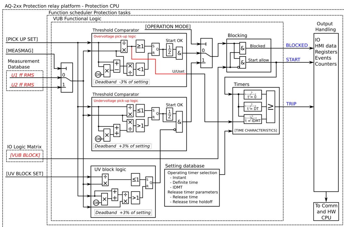
Figure. 5.4.14 - 144. Simplified function block diagram of the U1/U2&gt;/&lt; function.
