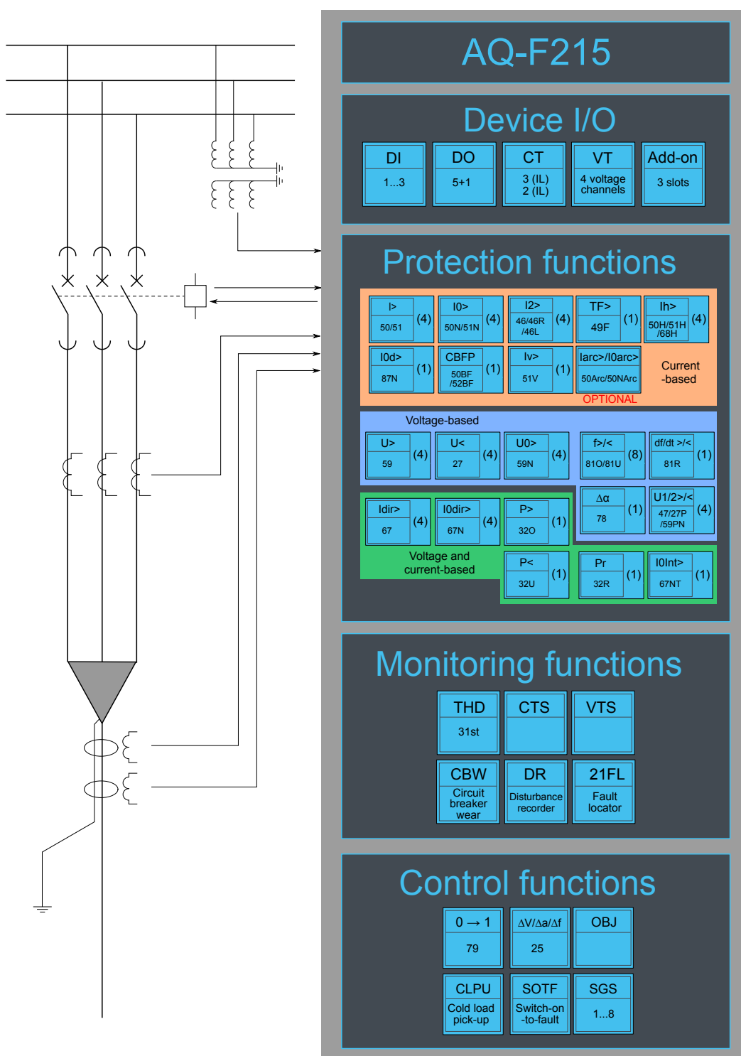
Figure. 7.1 - 254. AQ-F215 application example with function block diagram.
