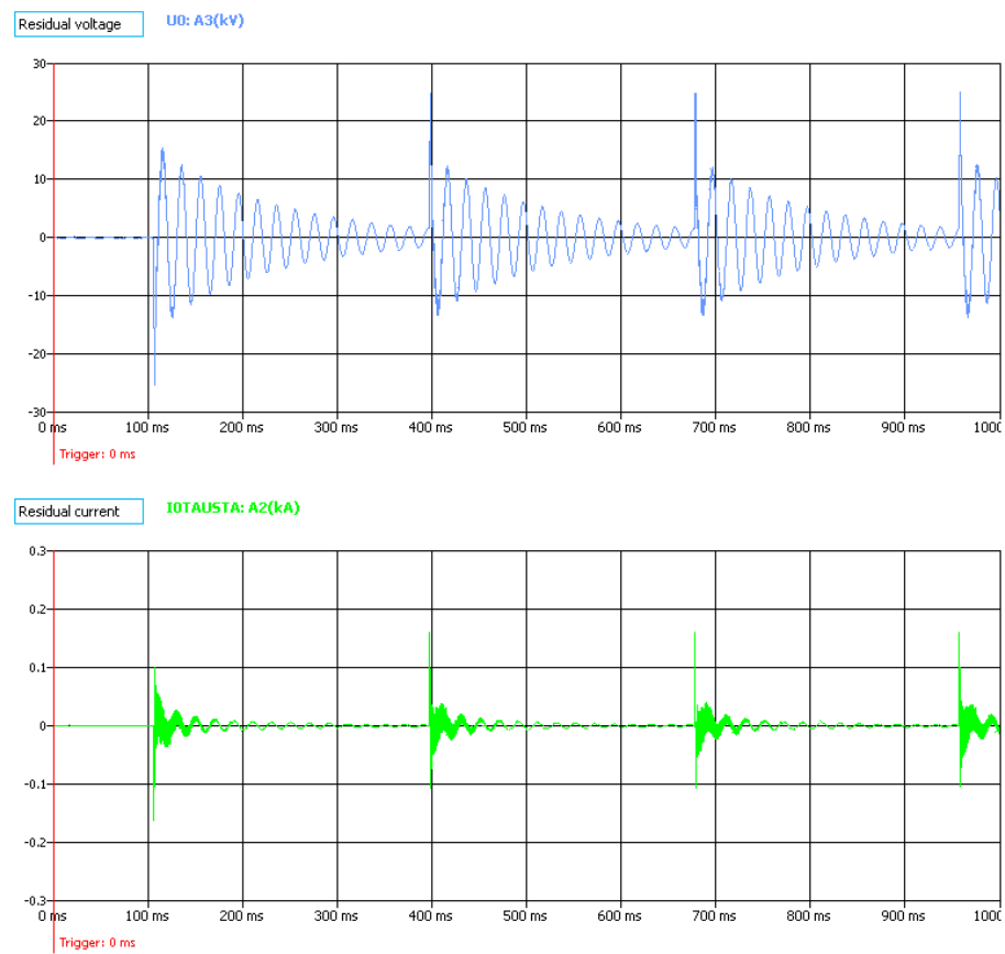
Figure. 5.4.6 - 99. An intermittent earth fault in a network tuned close to resonance, as seen by a healthy feeder relay.
