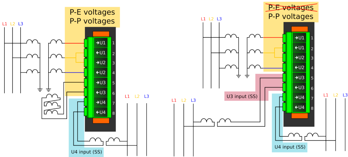
Figure. 5.4.12 - 132. Selectable measurement magnitudes with 2LL+U4 VT connection (P-E voltages not available without residual voltage).
