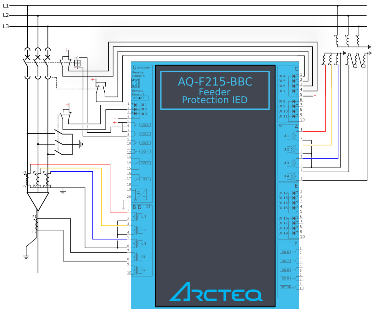
Figure. 7.2 - 255. Application example and its connections.
