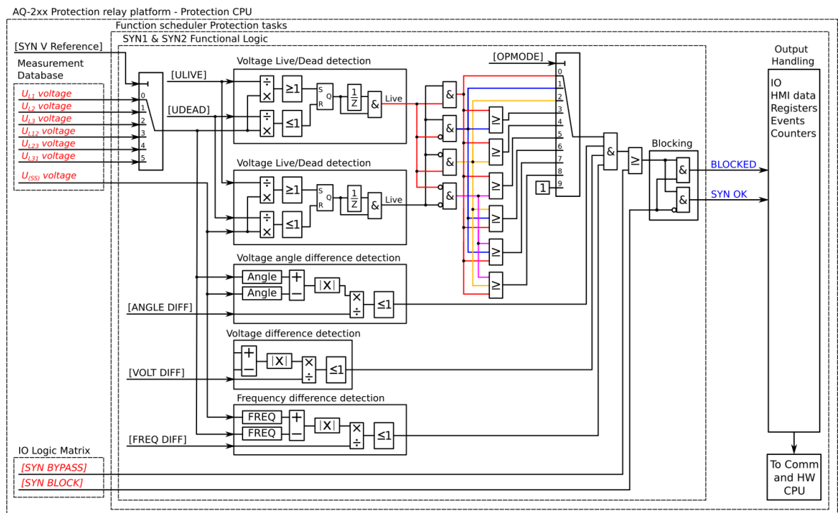
Figure. 5.5.9 - 222. Simplified function block diagram of the SYN1 and SYN2 function.
