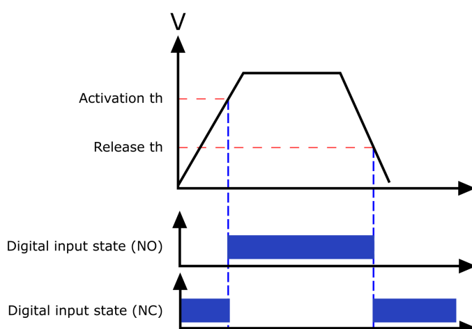
Figure. 8.5 - 268. Digital input state when energizing and de-energizing the digital input channels.
