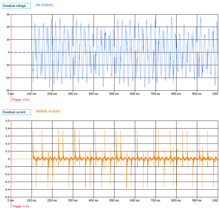
Figure. 5.4.6 - 100. An intermittent earth fault in an undercompensated medium size network, as seen by a faulty feeder relay.
