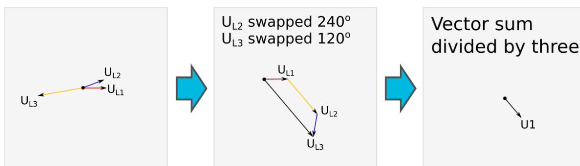
Figure. 5.4.14 - 140. Close-distance short-circuit between phases 1 and 3.
