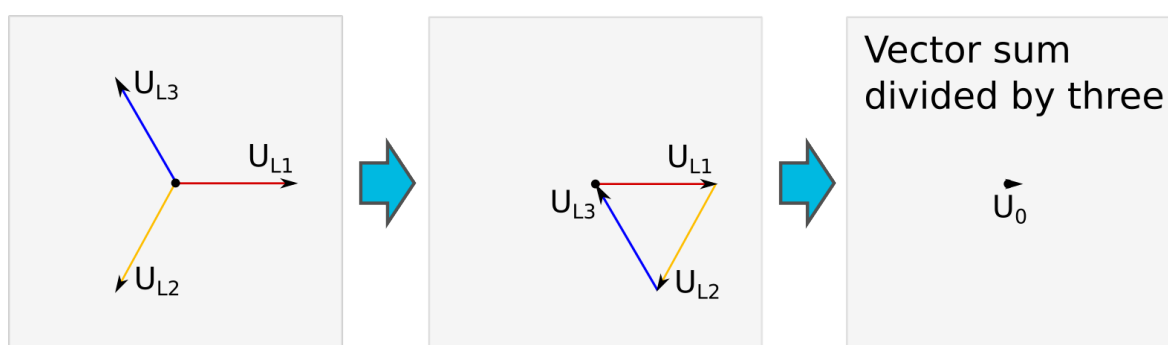
Figure. 5.4.13 - 134. Normal situation.
