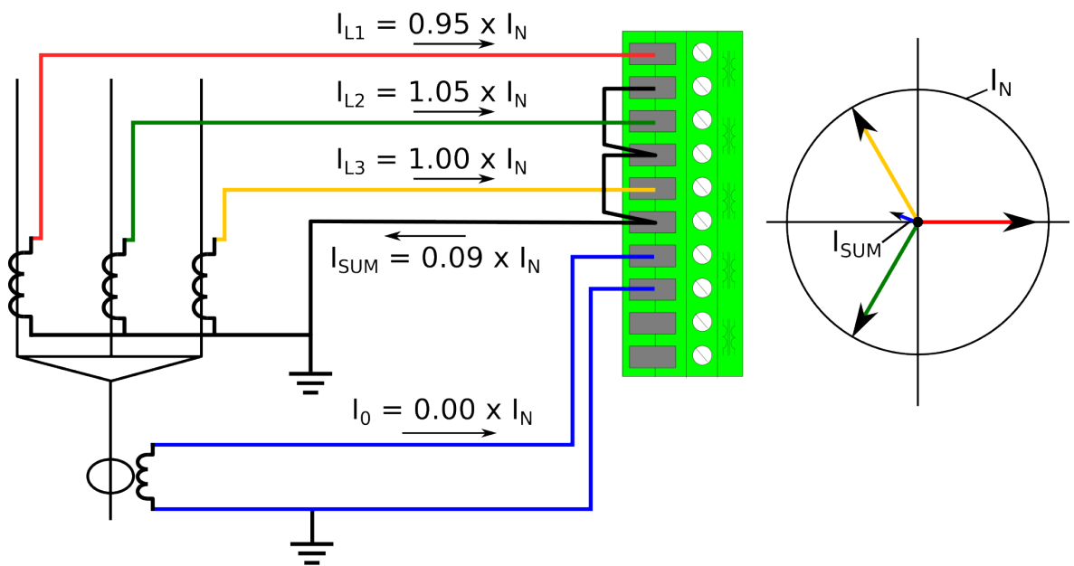
Figure. 5.4.10 - 121. Cable end differential with natural unbalance in the phase current measurement.
