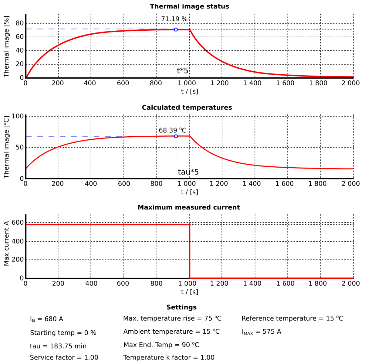
Figure. 5.4.21 - 167. Thermal image response with nominal load (installation according to presumptions).
