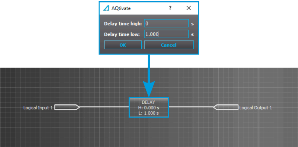
Figure. 5.5.15 - 230. Extending a logical input pulse.
