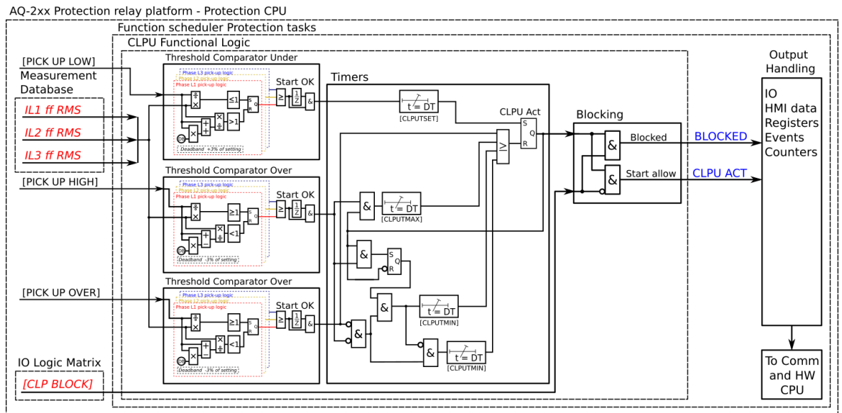
Figure. 5.5.7 - 206. Simplified function block diagram of the cold load pick-up function.
