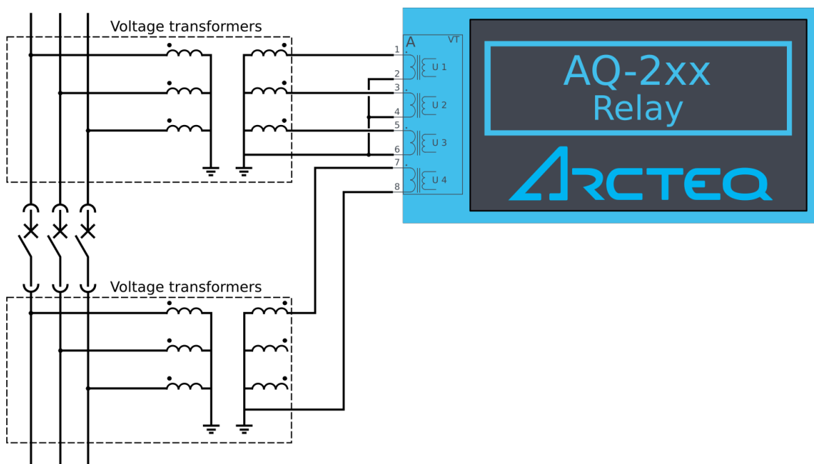
Figure. 5.5.9 - 214. Example connection of the synchrocheck function (3LN+U4 mode, SYN1 in use, UL1 as reference voltage).
