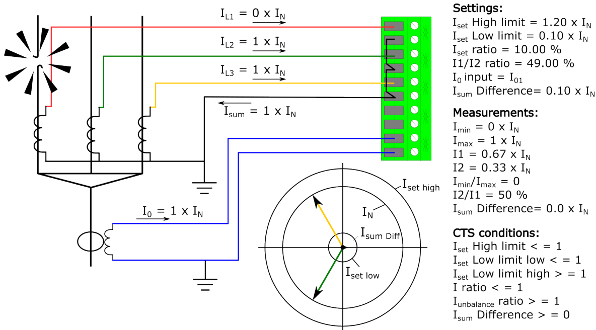
Figure. 5.6.1 - 192. Broken primary phase current wiring.
