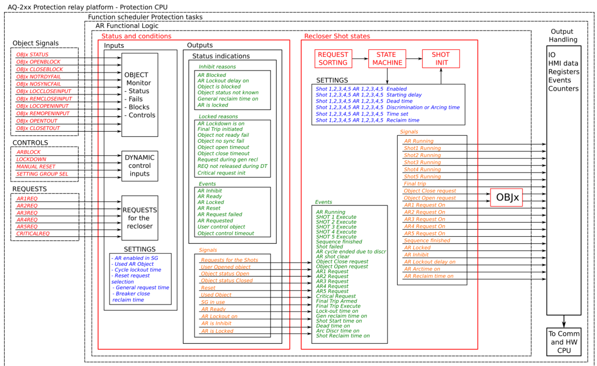
Figure. 5.5.6 - 153. Simplified function block diagram of the auto-recloser function.
