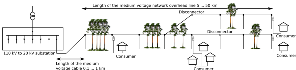
Figure. 5.5.6 - 137. Diagram of a typical radial medium-voltage network in rural areas.
