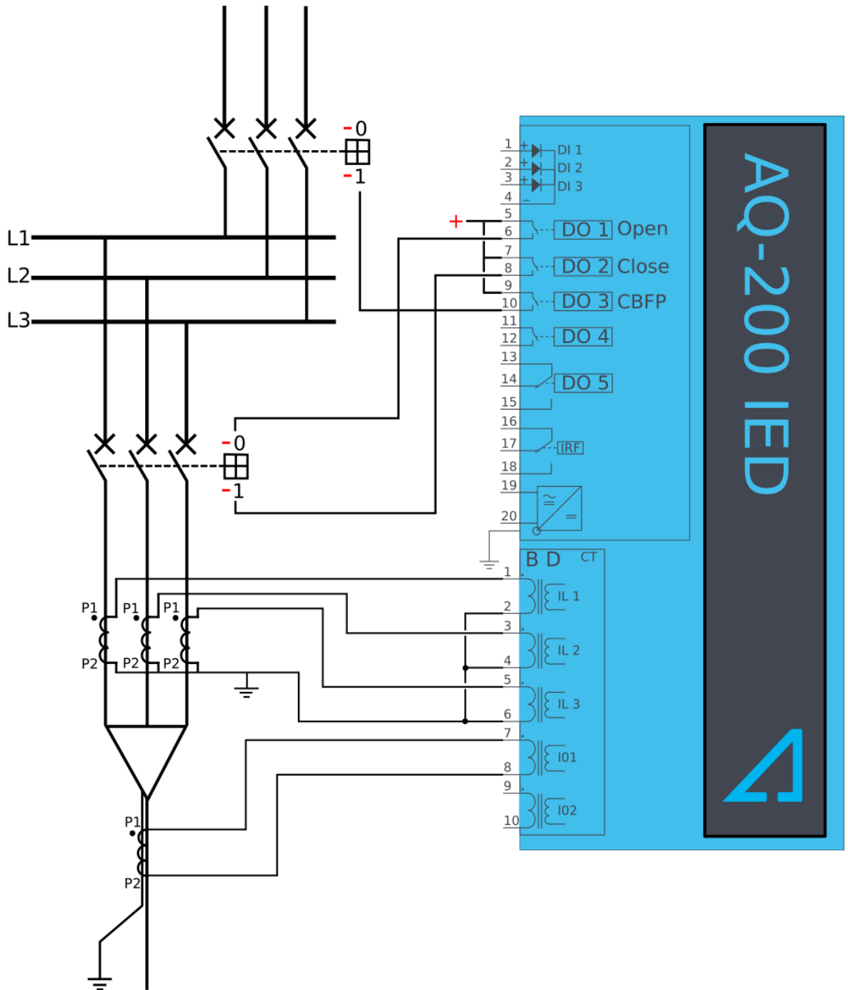
Figure. 5.4.10 - 60. Wiring diagram when Trip and CBFP are configured to the device.
