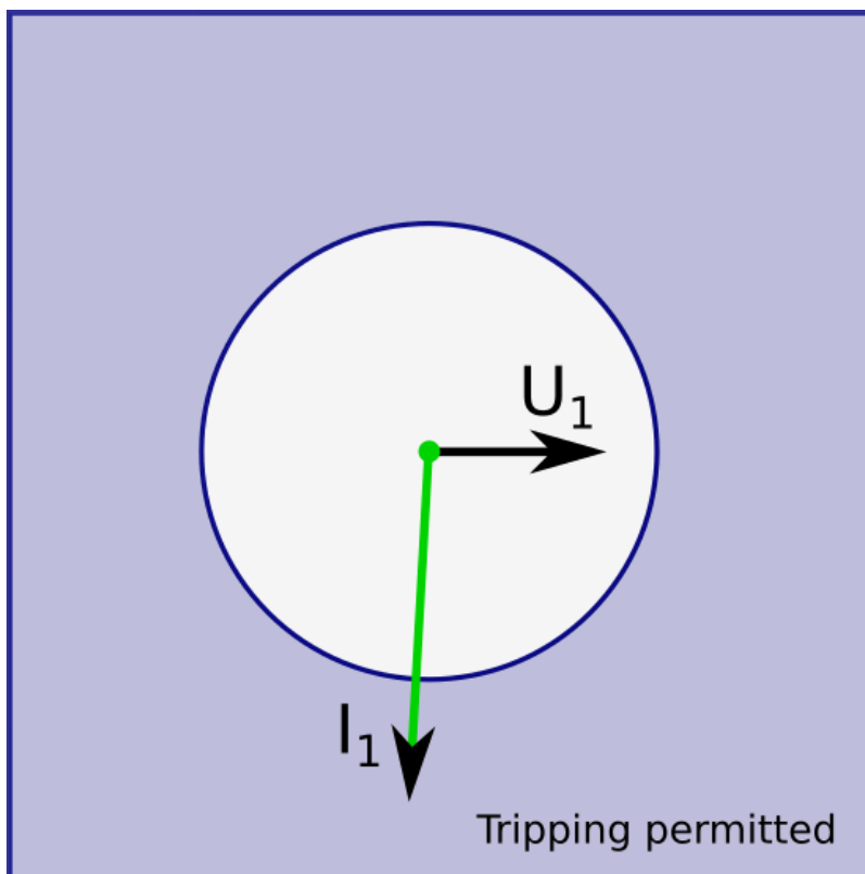
Figure. 5.4.5 - 41. When I_{dir}> function has been set to "Non-directional" the function works basically just like a traditional non-directional overcurrent protection function.
