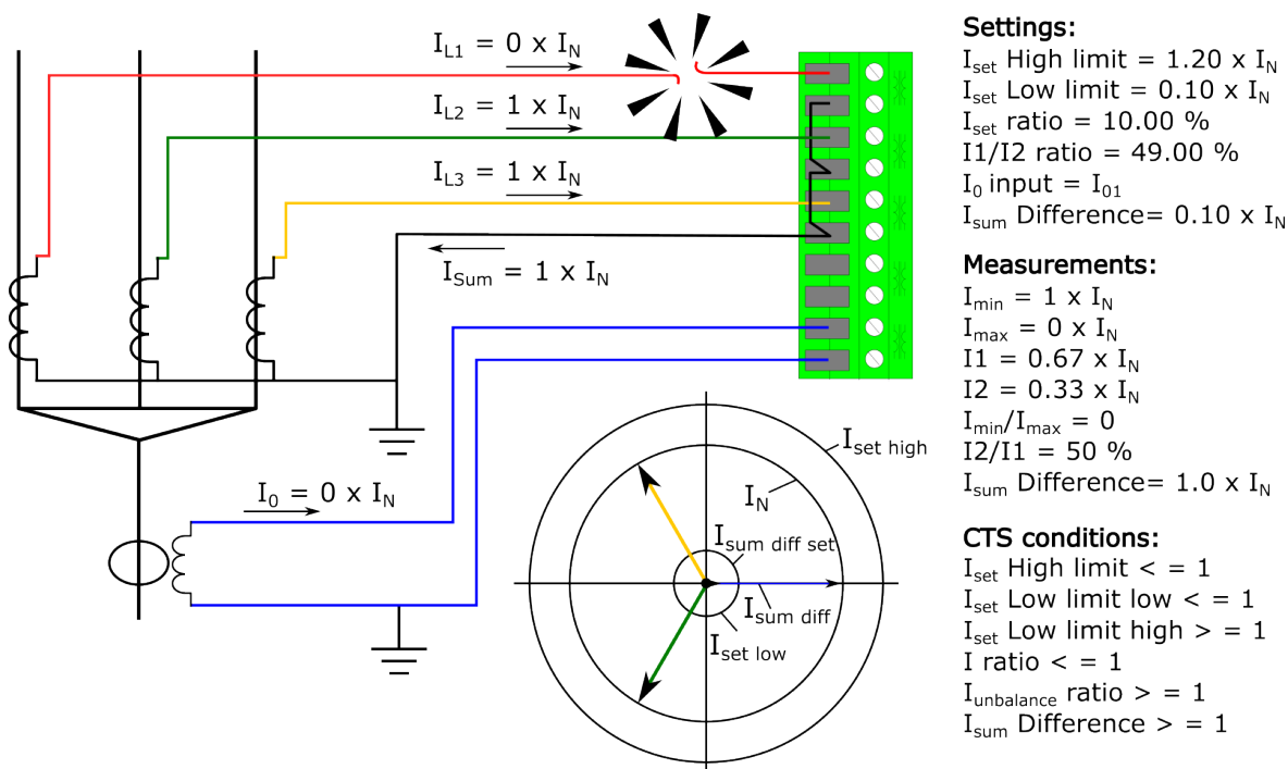
Figure. 5.6.1 - 191. Broken secondary phase current wiring.
