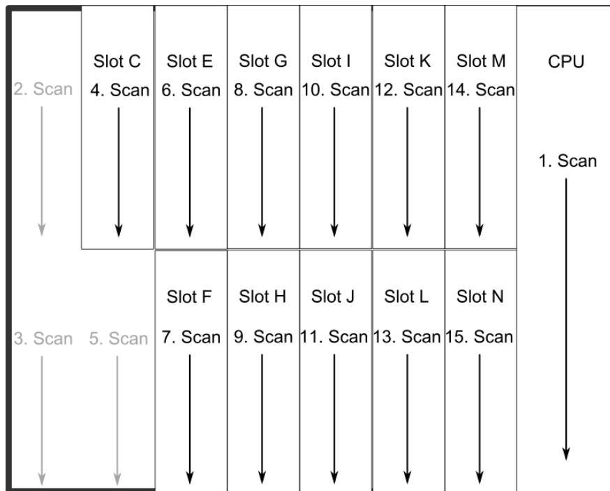
Figure. 8.1 - 218. AQ-X255 hardware scanning and I/O naming principles.
