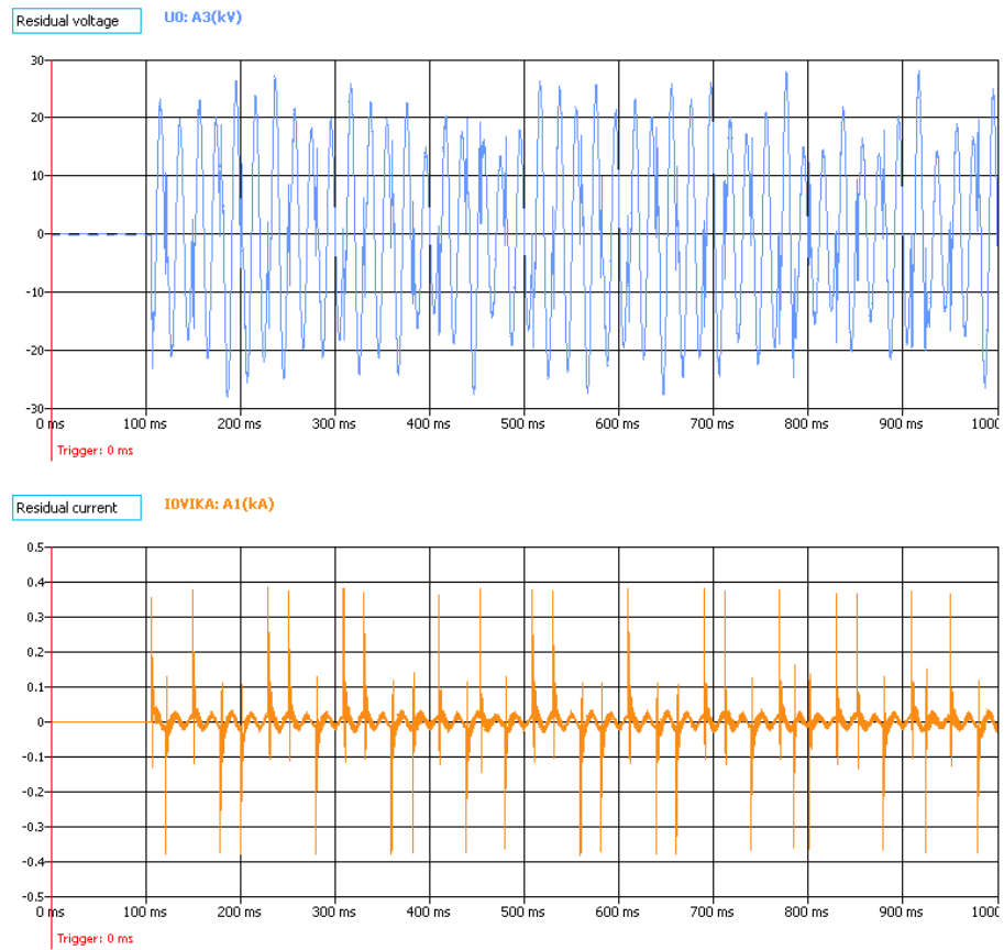
Figure. 5.4.7 - 50. An intermittent earth fault in an undercompensated medium size network, as seen by a faulty feeder relay.
