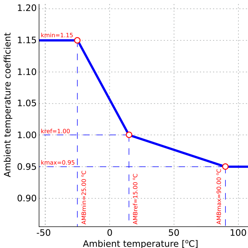
Figure. 5.4.22 - 110. Ambient temperature coefficient calculation (a three-point linear approximation and a settable correction curve).
