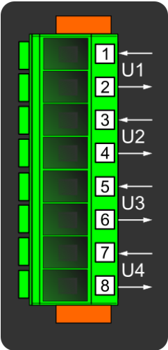
Figure. 8.4 - 221. Voltage measurement module.
