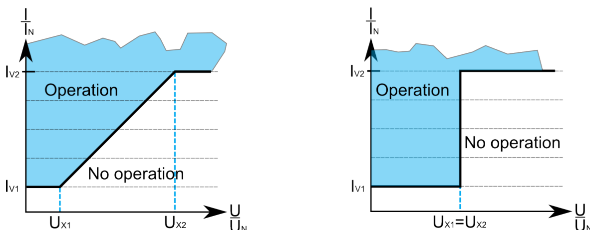
Figure. 5.4.21 - 107. Pick-up levels in the two modes.
