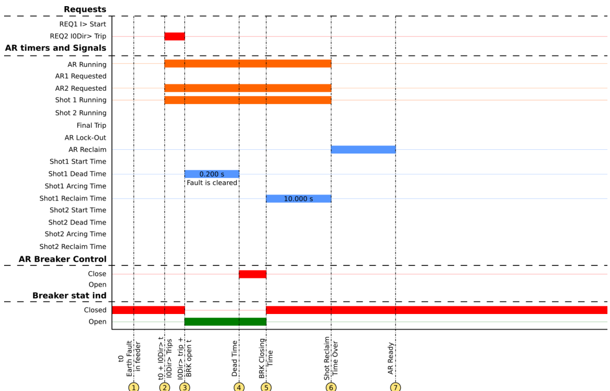
Figure. 5.5.6 - 145. Signal status graph of the transient earth fault auto-recloser cycle.
