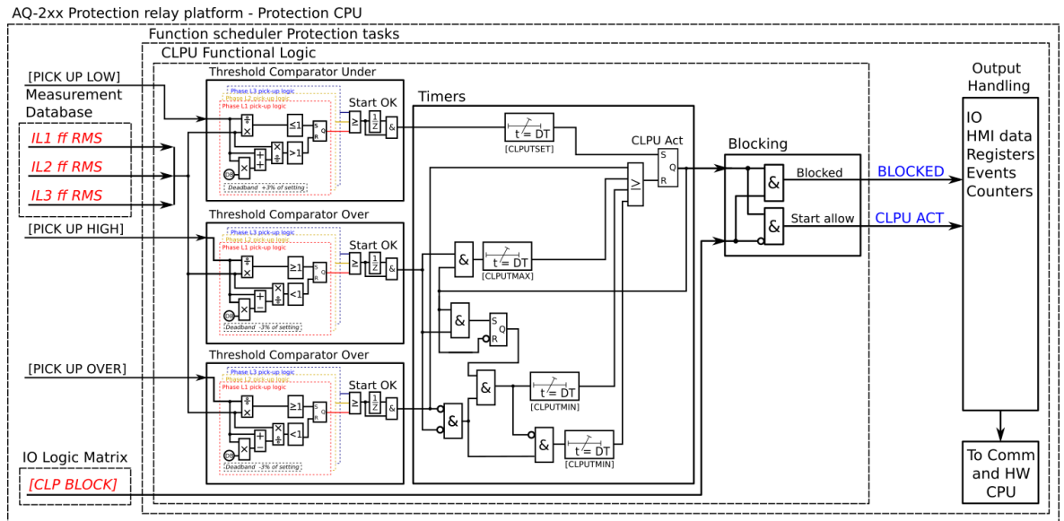
Figure. 5.5.8 - 156. Simplified function block diagram of the cold load pick-up function.
