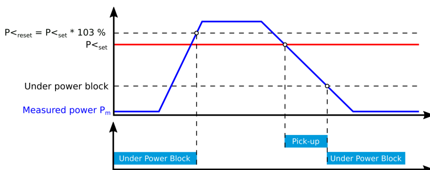
Figure. 5.4.19 - 104. Activation and deactivation characteristics of low power blocking.
