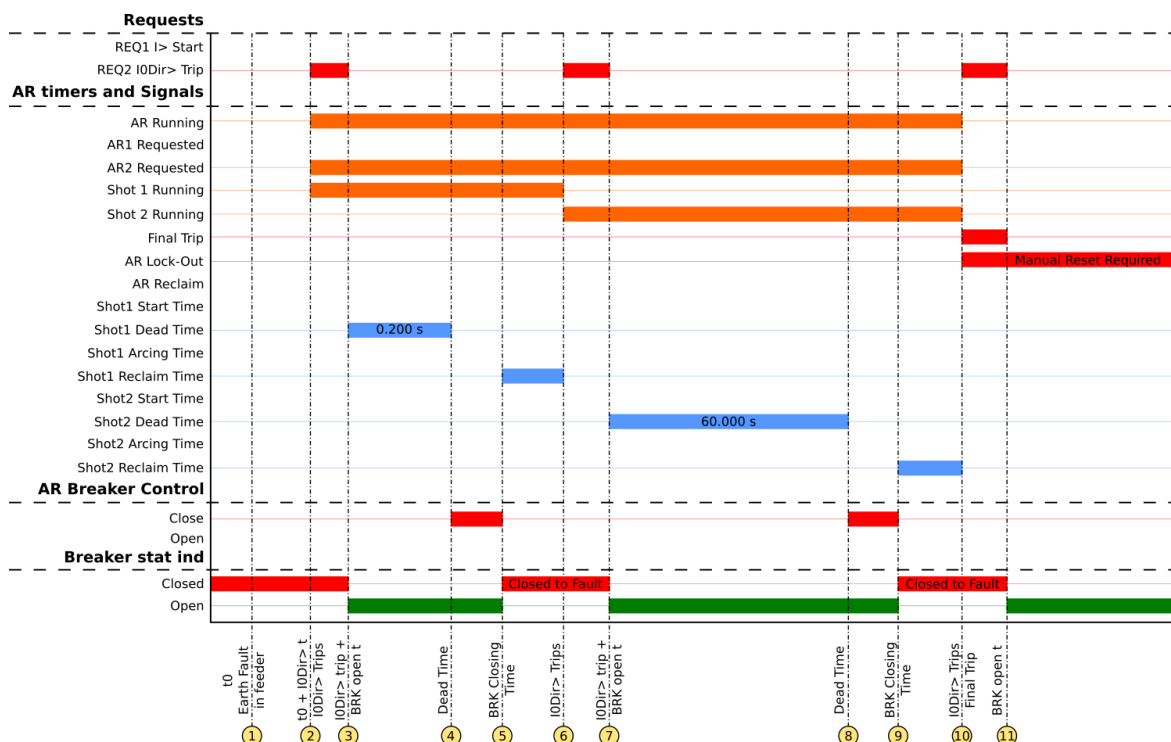
Figure. 5.5.6 - 141. Signal status graph of the permanent earth fault auto-recloser cycle.
