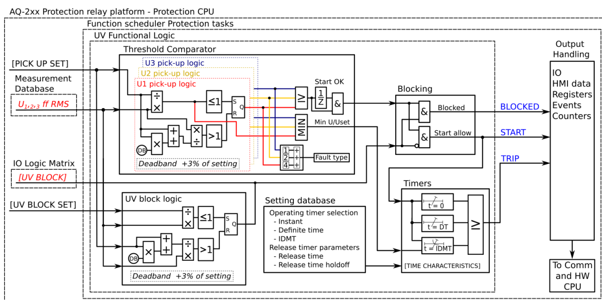
Figure. 5.4.13 - 79. Simplified function block diagram of the U< function.
