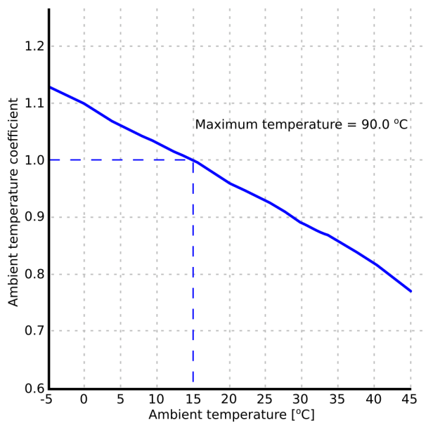
Figure. 5.4.22 - 113. Set correction curve for ambient temperature.
