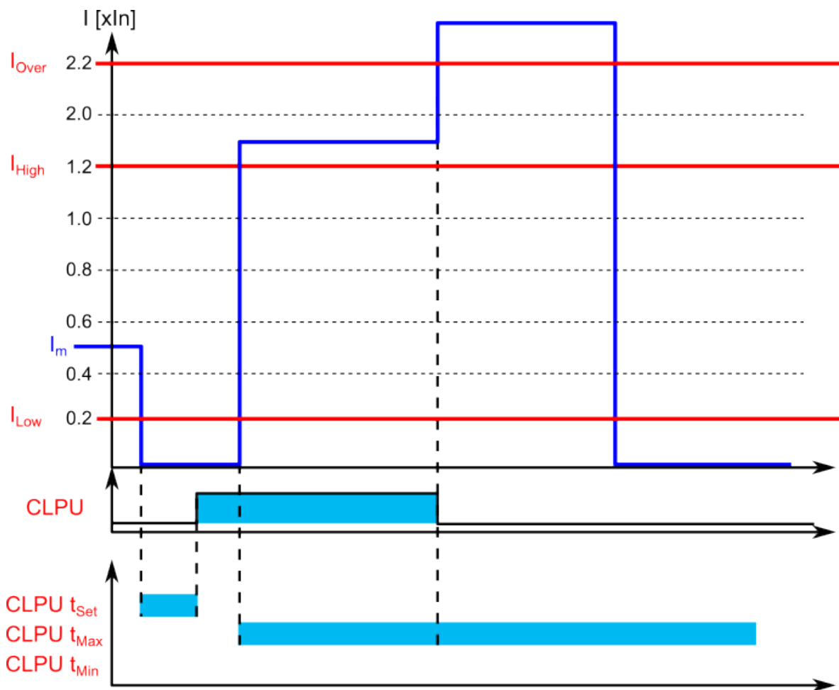
Figure. 5.5.8 - 159. Example of timers and pick-up parameters (activated pick-up and instant release due to overcurrent).
