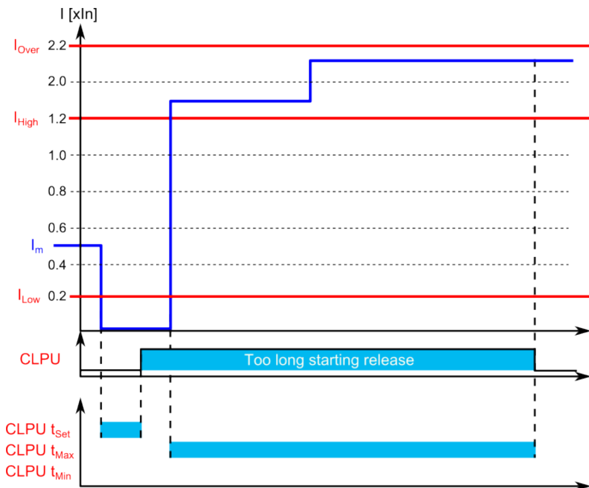
Figure. 5.5.8 - 160. Example of timers and pick-up parameters (activated pick-up and instant release due to too long starting).
