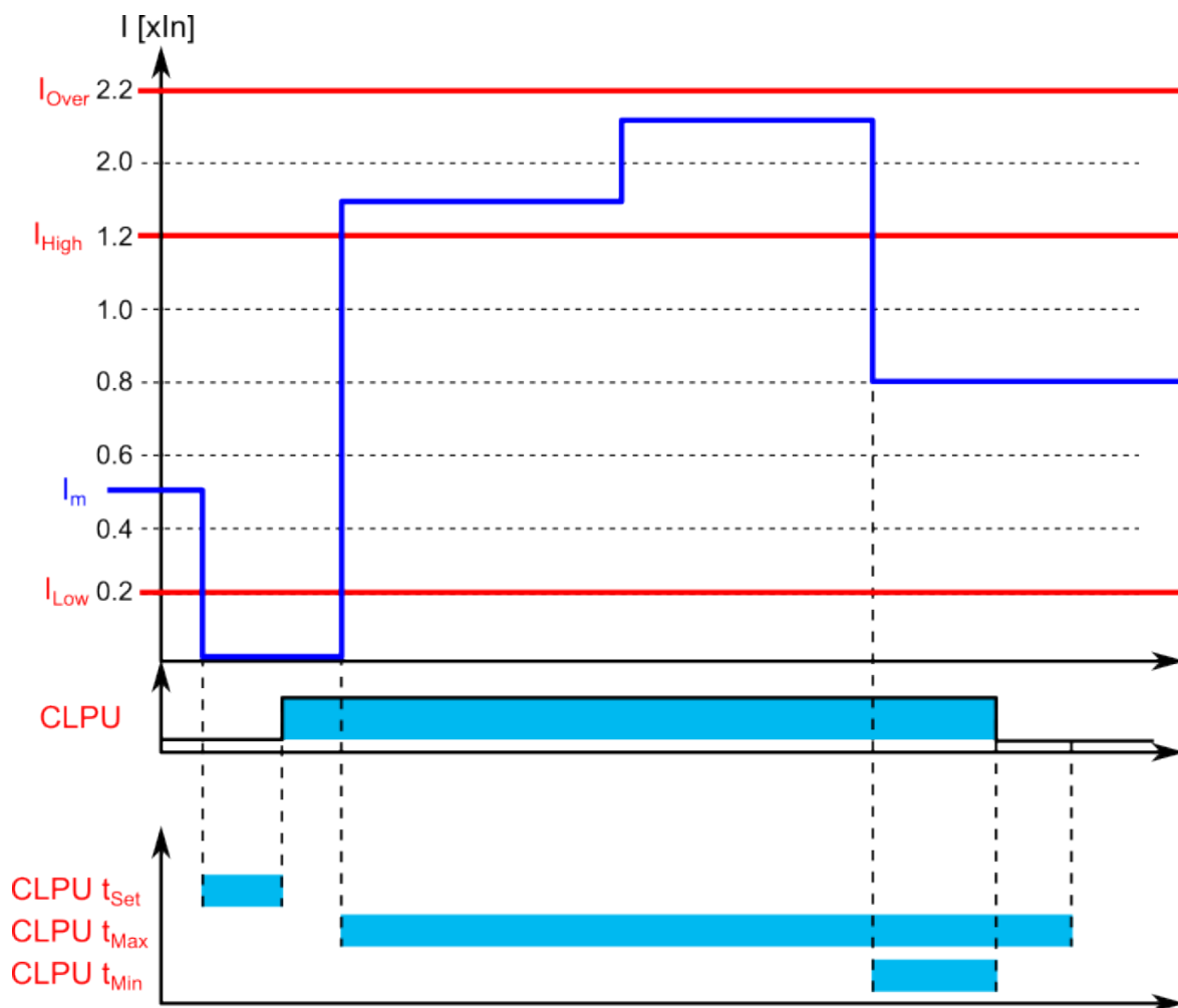
Figure. 5.5.8 - 157. Example of timers and pick-up parameters (normal CLPU situation).
