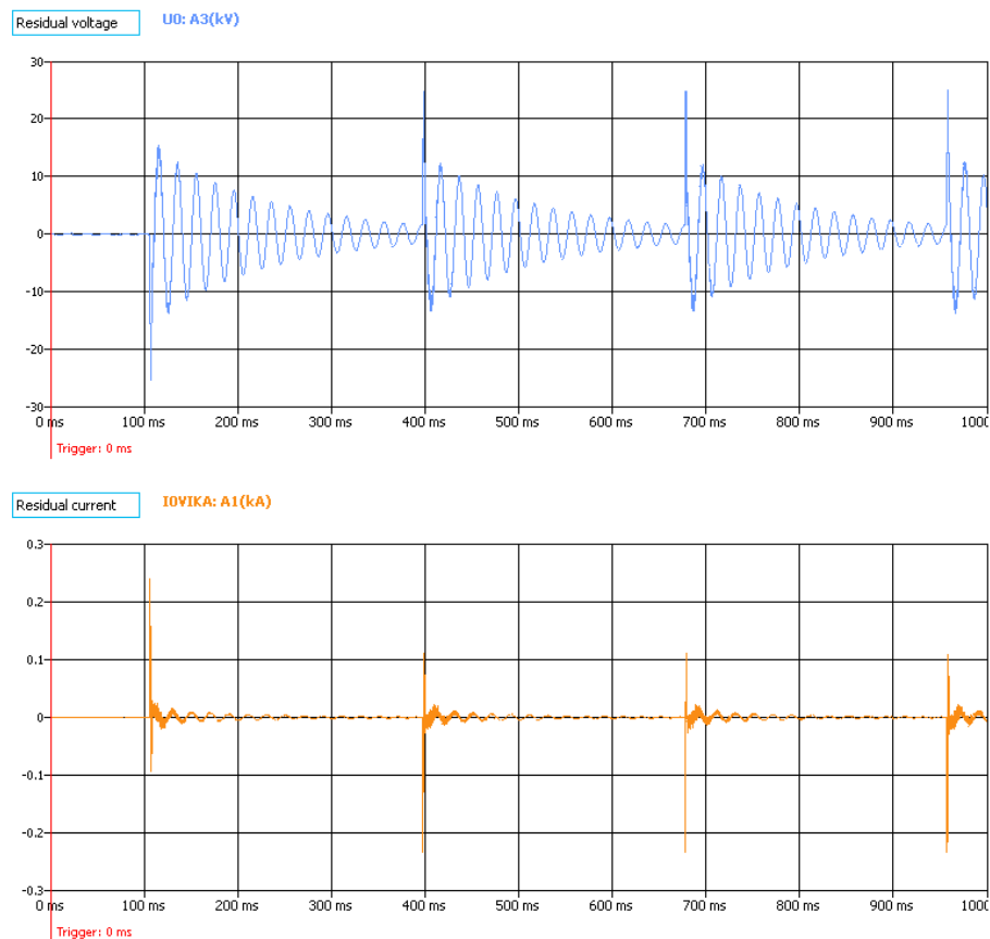
Figure. 5.4.7 - 48. An intermittent earth fault in a medium size network tuned close to resonance, as seen by a faulty feeder relay.
