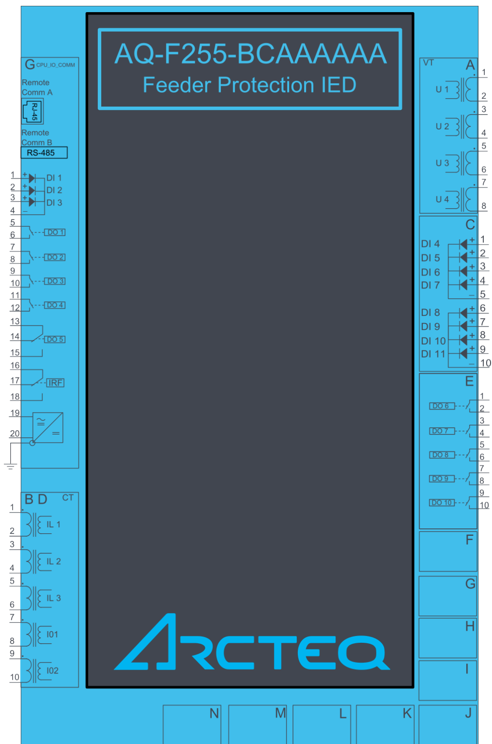
Figure. 7.1 - 207. AQ-F255 variant with digital input and output modules.
