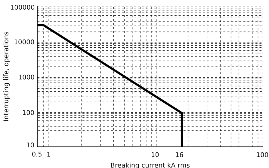
Figure. 5.6.3 - 196. Example of the circuit breaker interrupting life operations.
