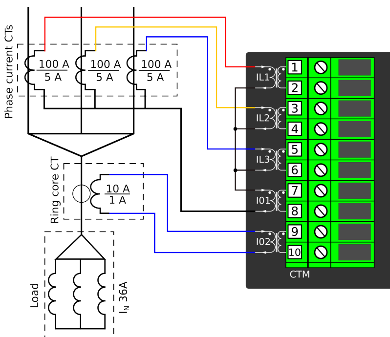
Figure. 5.2.1 - 3. Connections.
