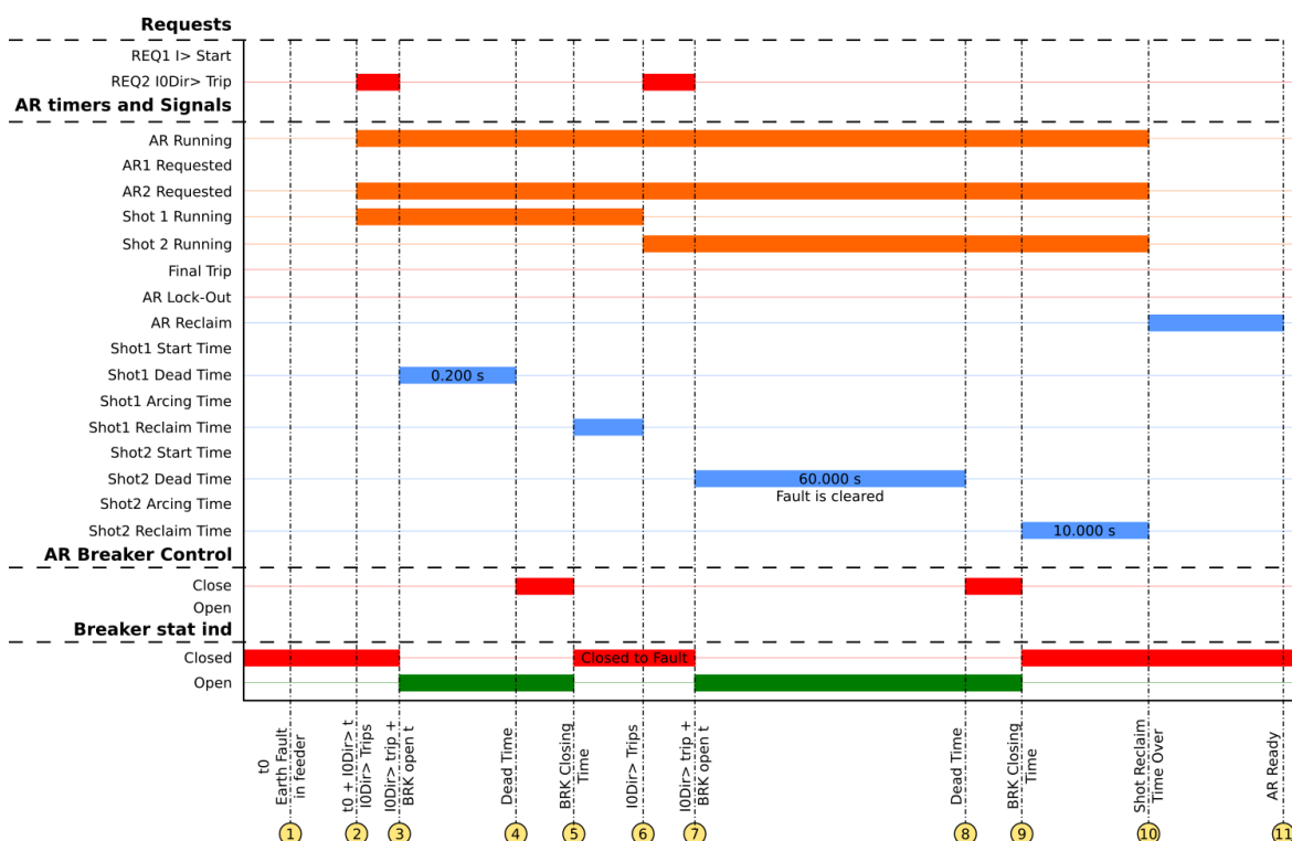
Figure. 5.5.6 - 143. Signal status graph of the semi-permanent earth fault auto-recloser cycle.
