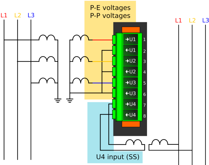
Figure. 5.4.13 - 80. Selectable measurement magnitudes with 3LN+U4 VT connection.
