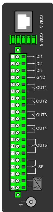
Figure. 8.2 - 219. CPU module.
