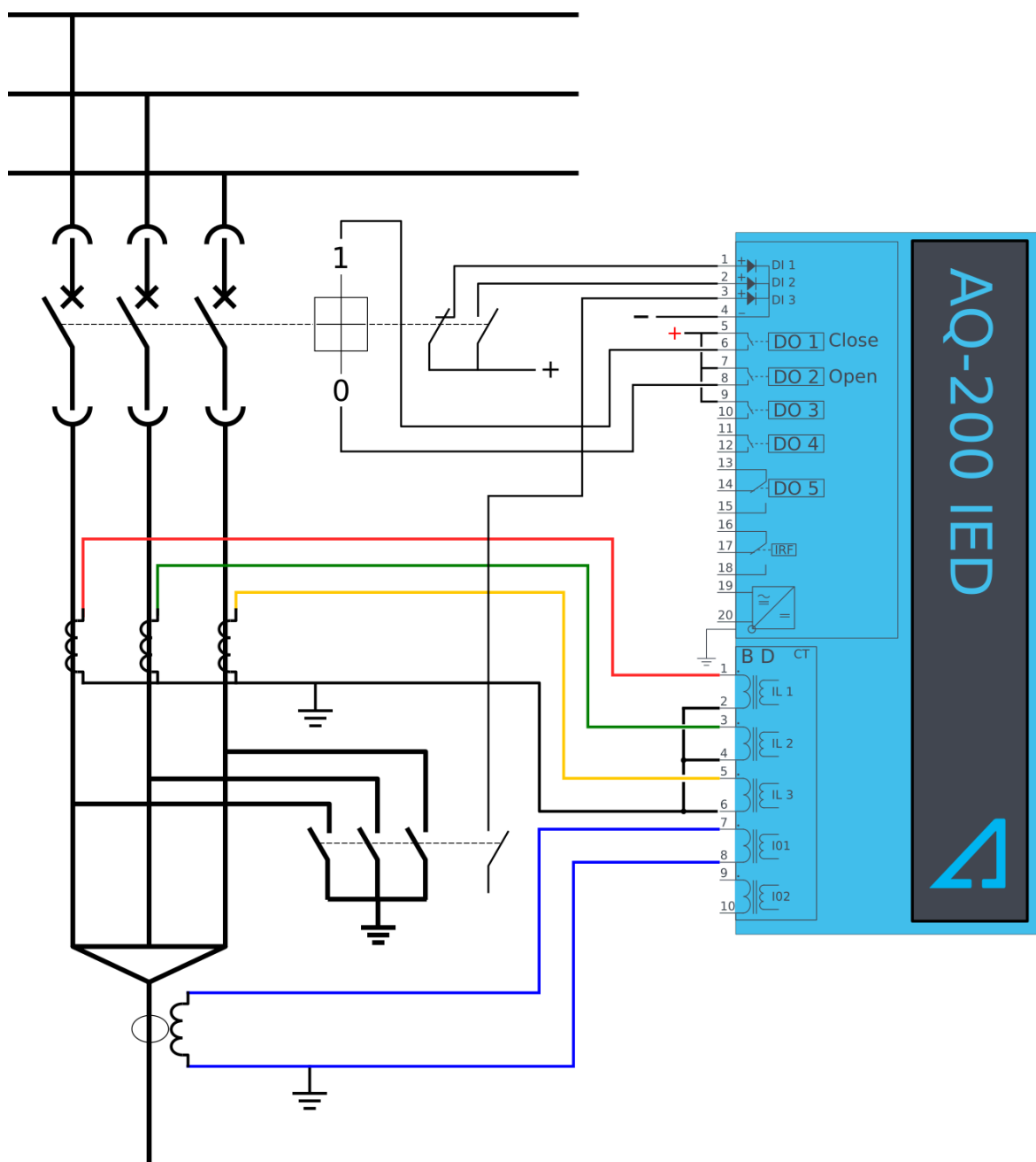
Figure. 5.5.4 - 136. Example of an interlock application.
