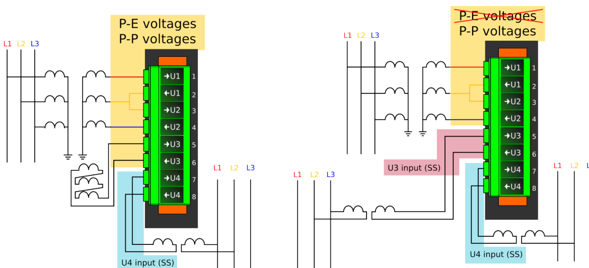
Figure. 5.4.13 - 82. Selectable measurement magnitudes with 2LL+U4 VT connection (P-E voltages not available without residual voltage).
