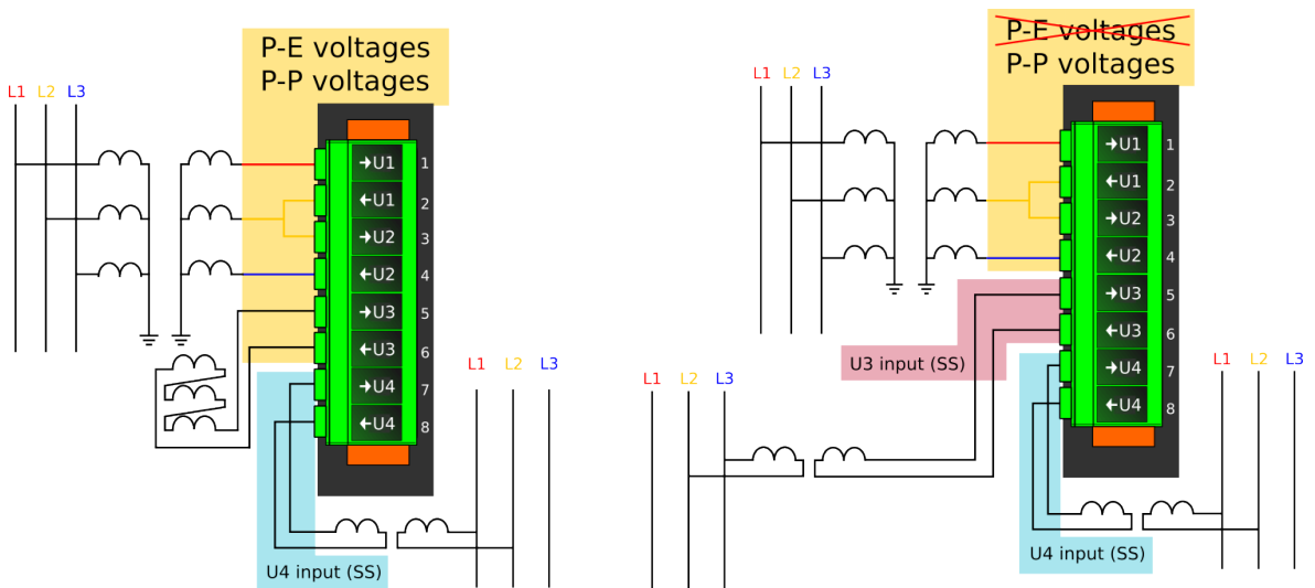
Figure. 5.4.12 - 78. Selectable measurement magnitudes with 2LL+U3+U4 VT connection (P-E voltages not available without residual voltage).
