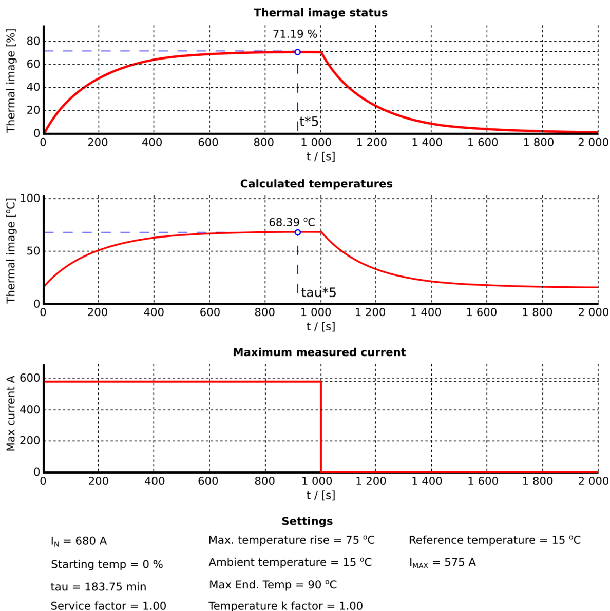
Figure. 5.4.22 - 117. Thermal image response with nominal load (installation according to presumptions).
