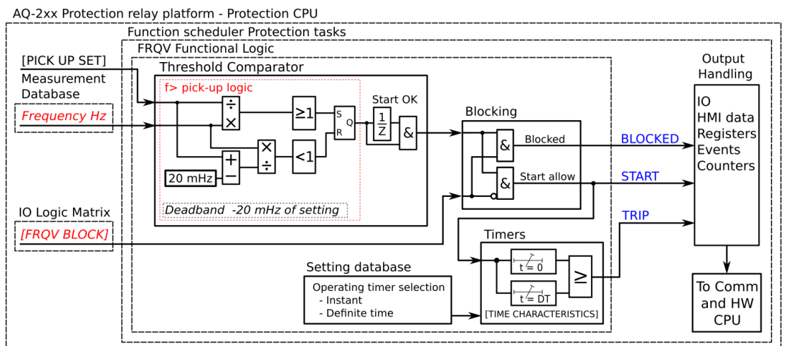
Figure. 5.4.16 - 96. Simplified function block diagram of the f > function.
