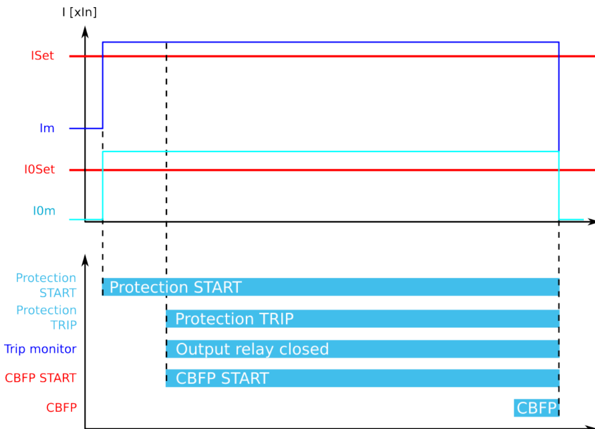
Figure. 5.4.10 - 62. CBFP when "Current and DO" is the selected criterion.
