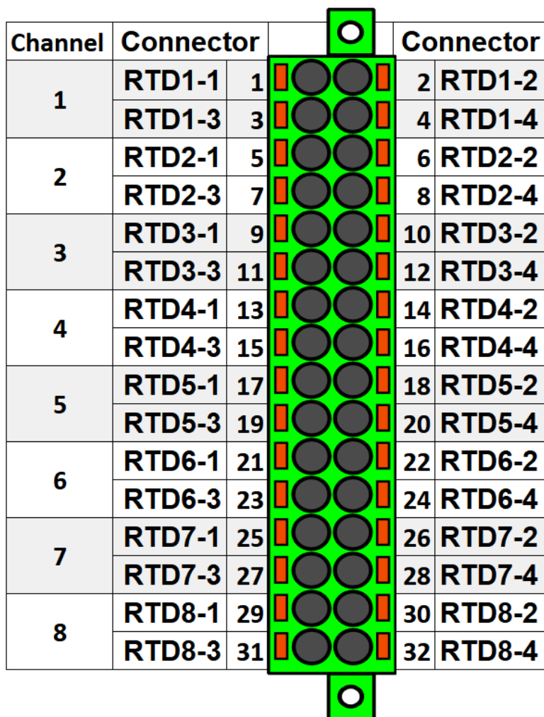
Figure. 8.8 - 226. RTD input module connectors.
