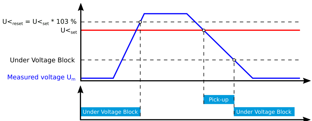
Figure. 5.4.13 - 83. Example of the block setting operation.
