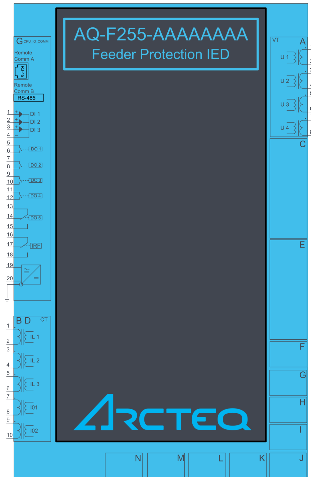
Figure. 7.1 - 206. AQ-F255 variant without add-on modules.
