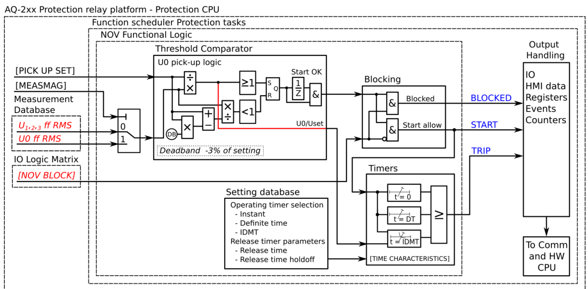
Figure. 5.4.14 - 87. Simplified function block diagram of the U0> function.
