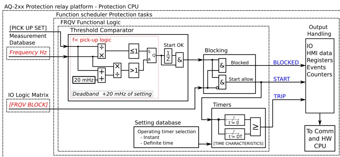
Figure. 5.4.16 - 97. Simplified function block diagram of the f< function.
