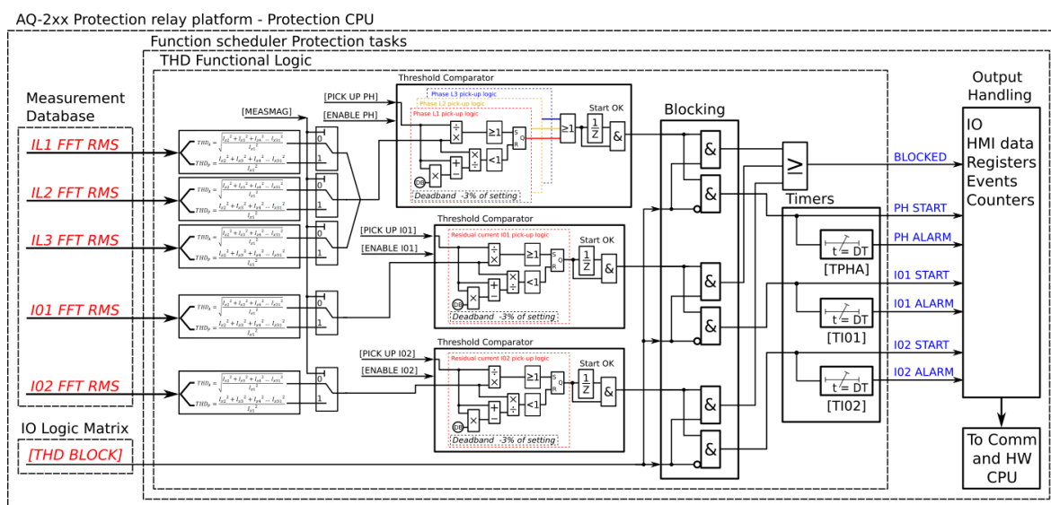
Figure. 5.6.4 - 199. Simplified function block diagram of the total harmonic distortion monitor function.
