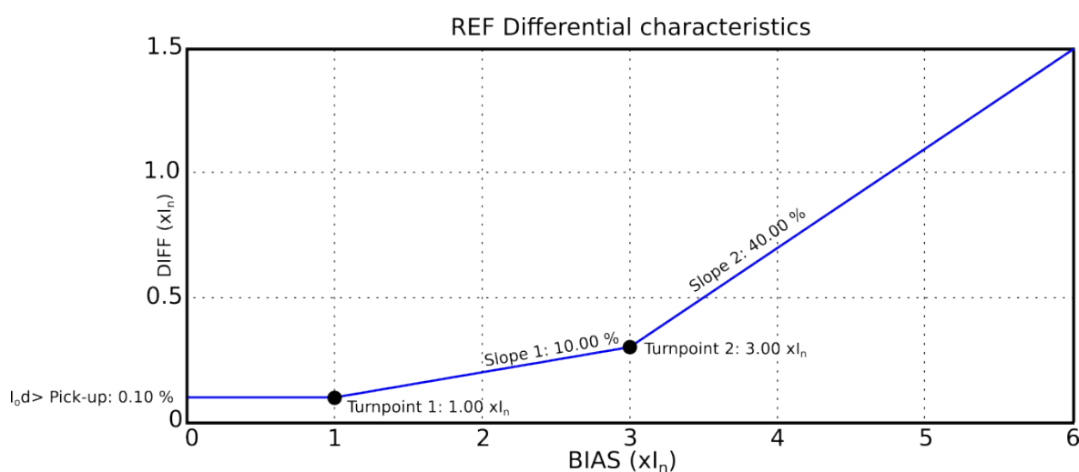
Figure. 5.4.11 - 67. Differential characteristics for the I 0d > function with default settings.
