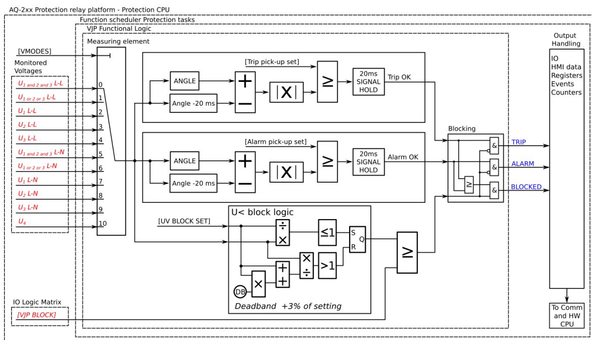
Figure. 5.5.13 - 176. Simplified function block diagram of the \Delta\phi function.
