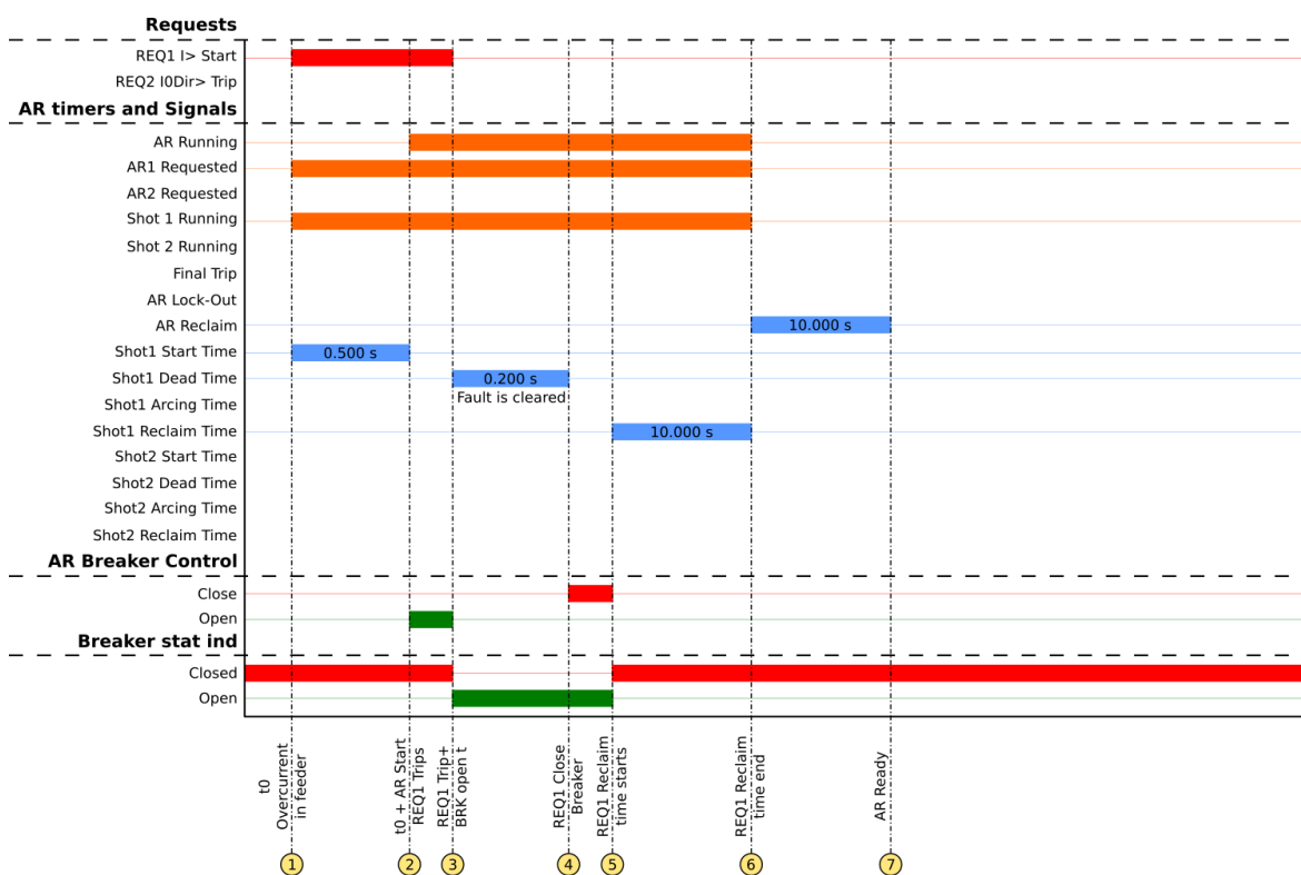
Figure. 5.5.6 - 151. Signal status graph of the transient overcurrent auto-recloser cycle.
