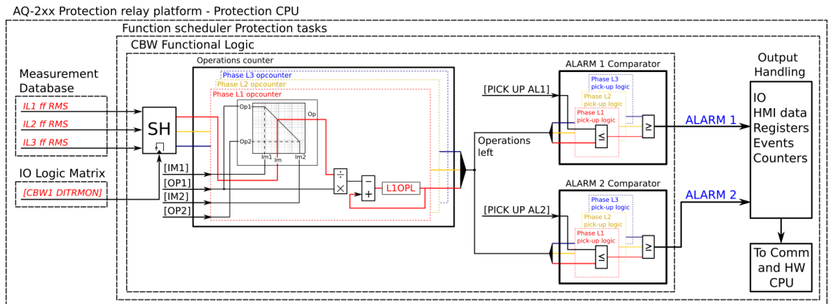
Figure. 5.6.3 - 197. Simplified function block diagram of the circuit breaker wear function.
