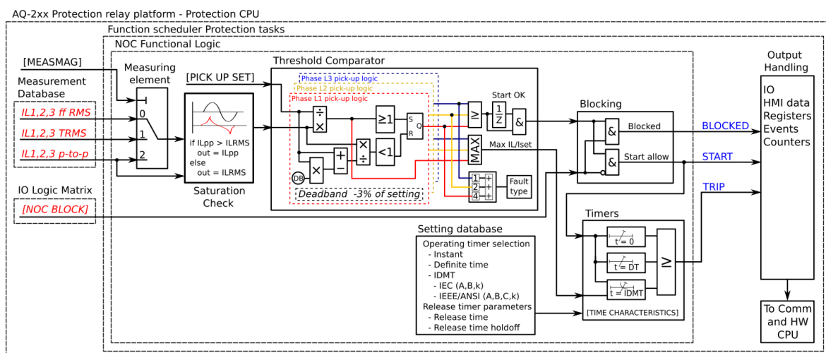
Figure. 5.4.3 - 35. Simplified function block diagram of the I> function.
