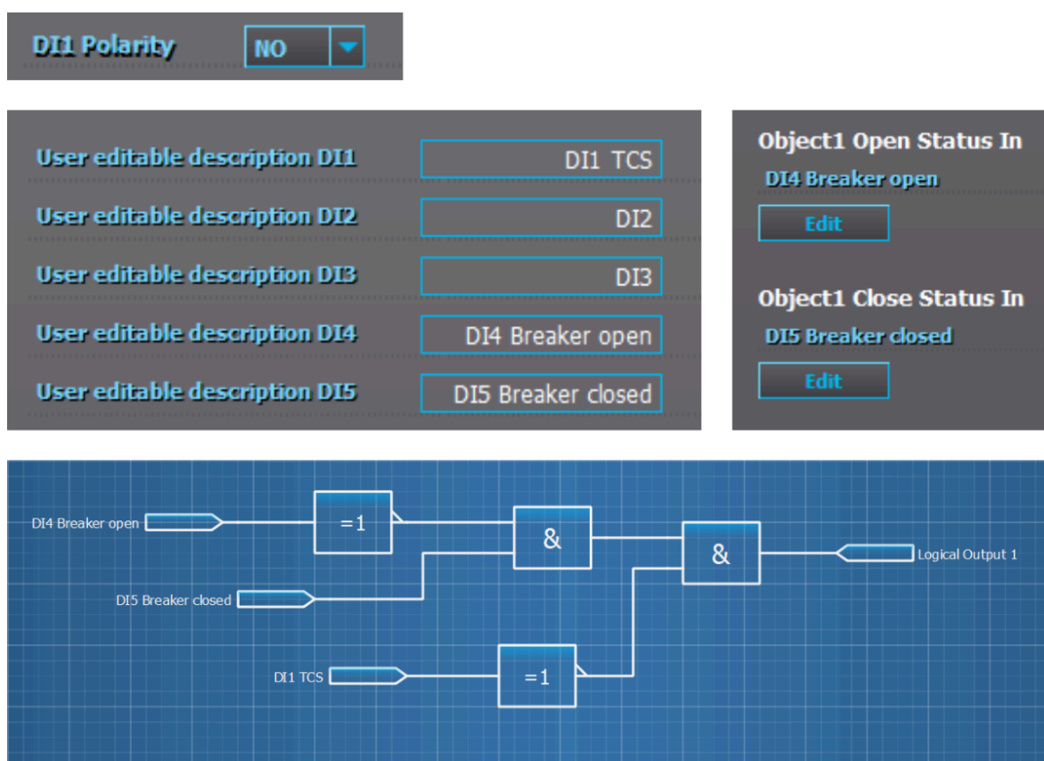
Figure. 7.4 - 215. Example block scheme.
