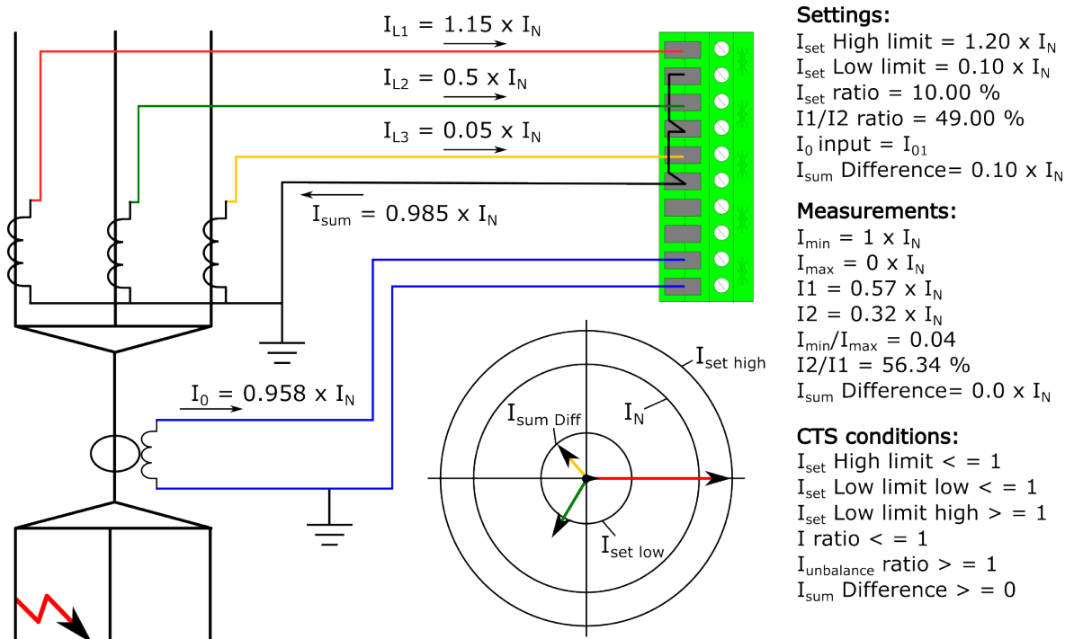
Figure. 5.6.1 - 193. Primary side high-impedance earth fault.
