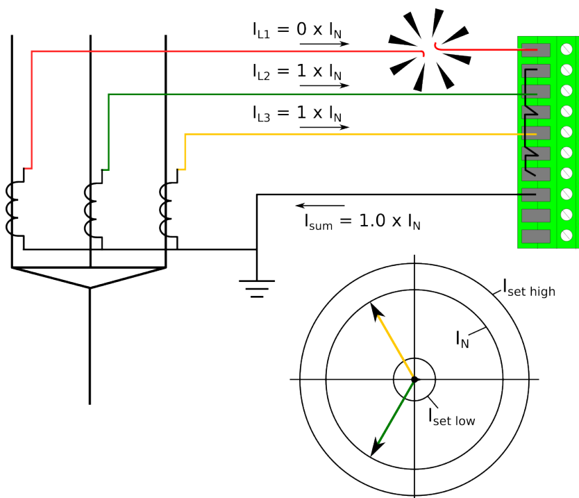
Figure. 5.6.1 - 186. Secondary circuit fault in phase L1 wiring.
