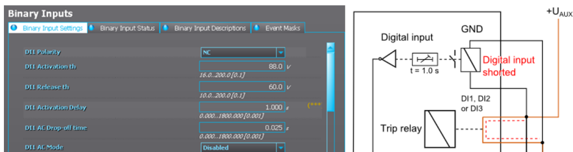
Figure. 7.4 - 212. Settings for a digital input used for trip circuit supervision.
