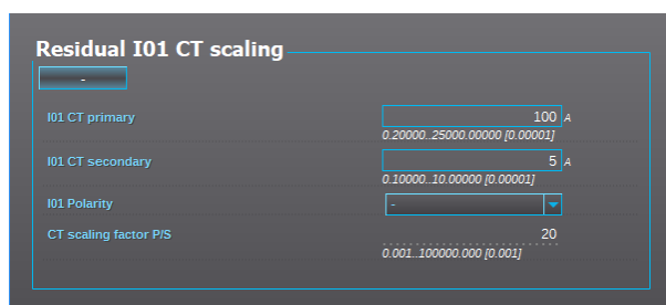
Figure. 5.2.1 - 6. Residual I01 CT scaling (coarse).
