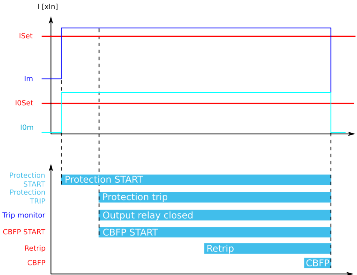
Figure. 5.4.10 - 58. Retrip and CBFP when "Current and DO" is the selected criterion.
