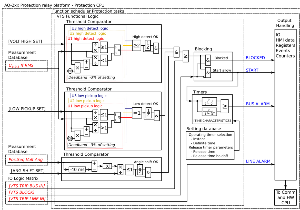
Figure. 5.6.2 - 195. Simplified function block diagram of the VTS function.
