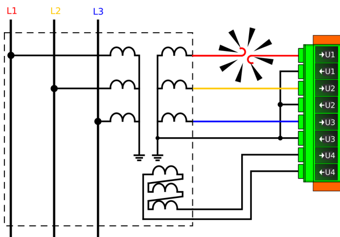
Figure. 5.6.2 - 194. Secondary circuit fault in phase L1 wiring.
