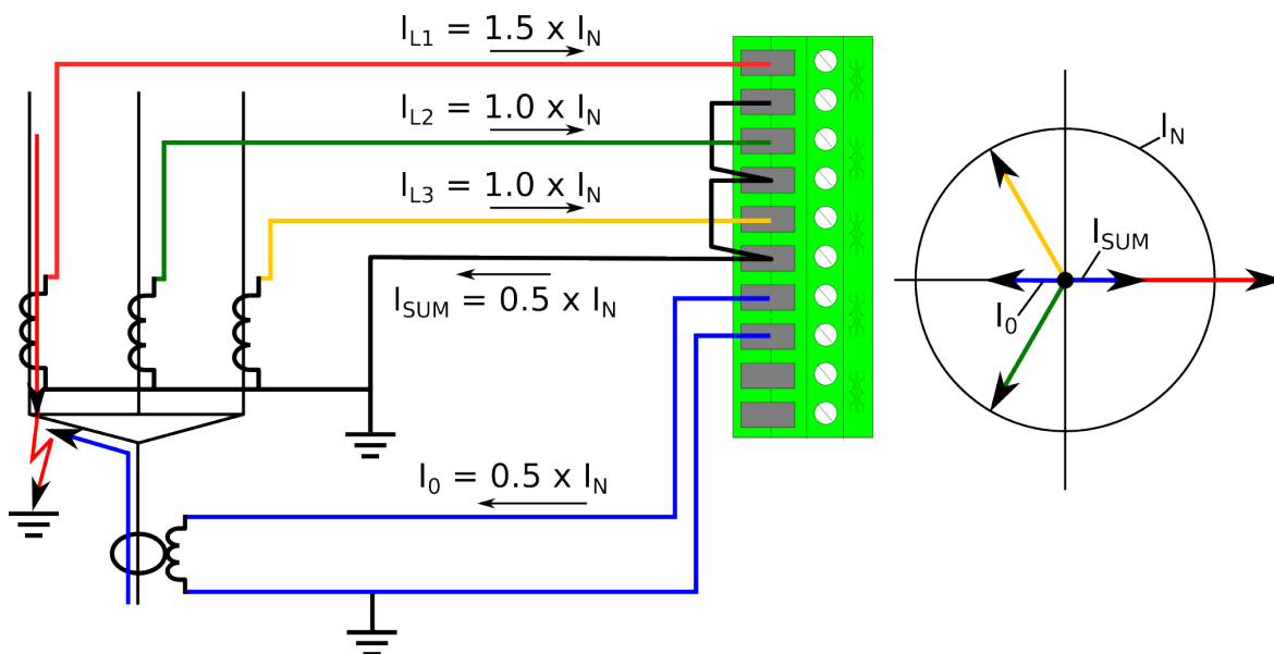
Figure. 5.4.11 - 72. Cable end differential when a fault occurs.
