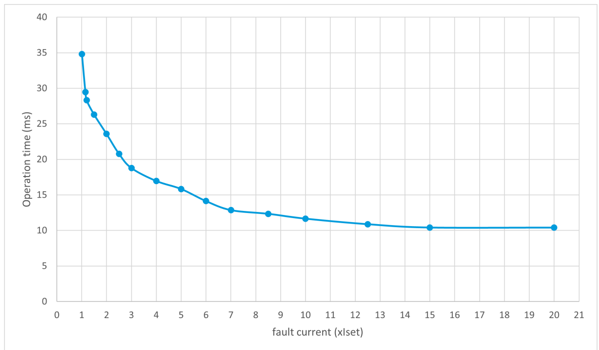
Figure. 5.4.3 - 36. Typical operation time delays with different current to setting ratios in instant operation mode.
