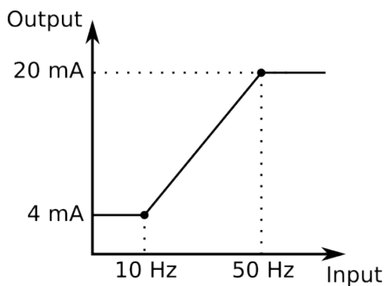
Figure. 5.5.11 - 174. Example of the effects of mA output channel settings.
