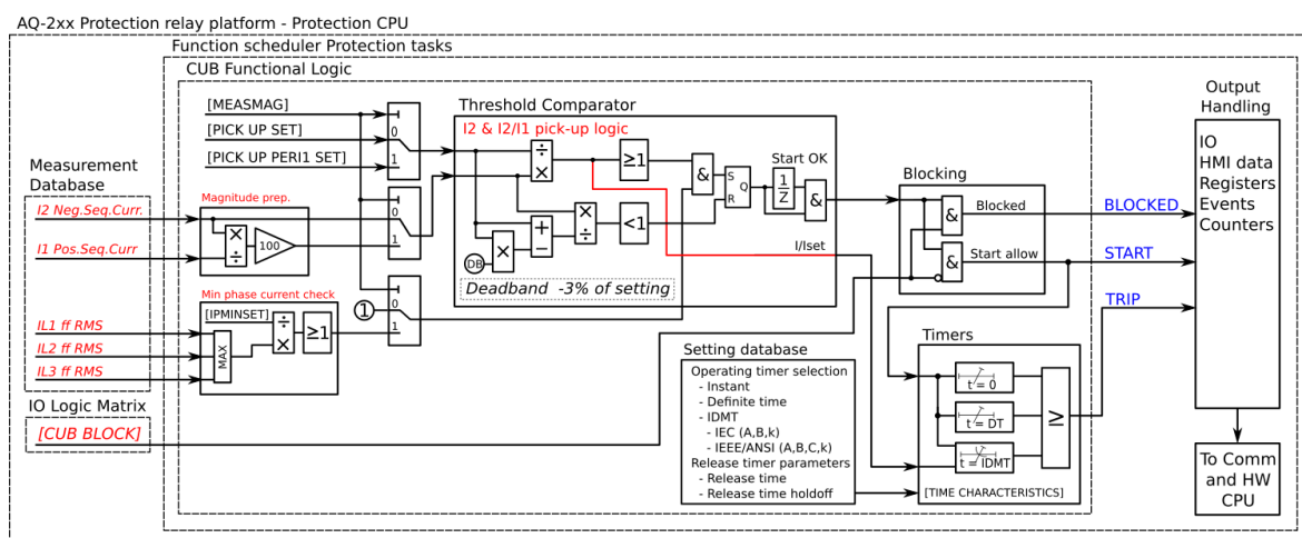
Figure. 5.4.8 - 52. Simplified function block diagram of the I2> function.
