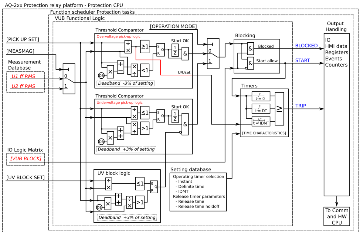
Figure. 5.4.15 - 94. Simplified function block diagram of the U1/U2>/< function.
