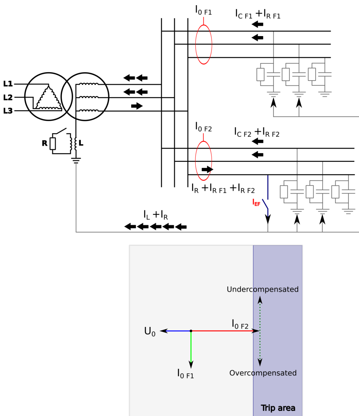
Figure. 5.4.6 - 44. Angle tracking of I_{0dir} function (Petersen coil earthed network model).
