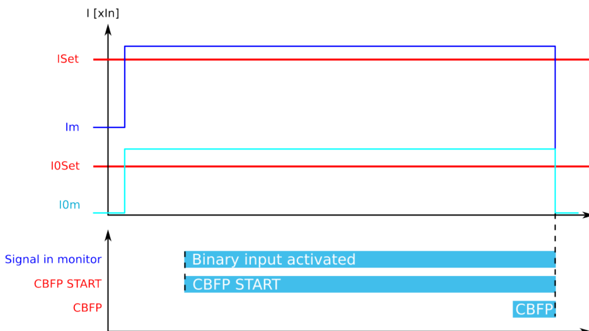
Figure. 5.4.10 - 65. Dedicated CBFP operation from digital input signal.
