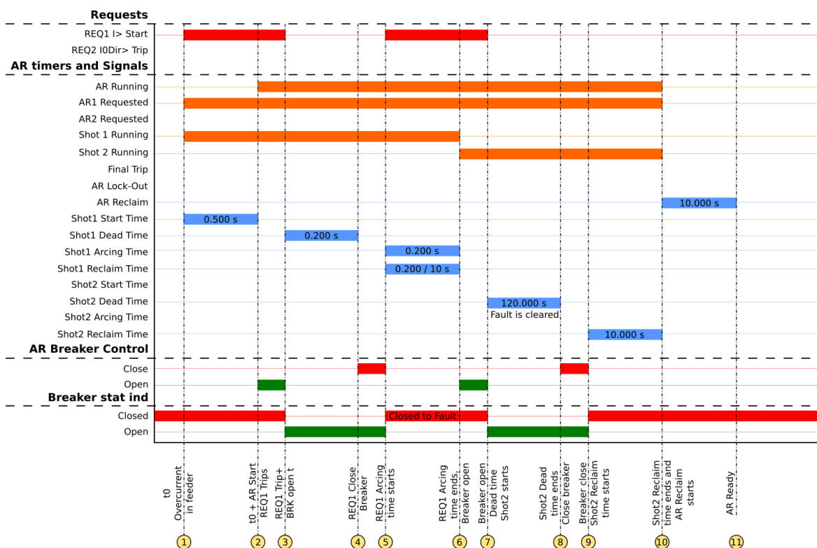
Figure. 5.5.6 - 149. Signal status graph of the semi-permanent overcurrent auto-recloser cycle.
