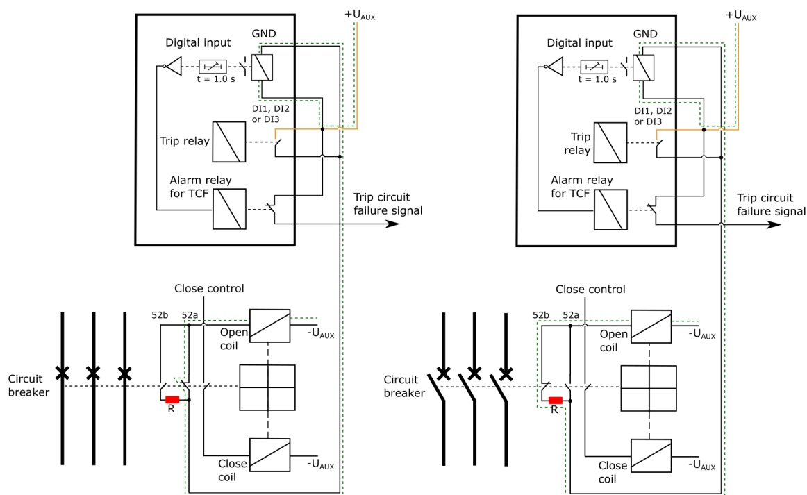
Figure. 7.4 - 211. Trip circuit supervision with one DI and one non-latched trip output.
