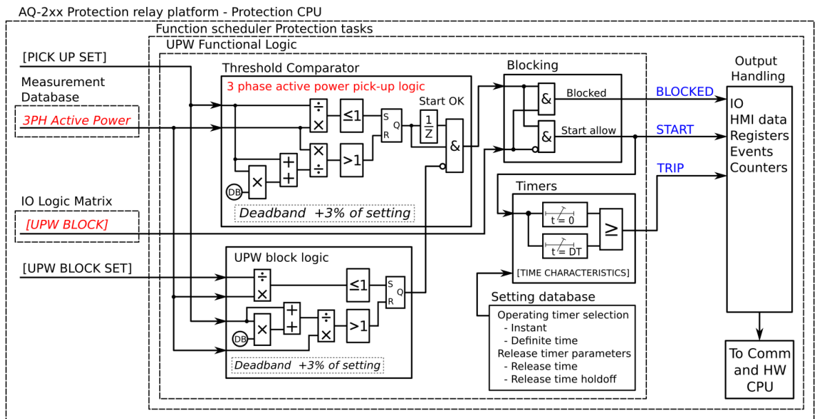
Figure. 5.4.19 - 103. Simplified function block diagram of the P< function.
