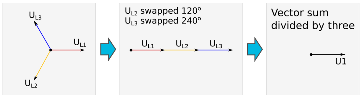
Figure. 5.4.15 - 89. Earth fault in an isolated network.
