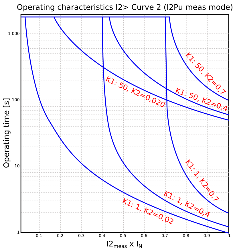
Figure. 5.4.8 - 53. Operation characteristics curve for I2> Curve2.
