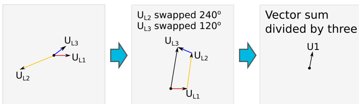
Figure. 5.4.15 - 93. Close-distance short-circuit between phases 1 and 3.
