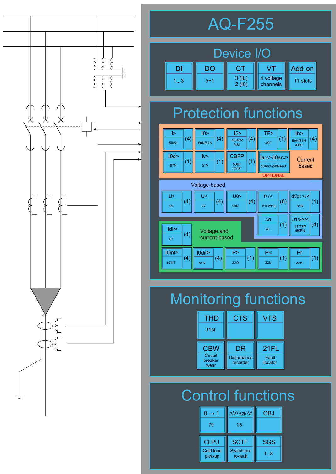
Figure. 7.1 - 208. AQ-F255 application example with function block diagram.
