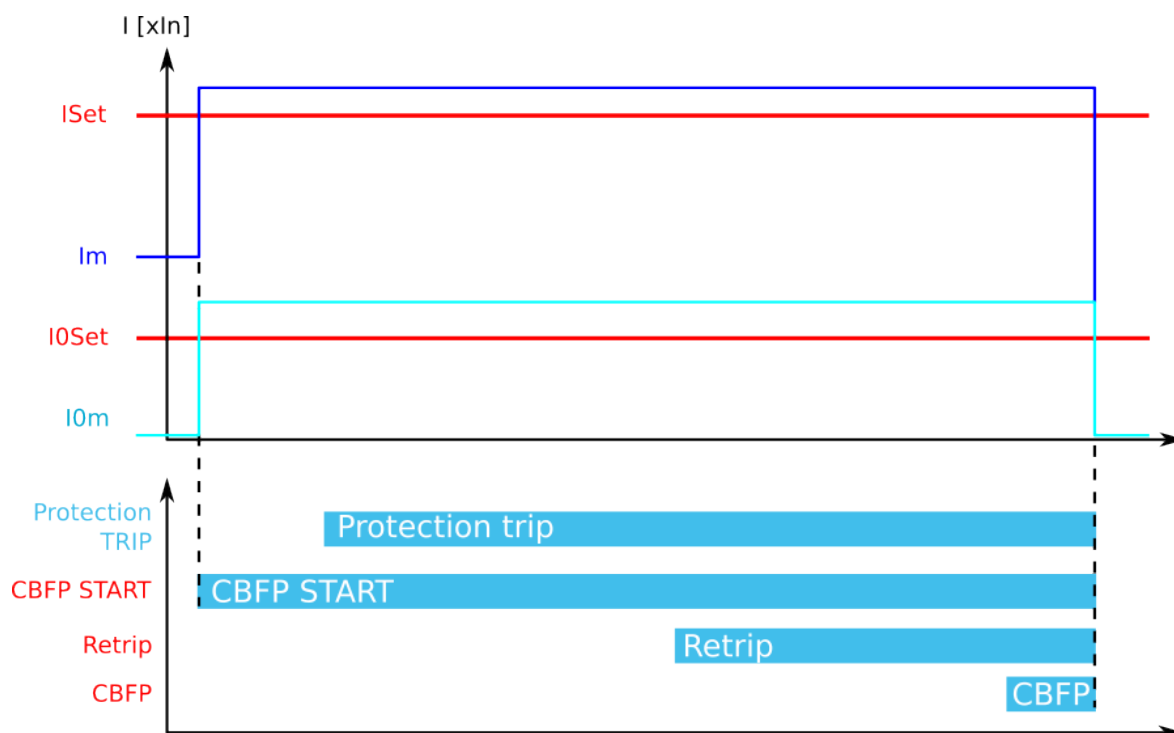
Figure. 5.4.10 - 57. Retrip and CBFP when "Current" is the selected criterion.
