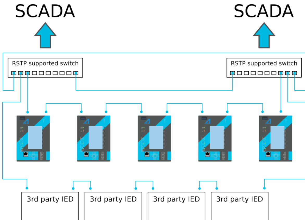
Figure. 8.11 - 231. Example of a ring configuration.
