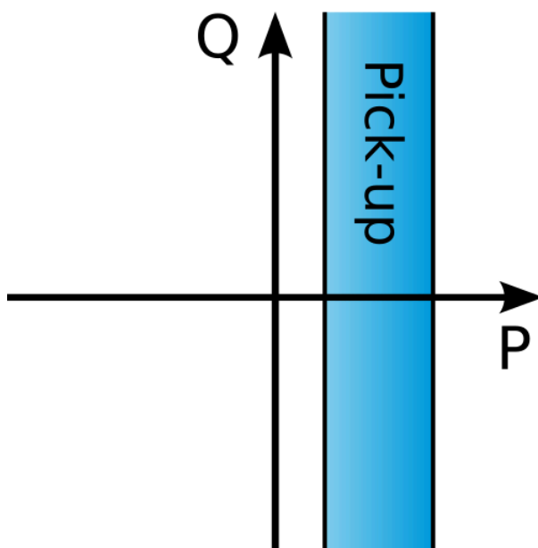
Figure. 5.4.19 - 102. Operating characteristics of underpower protection.
