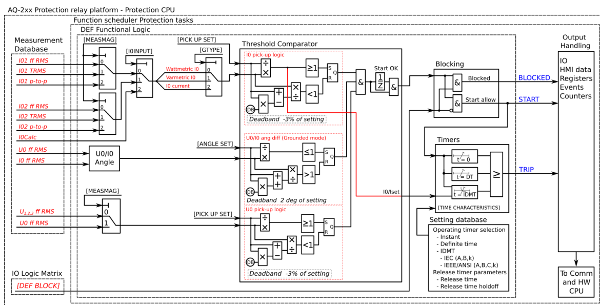
Figure. 5.4.6 - 42. Simplified function block diagram of the I0dir&gt; function.
