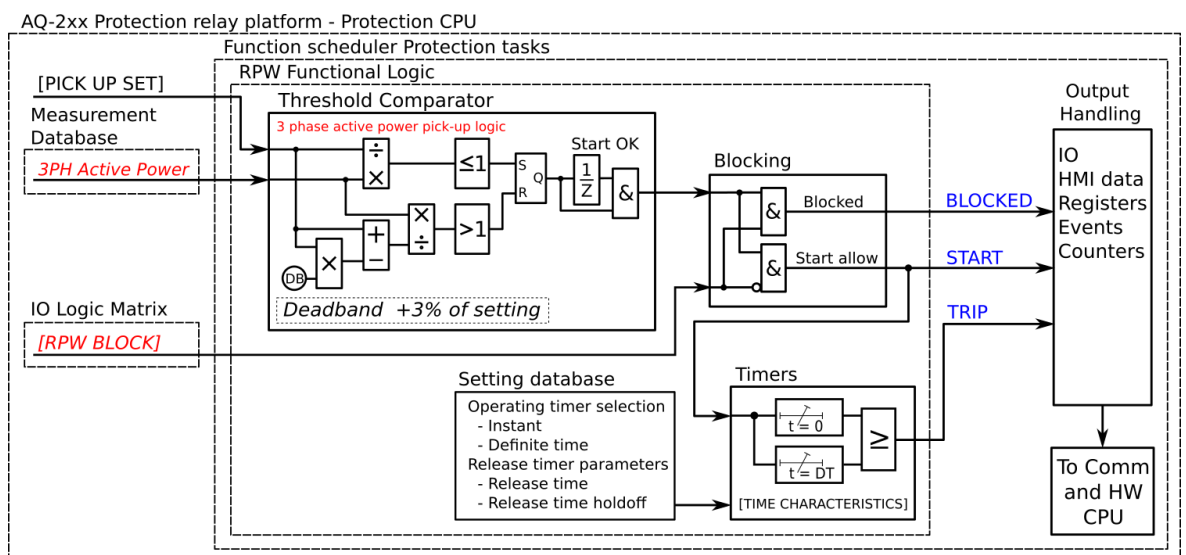
Figure. 5.4.20 - 106. Simplified function block diagram of the Pr function.
