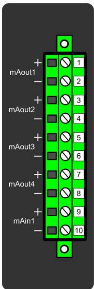
Figure. 8.13 - 235. Milliampere (mA) I/O module connections.
