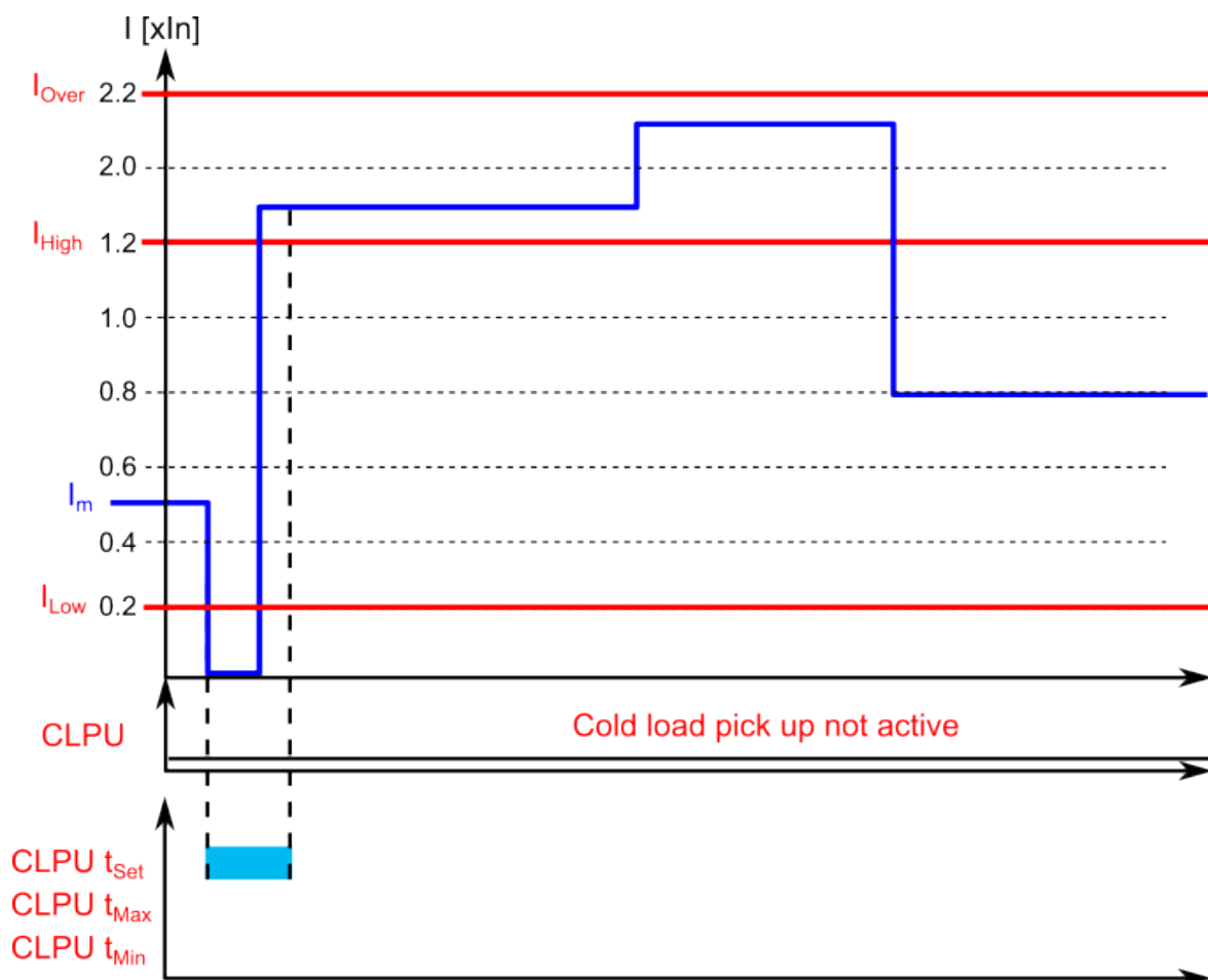
Figure. 5.5.8 - 158. Example of timers and pick-up parameters (no cold load pick-up, I_{low} too short).
