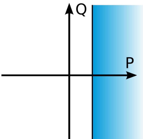
Figure. 5.4.18 - 100. Operating characteristics of overpower protection.
