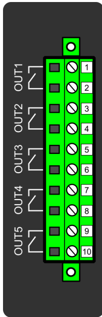
Figure. 8.6 - 224. Digital output module (DO5) with five add-on digital outputs.
