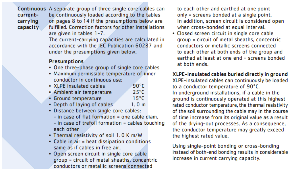
Figure. 5.4.22 - 115. General presumptions of high-voltage cables.
