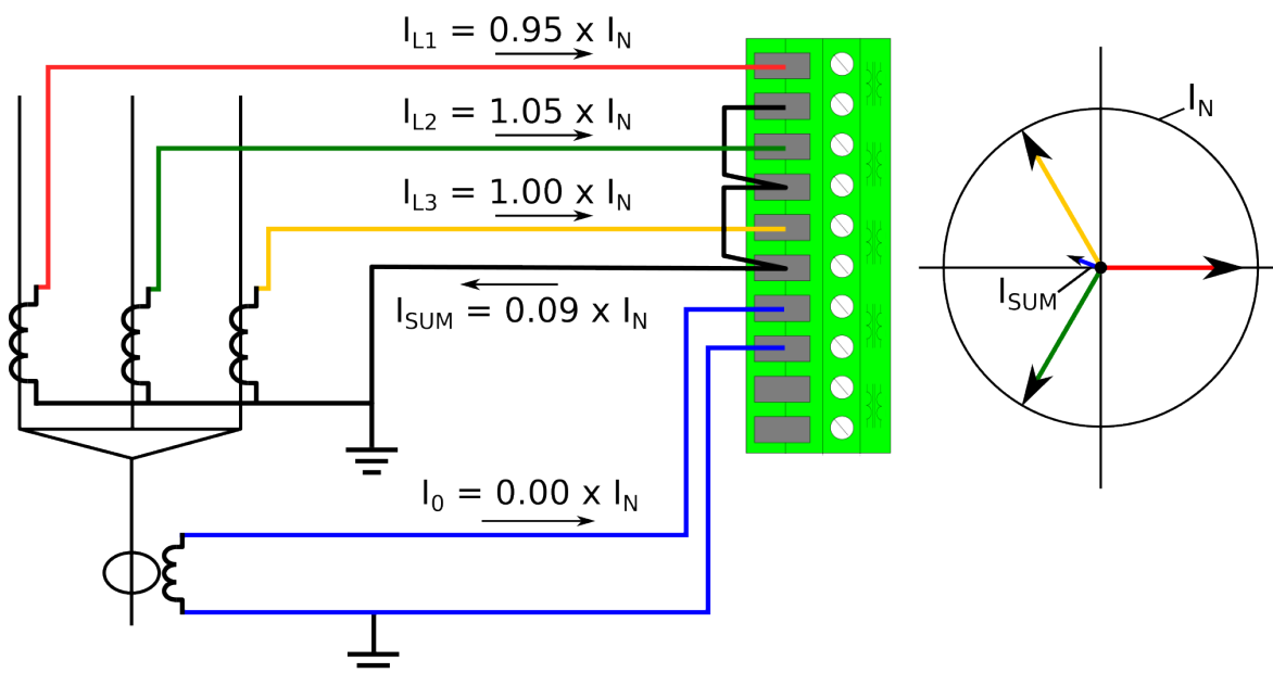
Figure. 5.4.11 - 71. Cable end differential with natural unbalance in the phase current measurement.
