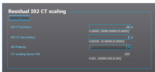
Figure. 5.2.1 - 7. Residual I02 CT scaling (sensitive).
