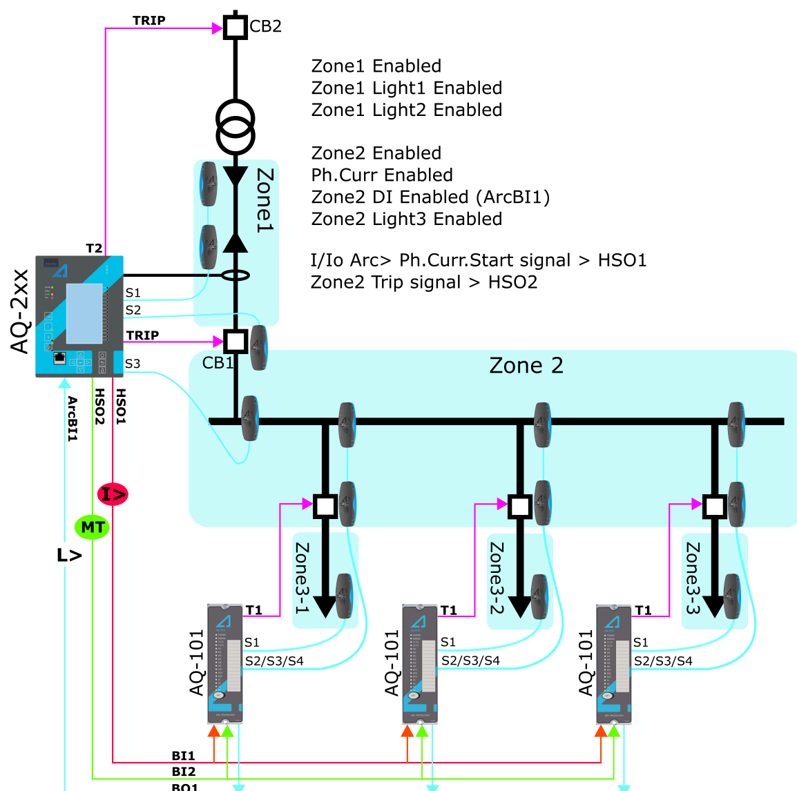
Figure. 5.4.23 - 123. Scheme IA1 (with AQ-101 arc protection relays).
