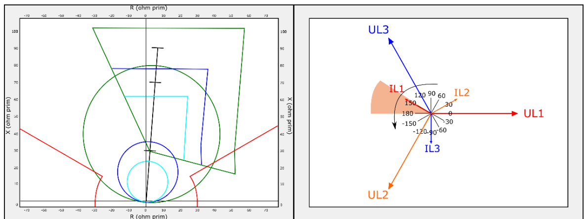
Figure. 5.4.24 - 125. Distance protection characteristics and directional overcurrent.
