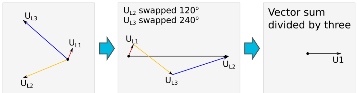
Figure. 5.4.15 - 90. Close-distance short-circuit between phases 1 and 3.
