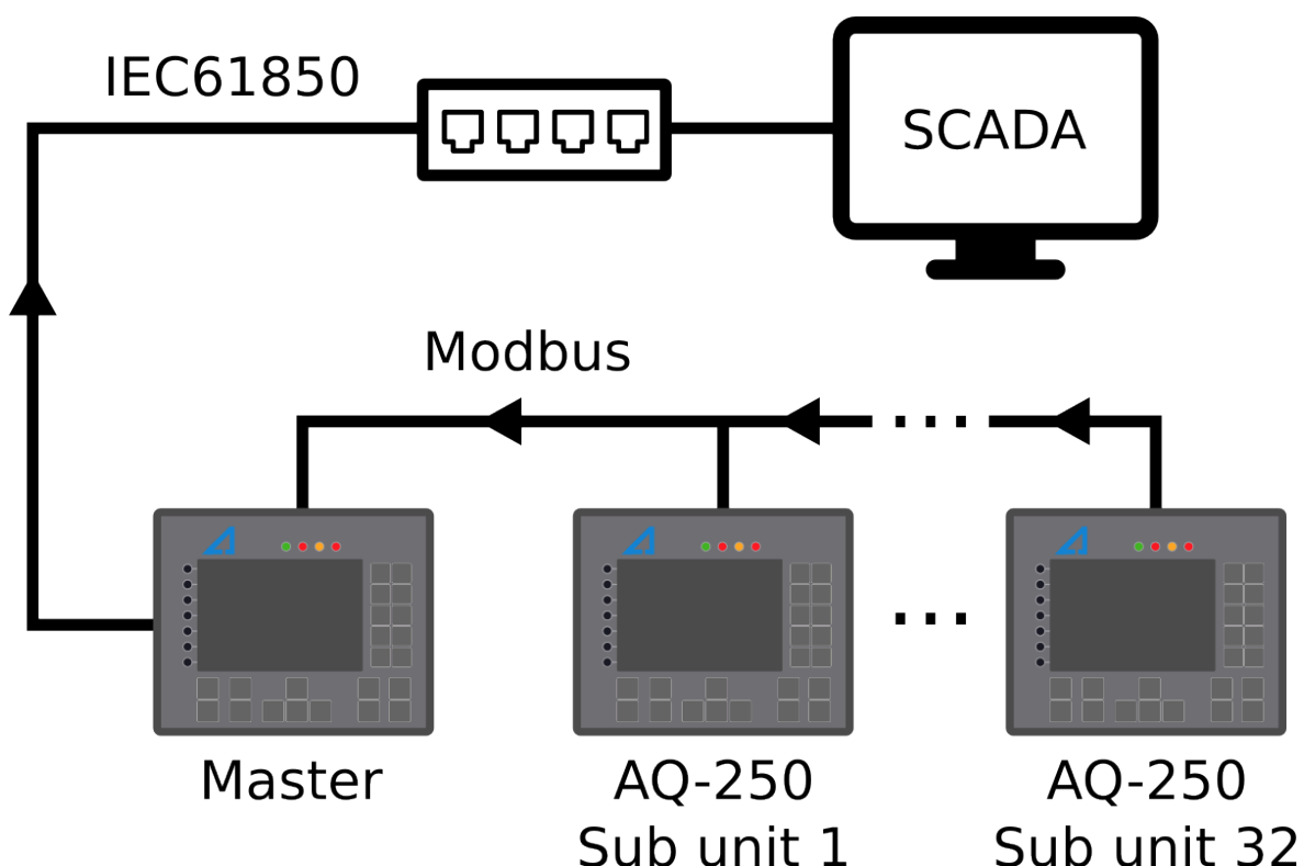
Figure. 6.6 - 205. Example setup of Modbus Gateway application.
