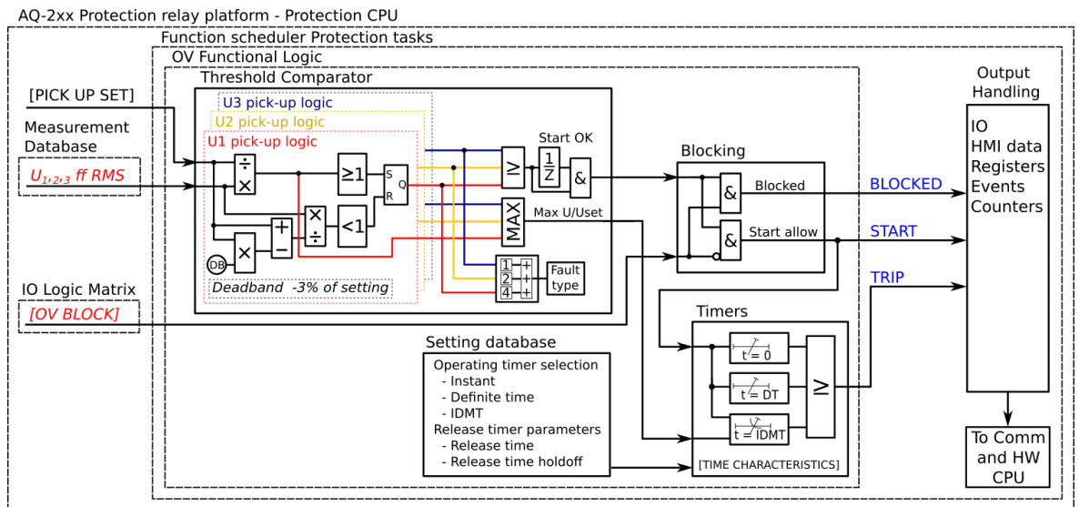
Figure. 5.4.12 - 75. Simplified function block diagram of the U> function.
