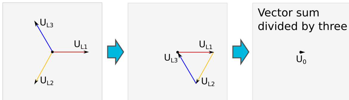
Figure. 5.4.14 - 85. Earth fault in isolated network.
