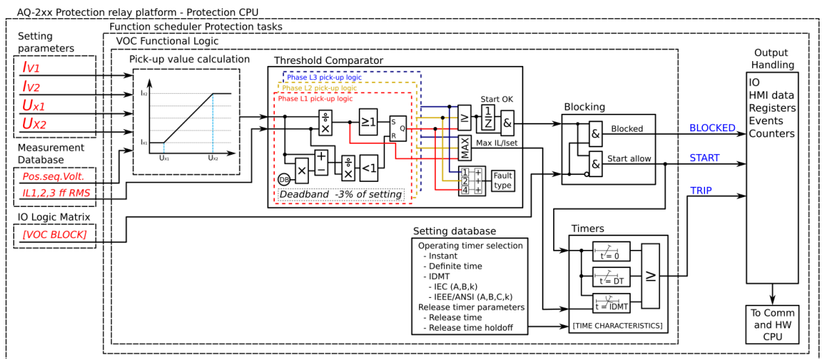
Figure. 5.4.21 - 108. Simplified function block diagram of the I_{V>} function.
