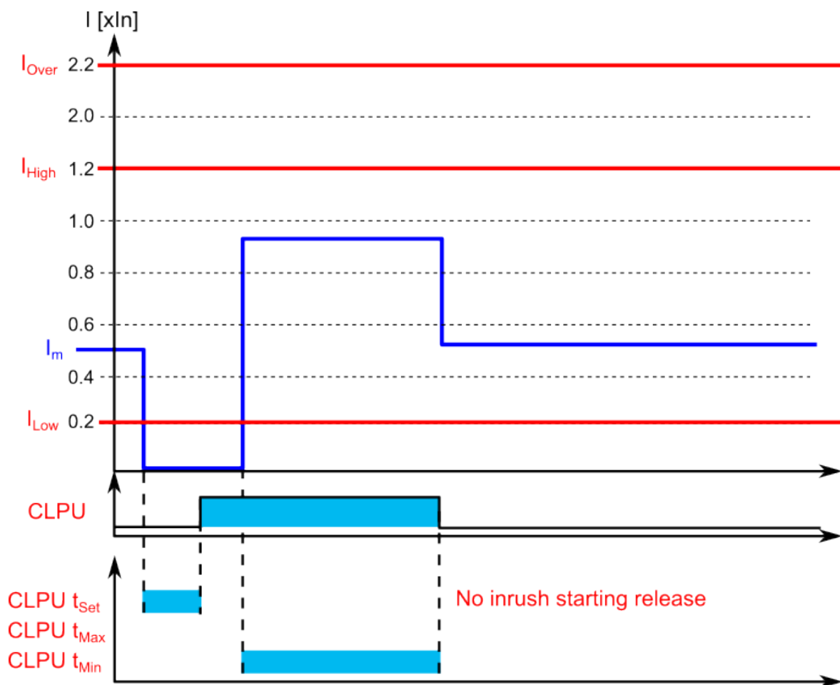
Figure. 5.5.8 - 161. Example of timers and pick-up parameters (no inrush current detected in the starting).
