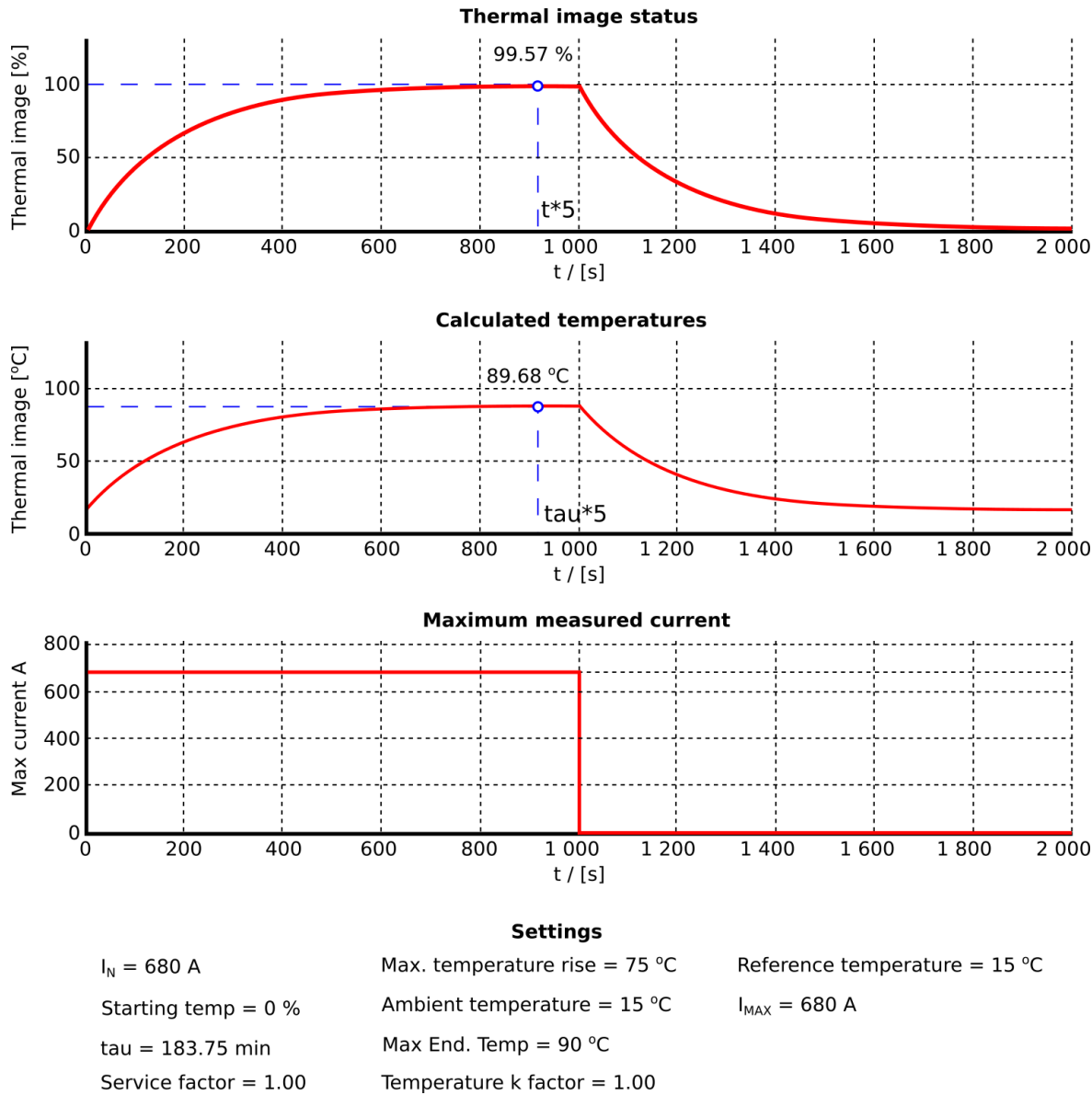
Figure. 5.4.22 - 118. Thermal image response with maximum load (installation according presumptions).
