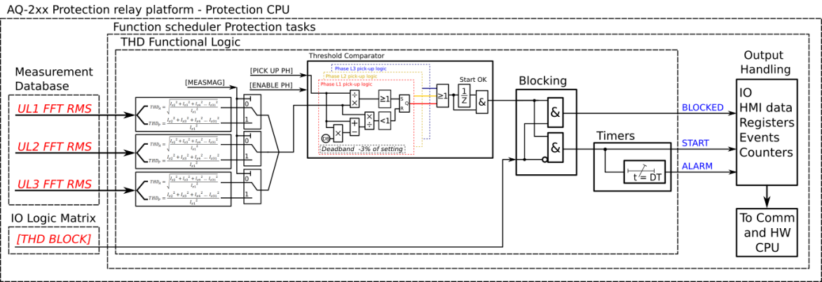
Figure. 5.6.5 - 201. Simplified function block diagram of the total harmonic distortion monitor function.
