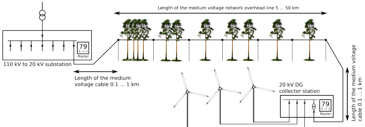
Figure. 5.5.6 - 152. Auto-reclosing with distributed generation in the line.
