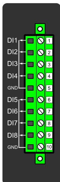
Figure. 8.5 - 222. Digital input module (DI8) with eight add-on digital inputs.
