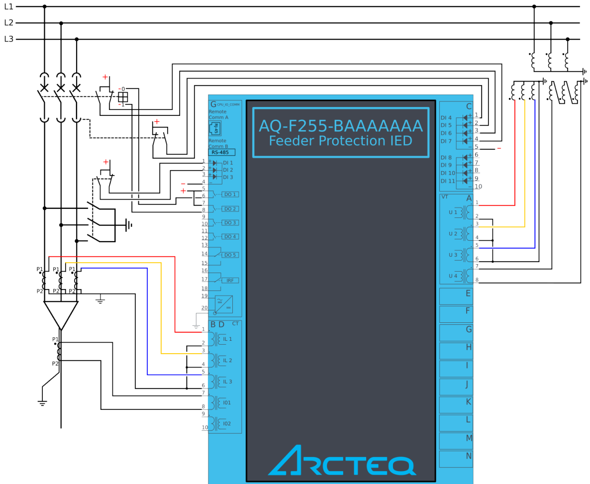
Figure. 7.2 - 209. Application example and its connections.
