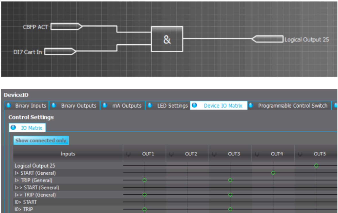
Figure. 5.5.17 - 180. Logic output example. Logical output is connected to an output relay in matrix.
