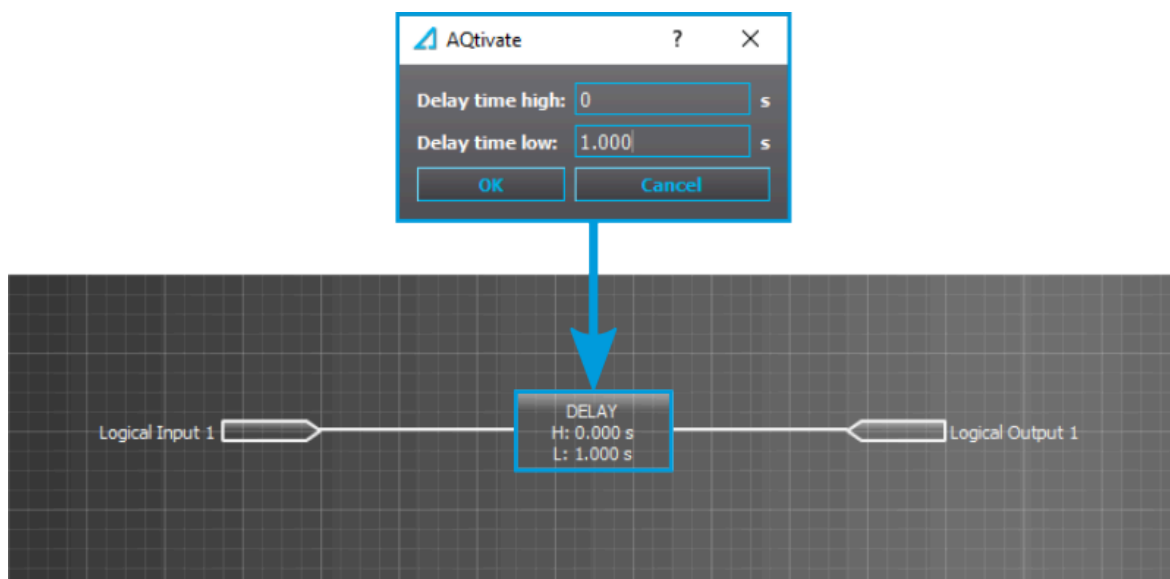
Figure. 5.5.18 - 182. Extending a logical input pulse.
