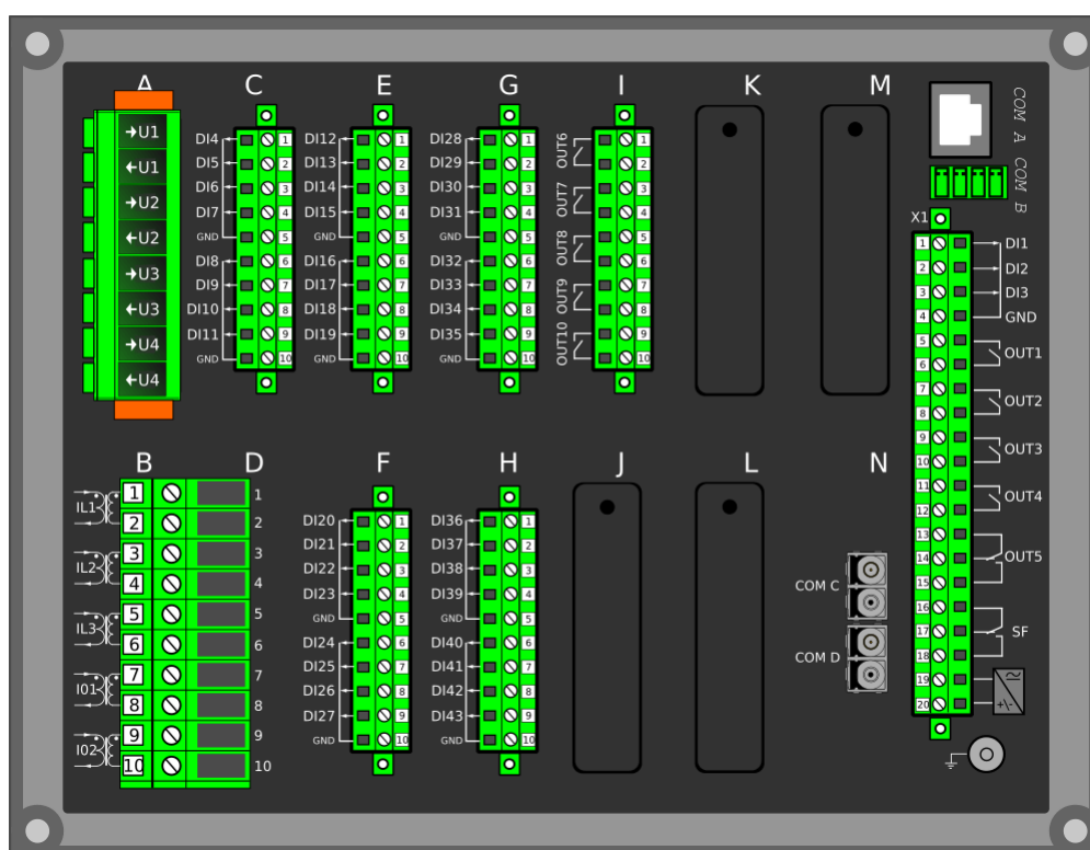
Figure. 8.1 - 217. Modular construction of AQ-X255-XXXXXXX-BBBBBBAAAAJ
