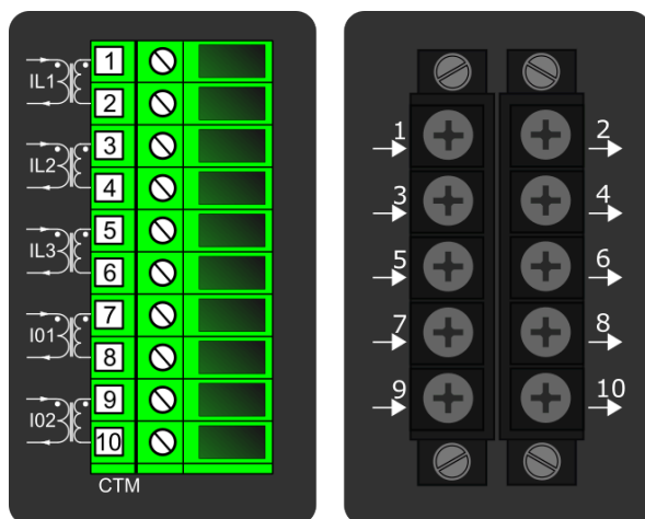
Figure. 8.3 - 220. Module connections with standard and ring lug terminals.
