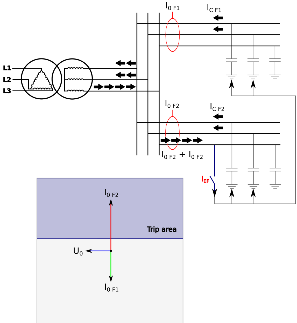
Figure. 5.4.6 - 43. Angle tracking of I_{0dir} function (unearthed network model) (32N)
