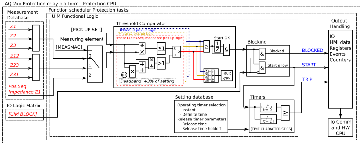
Figure. 5.4.23 - 122. Simplified function block diagram of the Z< function.
