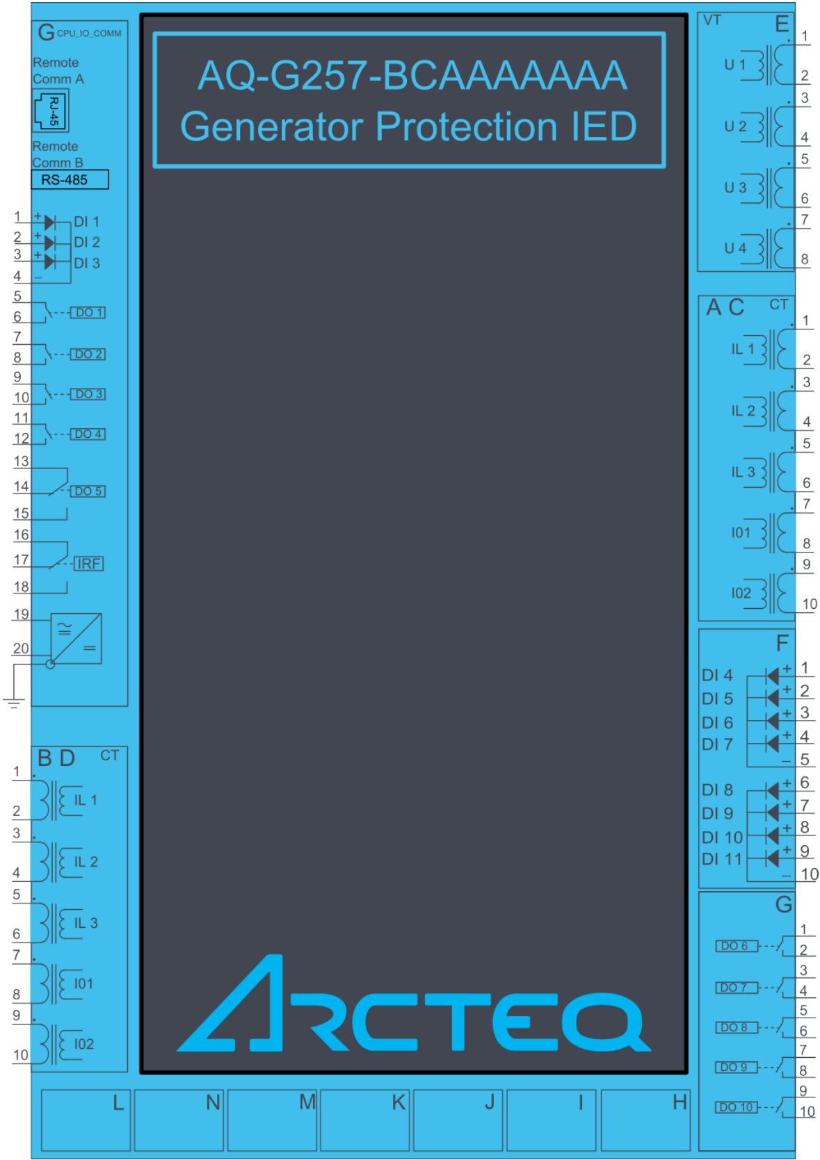
Figure. 7.1 - 212. AQ-G257 variant with digital input and output modules.
