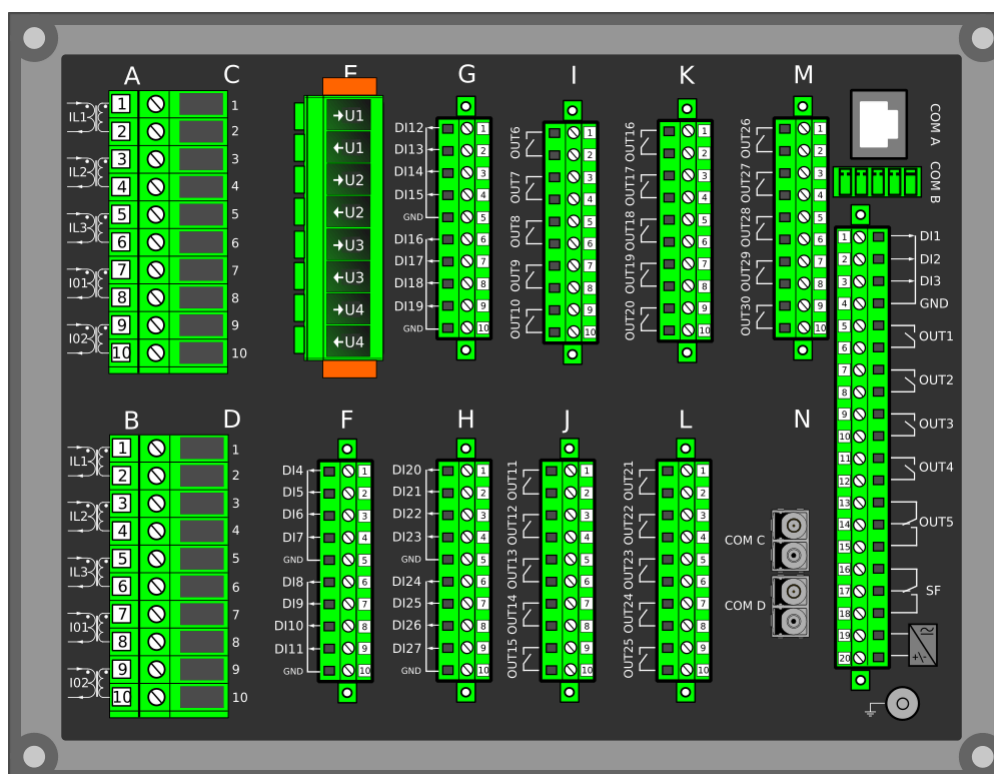
Figure. 8.1 - 222. Modular construction of AQ-X257-XXXXXXX-BBBCCCCCJ
