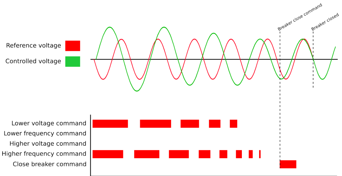
Figure. 5.5.9 - 184. Simplified presentation of synchronizer operation
