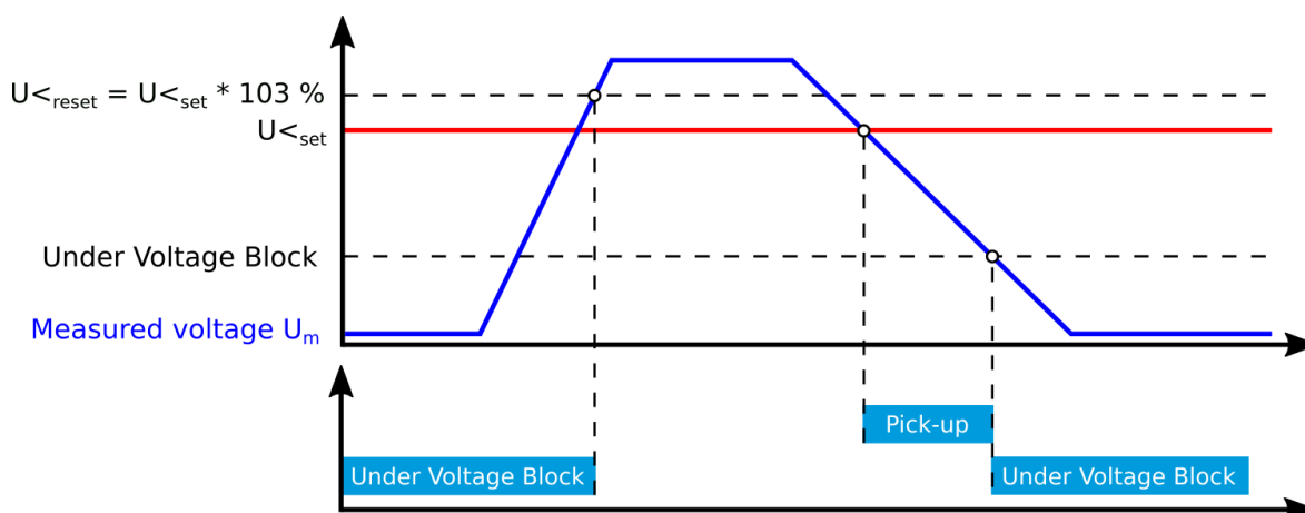
Figure. 5.4.12 - 76. Example of the block setting operation.
