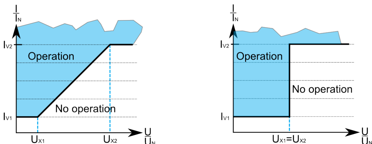
Figure. 5.4.21 - 115. Pick-up levels in the two modes.
