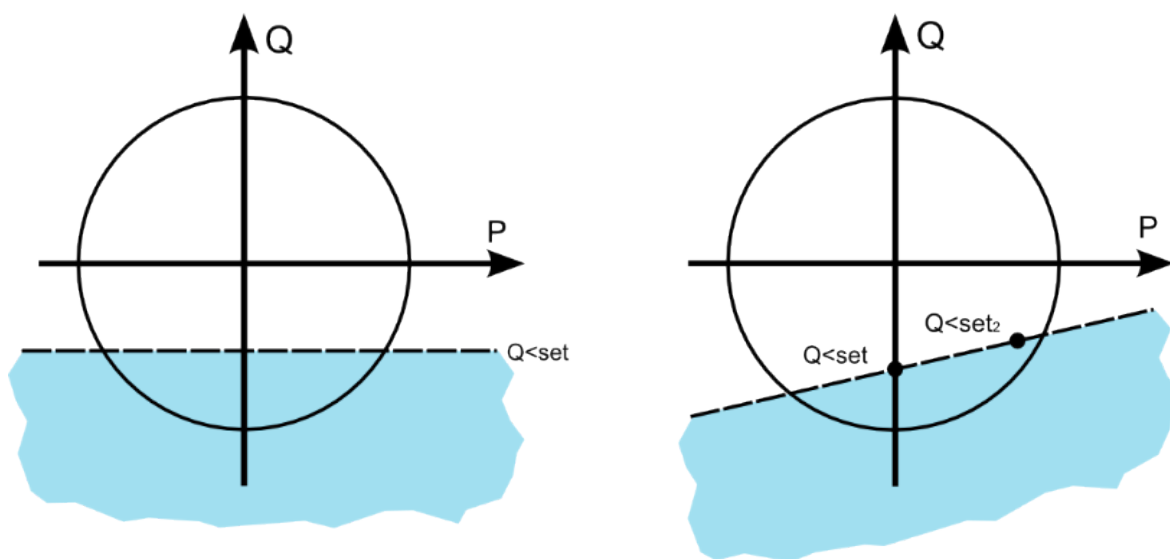
Figure. 5.4.18 - 110. Underexcitation modes.
