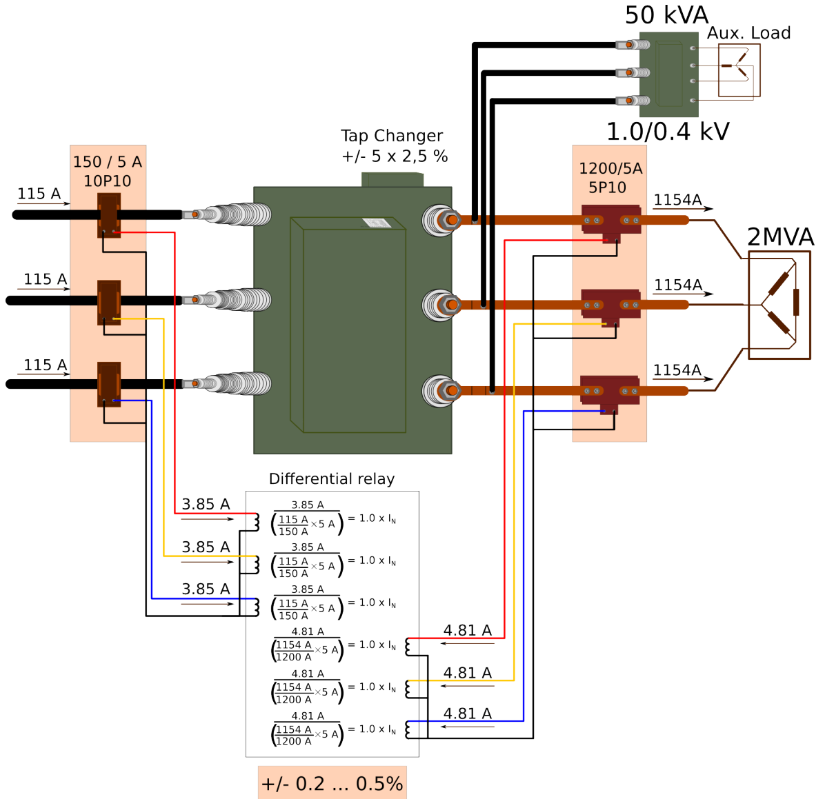
Figure. 5.4.27 - 140. Differential current sources (normal operation).
