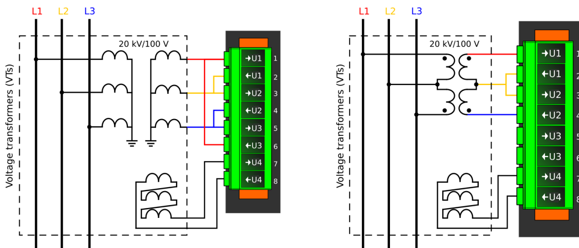
Figure. 5.2.2 - 13. Example connections for voltage line-to-line measurement.
