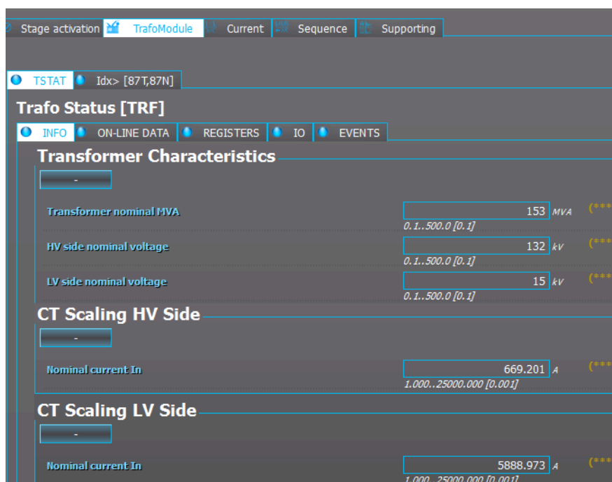
Figure. 5.2.1 - 3. Nominal current calculation in differential protection relays.
