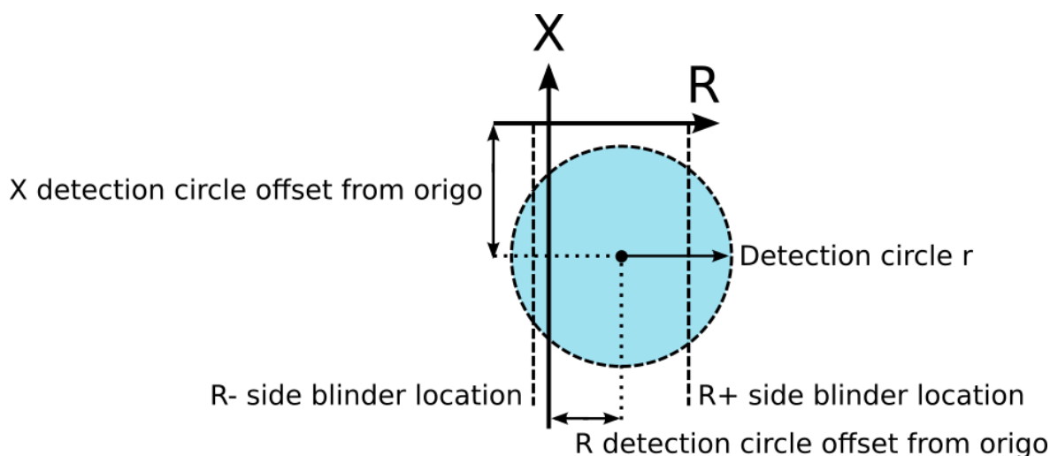
Figure. 5.4.26 - 125. Operating characteristics of pole slip protection.
