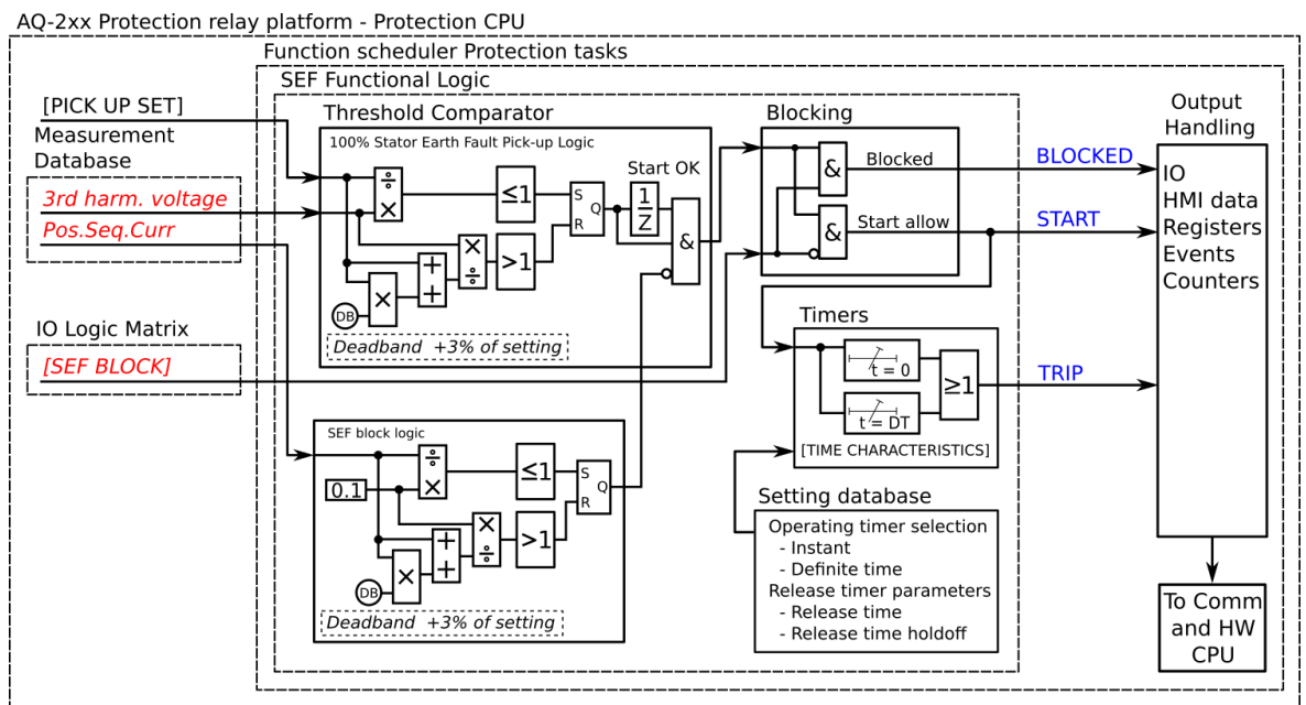
Figure. 5.4.20 - 114. Simplified function block diagram of the U03rd> function.
