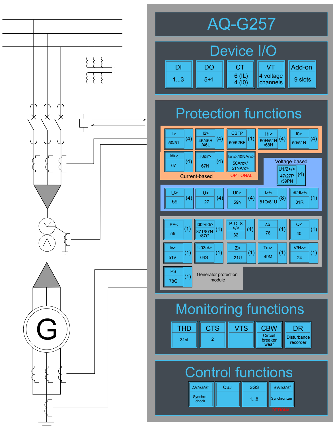
Figure. 7.1 - 213. AQ-G257 application example with function block diagram.
