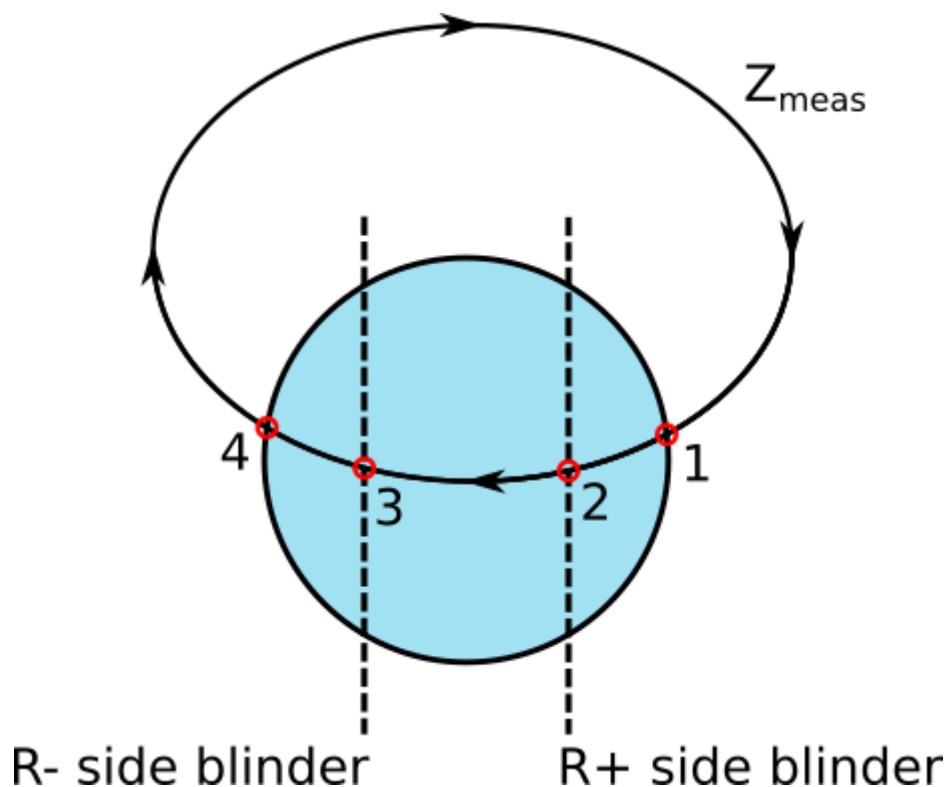
Figure. 5.4.26 - 126. Impedance must enter the circle first then cross the blinders and lastly exit the circle for the function to count a slip. Impedance can enter the circle from either side but it must keep entering the circle from the same side for the function to keep counting the slips.
