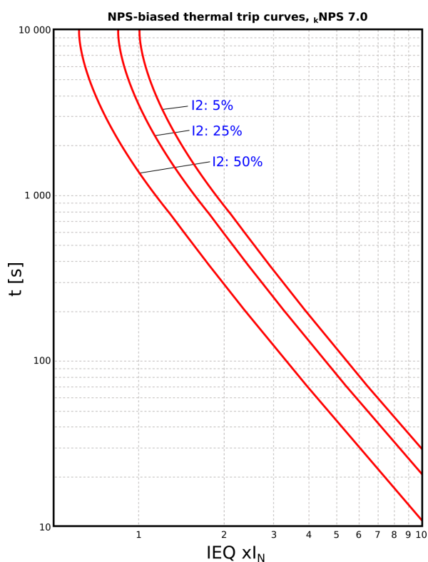
Figure. 5.4.17 - 107. NPS-biased thermal trip curves with k_{NPS} value of 7.
