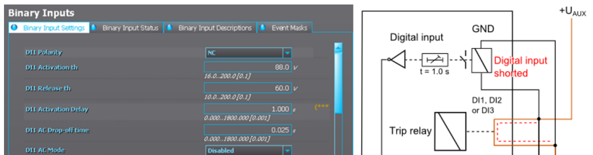
Figure. 7.3 - 217. Settings for a digital input used for trip circuit supervision.
