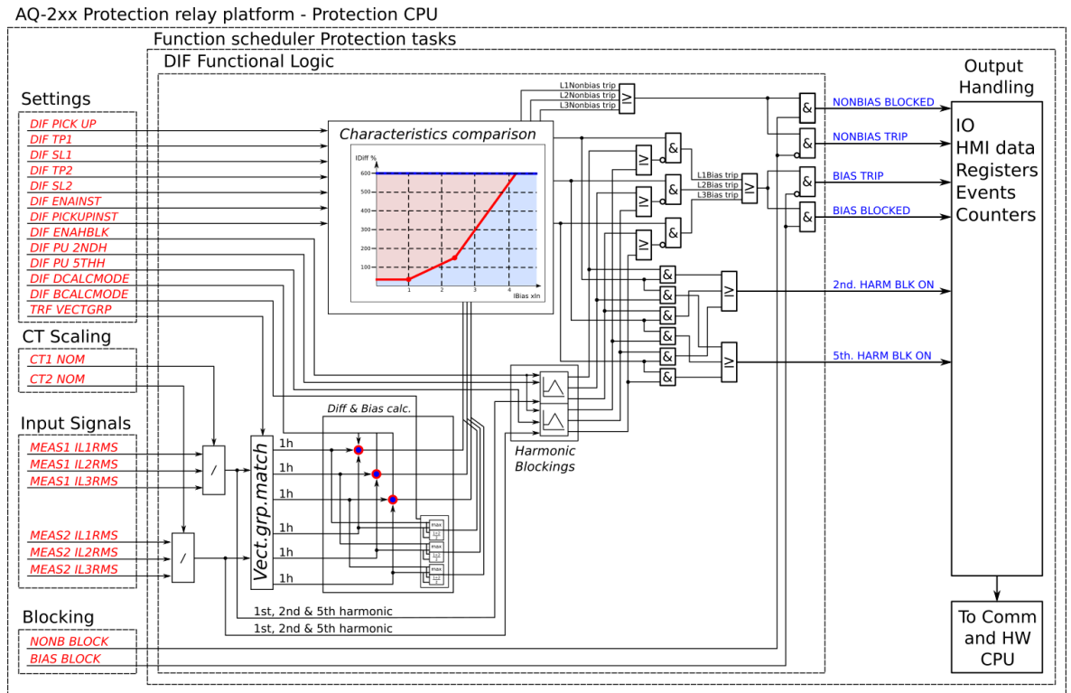
Figure. 5.4.27 - 153. Simplified function block diagram of the transformer differential function.
