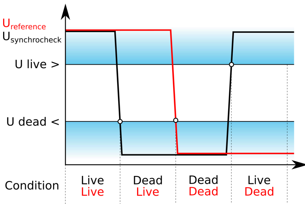
Figure. 5.5.5 - 176. System states.
