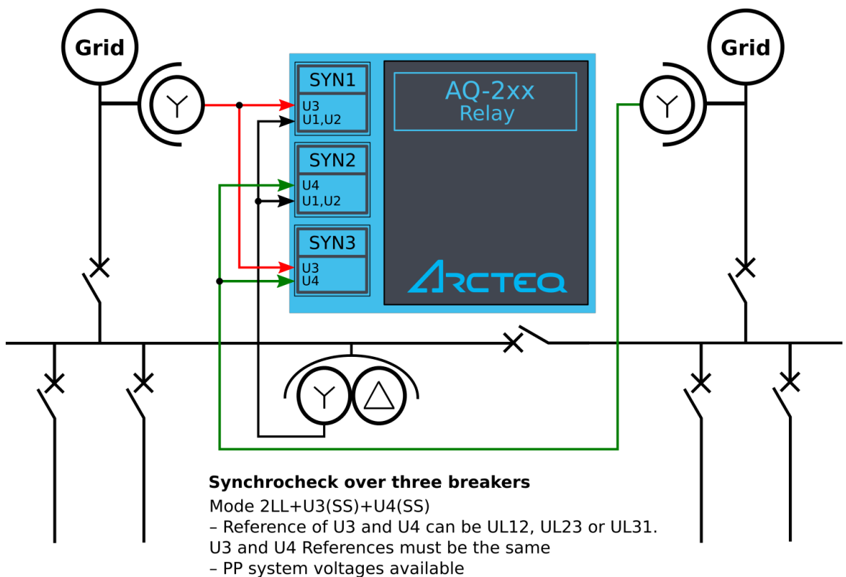
Figure. 5.5.5 - 175. Example application (synchrocheck over three breakers, with 2LL+U3+U4 connection).
