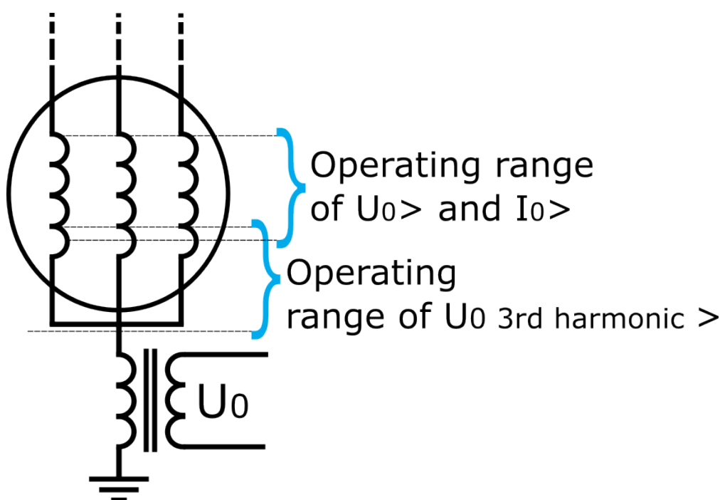
Figure. 5.4.20 - 113. Overlapping demonstration.
