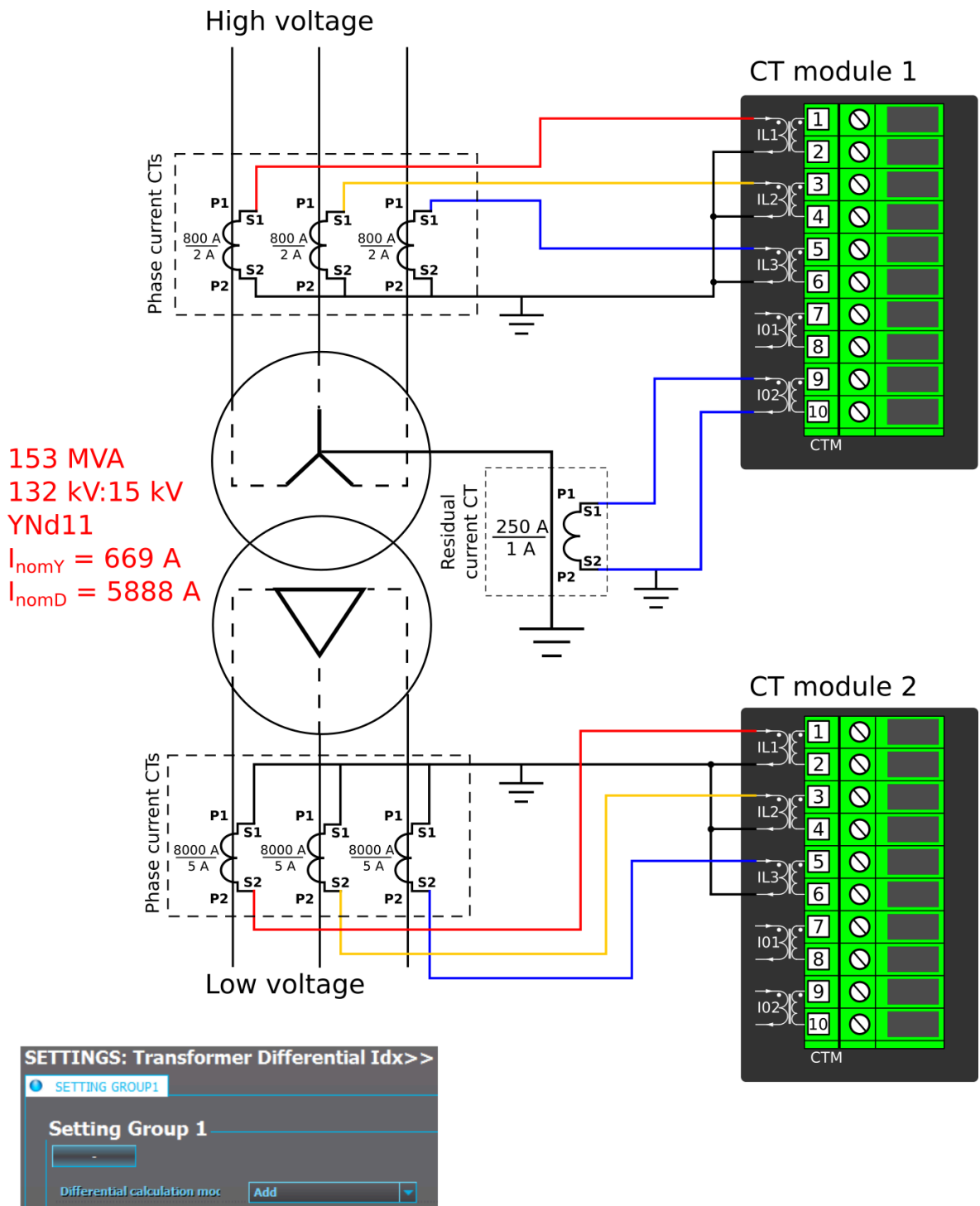
Figure. 5.2.1 - 8. Connections (application 2).
