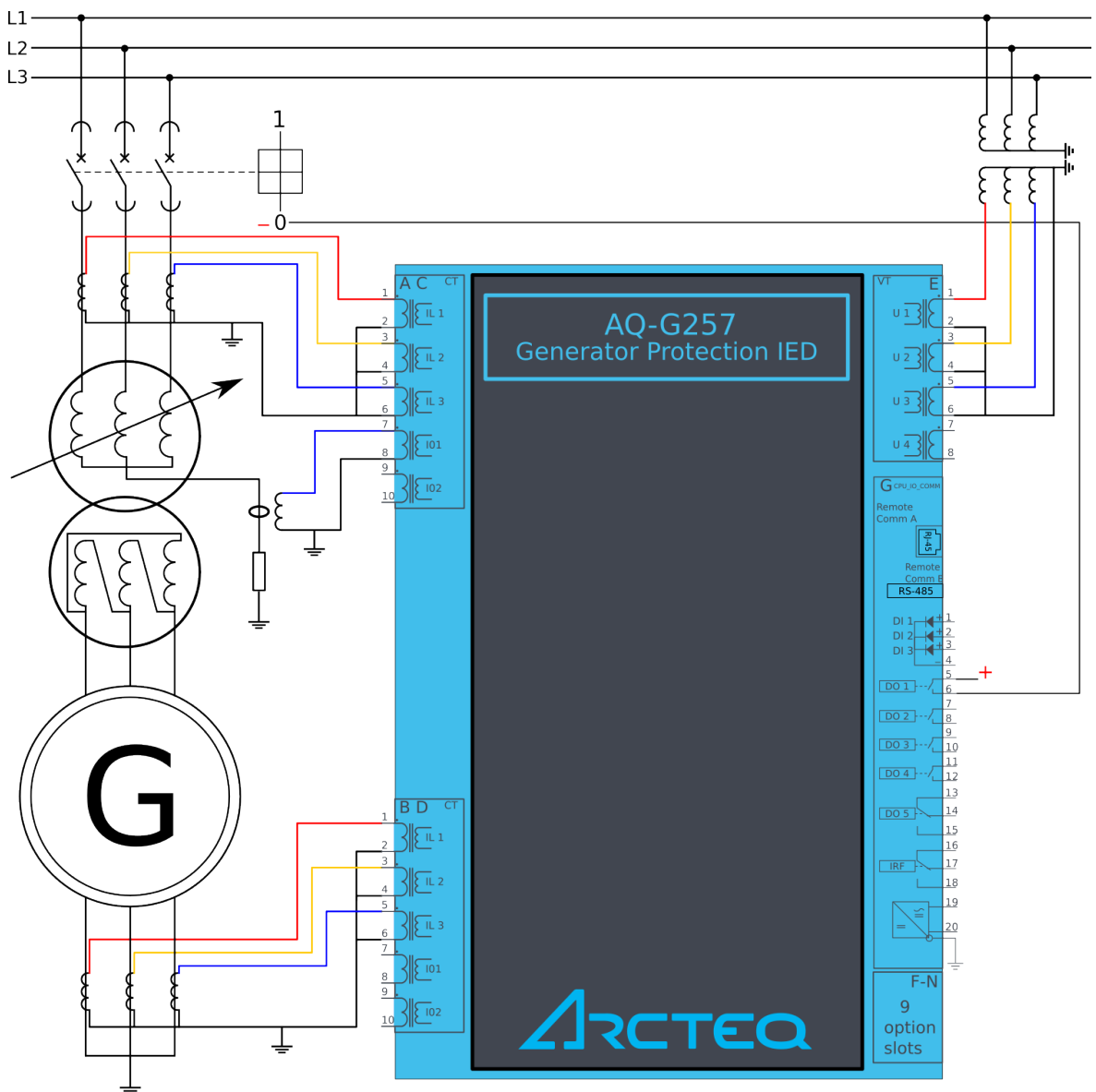
Figure. 7.2 - 214. Application example 1 and its connections.
