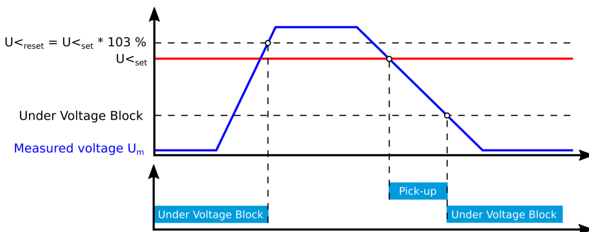
Figure. 5.4.10 - 64. Example of the block setting operation.
