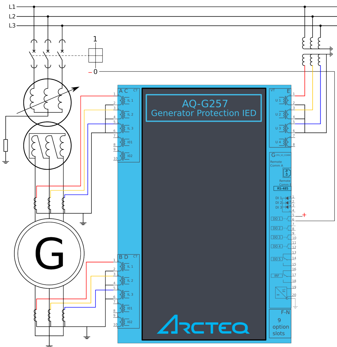
Figure. 7.2 - 215. Application example 2 and its connections.
