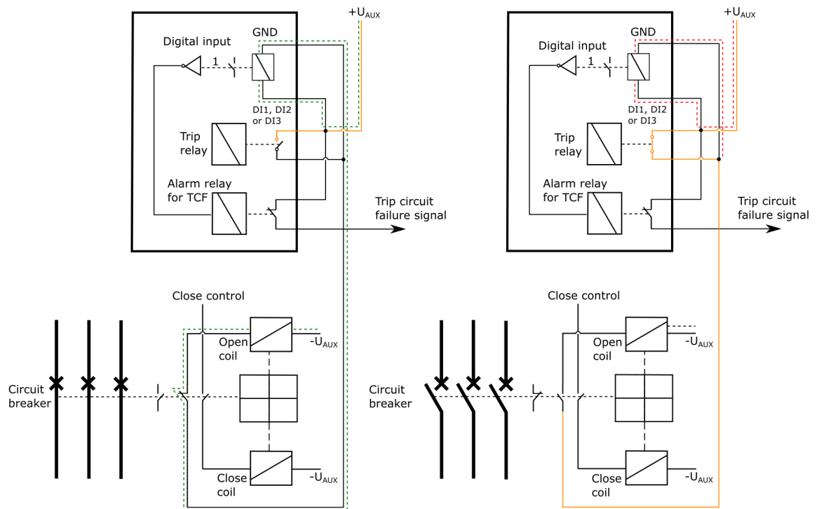
Figure. 7.3 - 219. Trip circuit supervision with one DI and one latched output contact.
