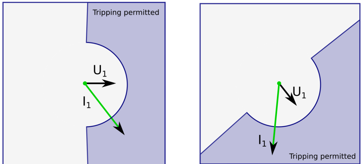
Figure. 5.4.4 - 33. Angle tracking of the I_{dir} function (3LN/3LL + U_0 mode).
