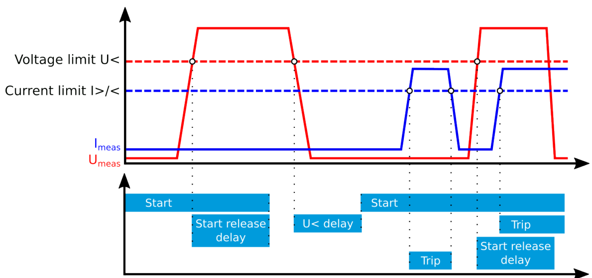
Figure. 5.4.25 - 124. Operating characteristics of inadvertent energizing protection.
