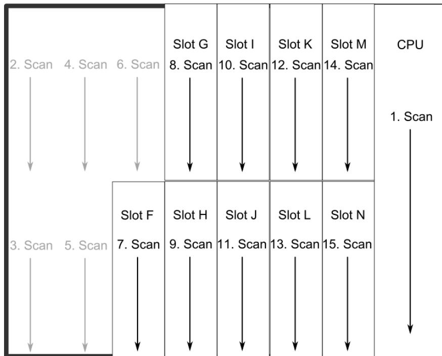
Figure. 8.1 - 223. AQ-X257 hardware scanning and I/O naming principles.
