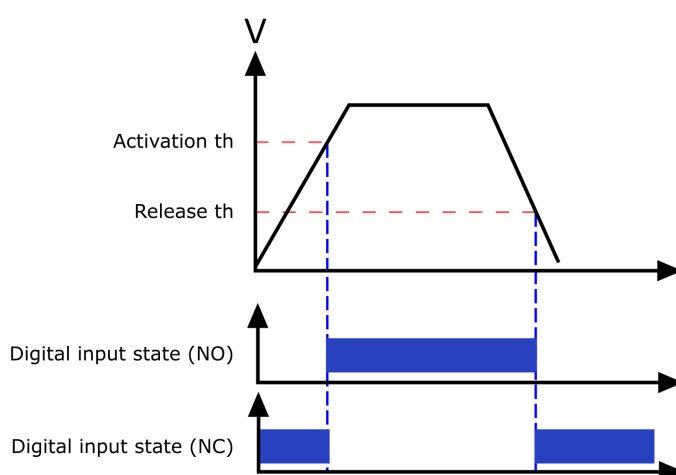
Figure. 8.5 - 228. Digital input state when energizing and de-energizing the digital input channels.
