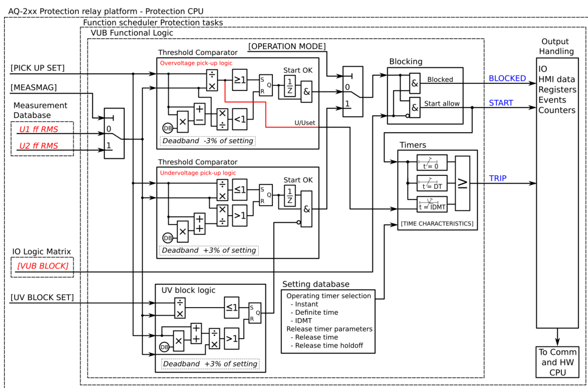
Figure. 5.4.12 - 75. Simplified function block diagram of the U1/U2>/< function.
