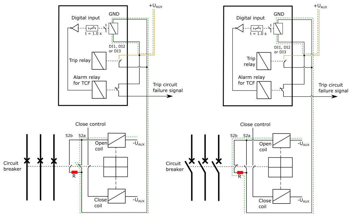
Figure. 7.3 - 216. Trip circuit supervision with one DI and one non-latched trip output.
