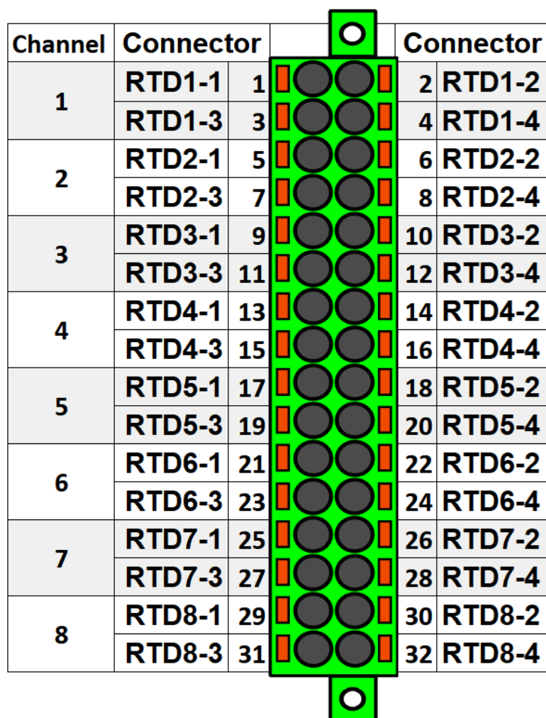
Figure. 8.8 - 231. RTD input module connectors.
