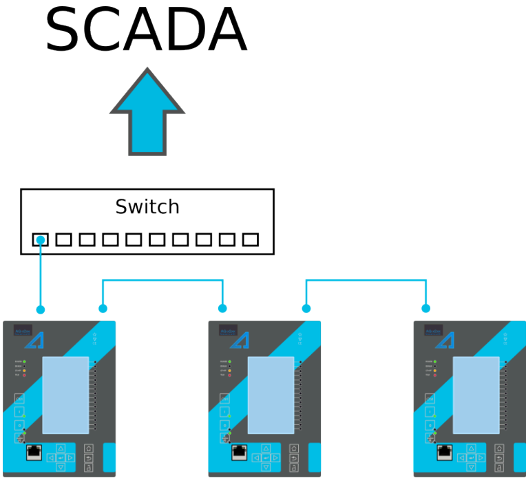
Figure. 8.11 - 237. Example of a multidrop configuration.
