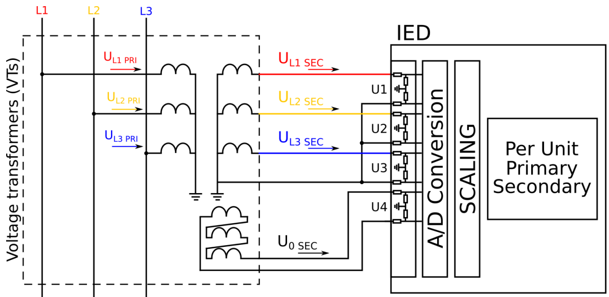
Figure. 5.2.2 - 9. Voltage measurement terminology
