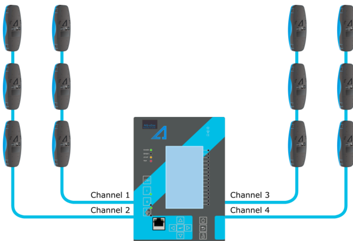
Figure. 5.4.29 - 155. IED equipped with arc protection.
