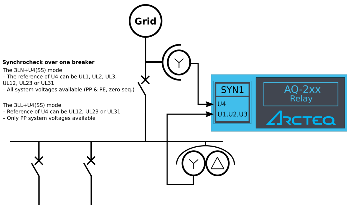
Figure. 5.5.5 - 172. Example application (synchrocheck over one breaker, with 3LL and 3LN VT connections).
