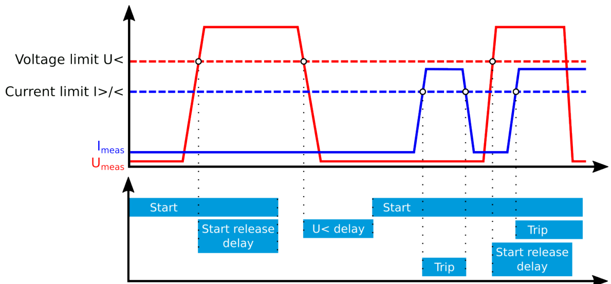
Figure. 5.4.24 - 123. Operating characteristics of inadvertent energizing protection.
