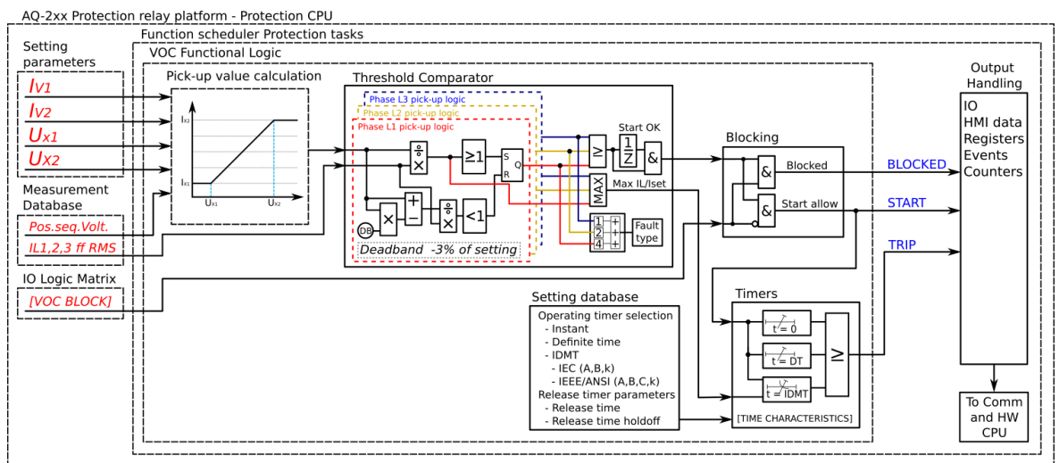
Figure. 5.4.21 - 116. Simplified function block diagram of the lv> function.
