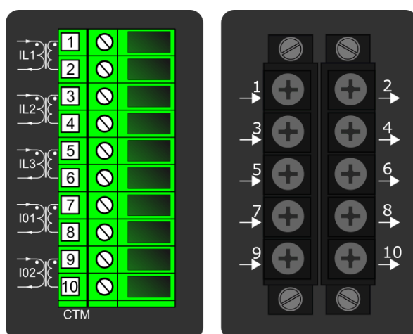
Figure. 8.3 - 225. Module connections with standard and ring lug terminals.
