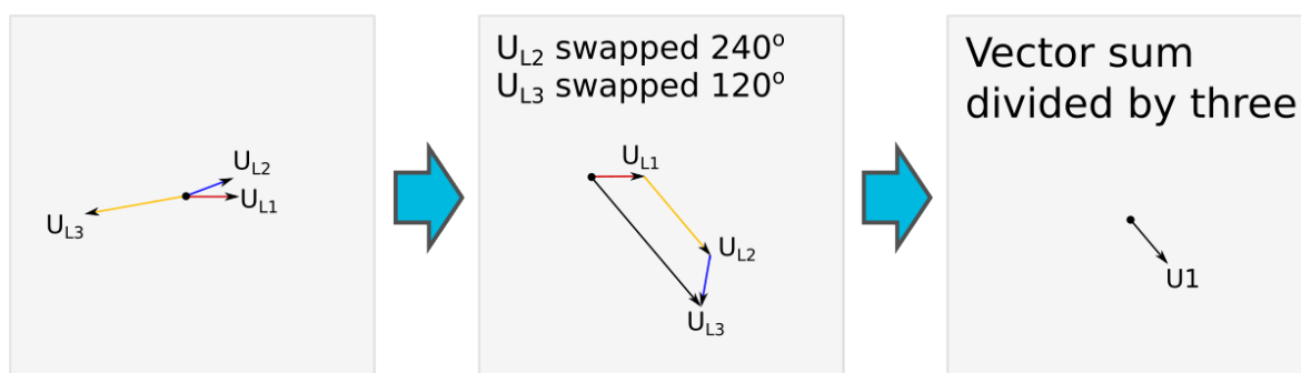
Figure. 5.4.12 - 71. Close-distance short-circuit between phases 1 and 3.
