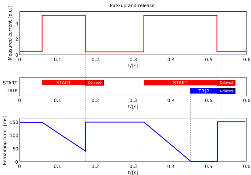
Figure. 5.4.1 - 27. Delayed pick-up release, delay counter value is held during the release time.
