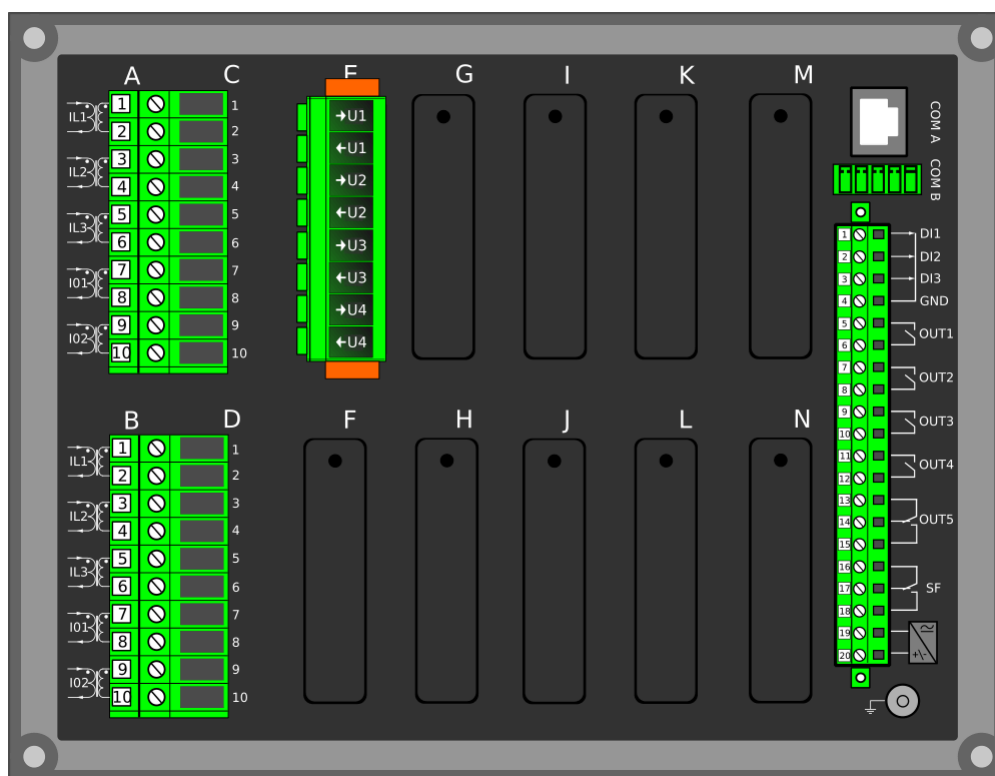
Figure. 8.1 - 221. Modular construction of AQ-X257-XXXXXXX-AAAAAAAAA
