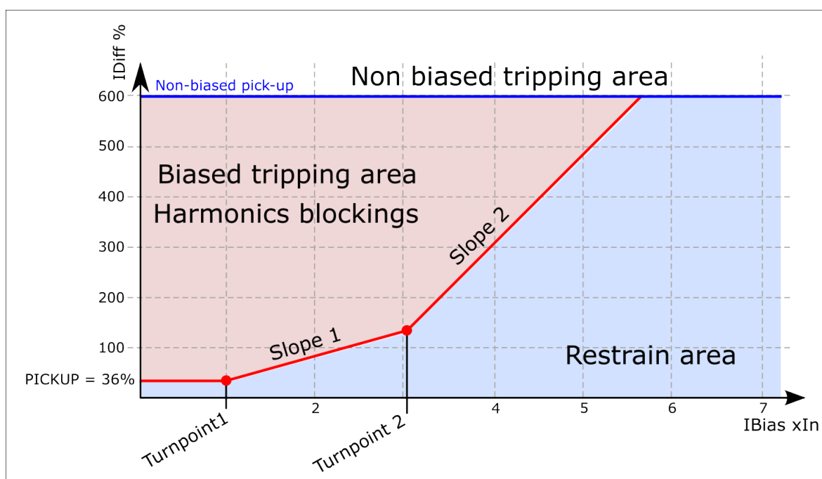
Figure. 5.4.27 - 139. Differential function characteristic, biased and non-biased.
