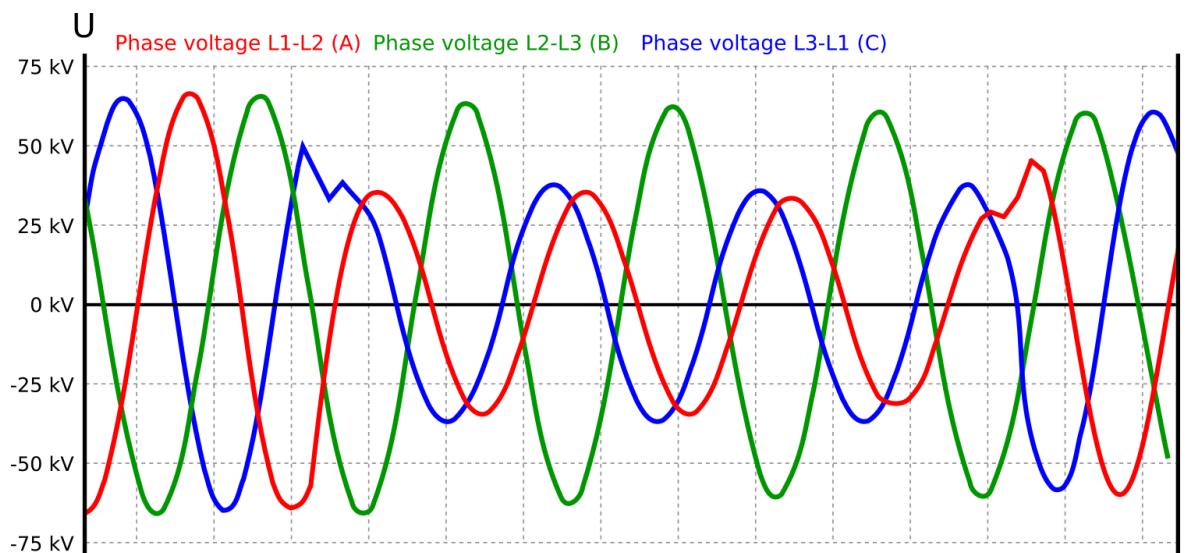
Figure. 5.5.8 - 182. Generator islanding.
