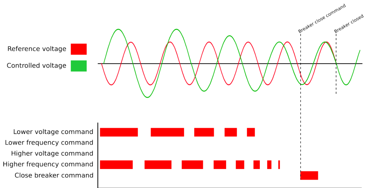
Figure. 5.5.7 - 180. Simplified presentation of synchronizer operation
