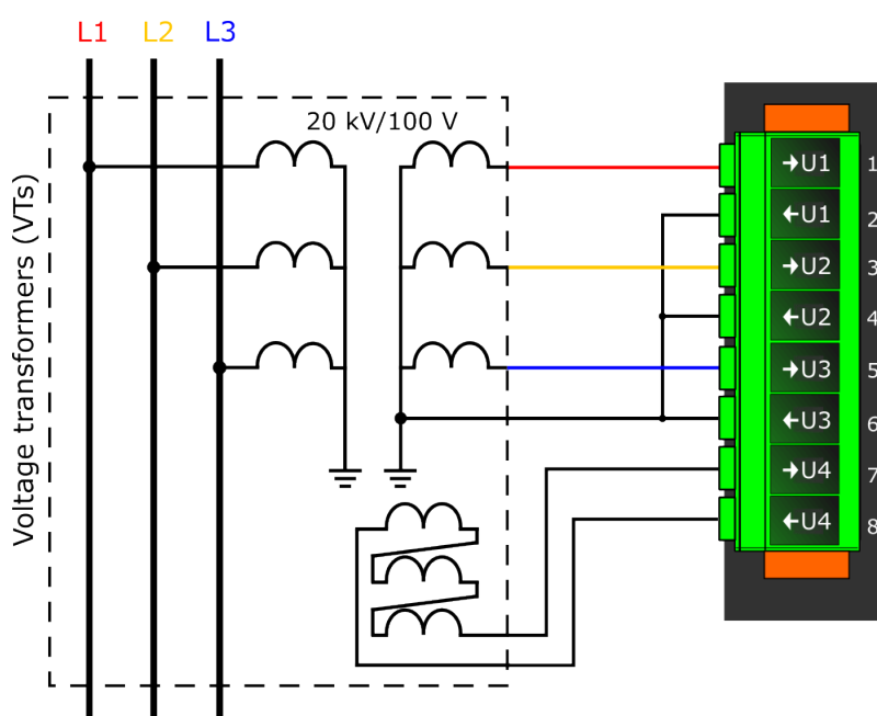
Figure. 5.2.2 - 10. Connections.
