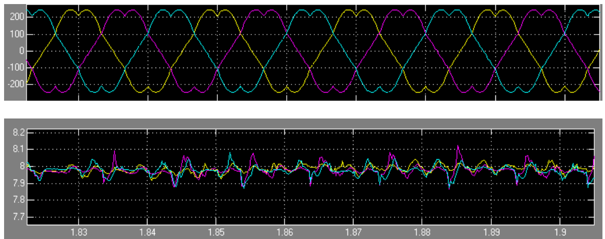
Figure. 5.4.27 - 151. Example waveforms.
