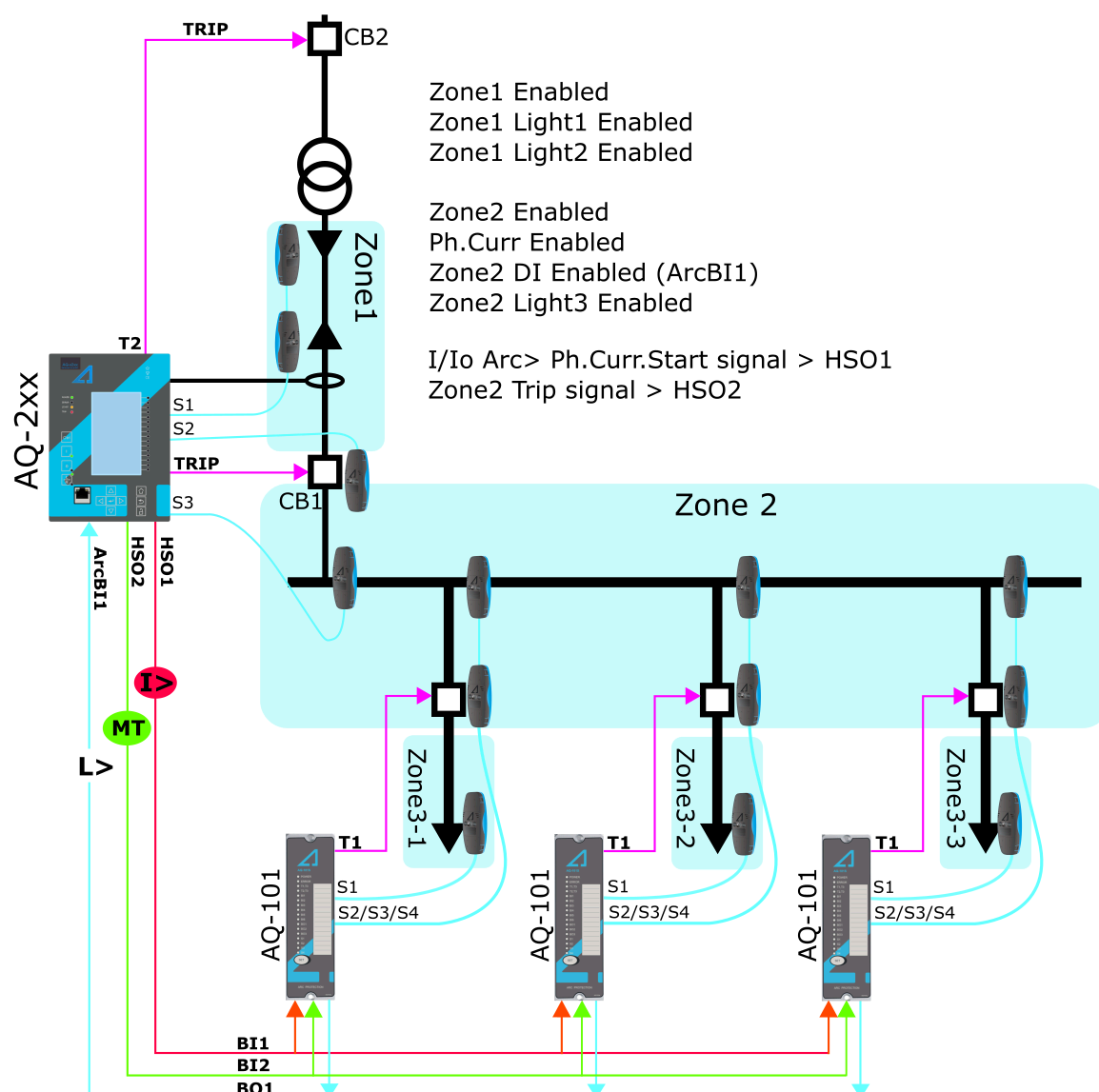
Figure. 5.4.29 - 156. Scheme 1A1 (with AQ-101 arc protection relays).
