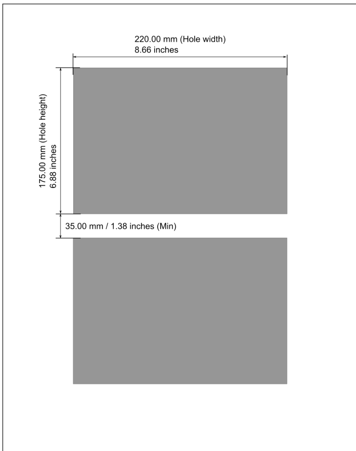
Figure. 8.14 - 243. Panel cut-out and spacing of the IED.
