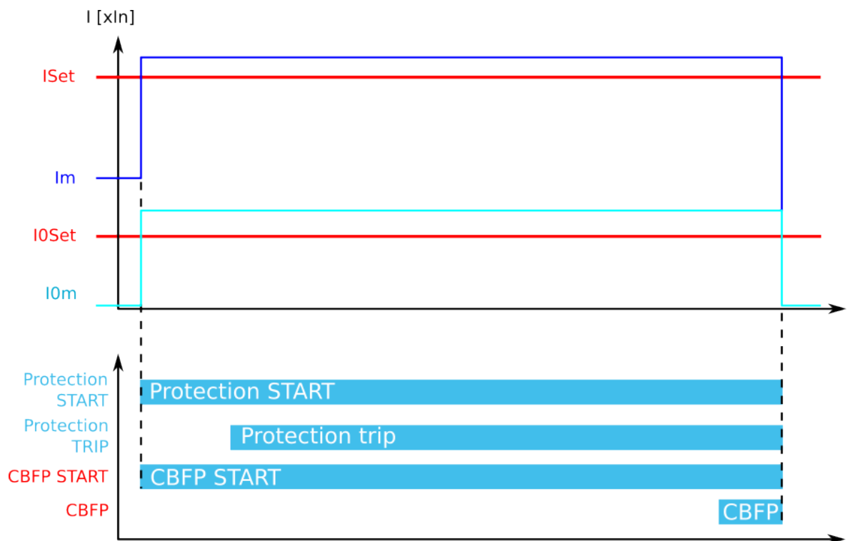
Figure. 5.4.8 - 103. CBFP when "Current" is the selected criterion.
