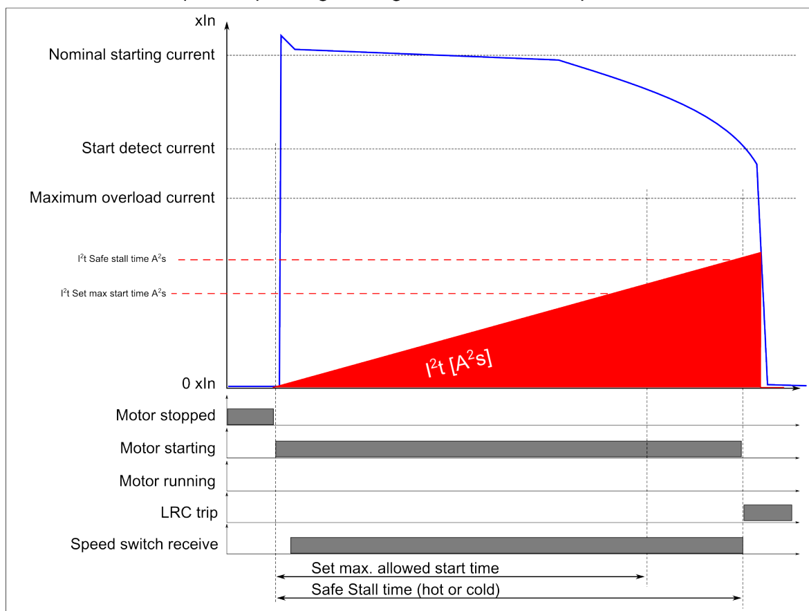
Figure. 5.4.20 - 158. Outputs when motor starting takes too long, with a speed switch.
