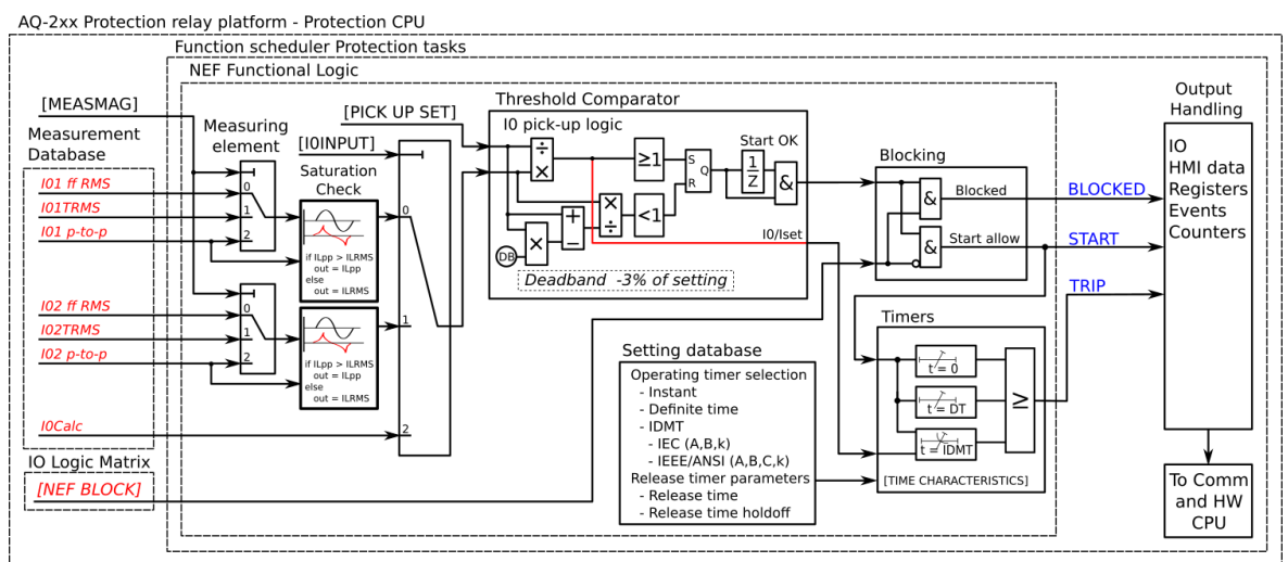
Figure. 5.4.3 - 83. Simplified function block diagram of the I0> function.
