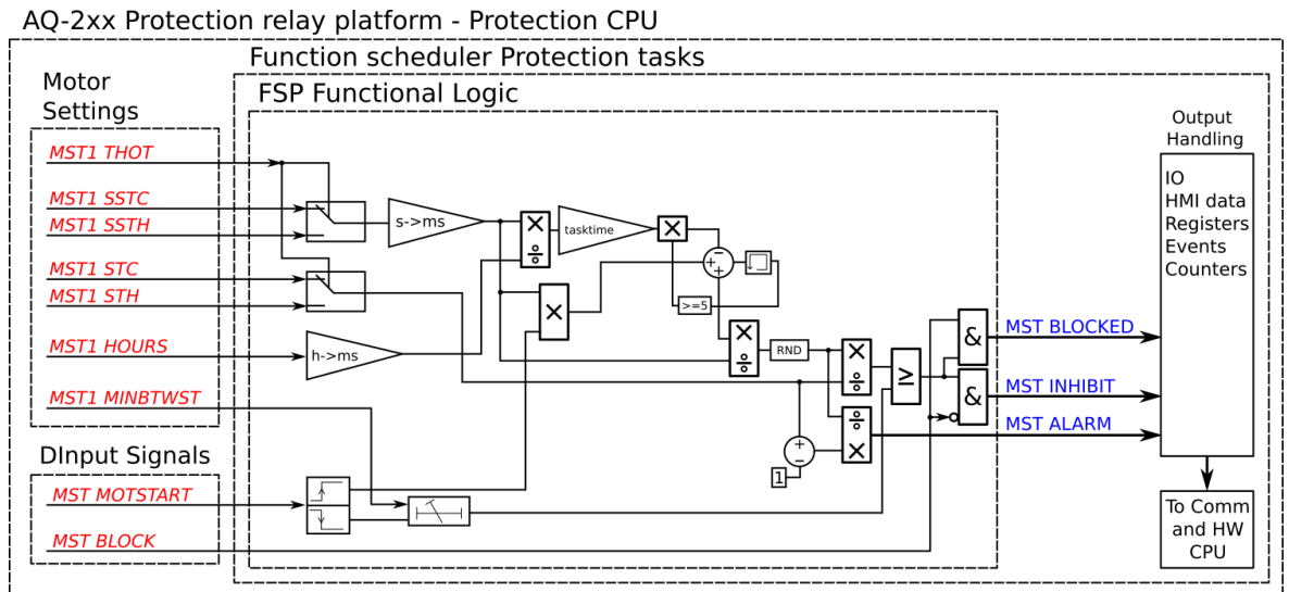
Figure. 5.4.21 - 160. Simplified function block diagram of the N> function.
