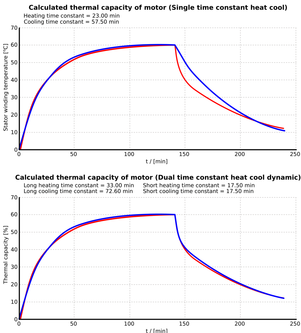
Figure. 5.4.25 - 176. Matching thermal replicas to the measured thermal capacity of the motor.
