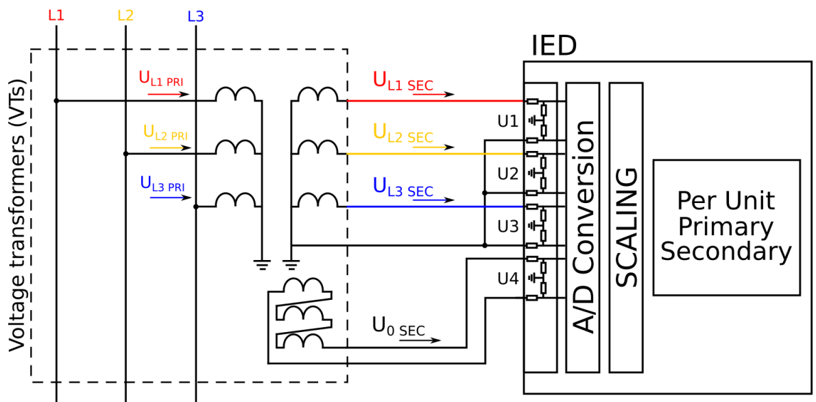
Figure. 5.2.2 - 62. Voltage measurement terminology
