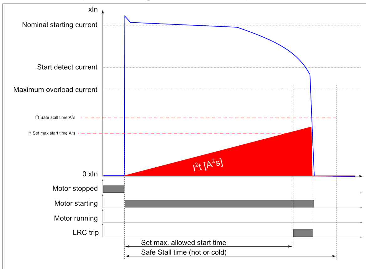
Figure. 5.4.20 - 156. Outputs when motor starting takes too long, no speed switch.
