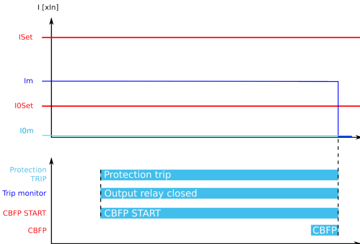
Figure. 5.4.8 - 105. CBFP when "Current or DO" is the selected criterion.
