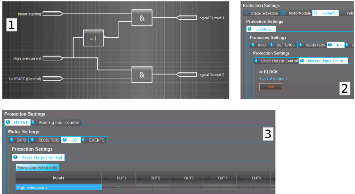
Figure. 5.4.19 - 153. Motor start up overcurrent control logic.
