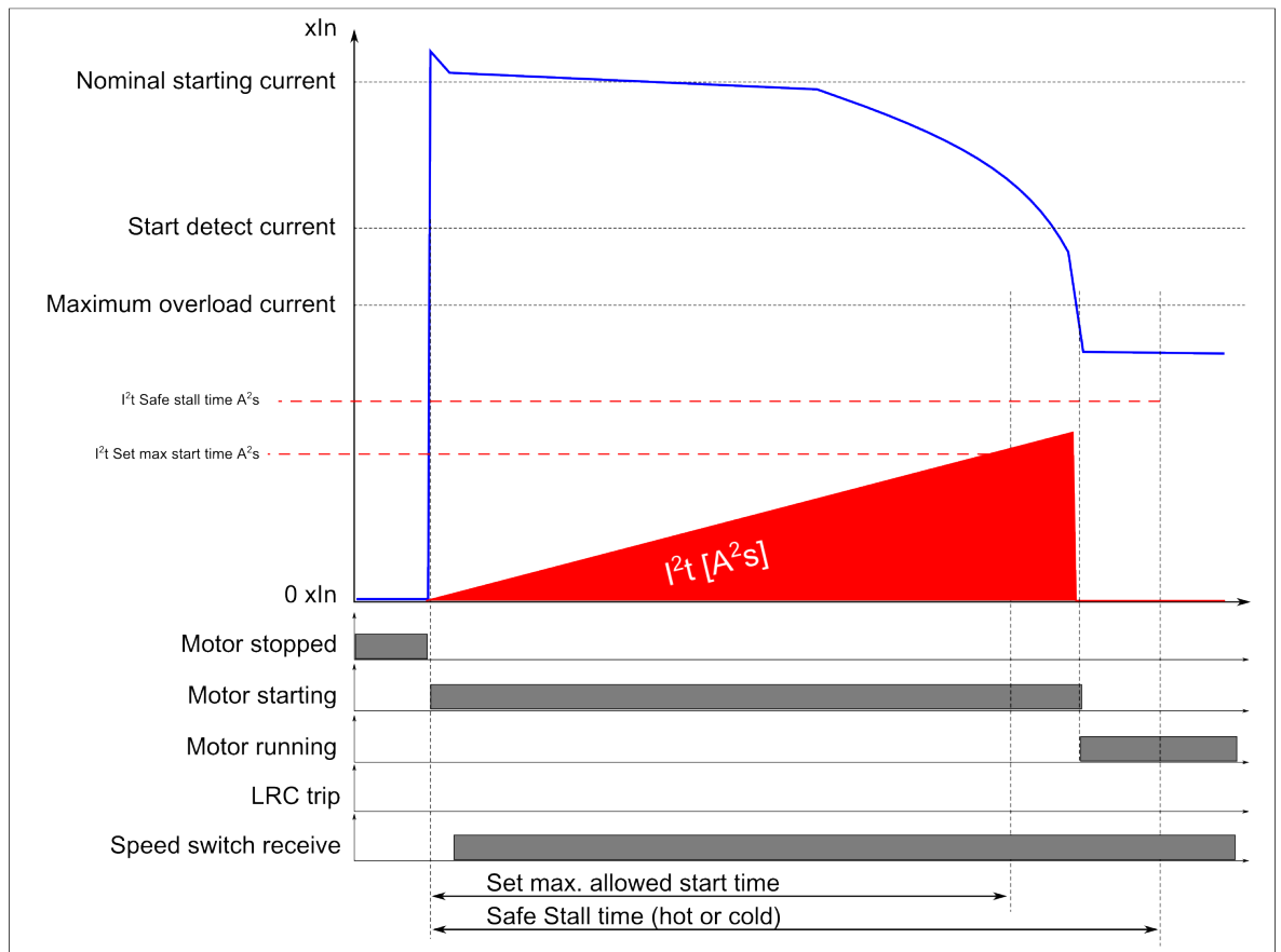
Figure. 5.4.20 - 157. Outputs in long motor starting, with a speed switch.
