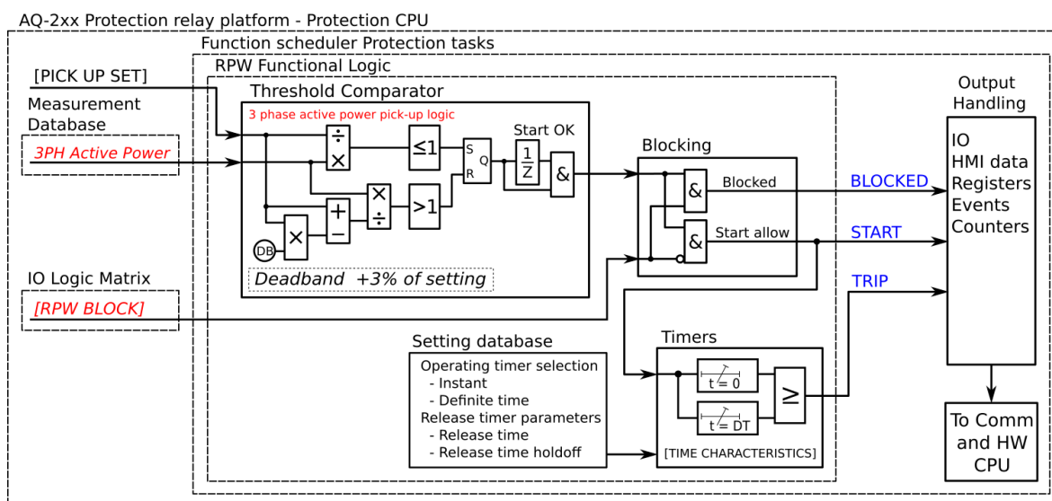
Figure. 5.4.18 - 148. Simplified function block diagram of the Pr function.
