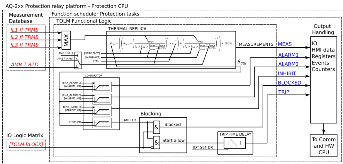
Figure. 5.4.25 - 191. Simplified function block diagram of the TM> function.
