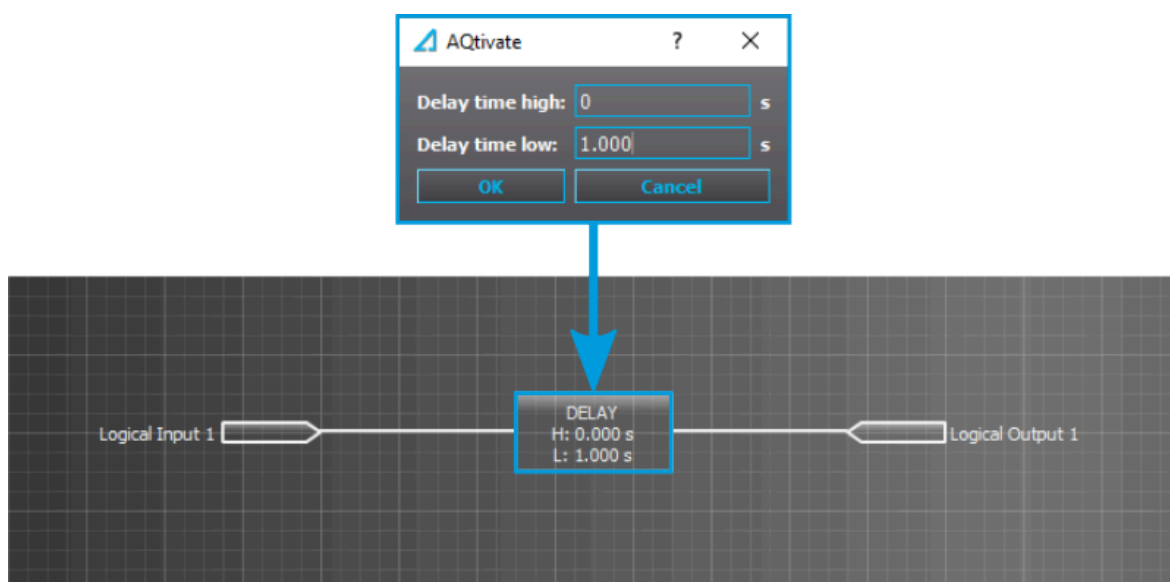
Figure. 5.5.9 - 210. Extending a logical input pulse.
