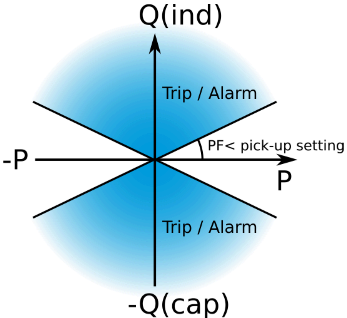
Figure. 5.4.24 - 165. Operating characteristics of power factor protection.
