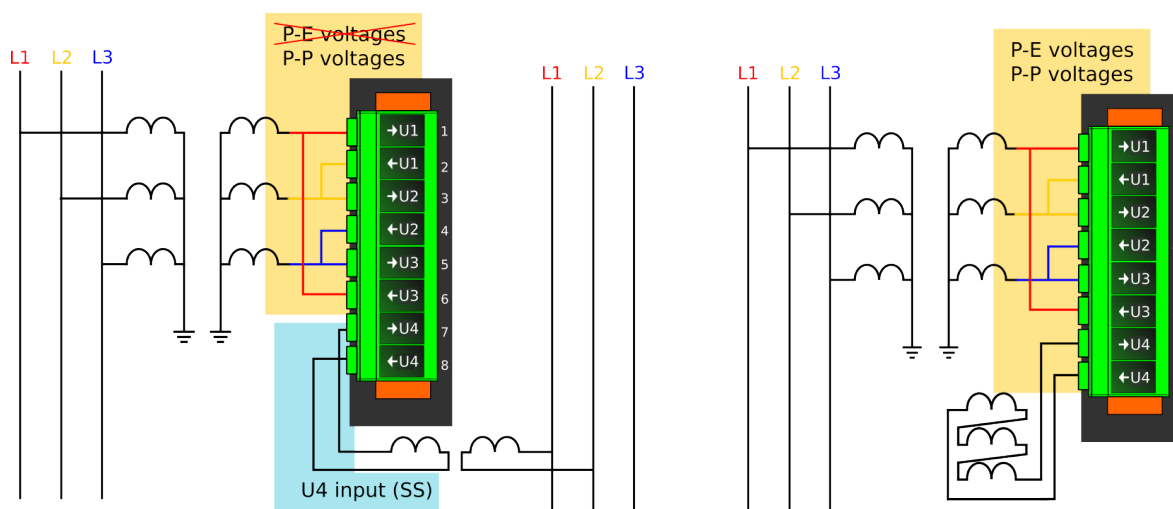
Figure. 5.4.11 - 123. Selectable measurement magnitudes with 3LL+U4 VT connection (P-E voltages not available without residual voltage).
