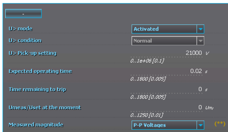
Figure. 5.2.2 - 64. Selecting the measured magnitude.
