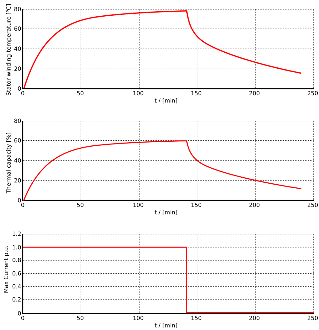
Figure. 5.4.25 - 175. Measured motor temperature in heating/cooling test.
