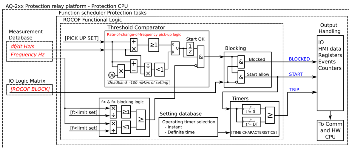
Figure. 5.4.15 - 141. Simplified function block diagram of the df/dt > / < function.
