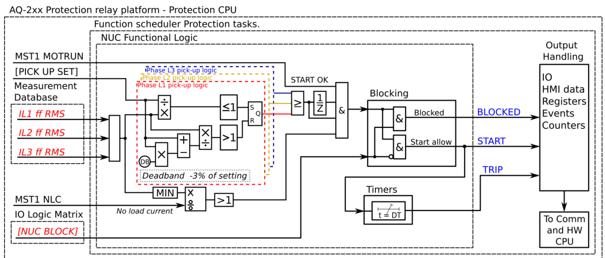
Figure. 5.4.22 - 163. Simplified function block diagram of the I< function.
