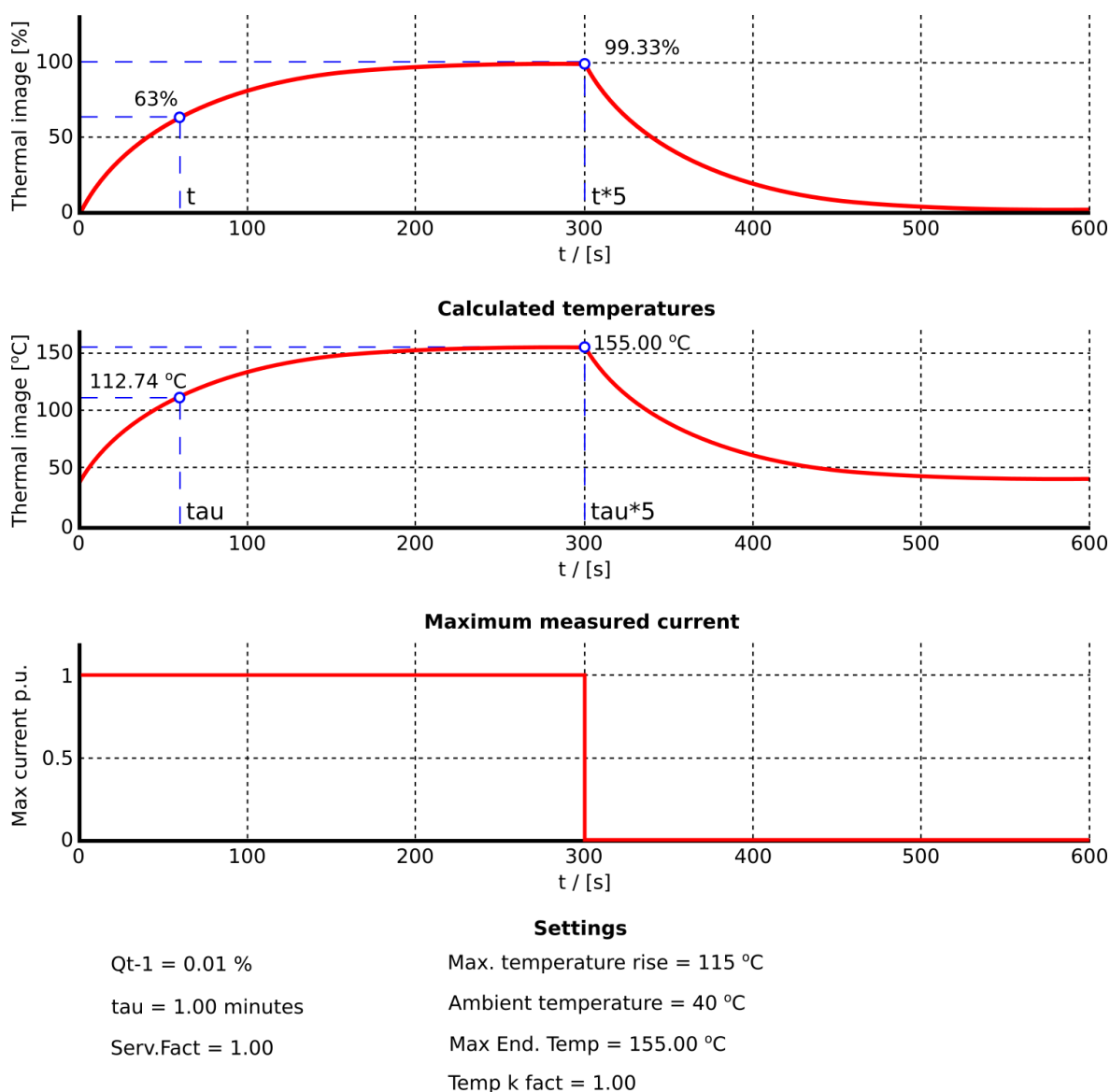
Figure. 5.4.25 - 169. Thermal image calculation with nominal conditions: single time constant thermal replica.
