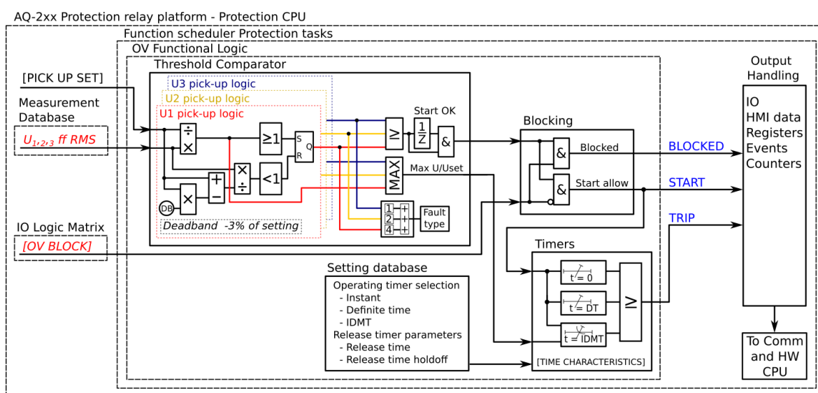
Figure. 5.4.10 - 117. Simplified function block diagram of the U> function.
