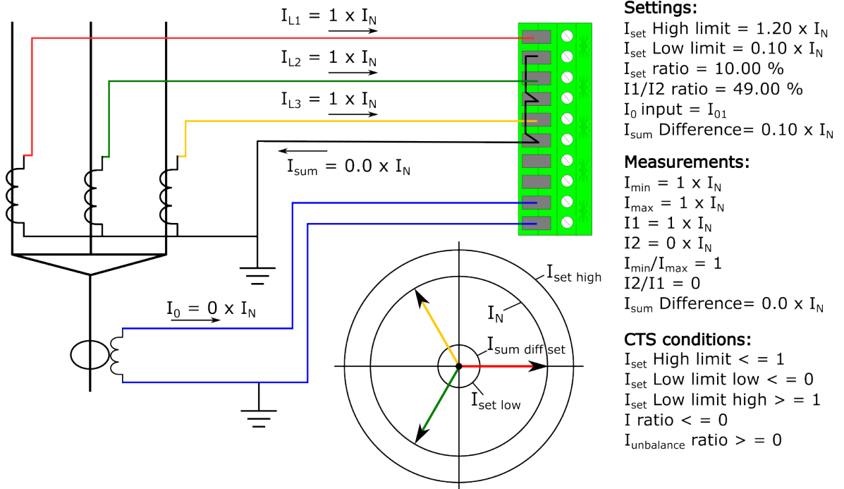
Figure. 5.6.1 - 218. Normal situation, residual current also measured.
