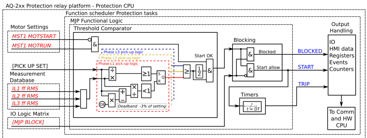
Figure. 5.4.23 - 164. Simplified function block diagram of the I_m > function.
