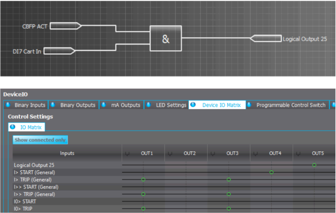
Figure. 5.5.8 - 208. Logic output example. Logical output is connected to an output relay in matrix.
