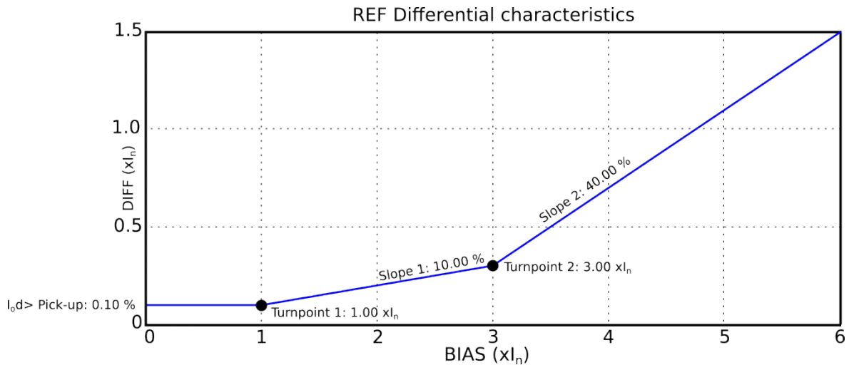
Figure. 5.4.9 - 109. Differential characteristics for the I 0d > function with default settings.
