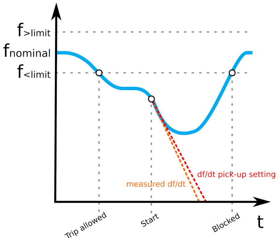
Figure. 5.4.15 - 140. Operation of the df/dt >/< function when the frequency starts but doesn't trip.
