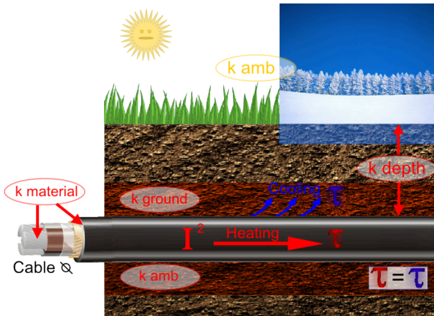
Figure. 5.4.25 - 172. Factors affecting the cooling and current-carrying capacity of a cable.
