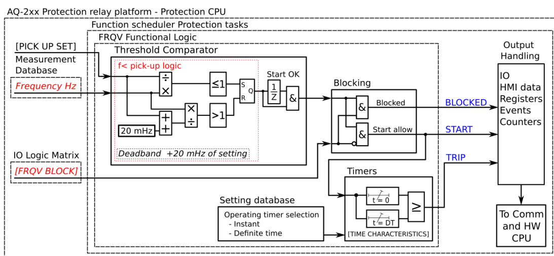
Figure. 5.4.14 - 139. Simplified function block diagram of the f< function.
