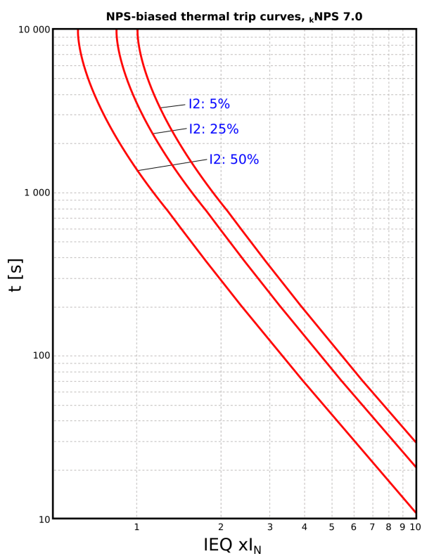
Figure. 5.4.25 - 189. NPS-biased thermal trip curves with k_{NPS} value of 7.
