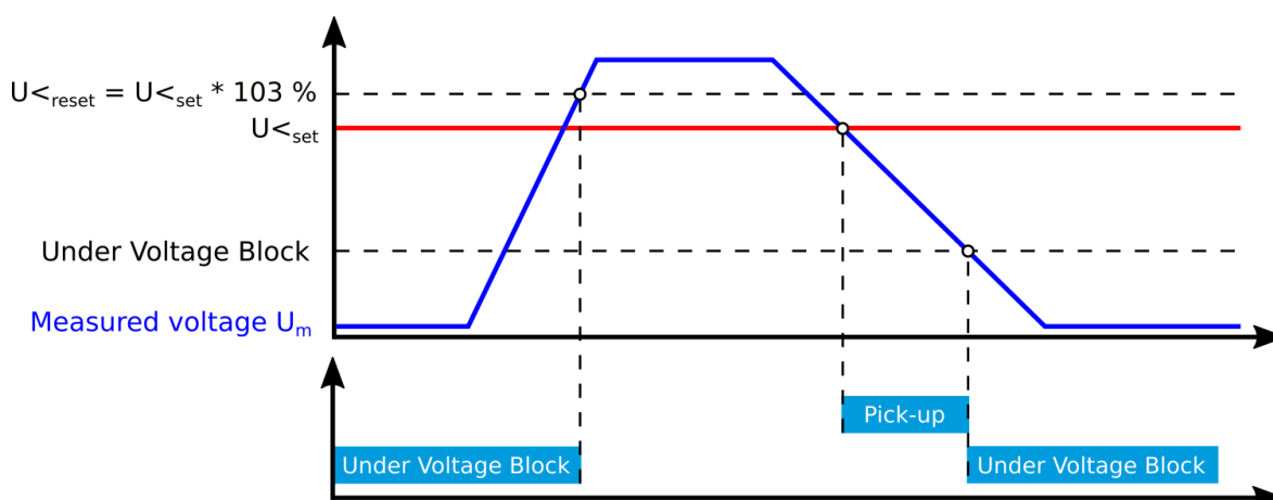
Figure. 5.4.11 - 125. Example of the block setting operation.
