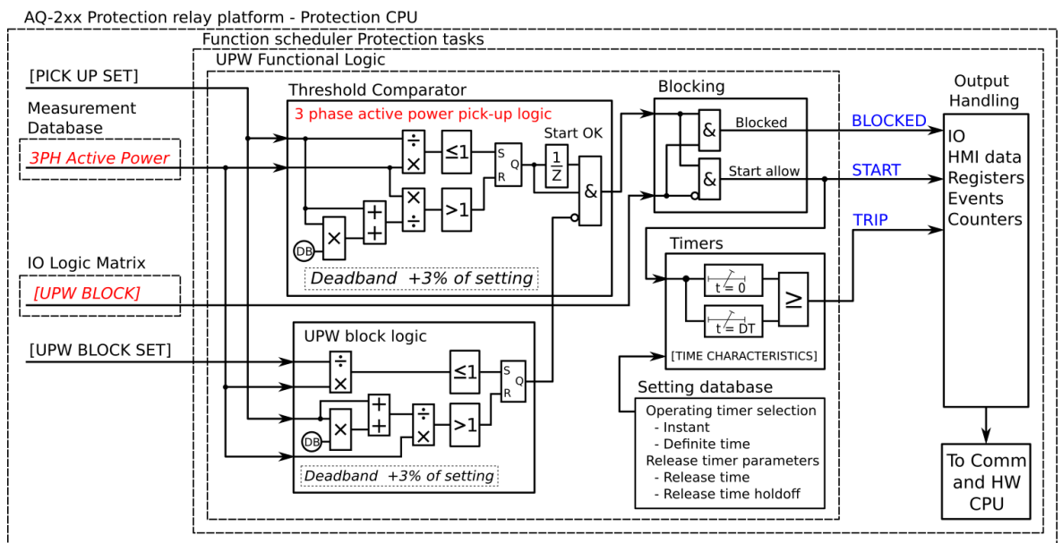
Figure. 5.4.17 - 145. Simplified function block diagram of the P< function.
