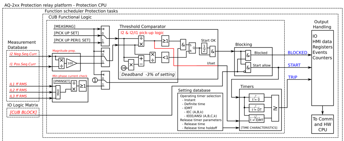
Figure. 5.4.6 - 94. Simplified function block diagram of the I2> function.
