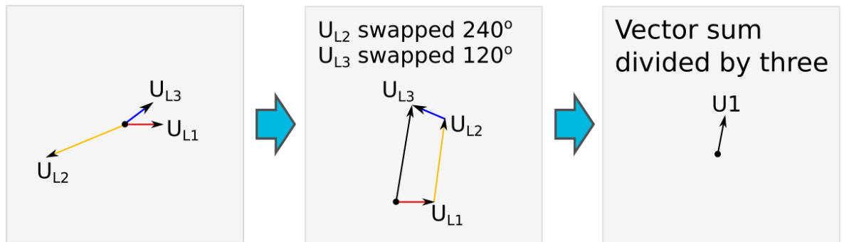
Figure. 5.4.13 - 135. Close-distance short-circuit between phases 1 and 3.
