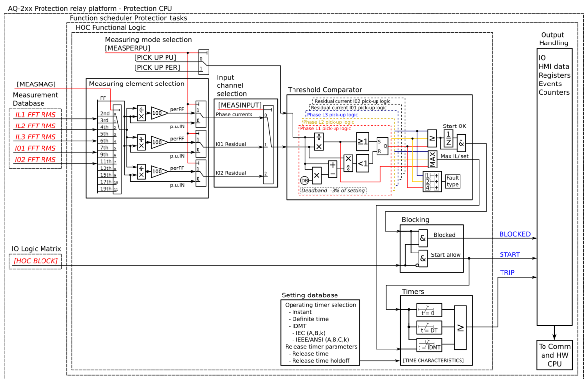
Figure. 5.4.7 - 96. Simplified function block diagram of the Ih> function.
