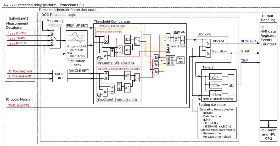
Figure. 5.4.4 - 84. Simplified function block diagram of the Idir> function.
