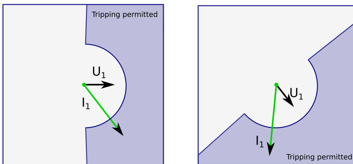
Figure. 5.4.4 - 85. Angle tracking of the I_{dir} function (3LN/3LL + U_0 mode).
