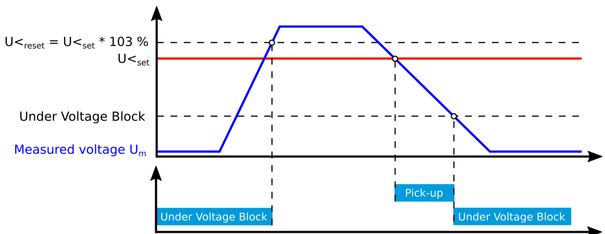
Figure. 5.4.13 - 137. Example of the block setting operation.
