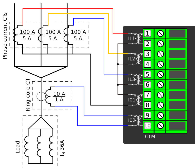
Figure. 5.2.1 - 52. Connections.
