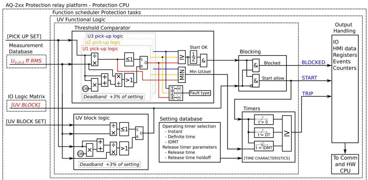
Figure. 5.4.11 - 121. Simplified function block diagram of the U< function.
