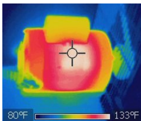
Figure. 5.4.25 - 174. Running motor's temperature with thermal image camera.
