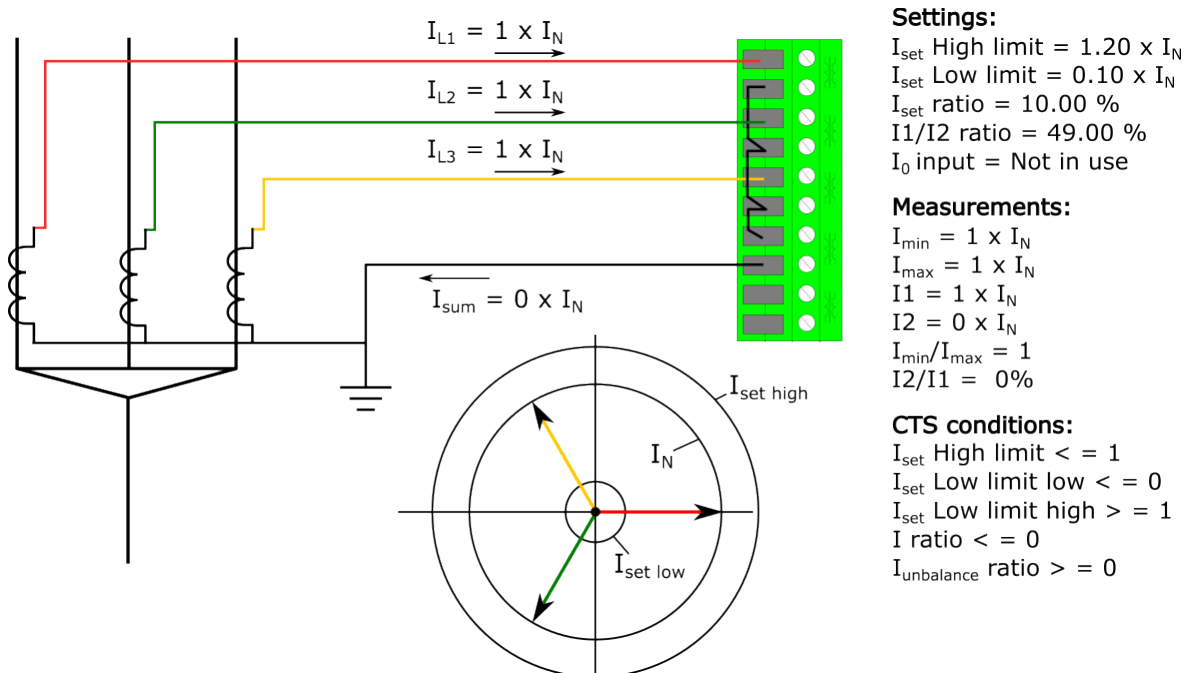
Figure. 5.6.1 - 213. All works properly, no faults.
