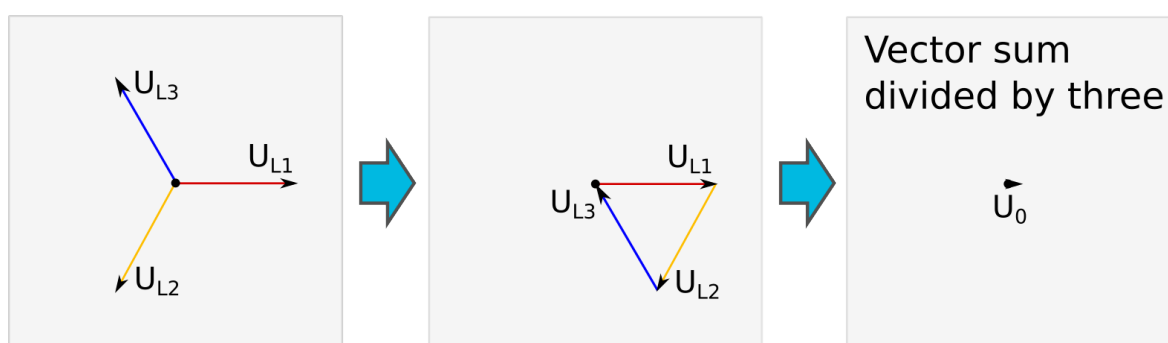
Figure. 5.4.12 - 126. Normal situation.
