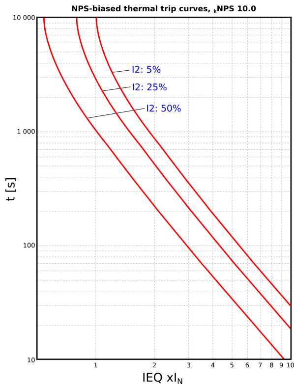
Figure. 5.4.25 - 190. NPS-biased thermal trip curves with k_{NPS} value of 10.
