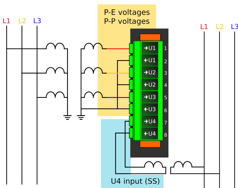
Figure. 5.4.11 - 123. Selectable measurement magnitudes with 3LL+U4 VT connection (P-E voltages not available without residual voltage).
