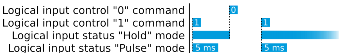
Figure. 5.5.9 - 209. Operation of logical input in "Hold" and "Pulse" modes.
