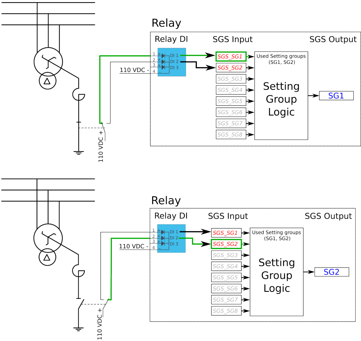
Figure. 5.5.2 - 202. Setting group control – two-wire connection from Petersen coil status.
