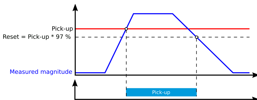
Figure. 5.4.1 - 74. Pick up and reset.
