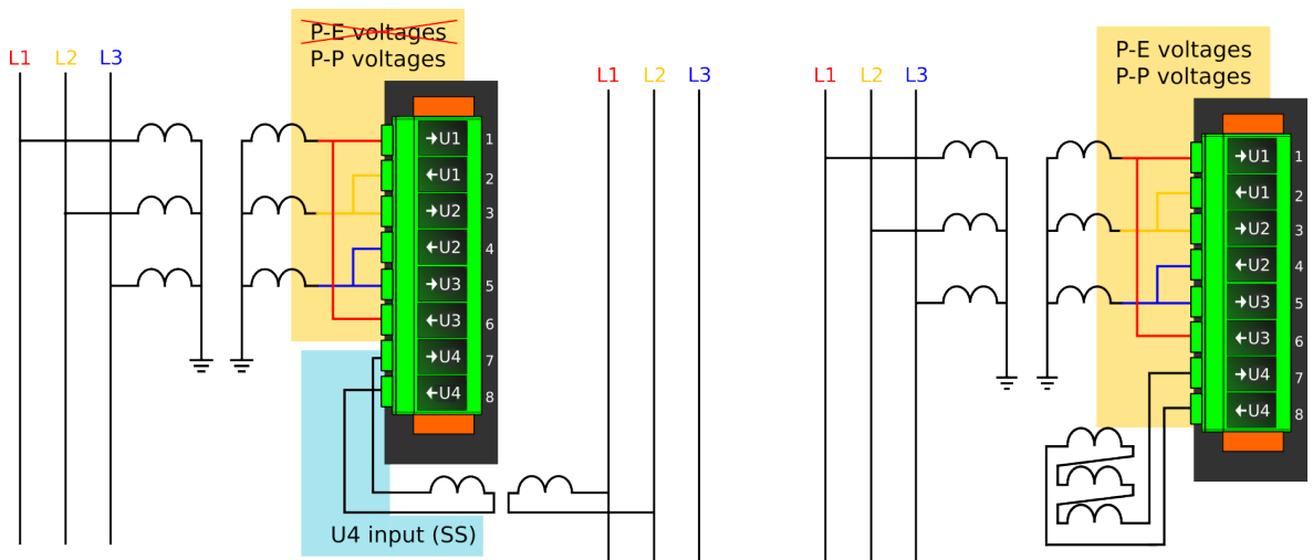
Figure. 5.4.10 - 119. Selectable measurement magnitudes with 3LL+U4 VT connection (P-E voltages not available without residual voltage).
