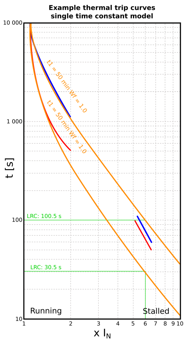
Figure. 5.4.25 - 178. Comparing single time constant thermal replica tripping curves to given motor thermal characteristics.
