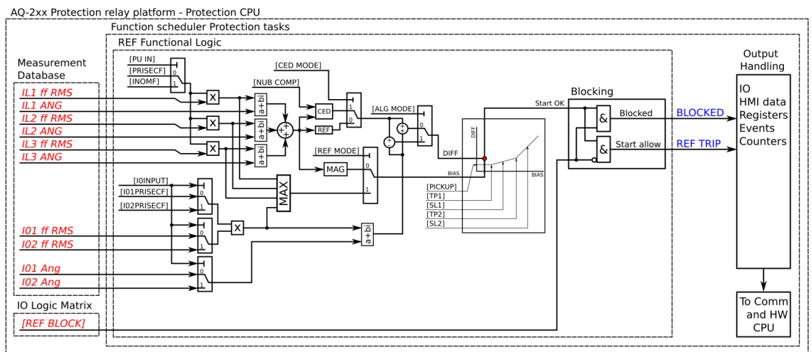
Figure. 5.4.9 - 108. Simplified function block diagram of the I0d> function.
