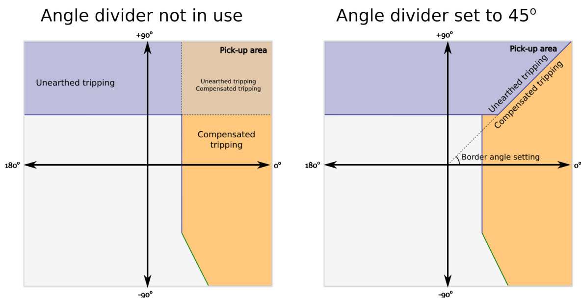
Figure. 5.4.5 - 93. Effect of angle divider when in use and when disabled.
