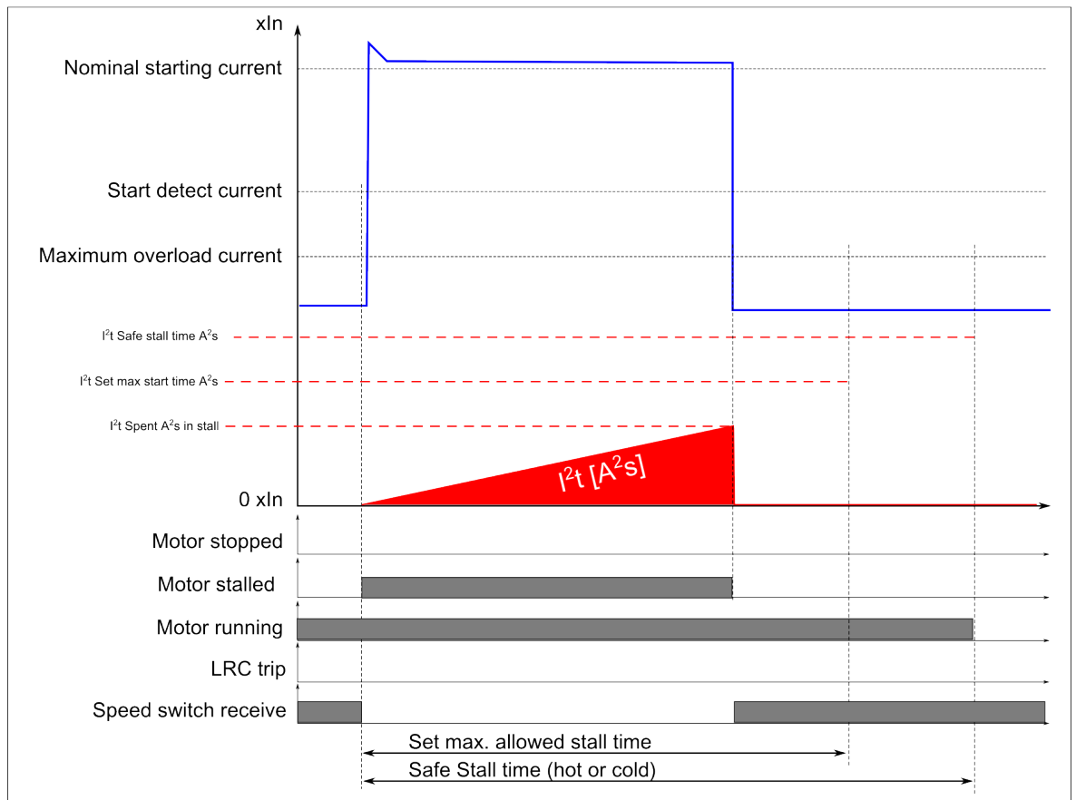
Figure. 5.4.20 - 159. Motor stall monitoring.
