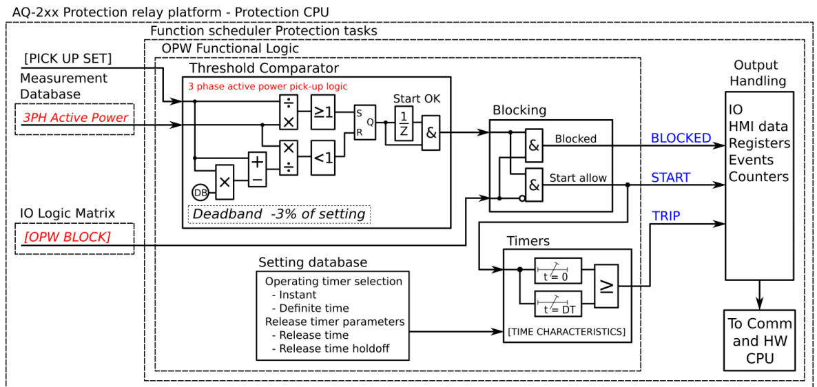
Figure. 5.4.16 - 143. Simplified function block diagram of the P> function.
