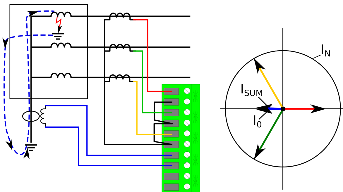
Figure. 5.4.9 - 116. Restricted earth fault inside a Y winding transformer.
