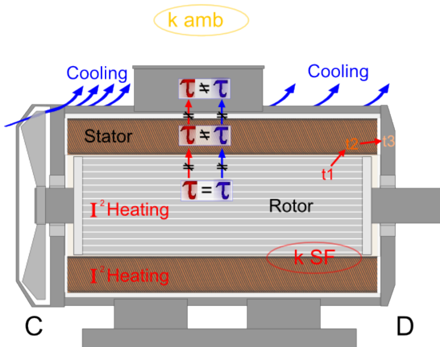
Figure. 5.4.25 - 173. Simplified motor construction and time constants.
