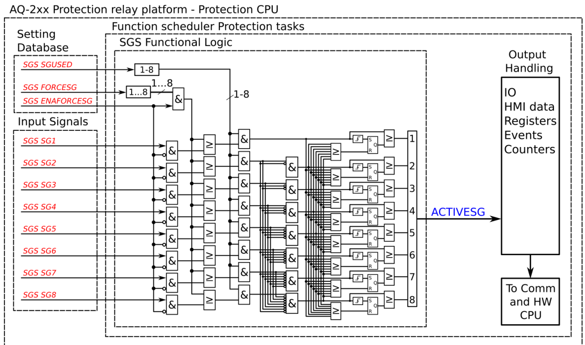
Figure. 5.5.2 - 199. Simplified function block diagram of the setting group selection function.
