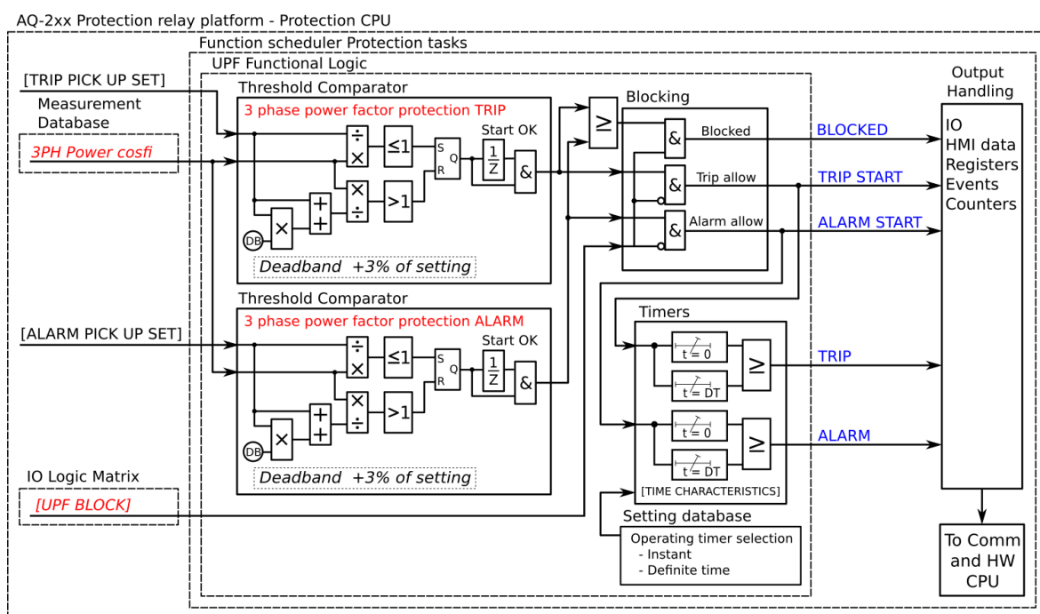
Figure. 5.4.24 - 166. Simplified function block diagram of the PF> function.
