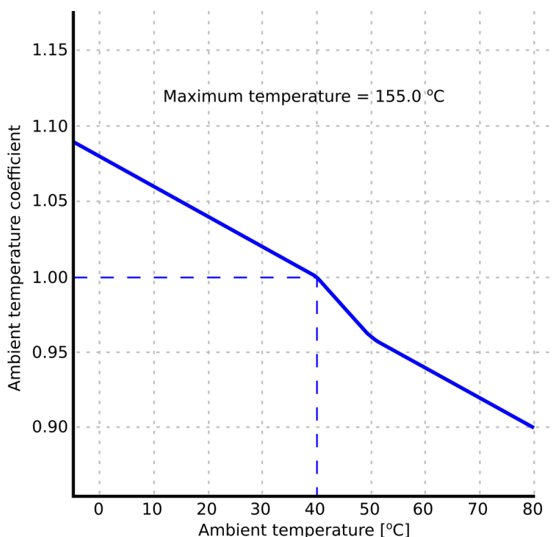
Figure. 5.4.25 - 171. Ambient temperature coefficient calculation (linear approximation, indefinite points).
