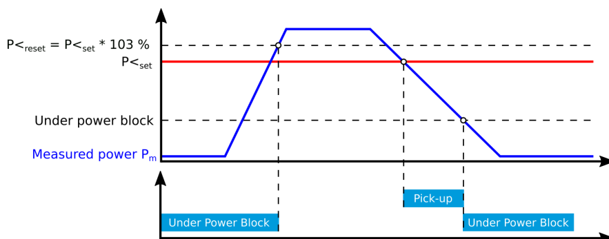
Figure. 5.4.17 - 146. Activation and deactivation characteristics of low power blocking.
