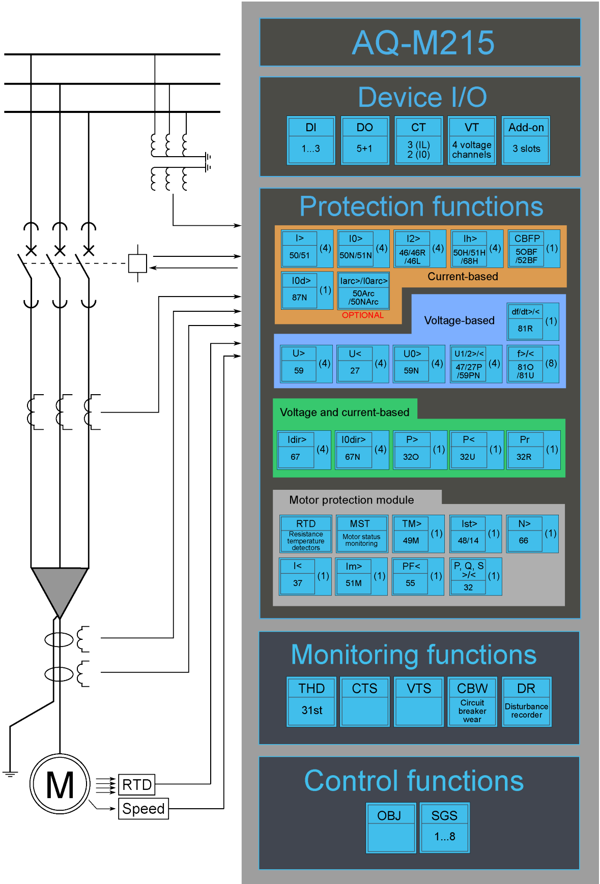
Figure. 7.1 - 234. AQ-M215 application example with function block diagram.
