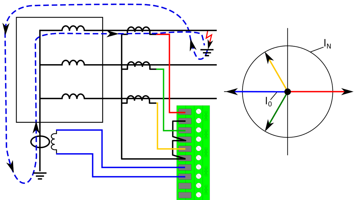
Figure. 5.4.9 - 115. Restricted earth fault outside a Y winding transformer.
