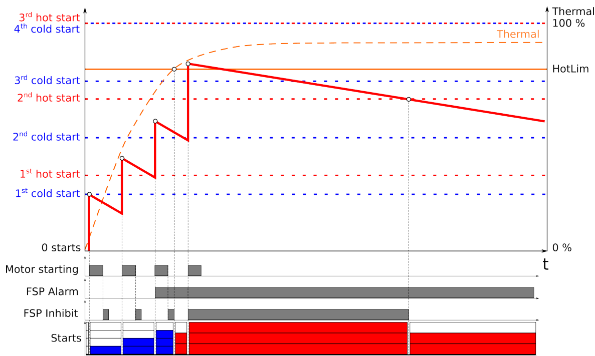
Figure. 5.4.21 - 162. Updating the starts counter when thermal hot and cold status taken into consideration.
