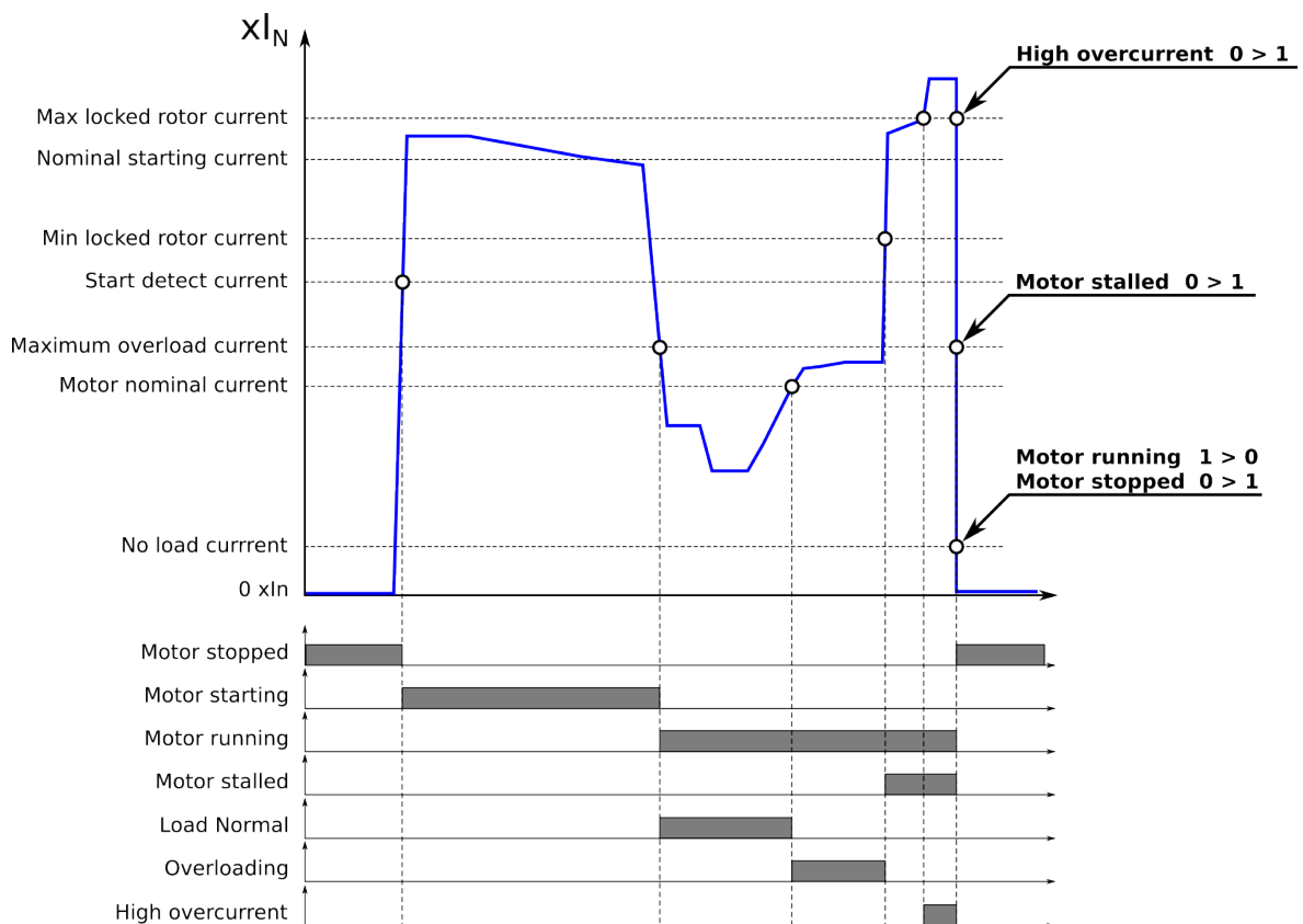
Figure. 5.4.19 - 150. Activation of the function's outputs.
