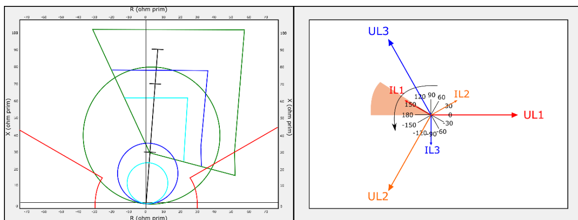
Figure. 5.4.28 - 196. Distance protection characteristics and directional overcurrent.
