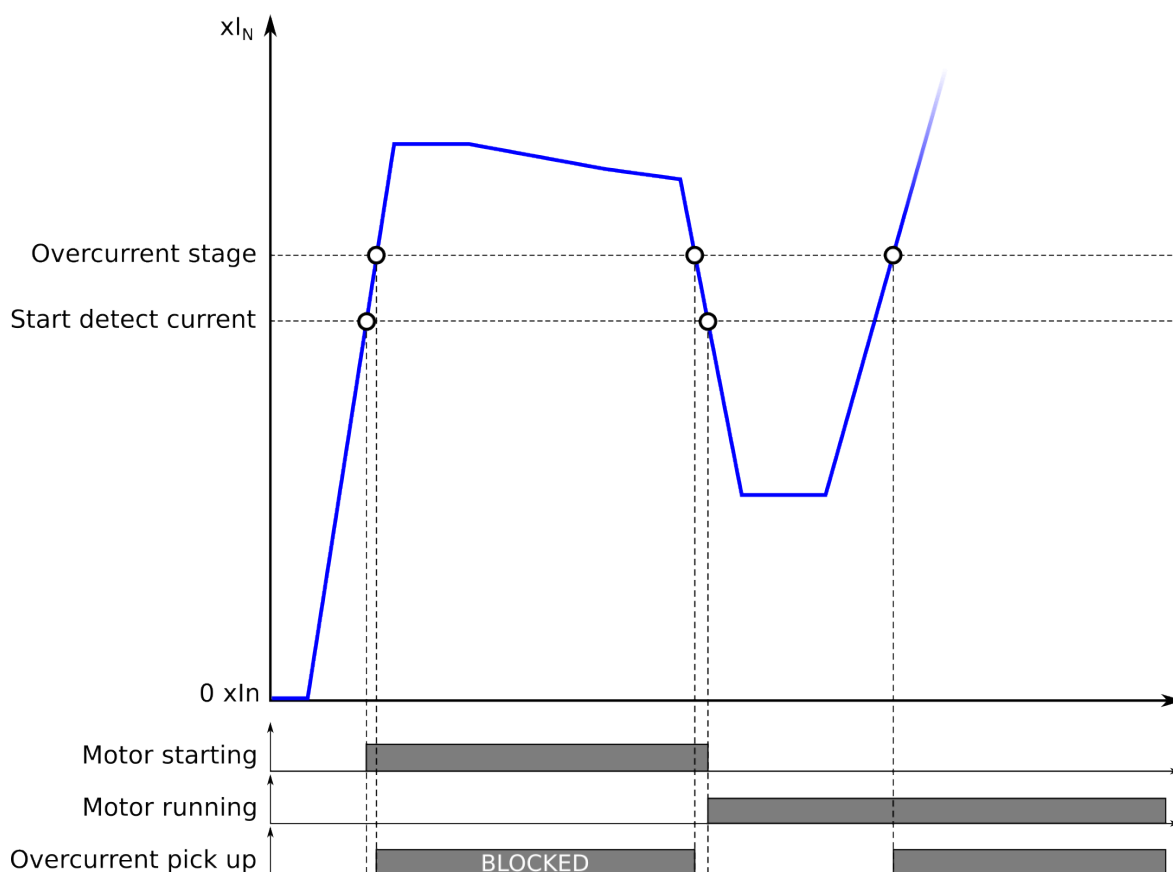
Figure. 5.4.19 - 151. Example of application: motor starting scheme and using motor status signals.
