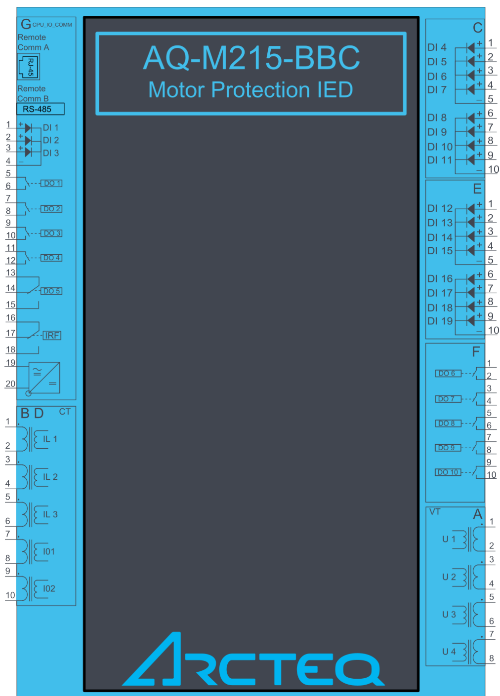
Figure. 7.1 - 233. AQ-M215 variant with digital input and output modules.
