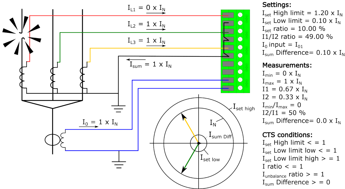
Figure. 5.6.1 - 220. Broken primary phase current wiring.
