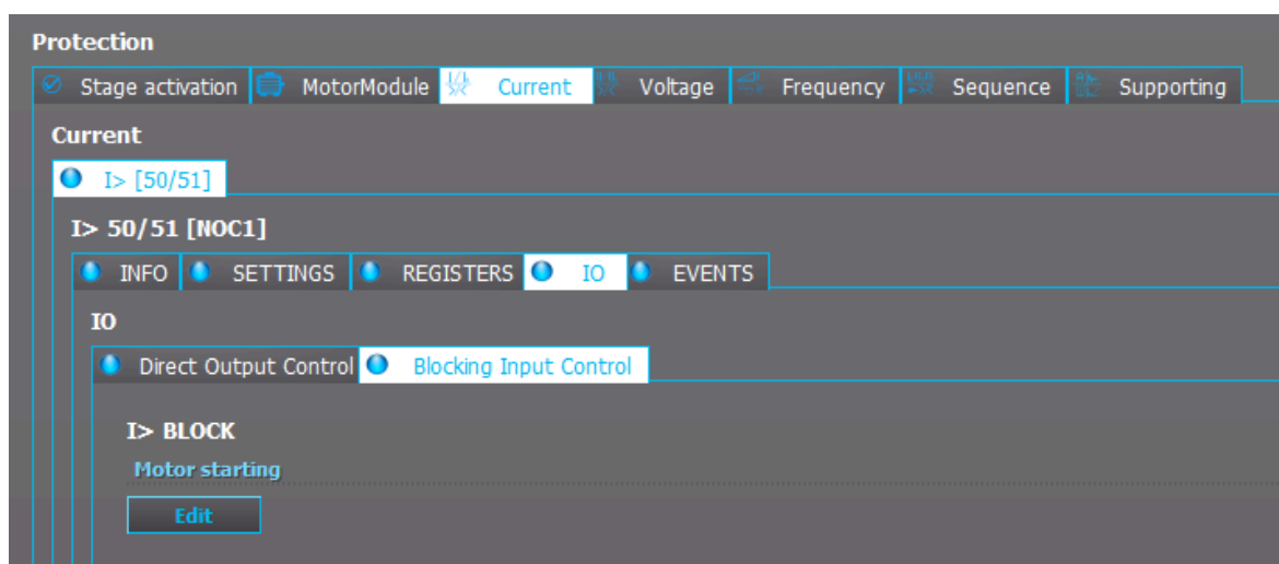
Figure. 5.4.19 - 152. Blocking application in the relay configuration.
