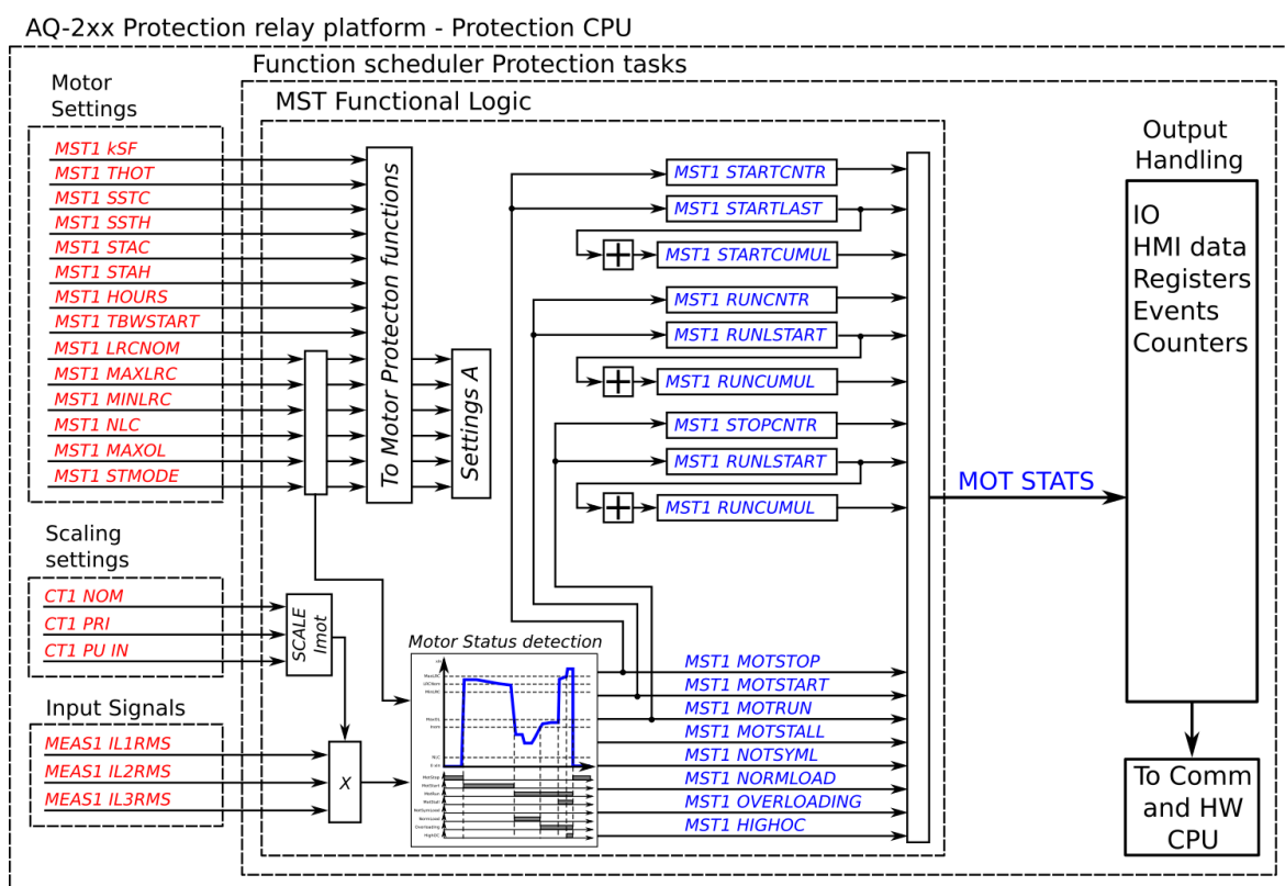
Figure. 5.4.19 - 149. Simplified function block diagram of the motor status monitoring function.
