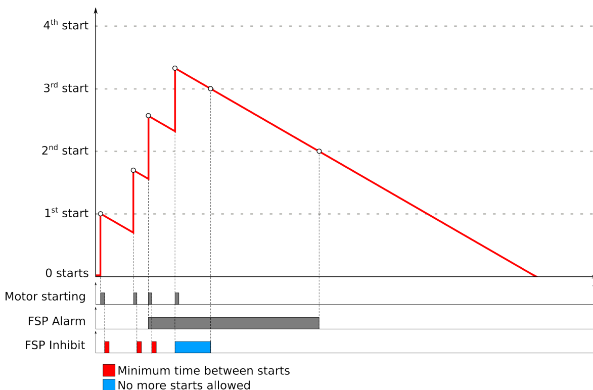
Figure. 5.4.21 - 161. Updating the function's start counter (image not to scale with regard to time).
