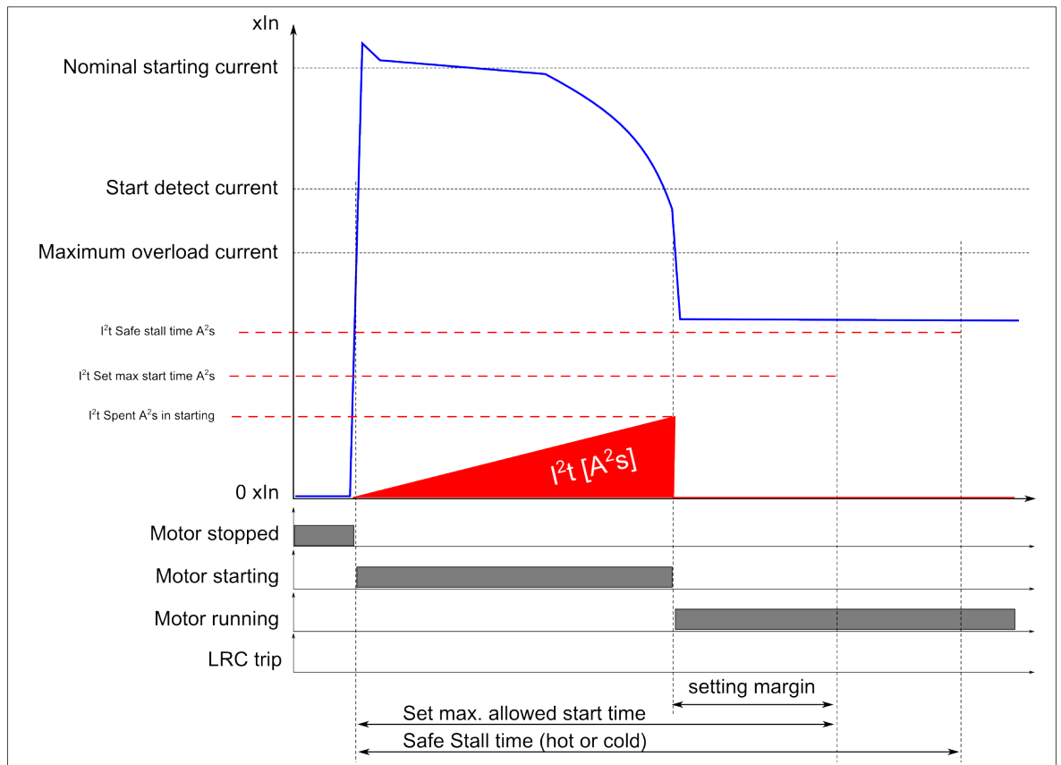
Figure. 5.4.20 - 155. Outputs in normal motor start, no speed switch.
