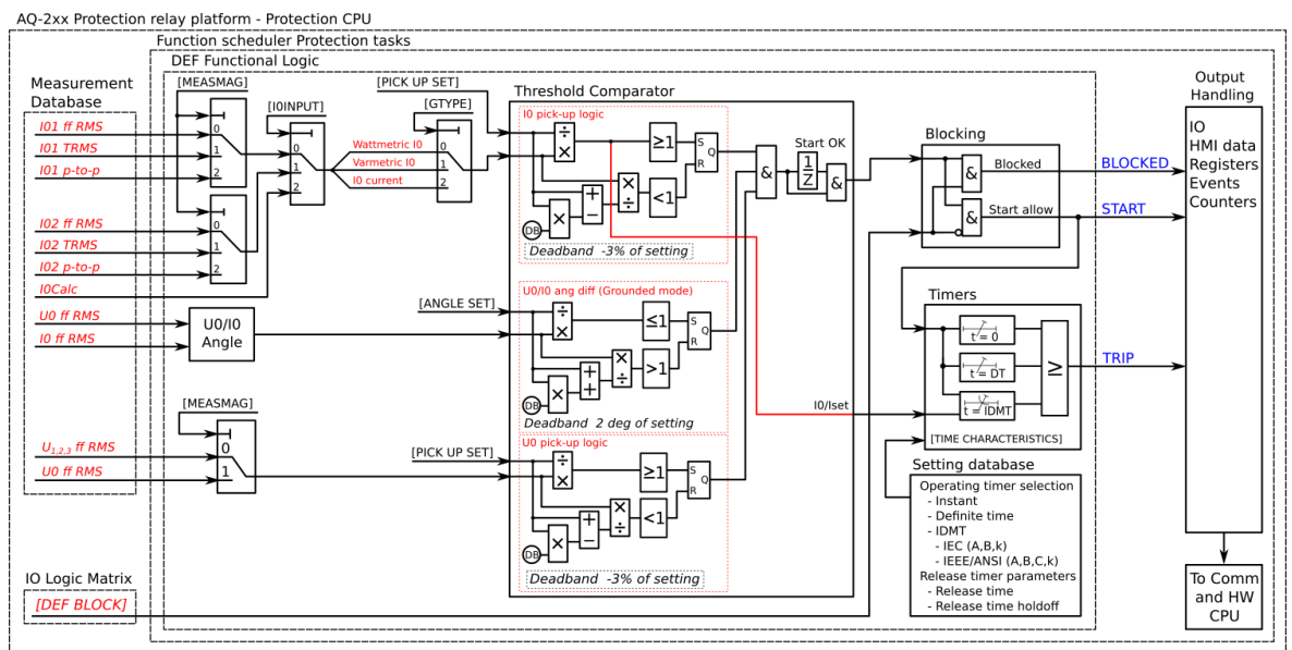
Figure. 5.4.5 - 40. Simplified function block diagram of the I0dir> function.
