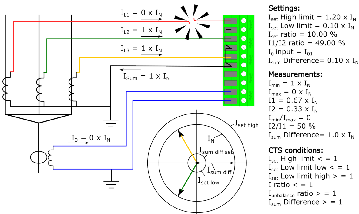
Figure. 5.6.1 - 166. Broken secondary phase current wiring.
