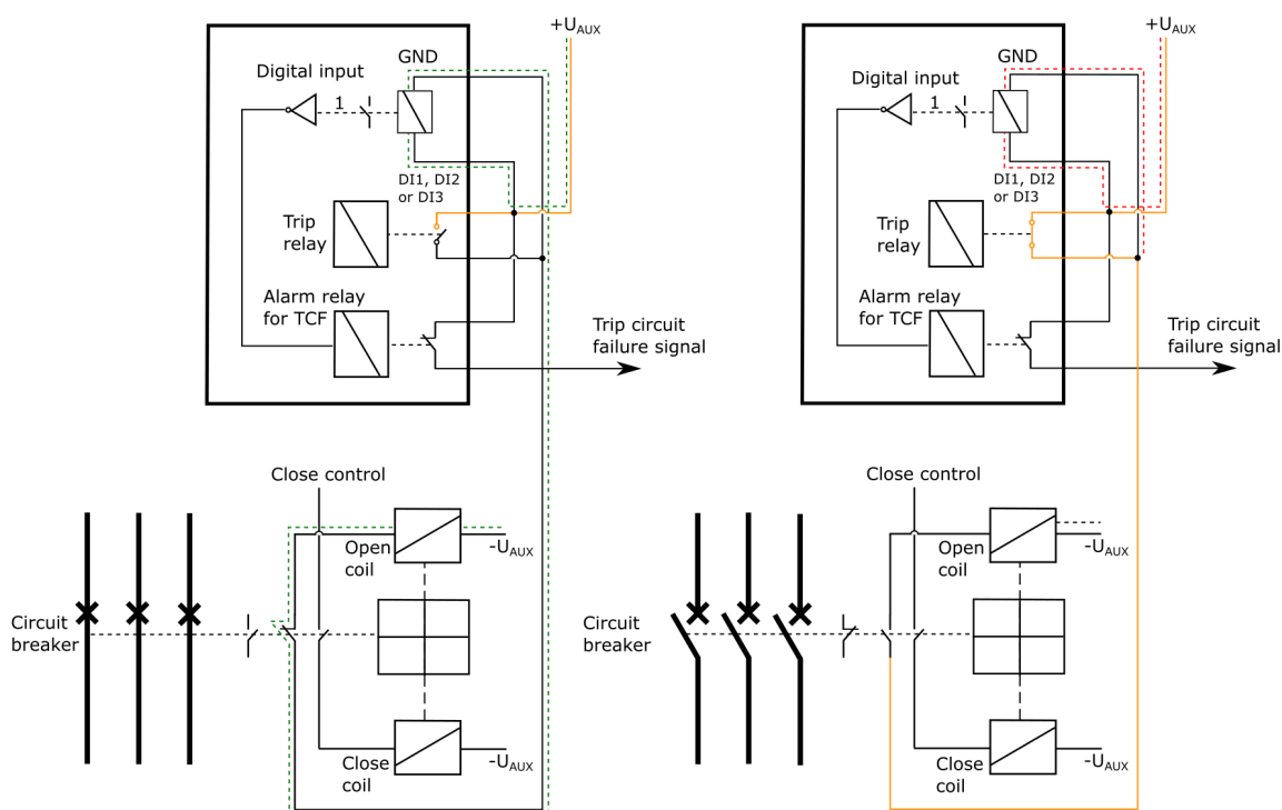
Figure. 7.4 - 189. Trip circuit supervision with one DI and one latched output contact.
