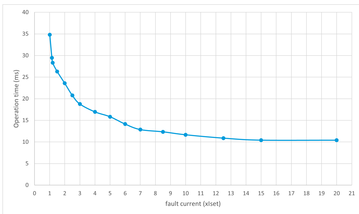
Figure. 5.4.2 - 34. Typical operation time delays with different current to setting ratios in instant operation mode.
