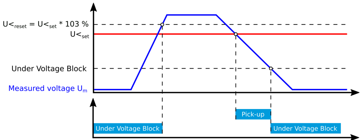
Figure. 5.4.13 - 89. Example of the block setting operation.
