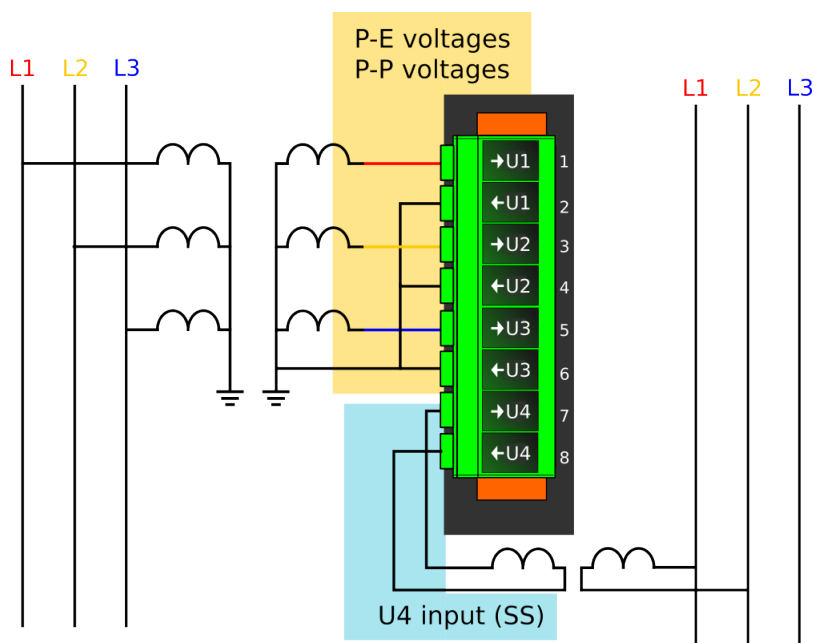
Figure. 5.4.11 - 74. Selectable measurement magnitudes with 3LN+U4 VT connection.
