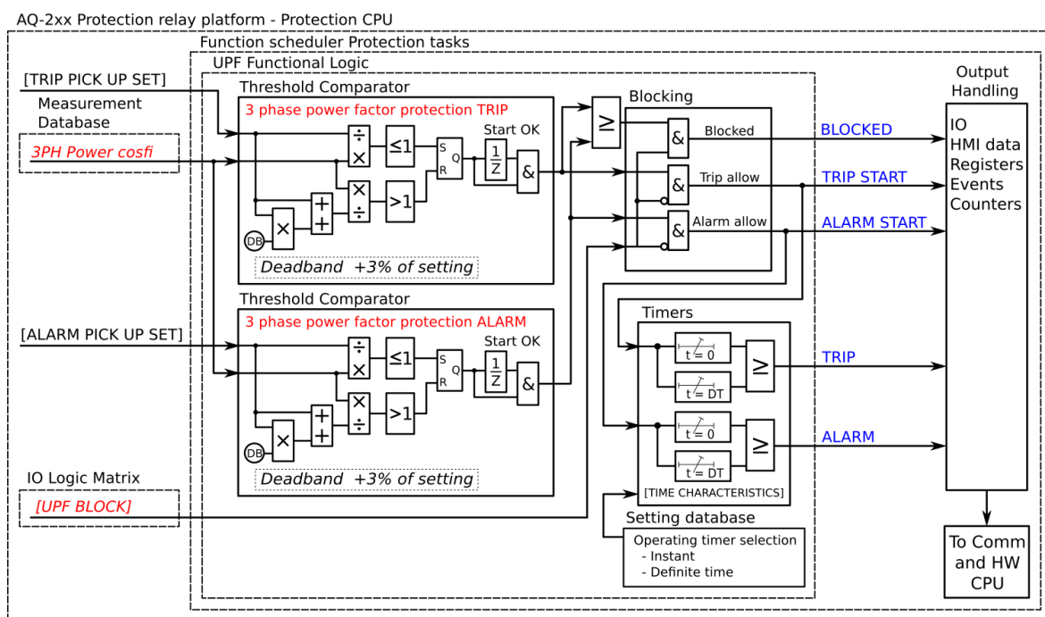
Figure. 5.4.22 - 113. Simplified function block diagram of the PF> function.
