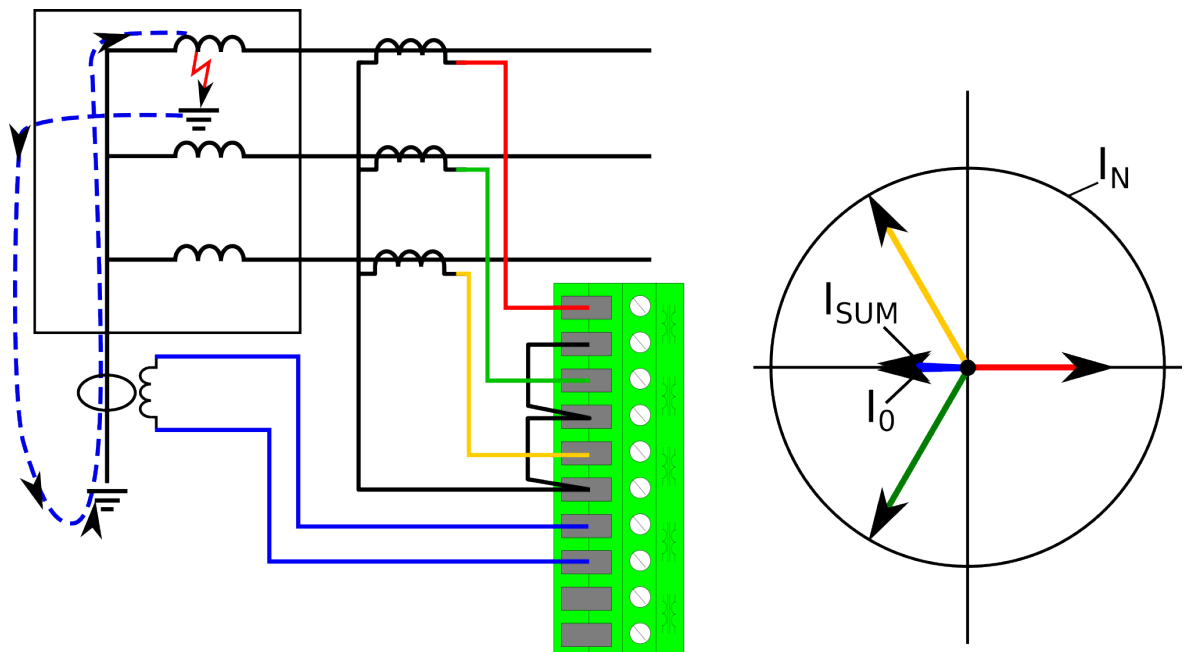
Figure. 5.4.9 - 68. Restricted earth fault inside a Y winding transformer.
