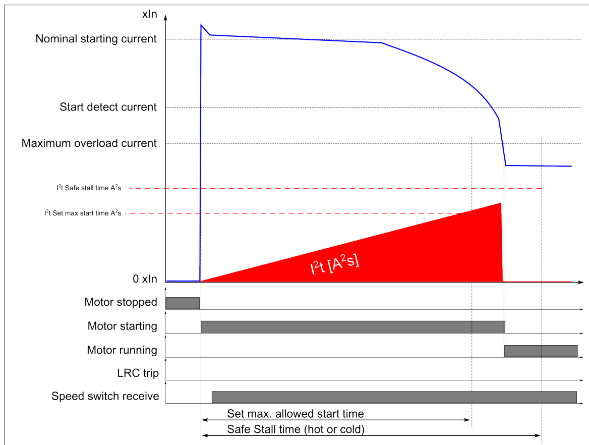
Figure. 5.4.18 - 104. Outputs in long motor starting, with a speed switch.
