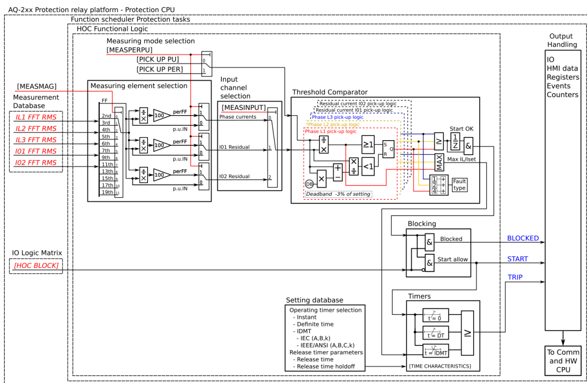
Figure. 5.4.7 - 48. Simplified function block diagram of the Ih> function.
