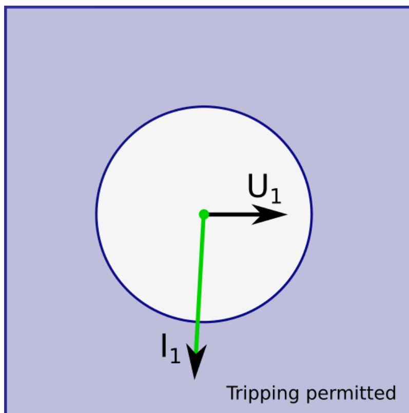
Figure. 5.4.4 - 39. When I_{dir} function has been set to "Non-directional" the function works basically just like a traditional non-directional overcurrent protection function.
