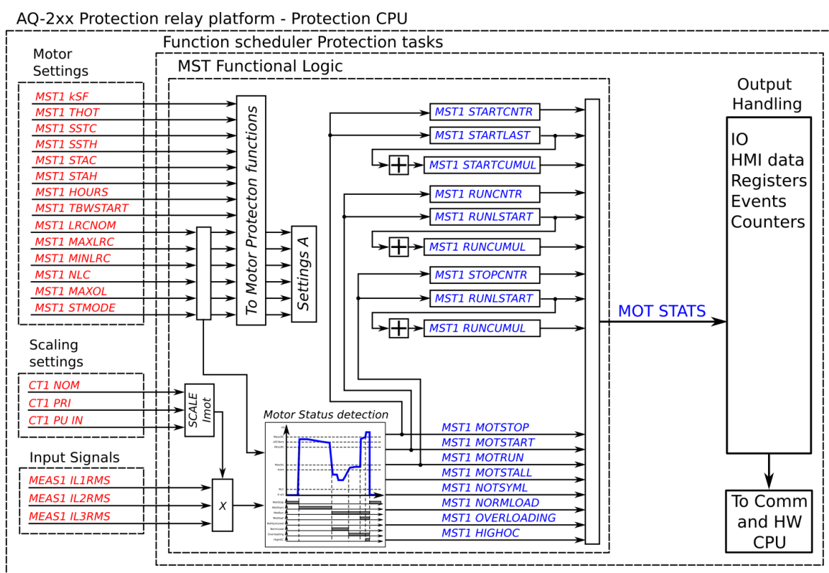
Figure. 5.4.17 - 96. Simplified function block diagram of the motor status monitoring function.
