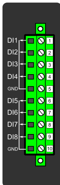
Figure. 8.5 - 197. Digital input module (DI8) with eight add-on digital inputs.
