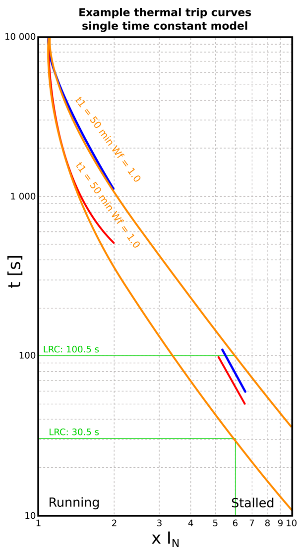
Figure. 5.4.23 - 125. Comparing single time constant thermal replica tripping curves to given motor thermal characteristics.
