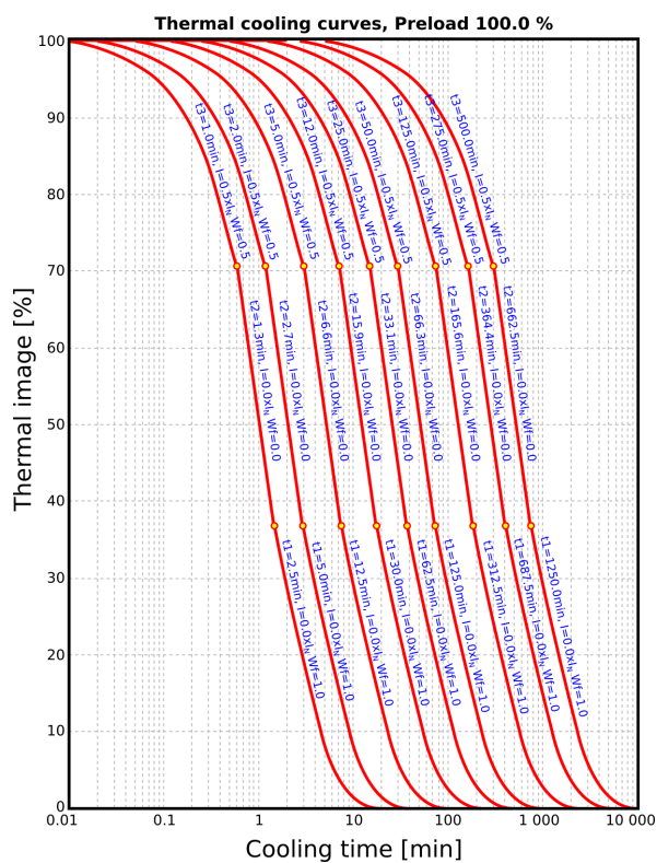
Figure. 5.4.23 - 133. Thermal cooling curves, dynamic triple time constant (motor is running without load in the first part with dedicated time constant).
