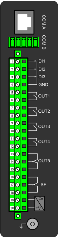
Figure. 8.2 - 194. CPU module.
