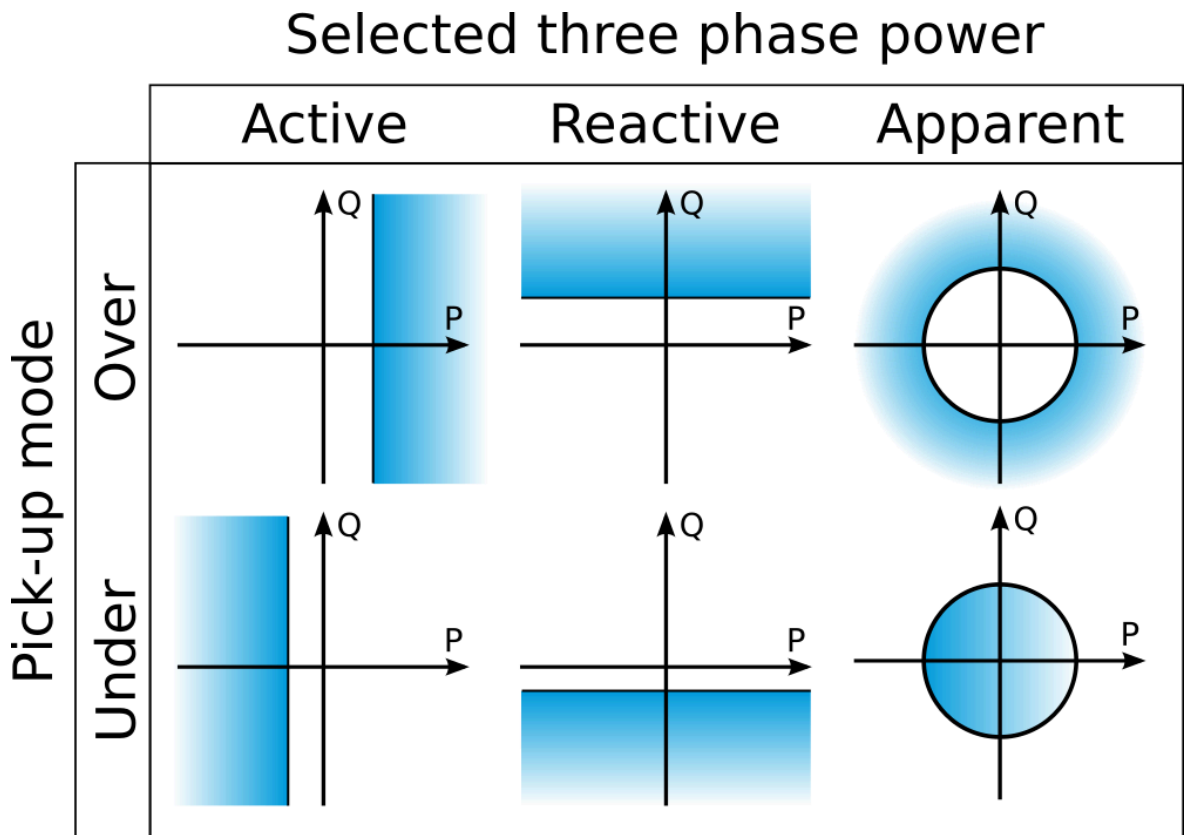
Figure. 5.4.16 - 94. PQ diagram of the pick-up areas in various modes.
