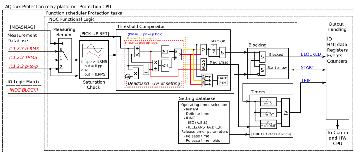
Figure. 5.4.2 - 33. Simplified function block diagram of the I> function.
