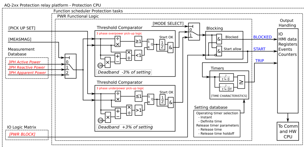
Figure. 5.4.16 - 95. Simplified function block diagram of the power protection function.
