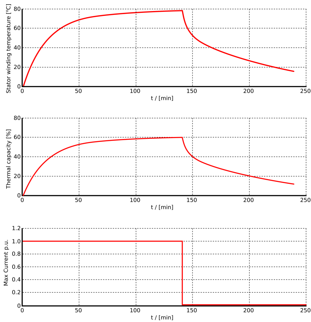
Figure. 5.4.23 - 122. Measured motor temperature in heating/cooling test.
