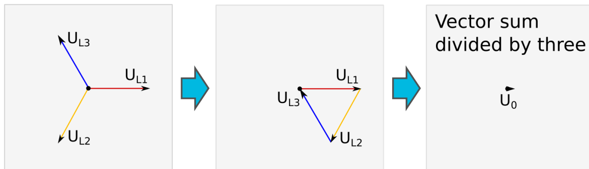
Figure. 5.4.12 - 79. Earth fault in isolated network.
