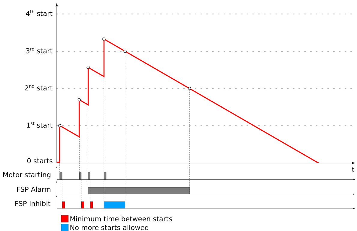
Figure. 5.4.19 - 108. Updating the function's start counter (image not to scale with regard to time).
