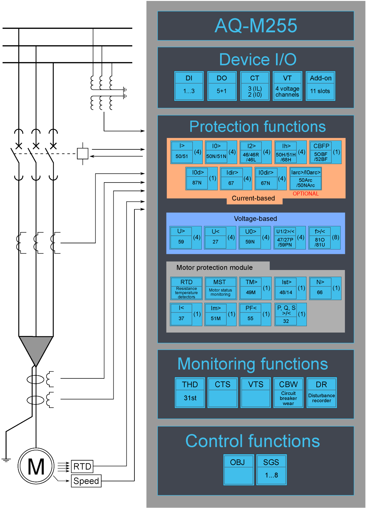
Figure. 7.1 - 183. AQ-M255 application example with function block diagram.
