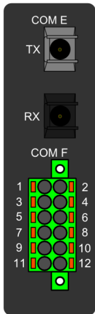
Figure. 8.9 - 203. Serial RS-232 module connectors.
