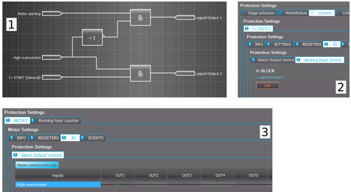
Figure. 5.4.17 - 100. Motor start up overcurrent control logic.
