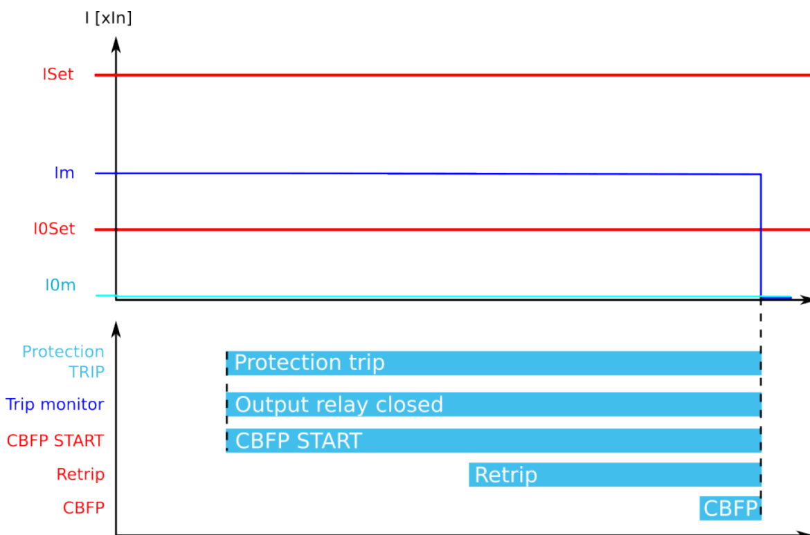
Figure. 5.4.8 - 53. Retrip and CBFP when "Current or DO" is the selected criterion.
