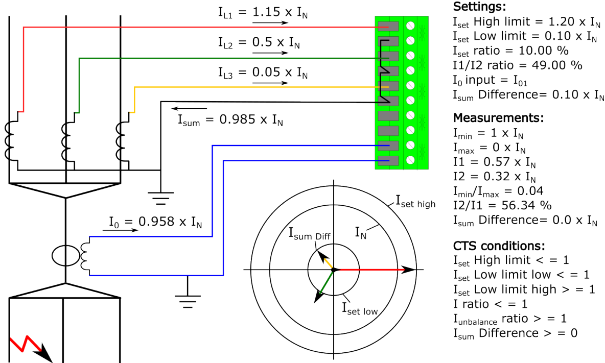
Figure. 5.6.1 - 168. Primary side high-impedance earth fault.
