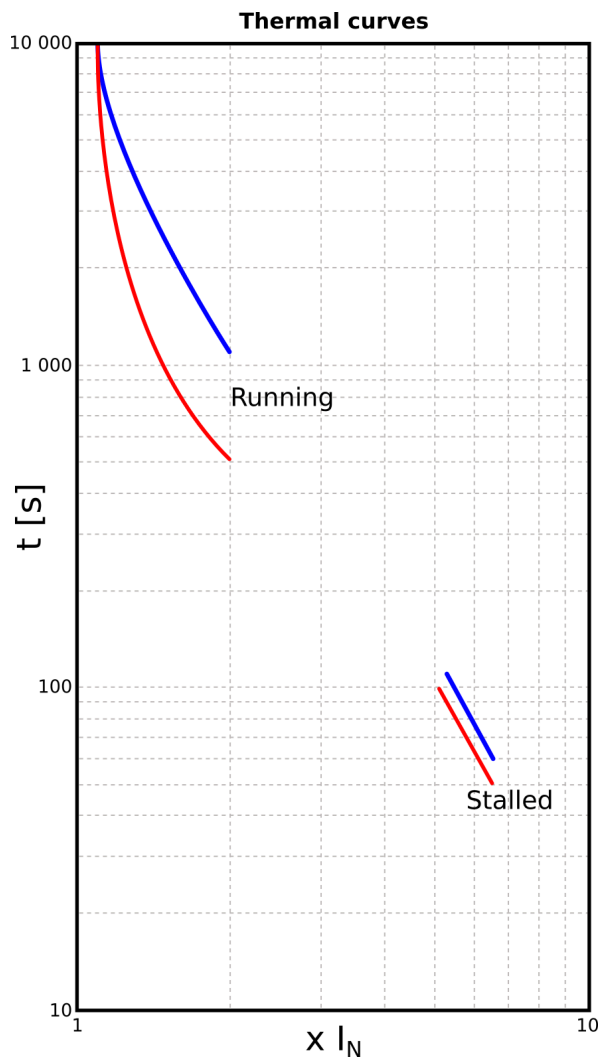
Figure. 5.4.23 - 124. Example of thermal limit curves in a motor.
