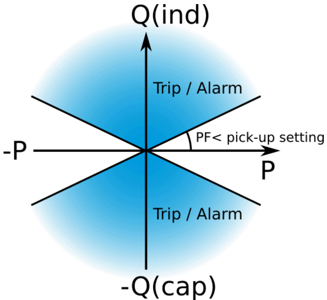
Figure. 5.4.22 - 112. Operating characteristics of power factor protection.
