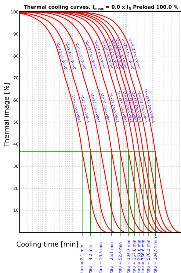
Figure. 5.4.23 - 132. Thermal cooling curves, dynamic dual time constant.
