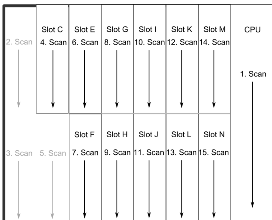
Figure. 8.1 - 193. AQ-X255 hardware scanning and I/O naming principles.
