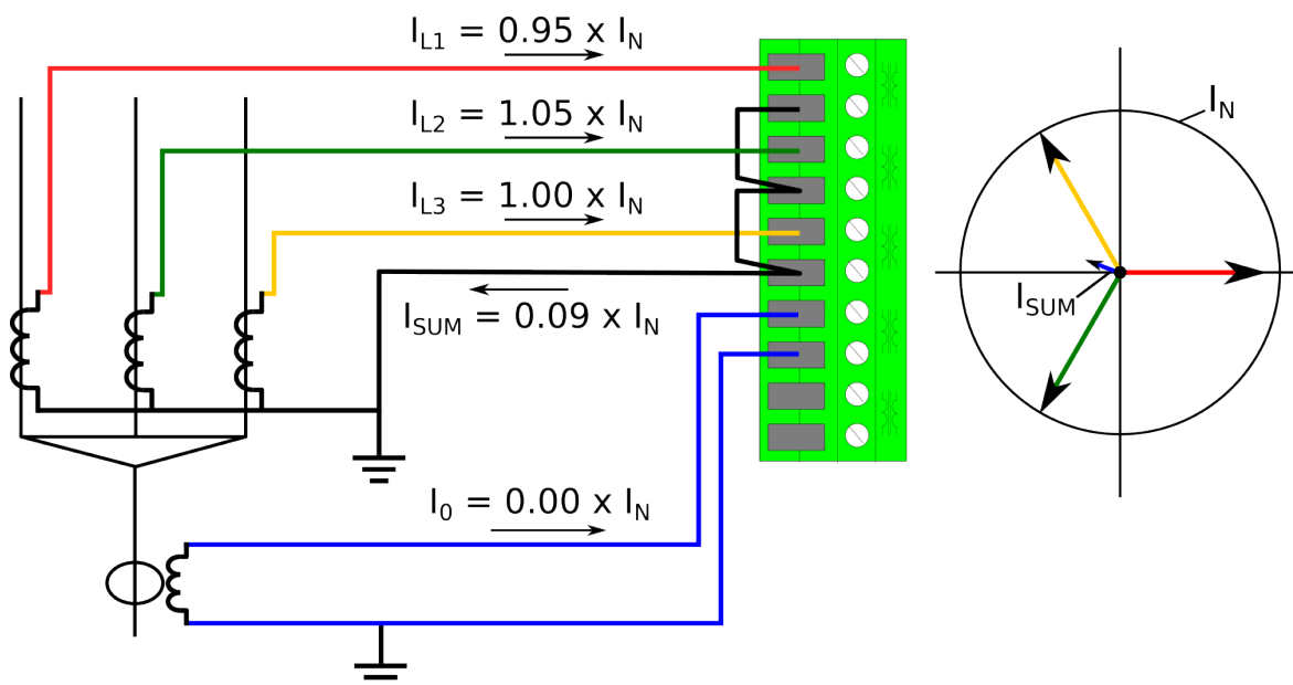
Figure. 5.4.9 - 65. Cable end differential with natural unbalance in the phase current measurement.
