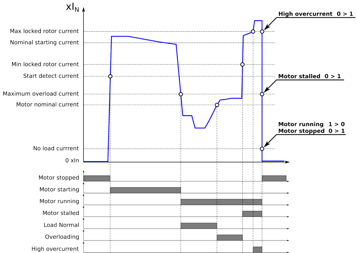
Figure. 5.4.17 - 97. Activation of the function's outputs.
