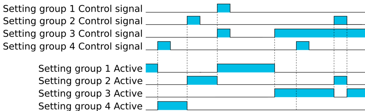
Figure. 5.5.2 - 147. Example sequences of group changing (control with pulse only, or with both pulses and static signals).
