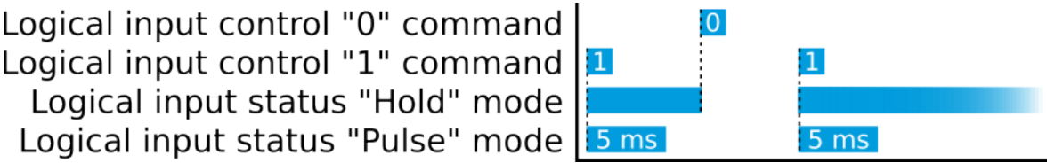
Figure. 5.5.9 - 156. Operation of logical input in "Hold" and "Pulse" modes.
