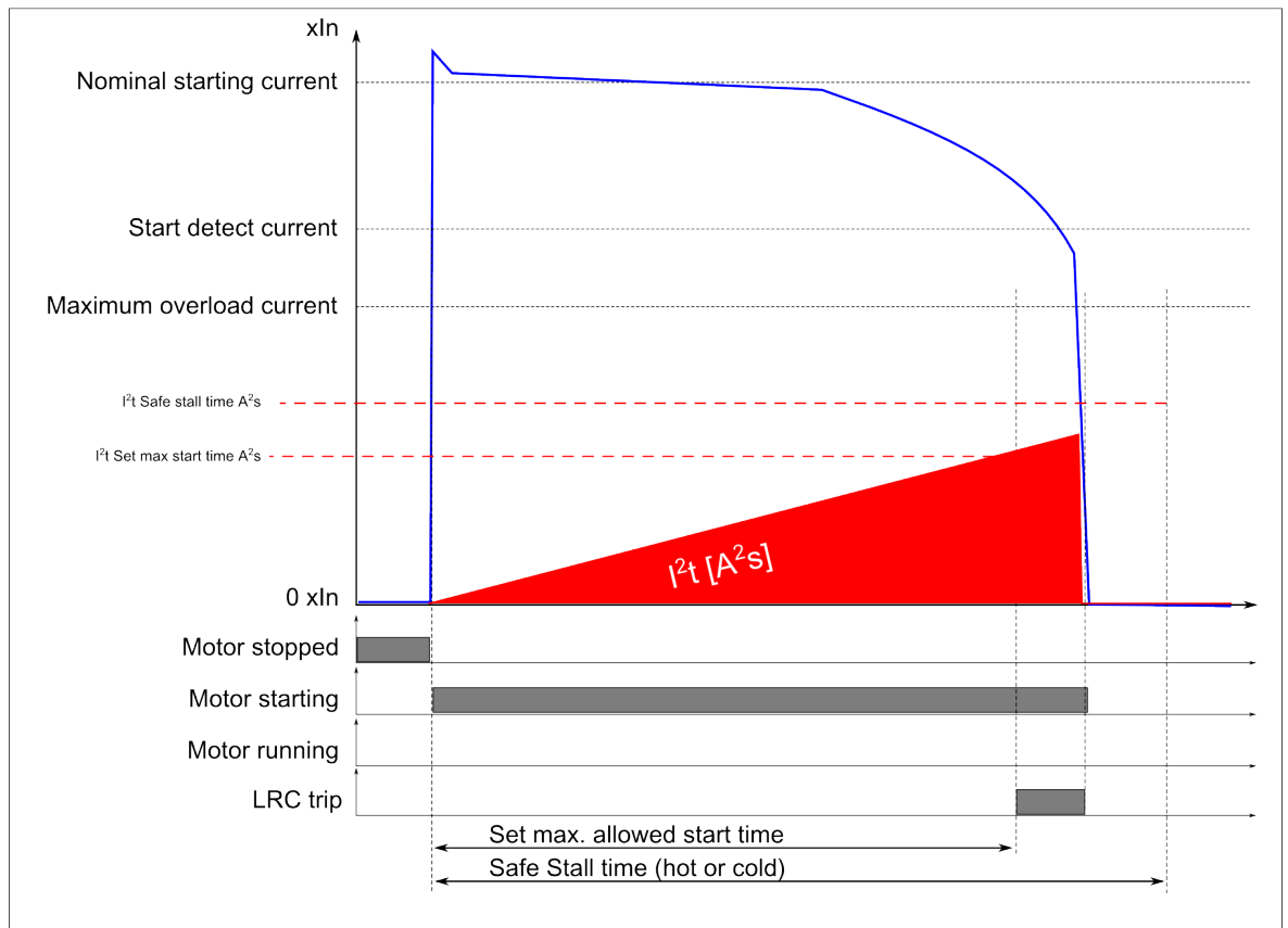
Figure. 5.4.18 - 103. Outputs when motor starting takes too long, no speed switch.
