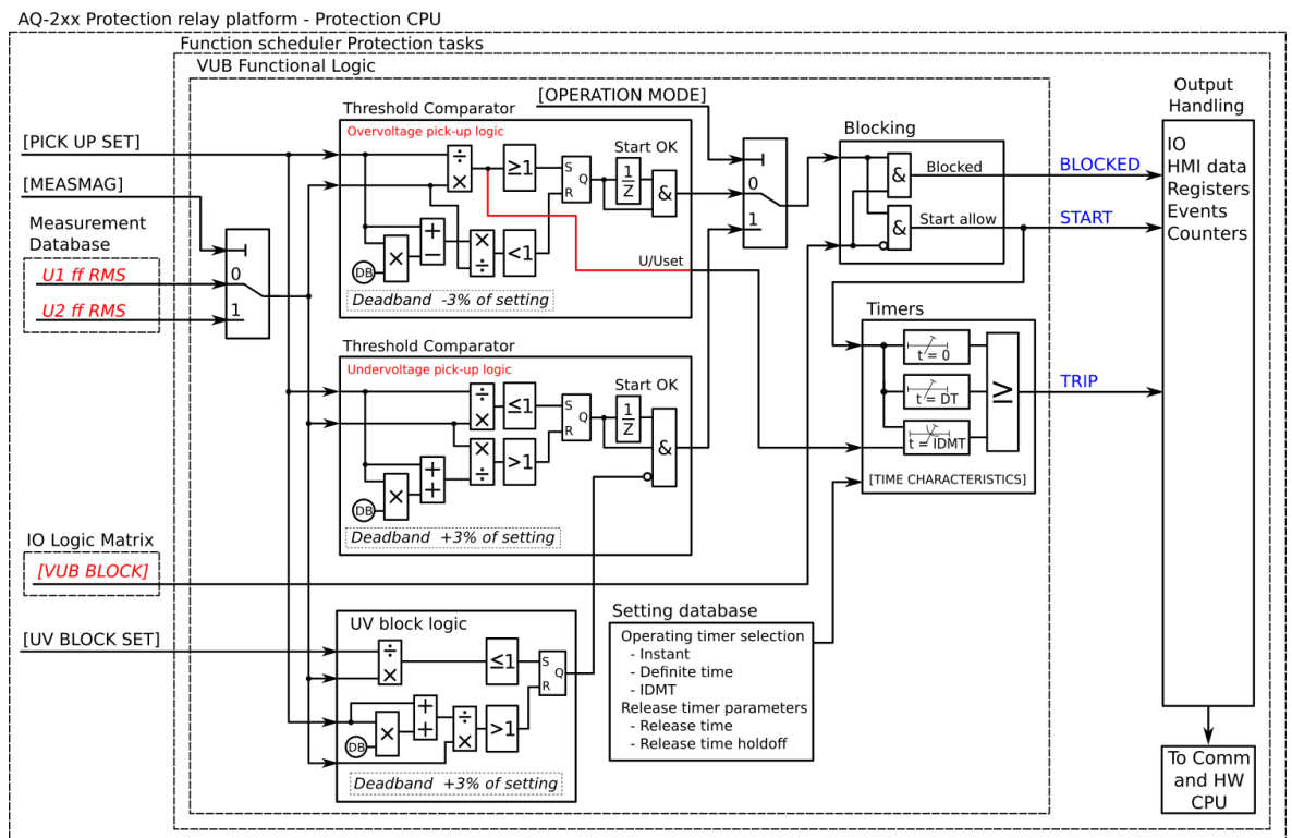
Figure. 5.4.13 - 88. Simplified function block diagram of the U1/U2>/< function.
