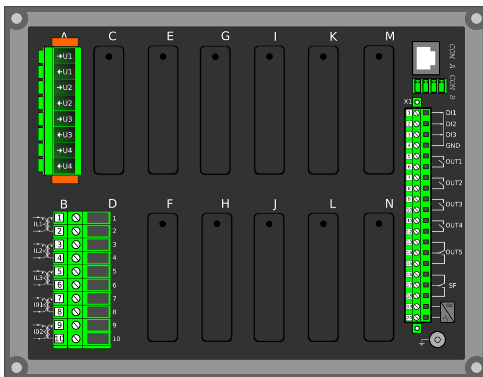
Figure. 8.1 - 191. Modular construction of AQ-X255-XXXXXXX-AAAAAAAAAAAA
