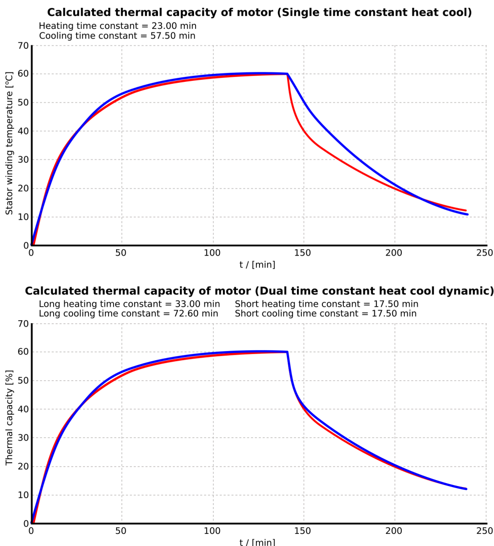
Figure. 5.4.23 - 123. Matching thermal replicas to the measured thermal capacity of the motor.
