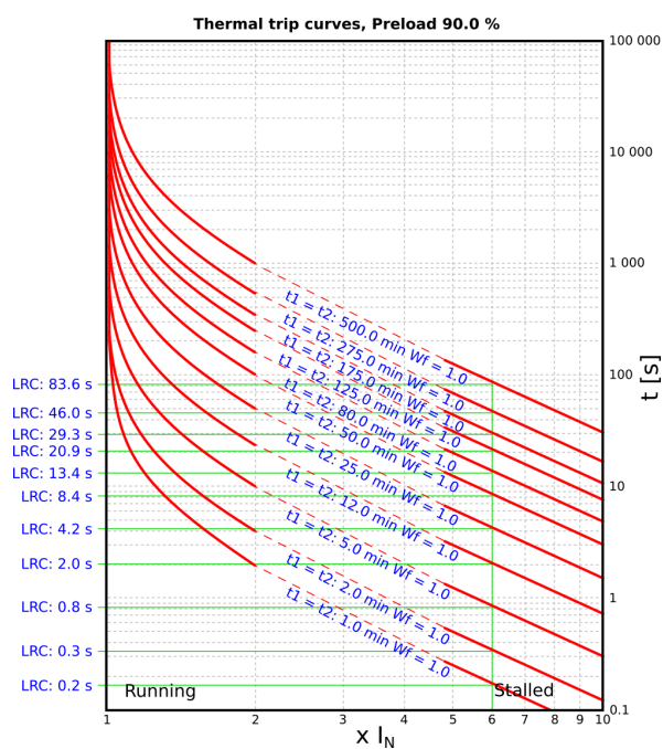
Figure. 5.4.23 - 128. Thermal tripping curves with single time constant, pre-load 90% (hot).
