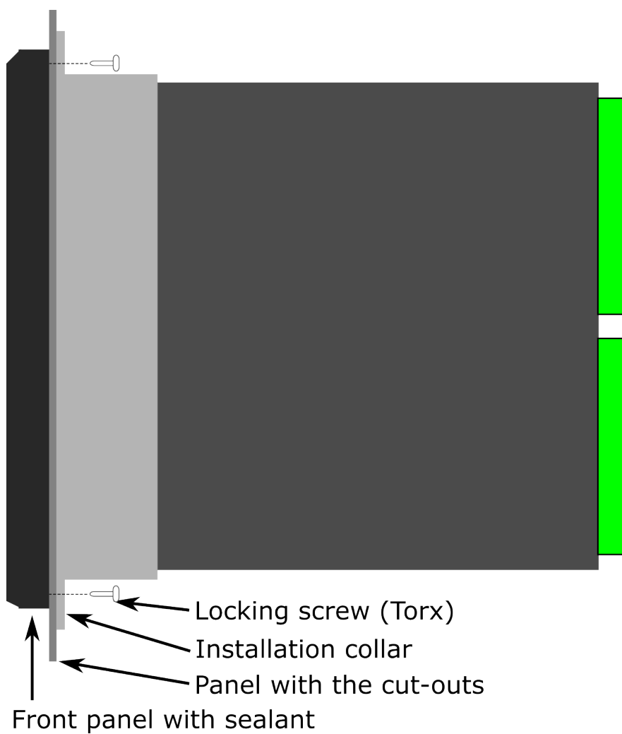
Figure. 8.14 - 212. Device installation.
