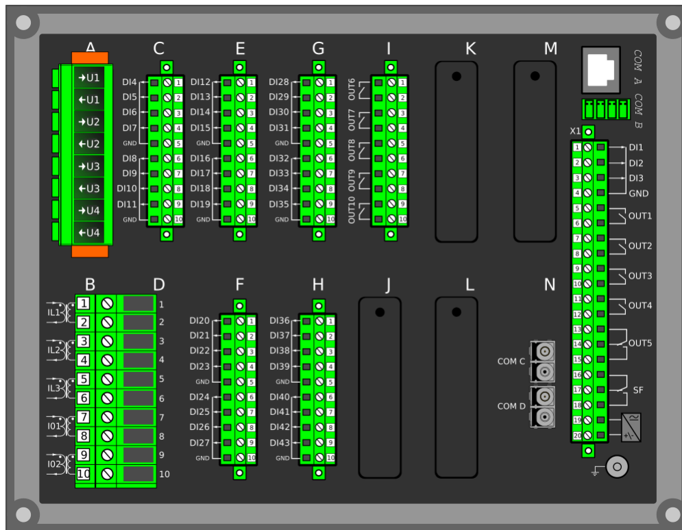
Figure. 8.1 - 192. Modular construction of AQ-X255-XXXXXXX-BBBBBCAAAAJ
