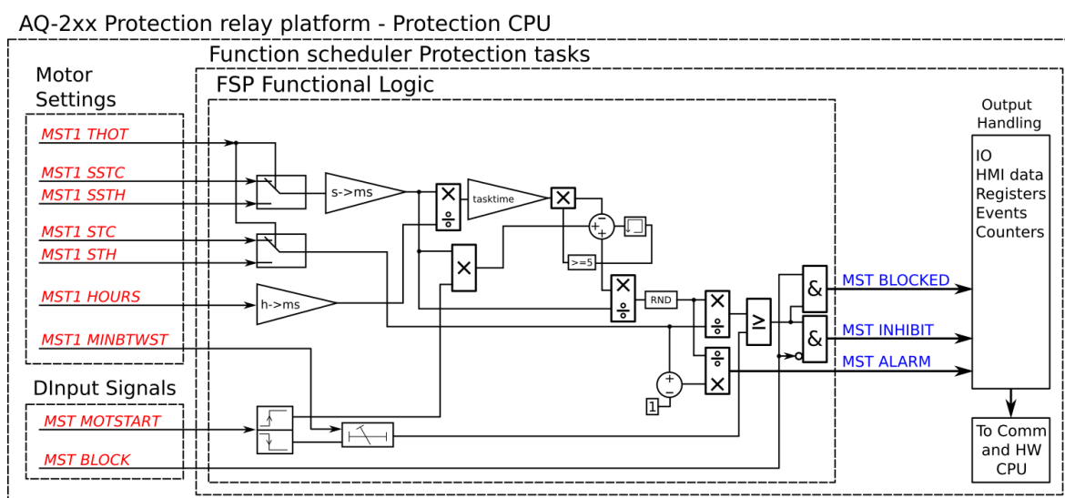
Figure. 5.4.19 - 107. Simplified function block diagram of the N> function.
