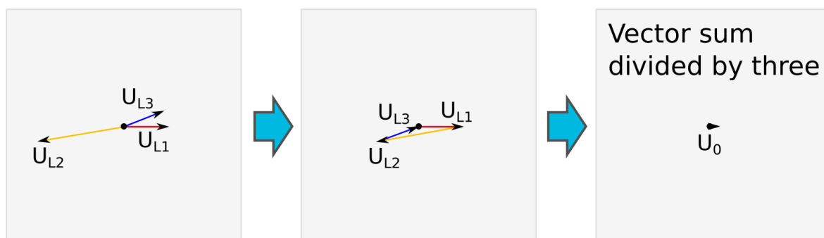
Figure. 5.4.12 - 80. Close-distance short-circuit between phases 1 and 3.
