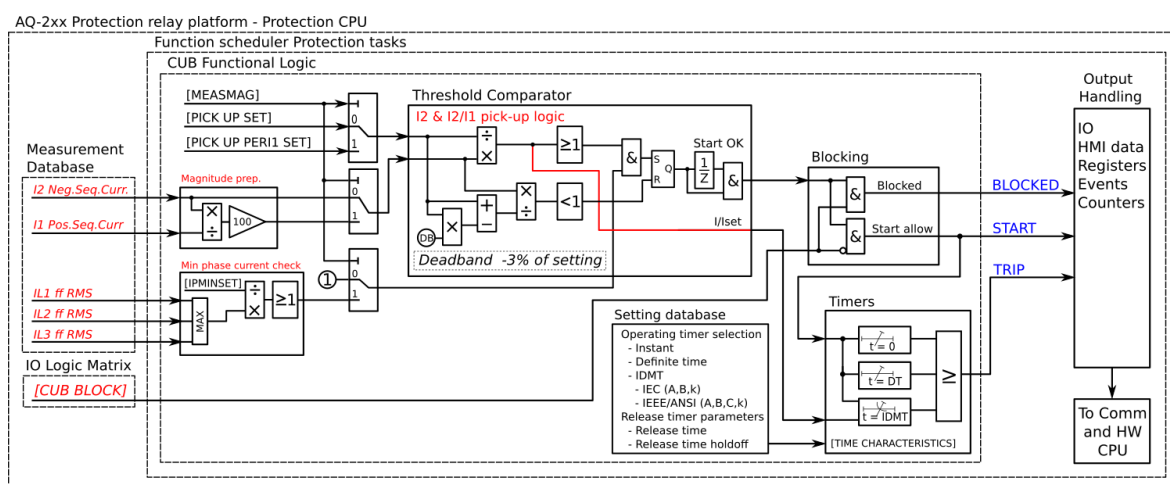
Figure. 5.4.6 - 46. Simplified function block diagram of the I2> function.
