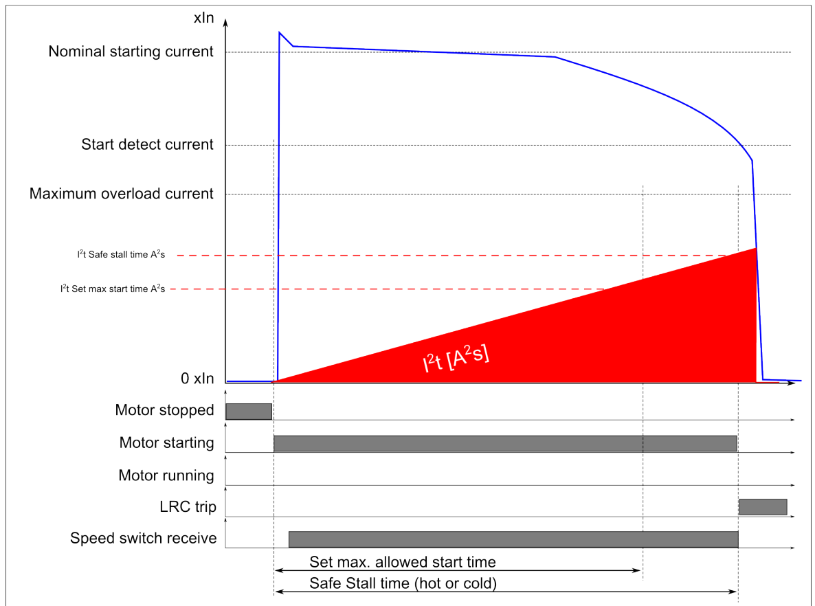
Figure. 5.4.18 - 105. Outputs when motor starting takes too long, with a speed switch.
