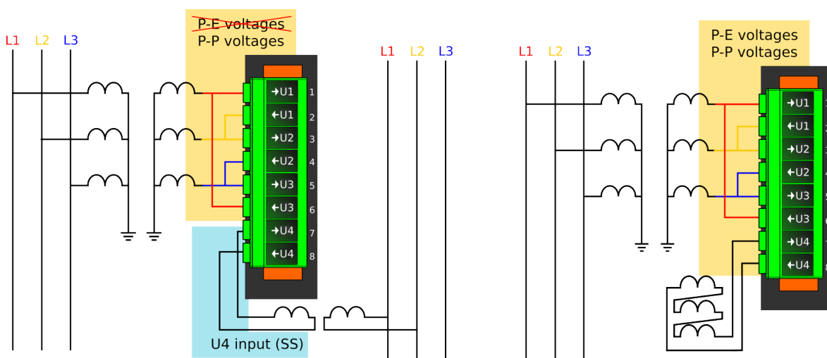
Figure. 5.4.10 - 71. Selectable measurement magnitudes with 3LL+U4 VT connection (P-E voltages not available without residual voltage).
