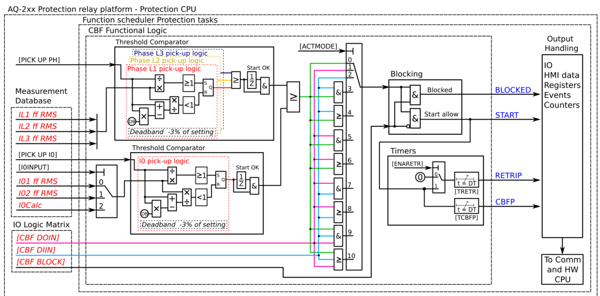
Figure. 5.4.8 - 49. Simplified function block diagram of the CBFP function.
