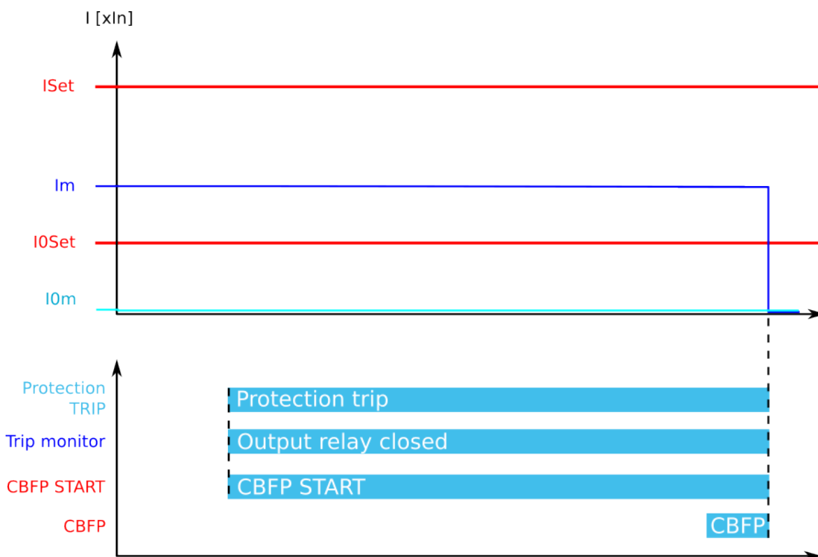
Figure. 5.4.8 - 57. CBFP when "Current or DO" is the selected criterion.
