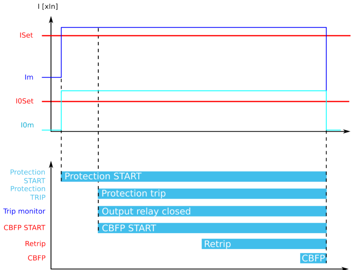
Figure. 5.4.8 - 52. Retrip and CBFP when "Current and DO" is the selected criterion.
