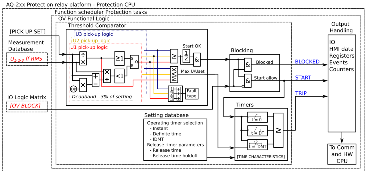
Figure. 5.4.10 - 69. Simplified function block diagram of the U> function.
