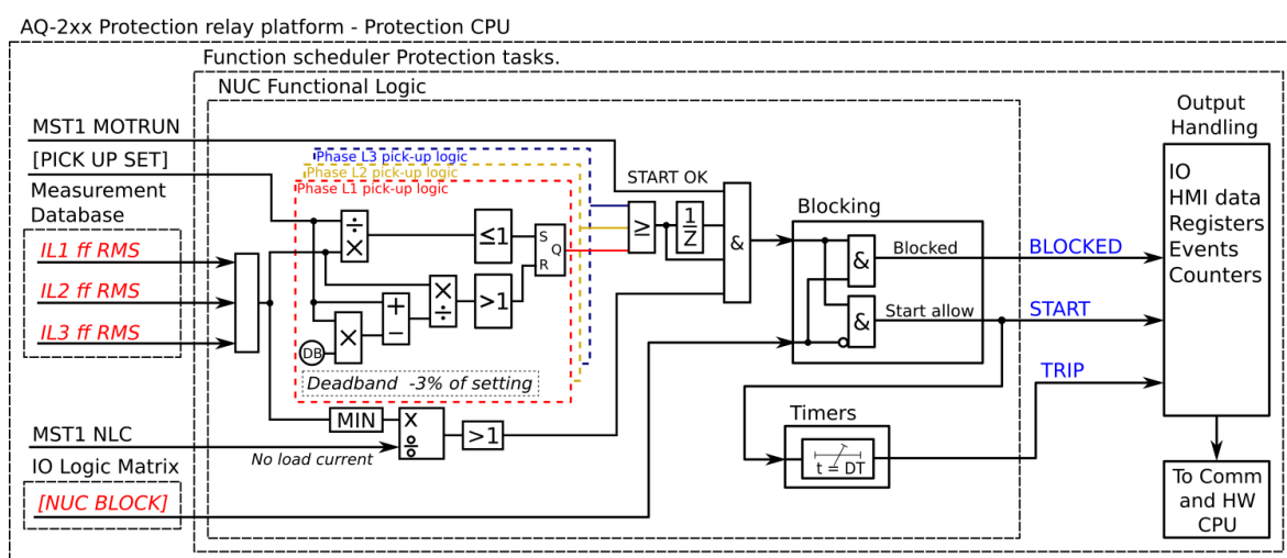
Figure. 5.4.20 - 110. Simplified function block diagram of the I< function.
