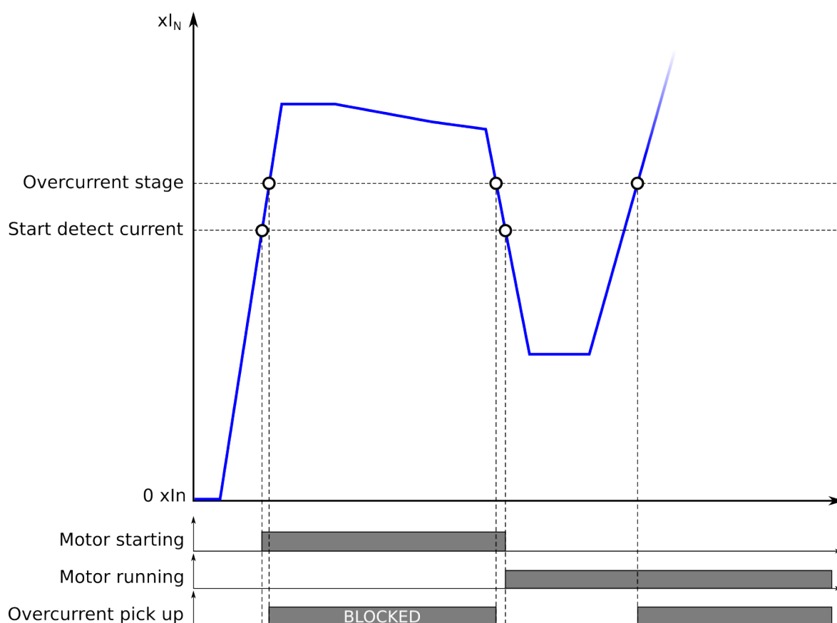
Figure. 5.4.17 - 98. Example of application: motor starting scheme and using motor status signals.
