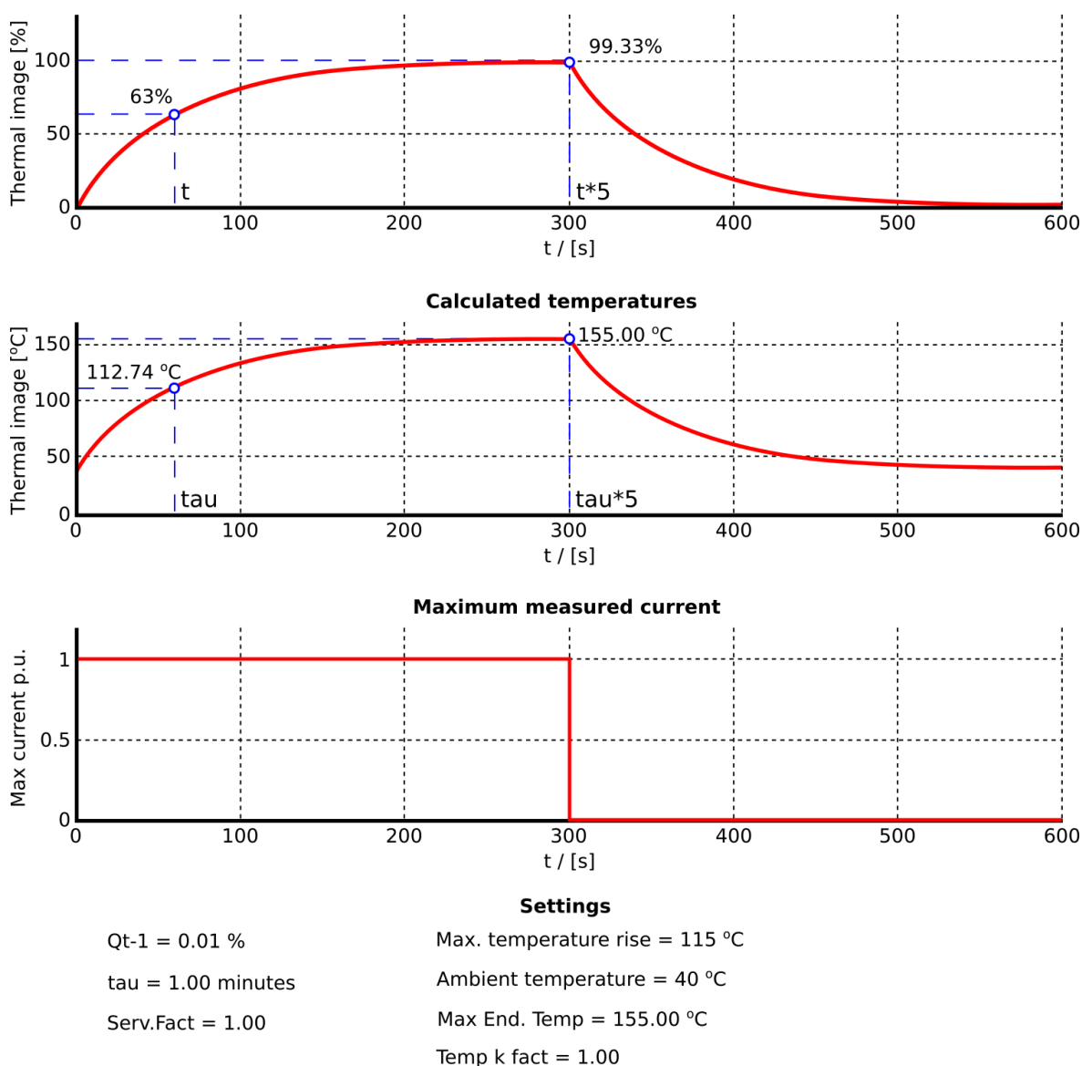
Figure. 5.4.23 - 116. Thermal image calculation with nominal conditions: single time constant thermal replica.
