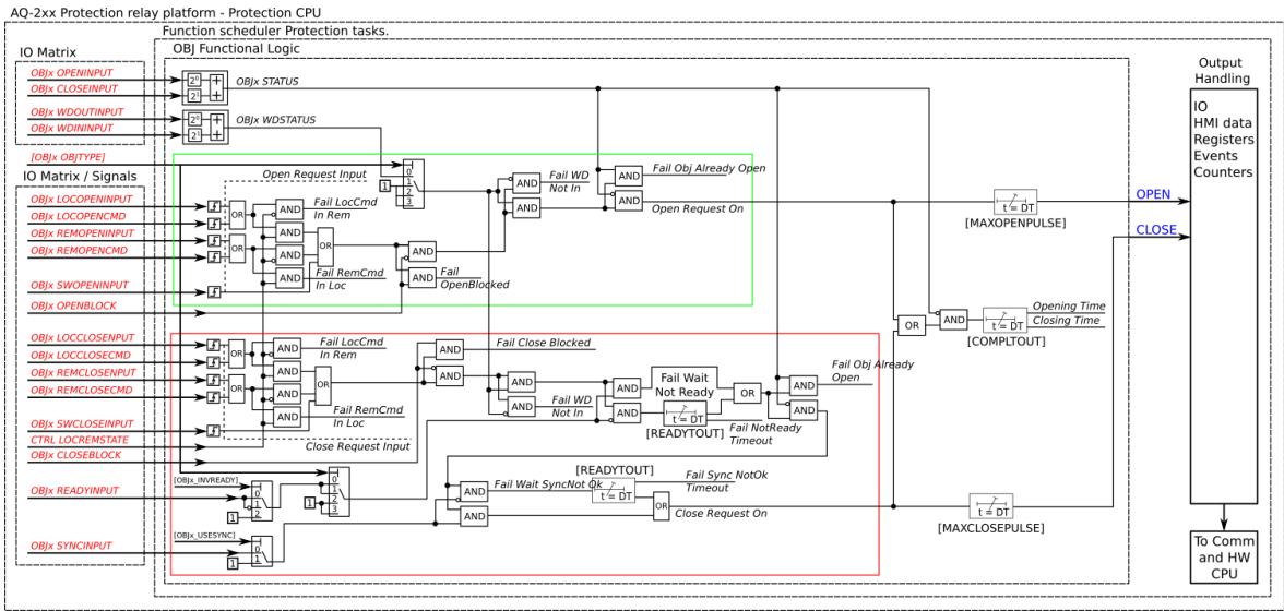
Figure. 5.5.3 - 152. Simplified function block diagram of the object control and monitoring function.
