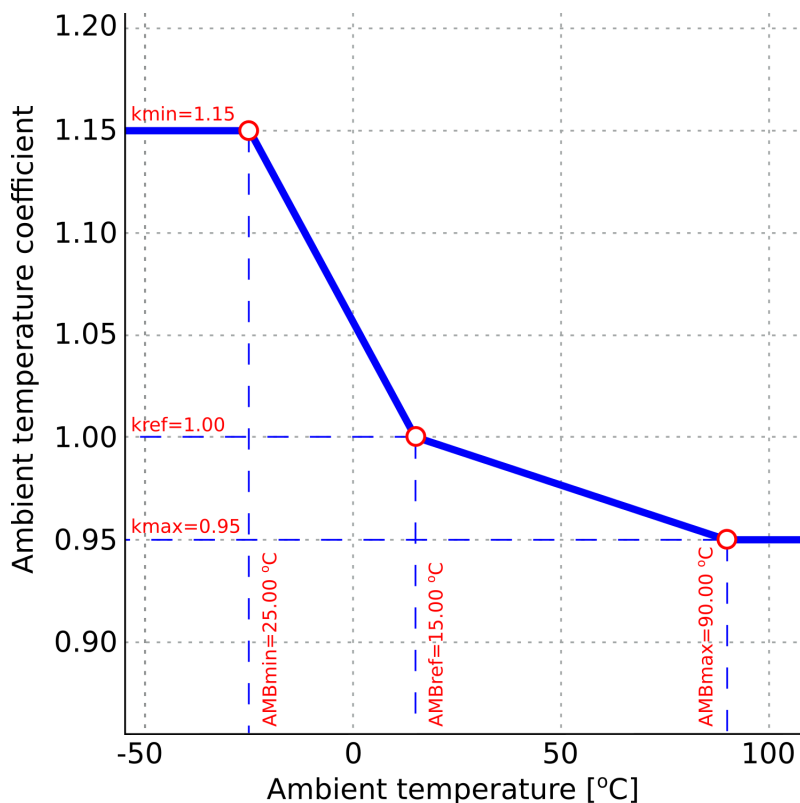
Figure. 5.4.23 - 117. Ambient temperature coefficient calculation (linear approximation, three points).
