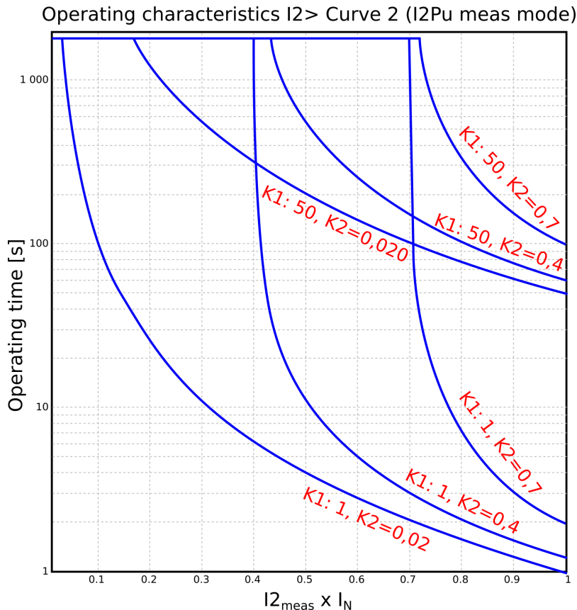
Figure. 5.4.6 - 47. Operation characteristics curve for I2> Curve2.
