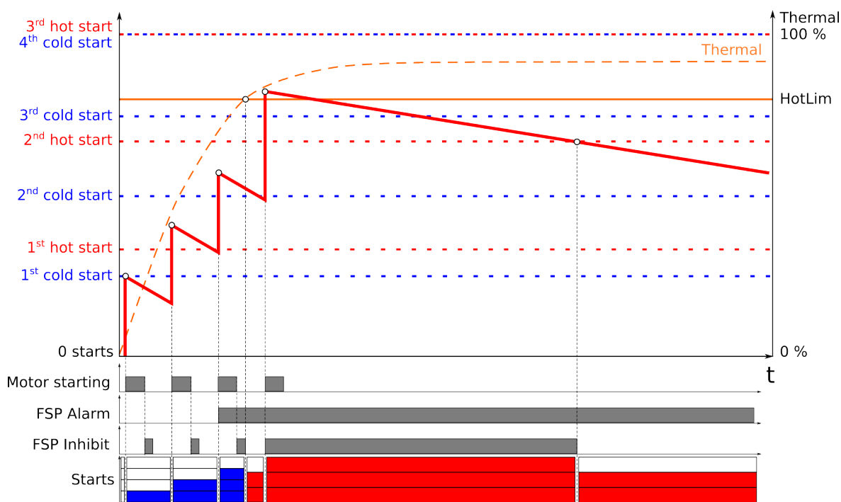
Figure. 5.4.19 - 109. Updating the starts counter when thermal hot and cold status taken into consideration.
