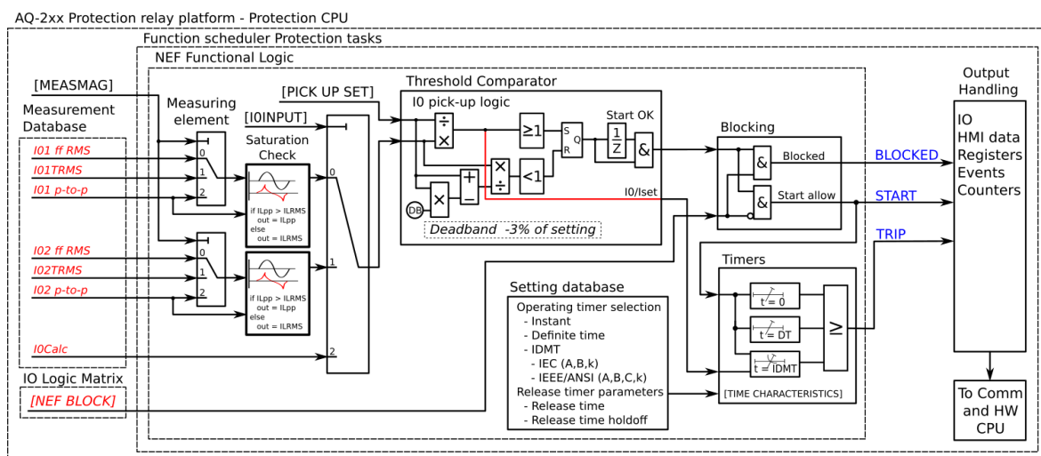
Figure. 5.4.3 - 35. Simplified function block diagram of the I0&gt; function.
