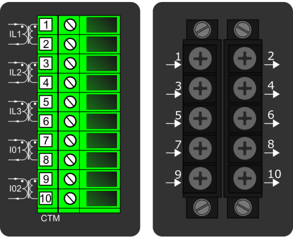
Figure. 8.3 - 195. Module connections with standard and ring lug terminals.
