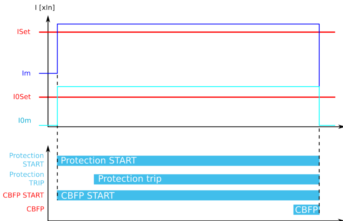
Figure. 5.4.8 - 55. CBFP when "Current" is the selected criterion.
