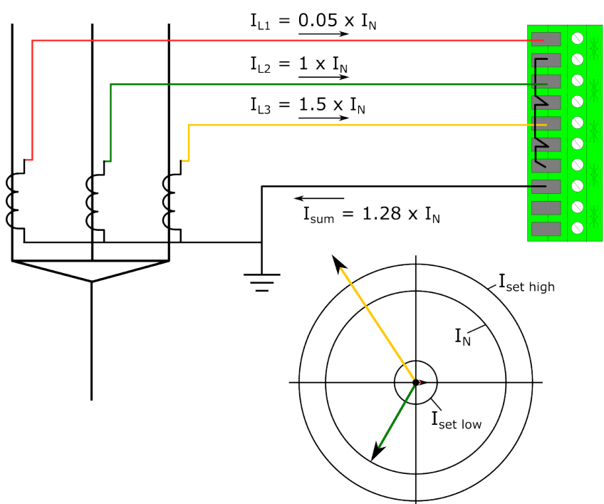
Figure. 5.6.1 - 163. No wiring fault but heavy unbalance.
