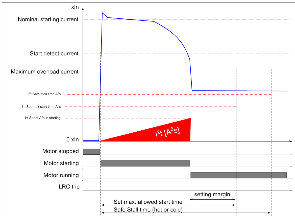
Figure. 5.4.18 - 102. Outputs in normal motor start, no speed switch.
