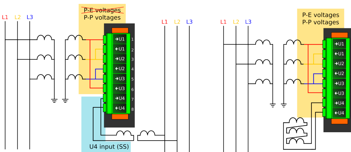
Figure. 5.4.11 - 76. Selectable measurement magnitudes with 2LL+U4 VT connection (P-E voltages not available without residual voltage).
