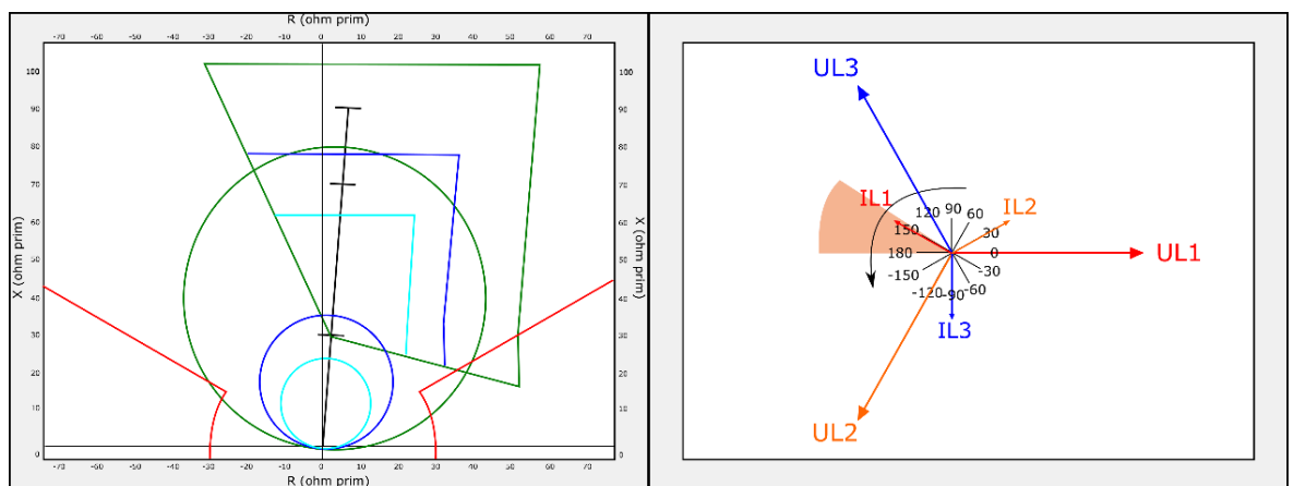
Figure. 5.4.26 - 143. Distance protection characteristics and directional overcurrent.
