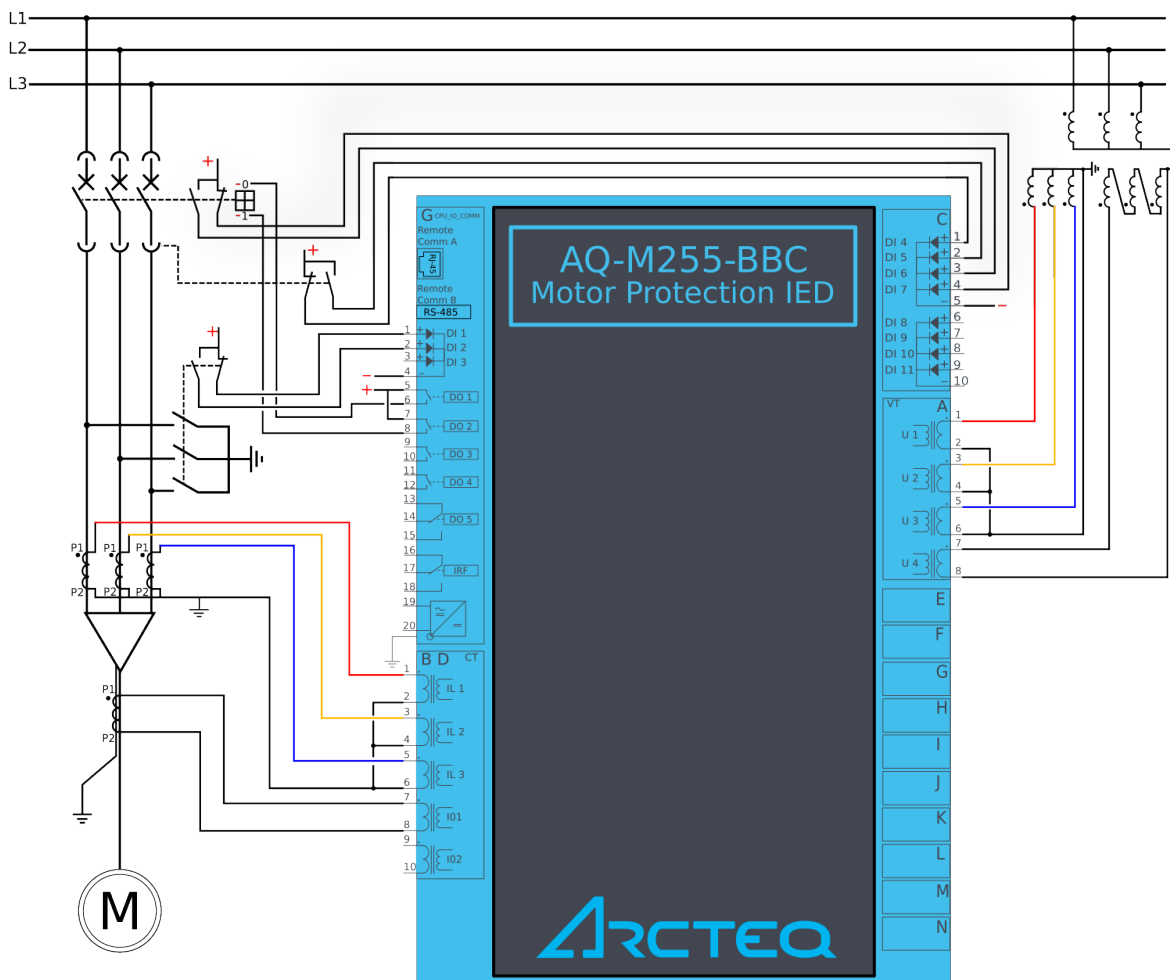
Figure. 7.2 - 184. Application example and its connections.
