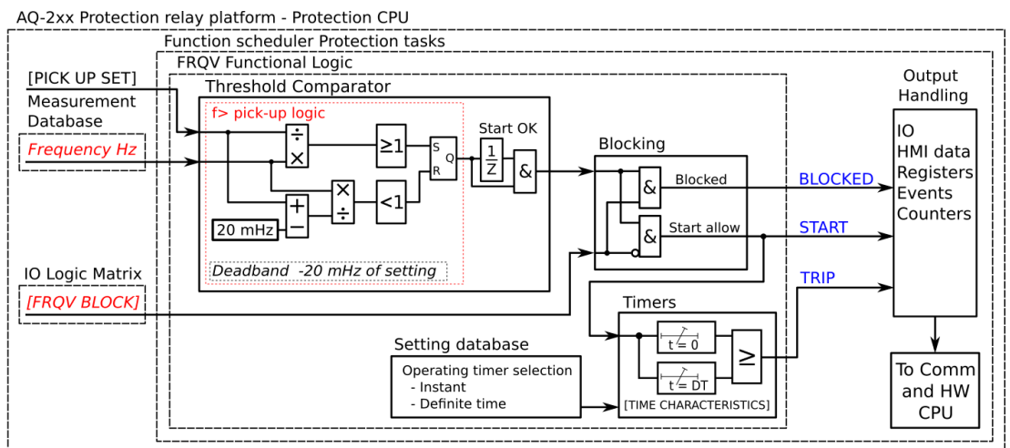
Figure. 5.4.14 - 90. Simplified function block diagram of the f > function.
