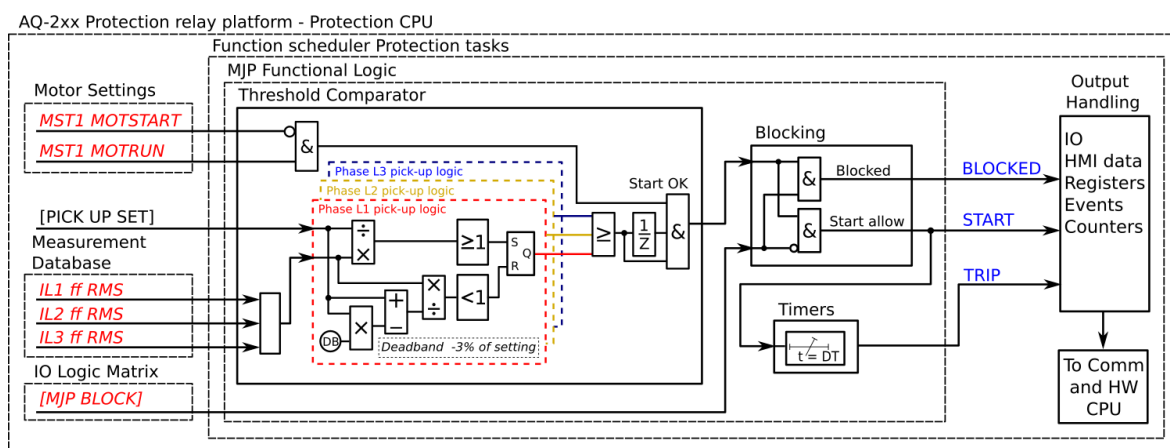
Figure. 5.4.21 - 111. Simplified function block diagram of the Im> function.
