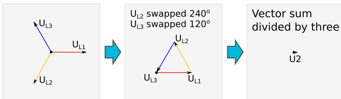
Figure. 5.4.13 - 86. Earth fault in isolated network.
