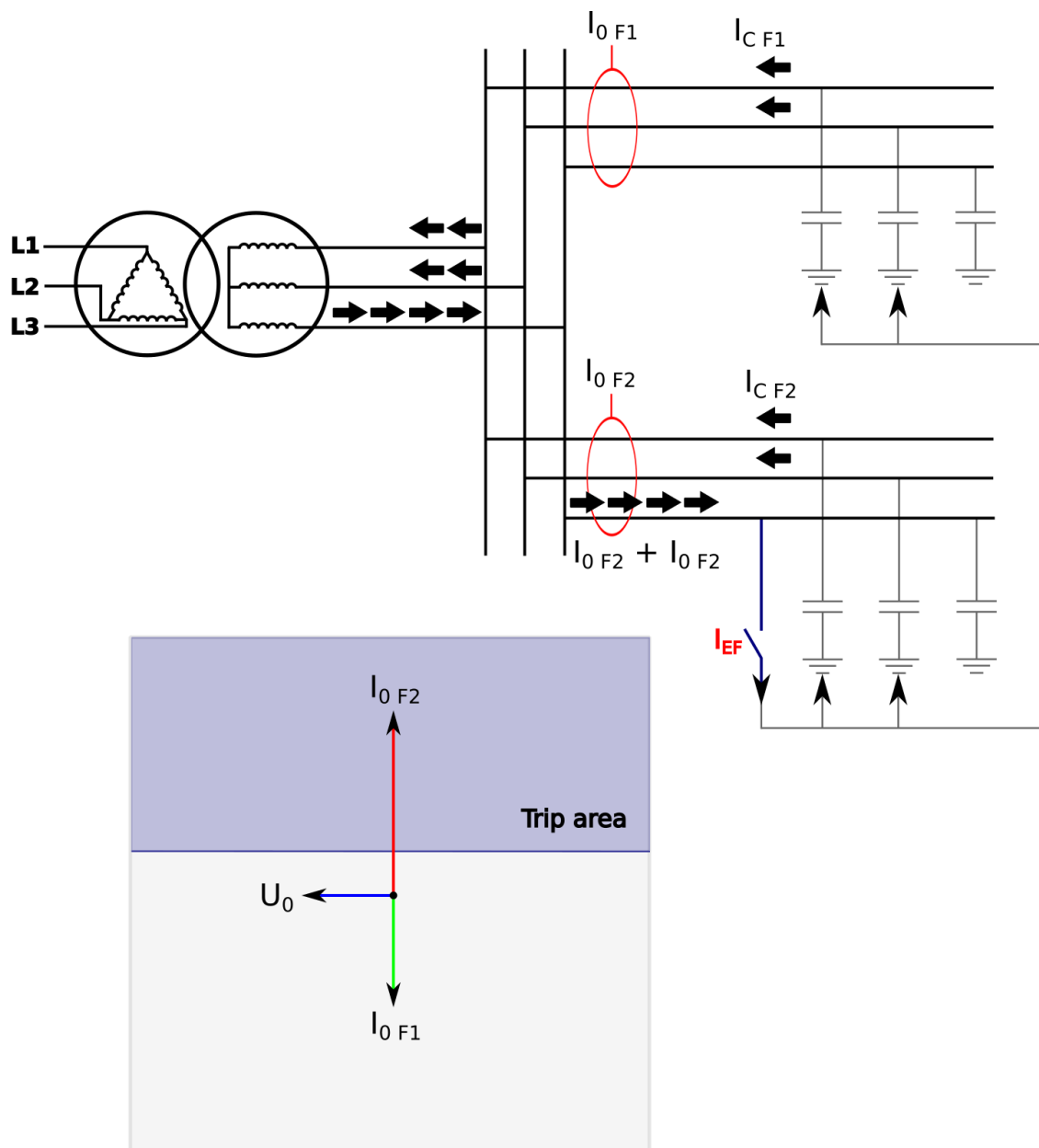
Figure. 5.4.5 - 41. Angle tracking of I_{0dir} function (unearthed network model) (32N)
