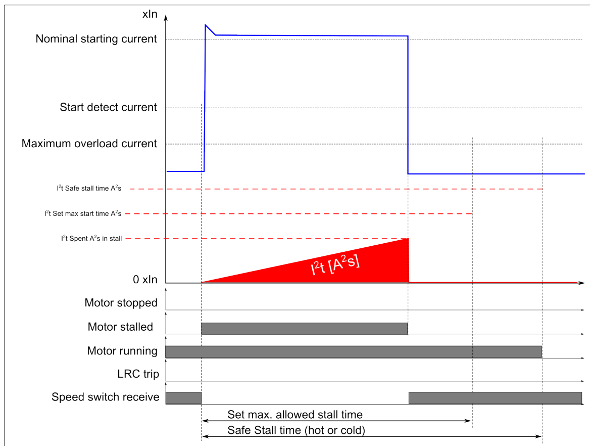
Figure. 5.4.18 - 106. Motor stall monitoring.
