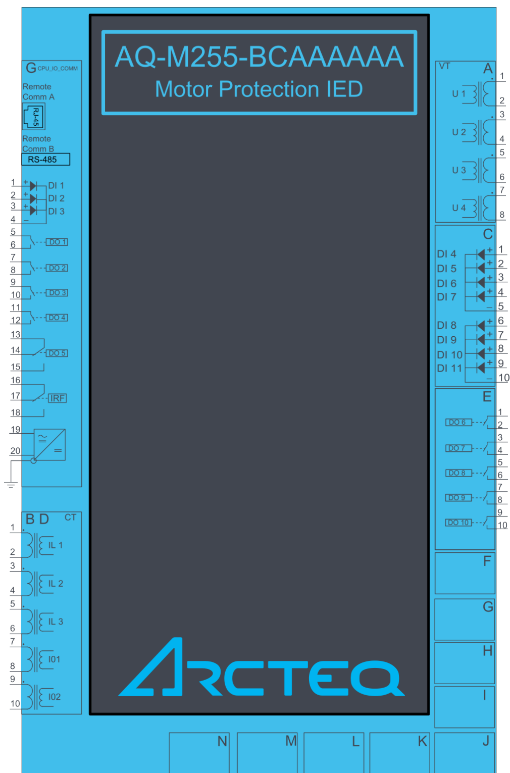
Figure. 7.1 - 182. AQ-M255 variant with digital input and output modules.
