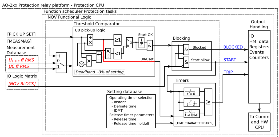
Figure. 5.4.12 - 81. Simplified function block diagram of the U0> function.
