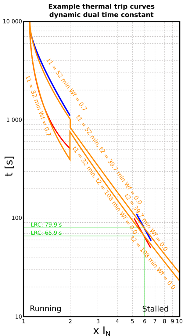
Figure. 5.4.23 - 126. Comparing dual time constant thermal replica tripping curves to given motor thermal characteristics.
