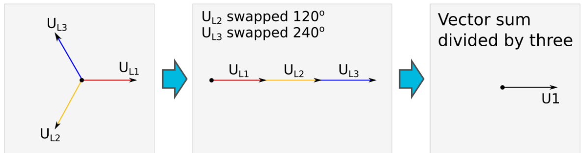
Figure. 5.4.13 - 83. Earth fault in an isolated network.
