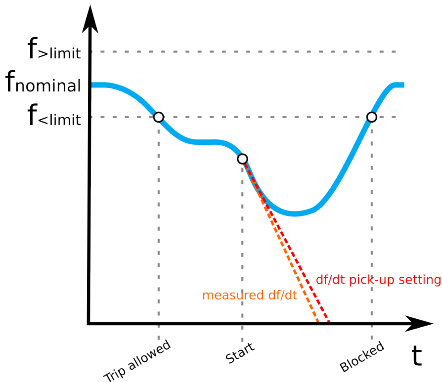
Figure. 5.4.15 - 92. Operation of the df/dt > / < function when the frequency starts but doesn't trip.
