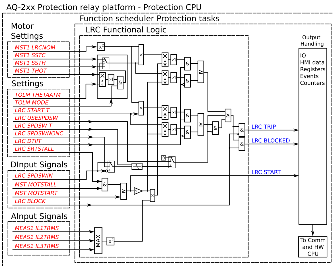
Figure. 5.4.18 - 101. Simplified function block diagram of the motor start/ locked rotor monitoring function.
