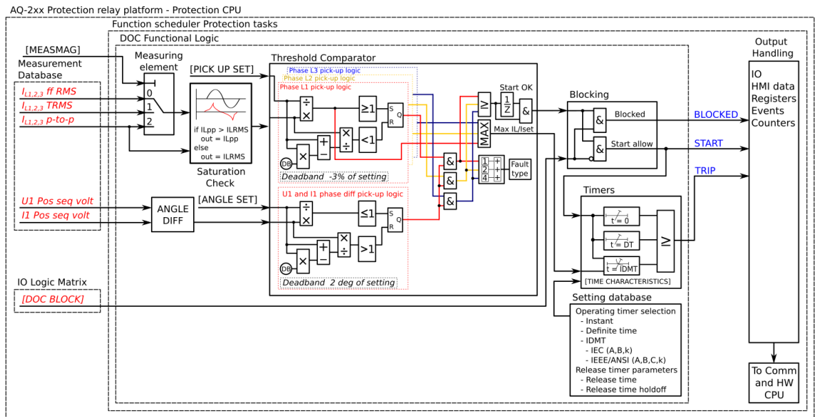
Figure. 5.4.4 - 36. Simplified function block diagram of the Idir> function.
