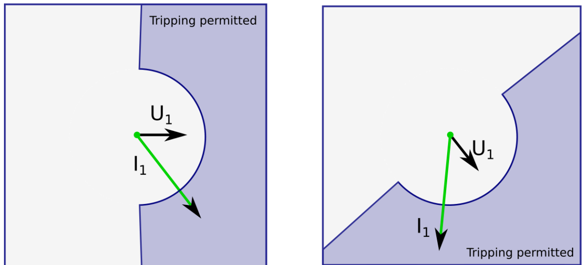
Figure. 5.4.4 - 37. Angle tracking of the I_{dir} function (3LN/3LL + U_0 mode).
