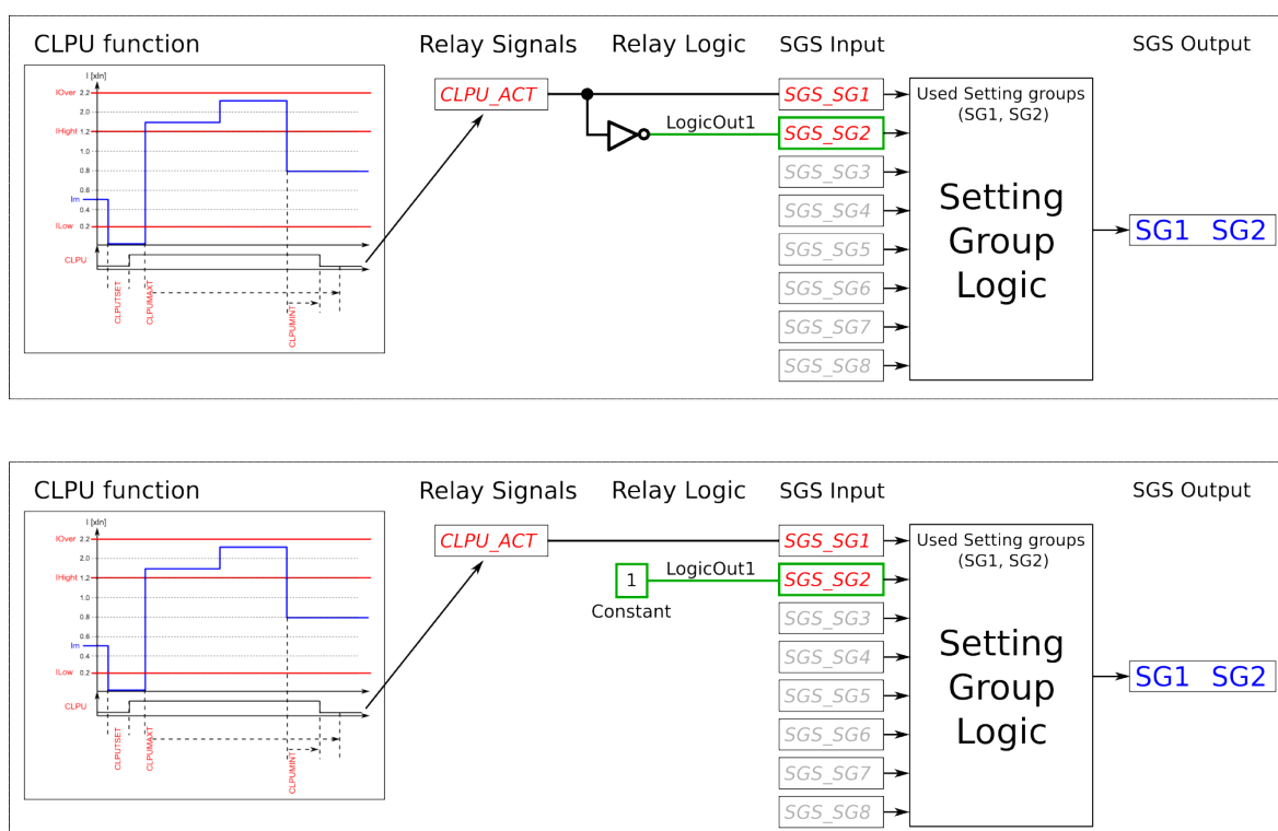
Figure. 5.5.2 - 151. Entirely application-controlled setting group change with the cold load pick-up function.
