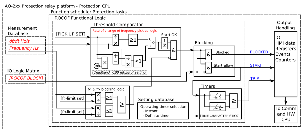
Figure. 5.4.15 - 93. Simplified function block diagram of the df/dt >/< function.
