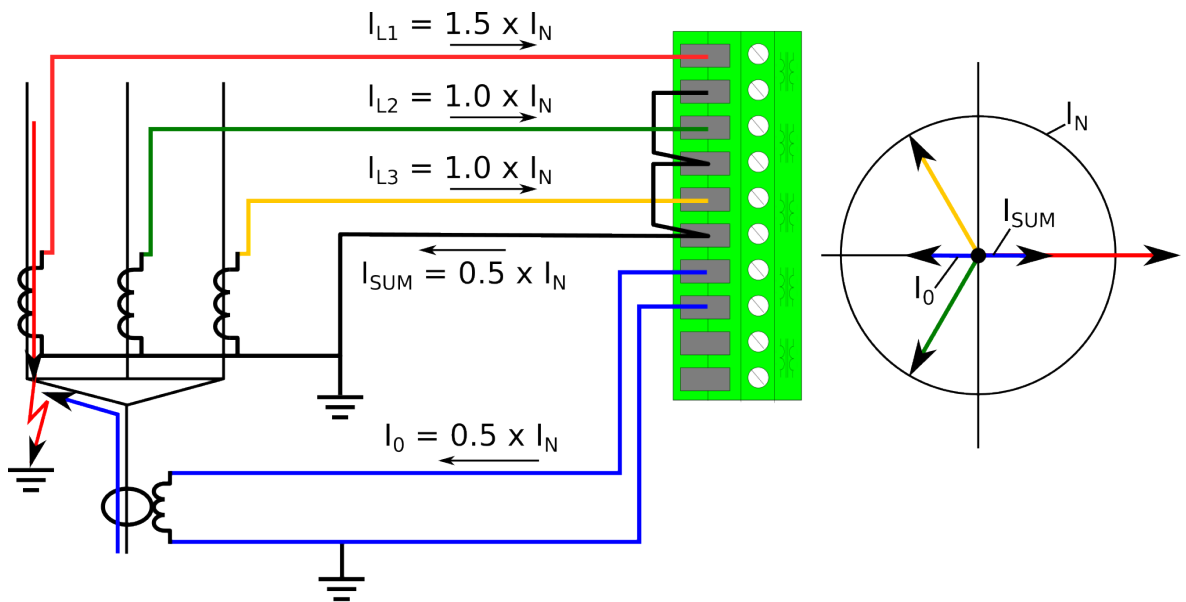
Figure. 5.4.11 - 126. Cable end differential when a fault occurs.
