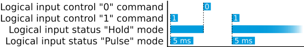
Figure. 5.5.13 - 220. Operation of logical input in "Hold" and "Pulse" modes.
