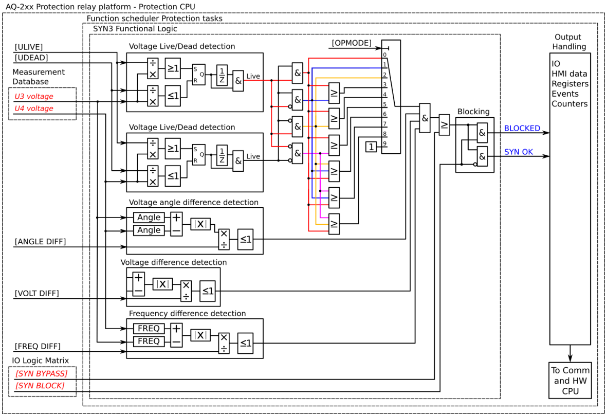
Figure. 5.5.9 - 218. Simplified function block diagram of the SYN3 function.
