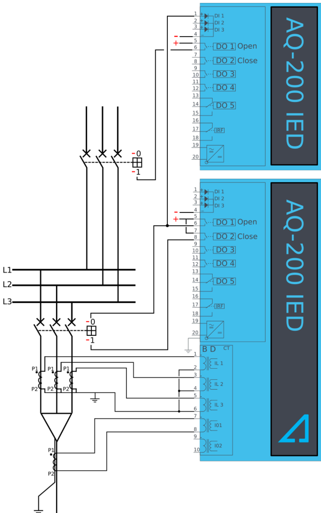
Figure. 5.4.10 - 118. Wiring diagram when the device is configured as a dedicated CBFP unit.
