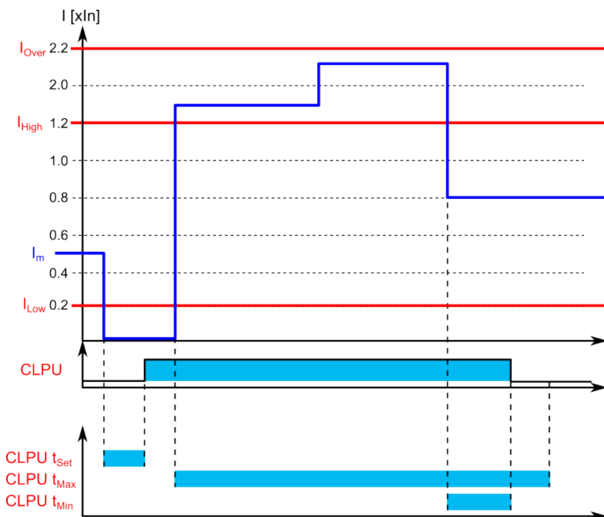
Figure. 5.5.7 - 202. Example of timers and pick-up parameters (normal CLPU situation).
