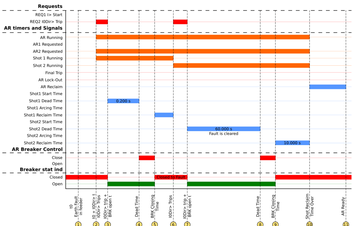
Figure. 5.5.5 - 188. Signal status graph of the semi-permanent earth fault auto-recloser cycle.
