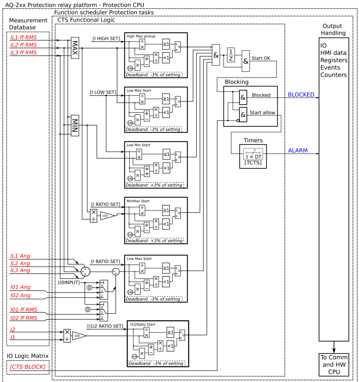
Figure. 5.6.1 - 223. Simplified function block diagram of the CTS function.
