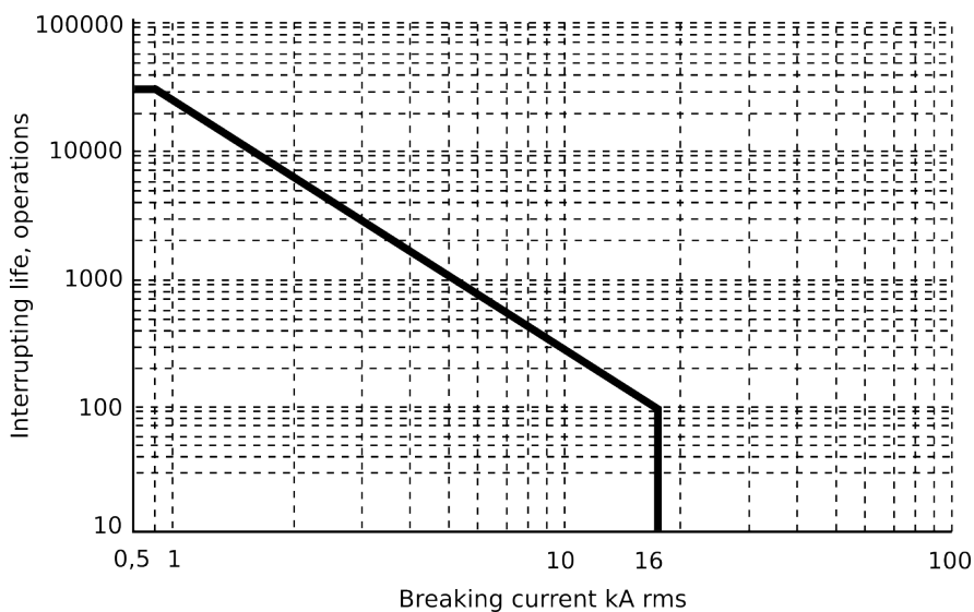
Figure. 5.6.3 - 235. Example of the circuit breaker interrupting life operations.
