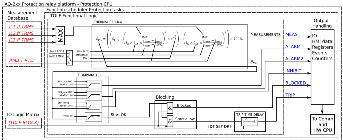
Figure. 5.4.21 - 173. Simplified function block diagram of the TF> function.
