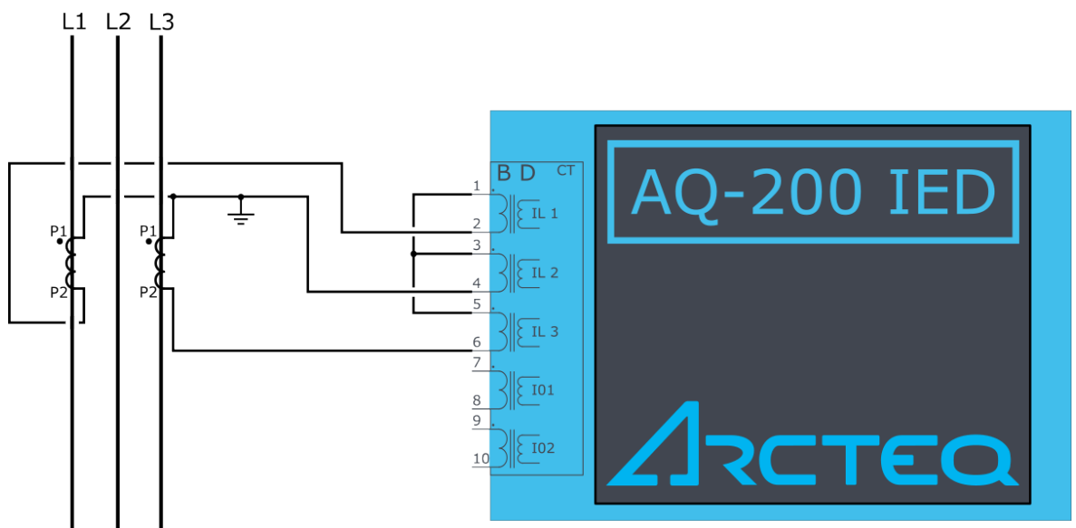
Figure. 7.2 - 246. ARON connection.
