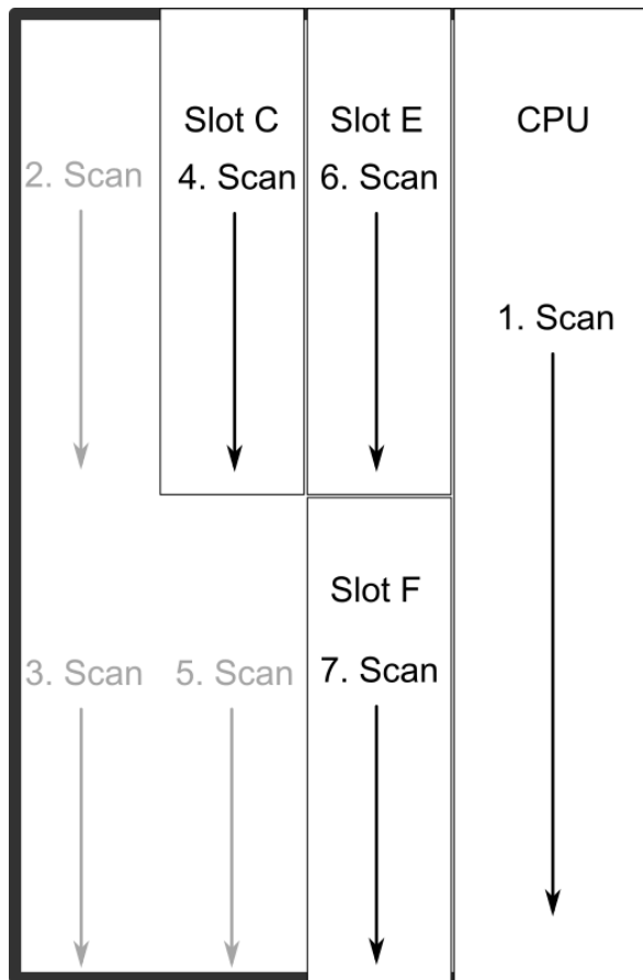
Figure. 8.1 - 248. AQ-X215 hardware scanning and I/O naming principles.
