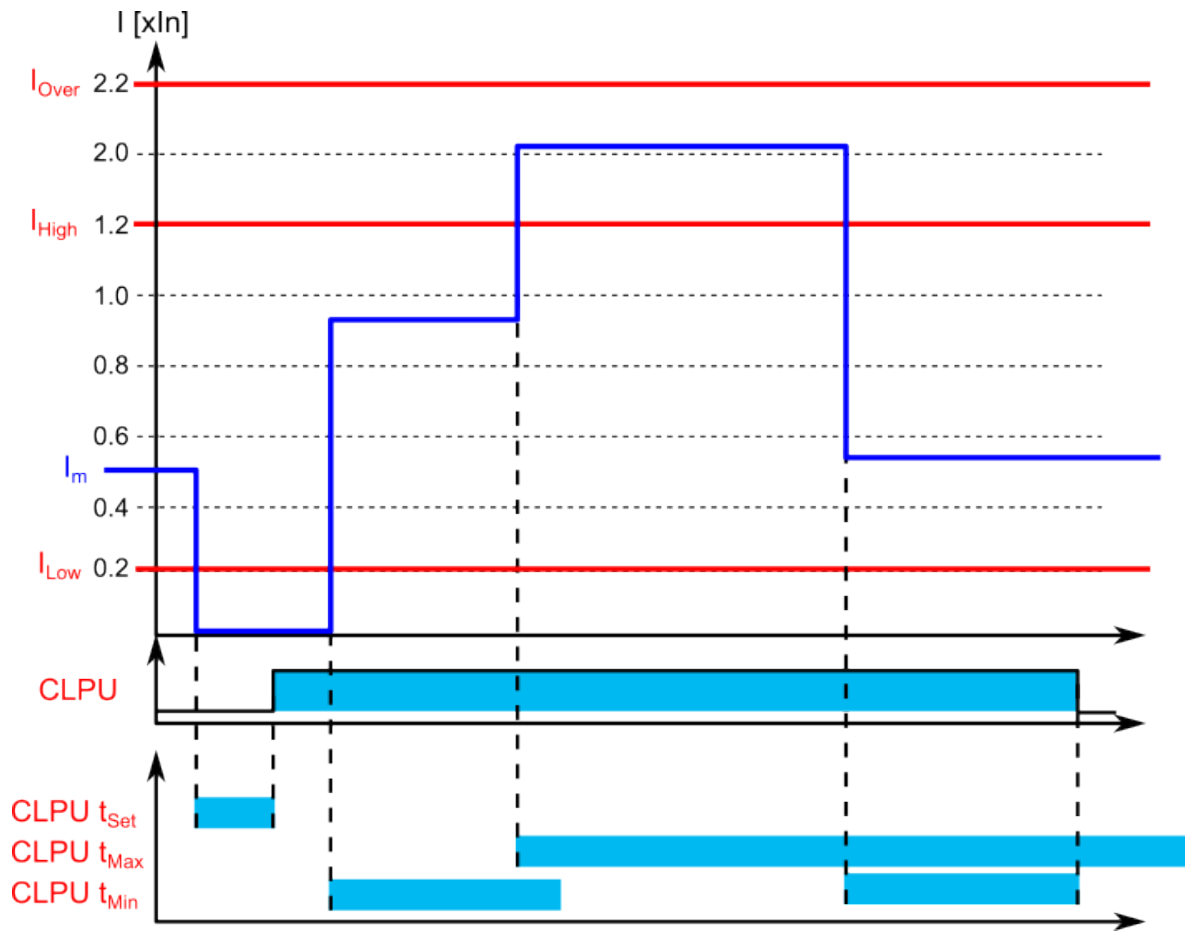
Figure. 5.5.7 - 207. Example of timers and pick-up parameters (an inrush current detected during T_{min} time).
