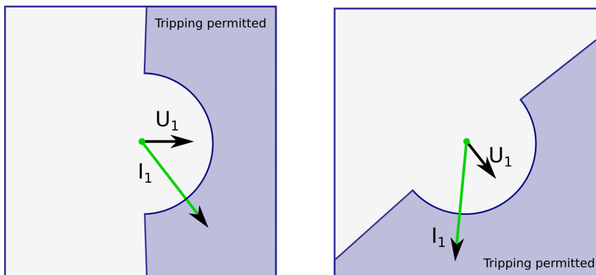
Figure. 5.4.5 - 93. Angle tracking of the I_{dir} function (3LN/3LL + U_0 mode).
