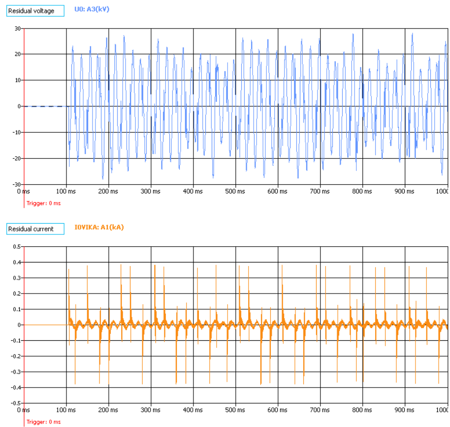
Figure. 5.4.7 - 104. An intermittent earth fault in an undercompensated medium size network, as seen by a faulty feeder relay.
