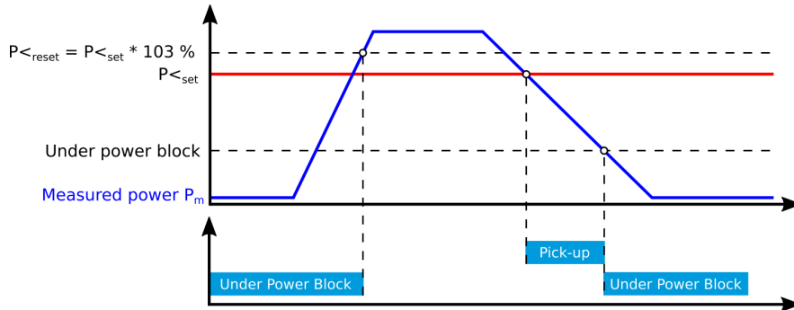
Figure. 5.4.19 - 158. Activation and deactivation characteristics of low power blocking.
