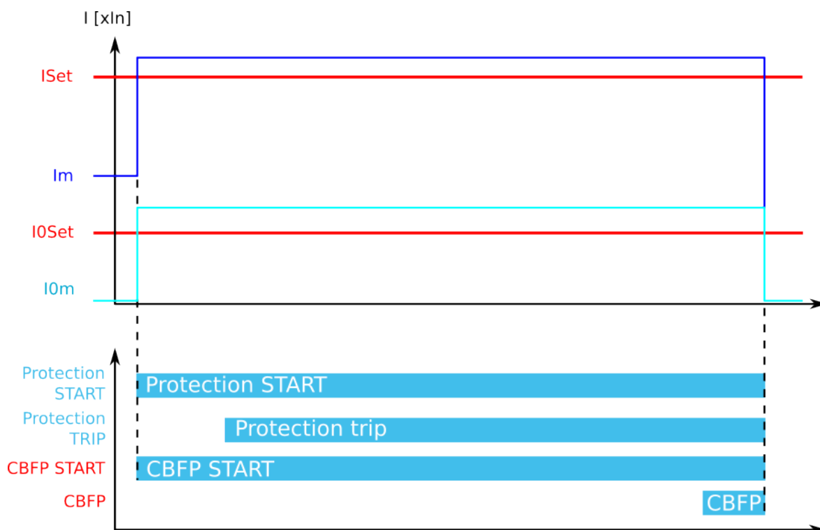
Figure. 5.4.10 - 115. CBFP when "Current" is the selected criterion.
