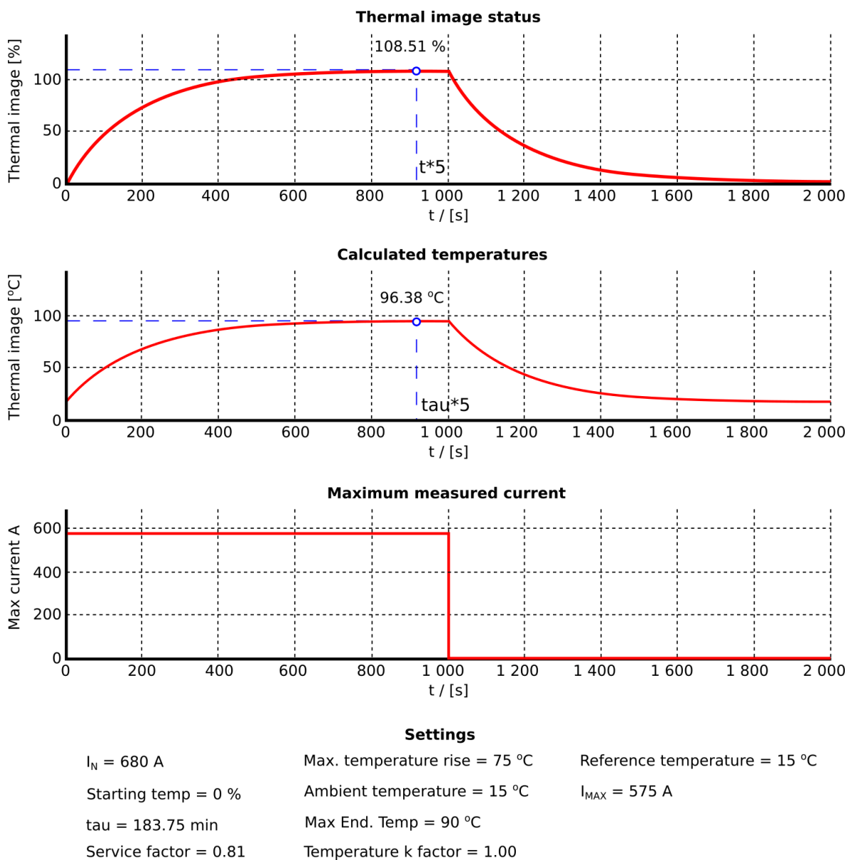
Figure. 5.4.21 - 171. Thermal image response with nominal currents and fine-tuned k_{\text{SF}} correction factor.
