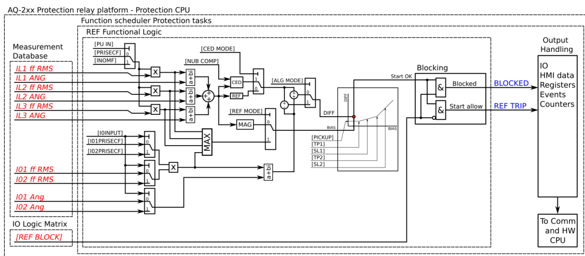
Figure. 5.4.11 - 120. Simplified function block diagram of the I0d> function.
