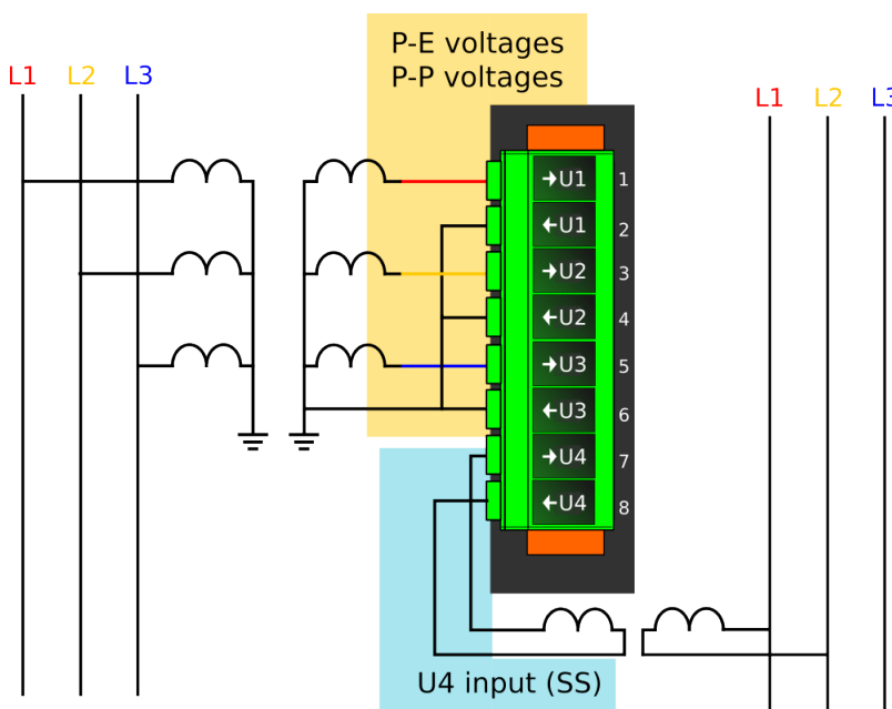
Figure. 5.4.12 - 131. Selectable measurement magnitudes with 3LL+U4 VT connection (P-E voltages not available without residual voltage).
