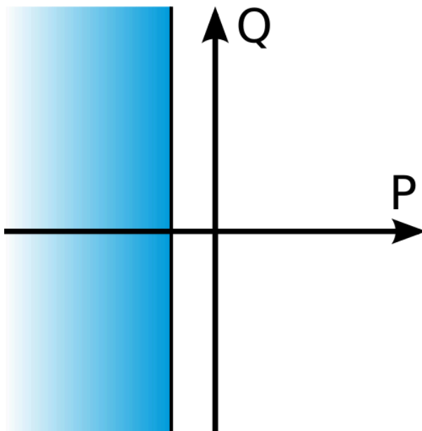
Figure. 5.4.20 - 159. Operating characteristics of reverse power protection.
