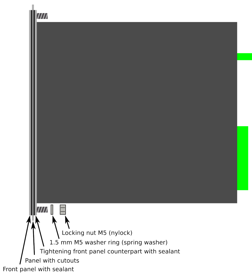
Figure. 8.14 - 267. Device installation.
