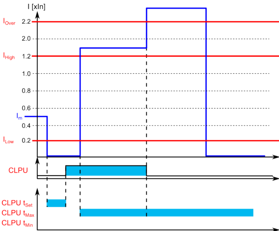
Figure. 5.5.7 - 204. Example of timers and pick-up parameters (activated pick-up and instant release due to overcurrent).
