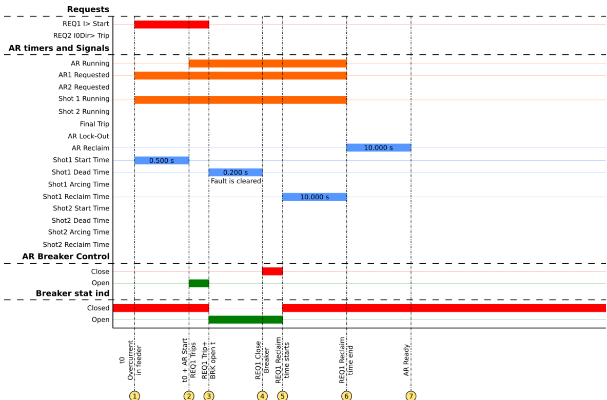
Figure. 5.5.5 - 196. Signal status graph of the transient overcurrent auto-recloser cycle.
