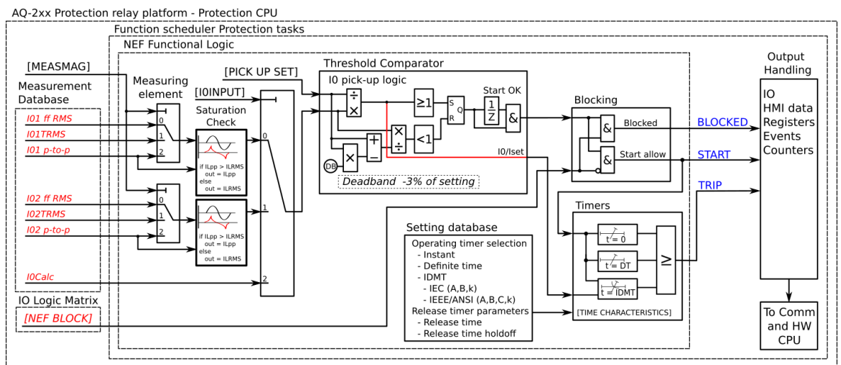
Figure. 5.4.4 - 91. Simplified function block diagram of the I0> function.
