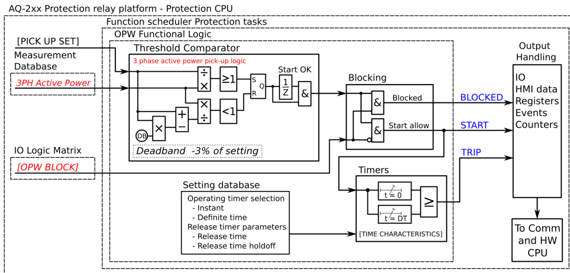
Figure. 5.4.18 - 155. Simplified function block diagram of the P > function.
