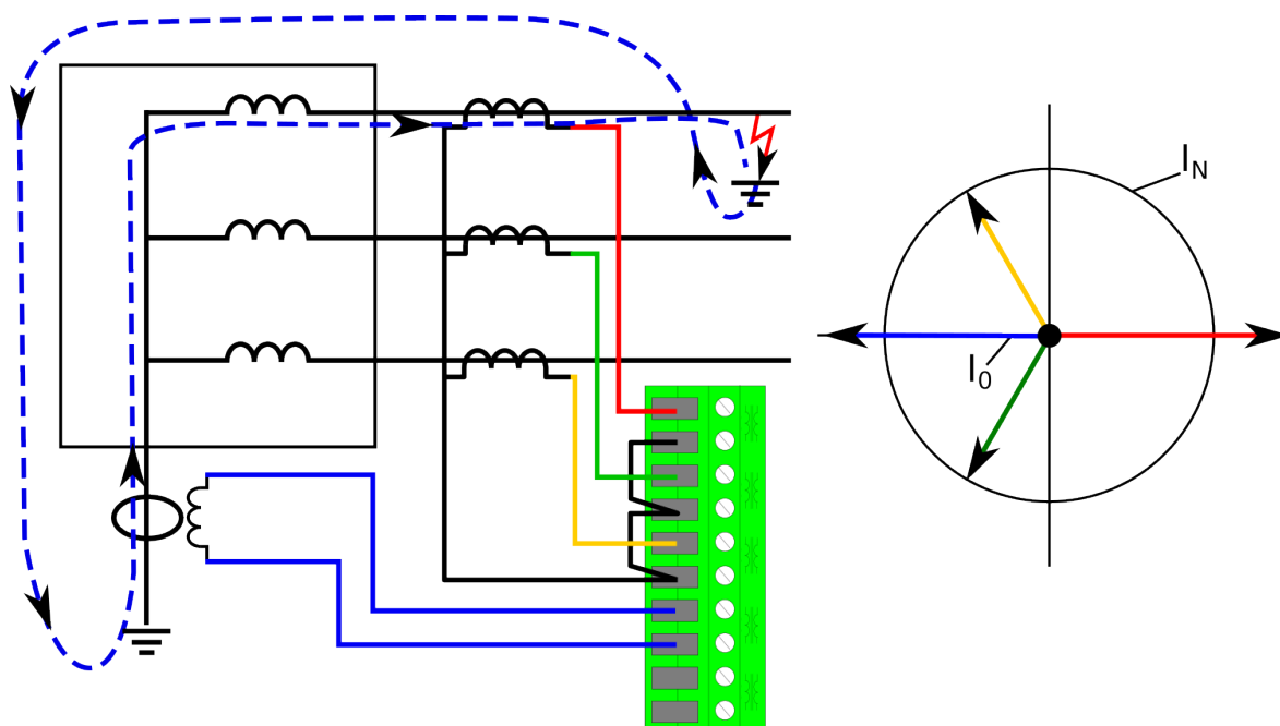
Figure. 5.4.11 - 127. Restricted earth fault outside a Y winding transformer.
