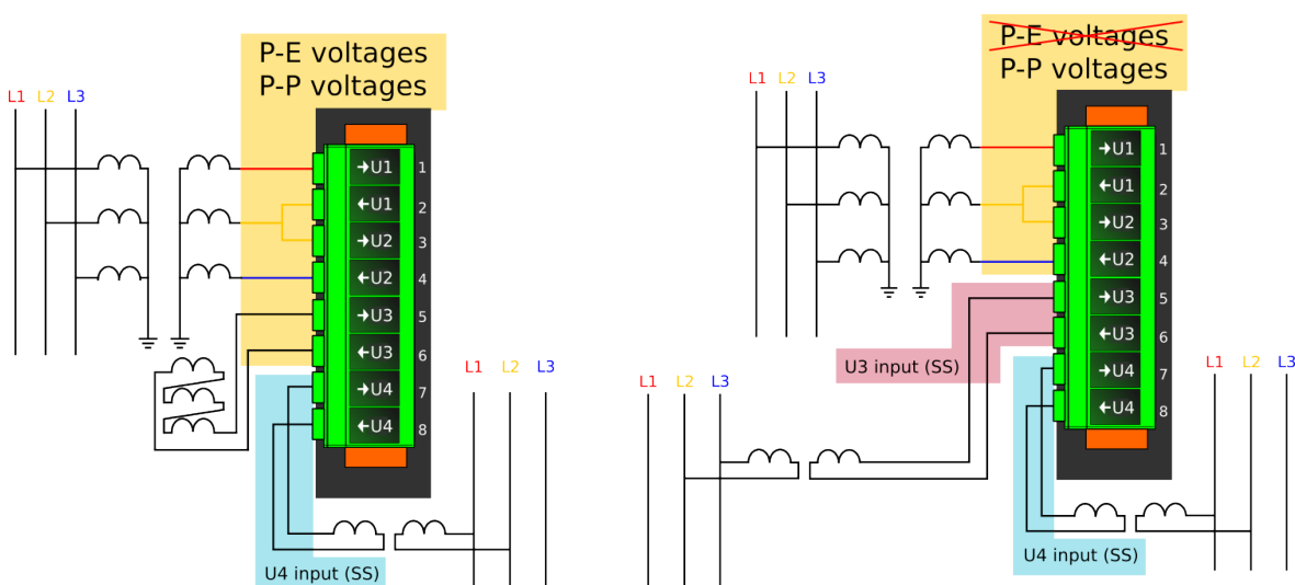
Figure. 5.4.13 - 136. Selectable measurement magnitudes with 2LL+U4 VT connection (P-E voltages not available without residual voltage).
