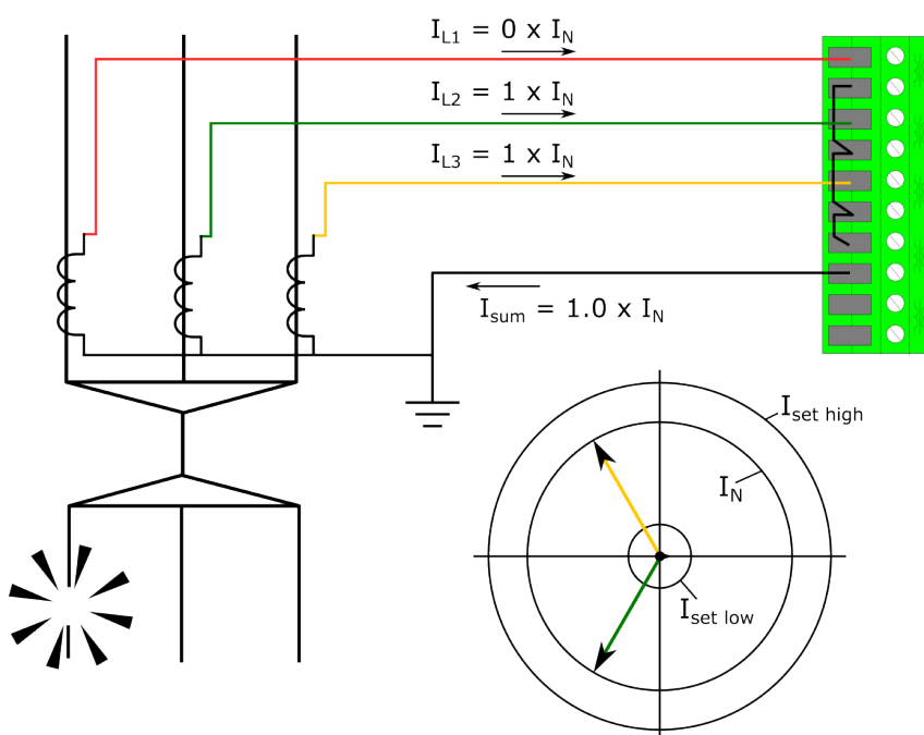
Figure. 5.6.1 - 226. Primary circuit fault in phase L1 wiring.
