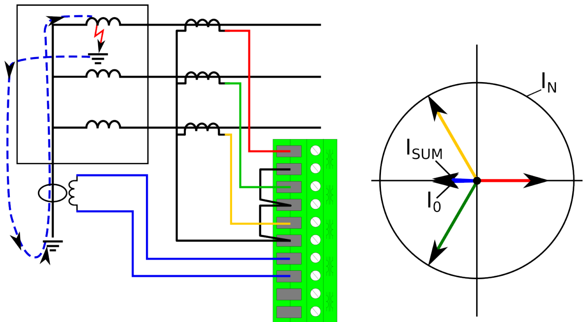
Figure. 5.4.11 - 128. Restricted earth fault inside a Y winding transformer.
