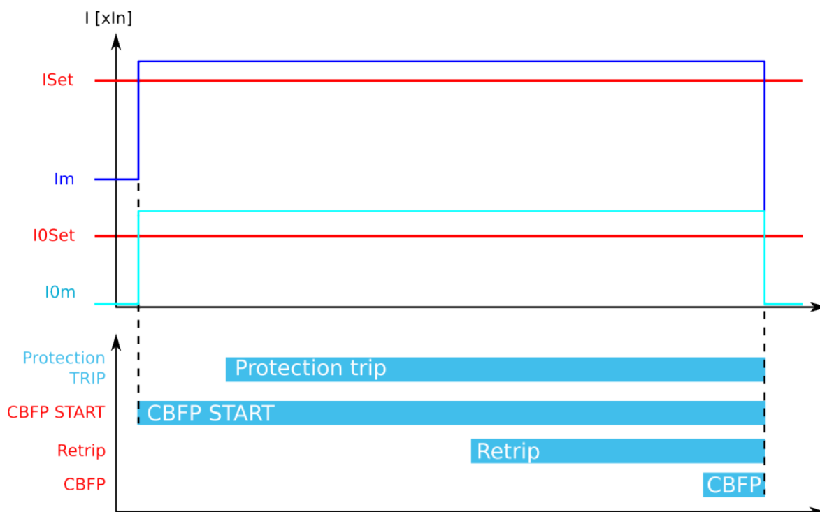
Figure. 5.4.10 - 111. Retrip and CBFP when "Current" is the selected criterion.
