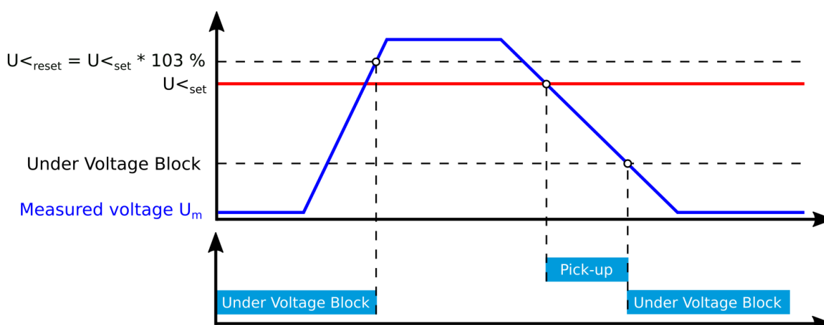
Figure. 5.4.15 - 149. Example of the block setting operation.
