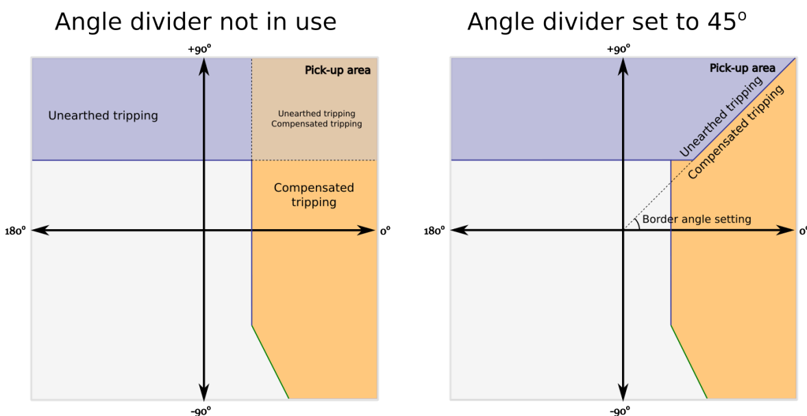
Figure. 5.4.6 - 101. Effect of angle divider when in use and when disabled.
