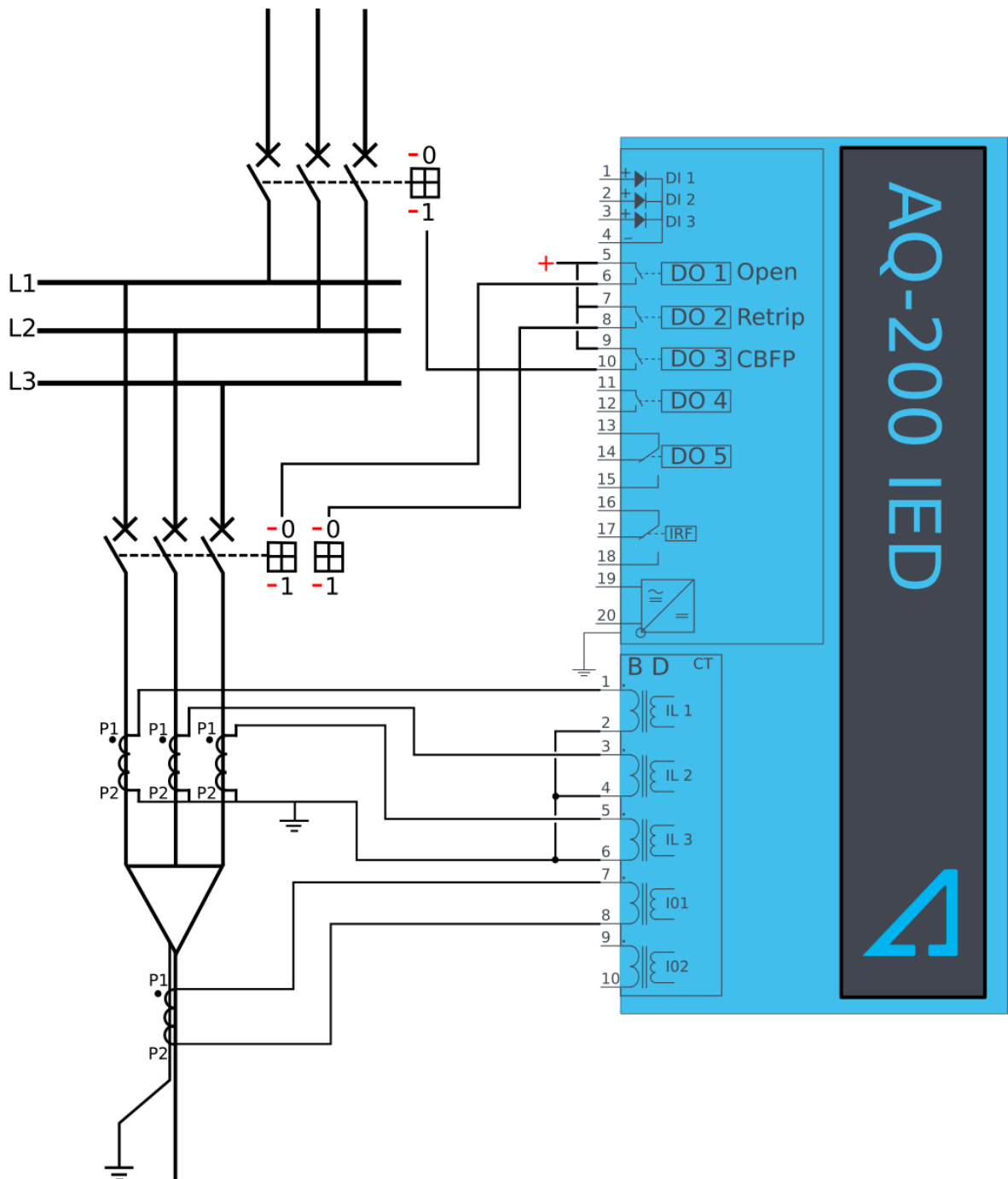
Figure. 5.4.10 - 110. Wiring diagram when Trip, Retrip and CBFP are configured to the device.
