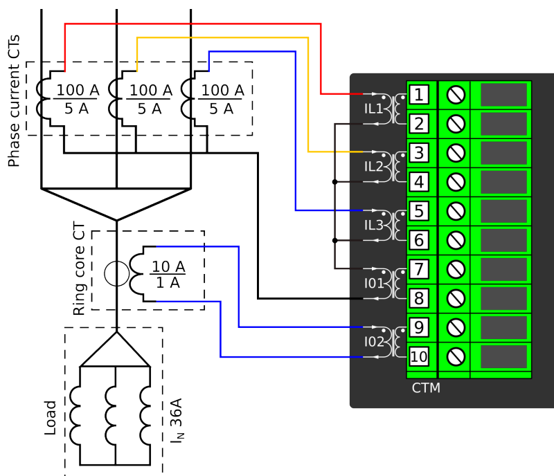
Figure. 5.2.1 - 56. Connections.
