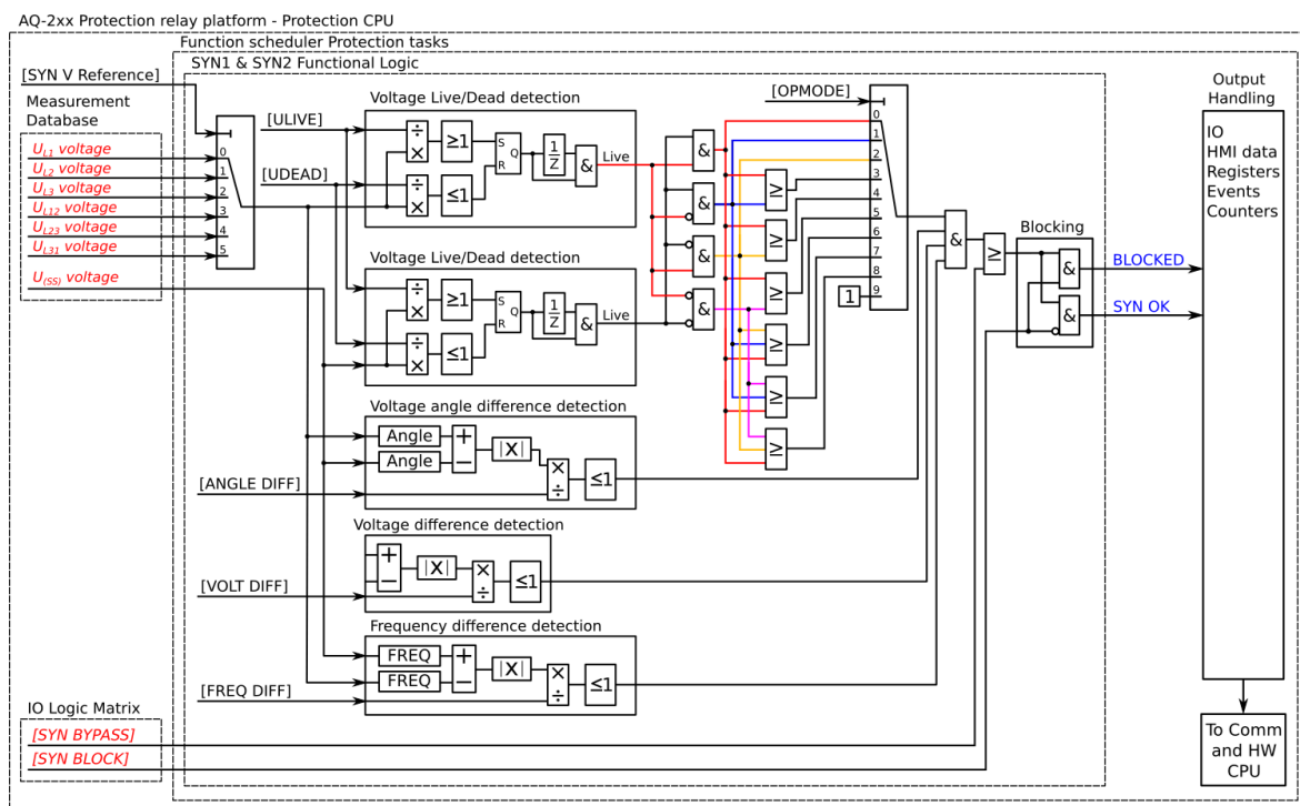
Figure. 5.5.9 - 217. Simplified function block diagram of the SYN1 and SYN2 function.
