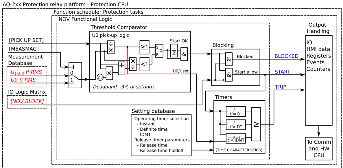
Figure. 5.4.14 - 141. Simplified function block diagram of the U0> function.
