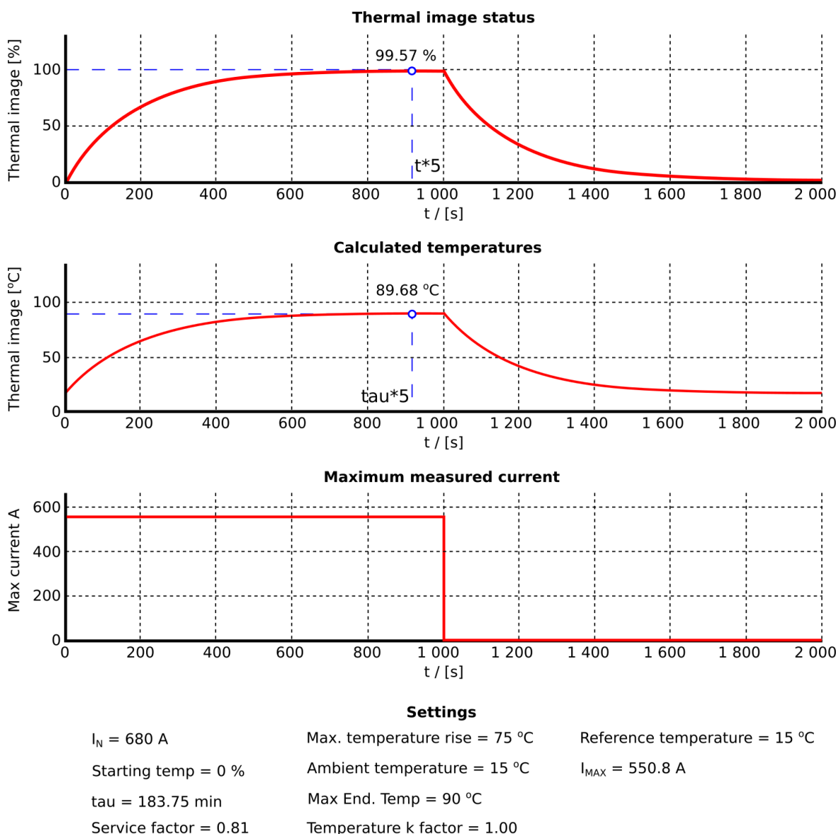
Figure. 5.4.21 - 172. Thermal response with k SF factor correctly set.
