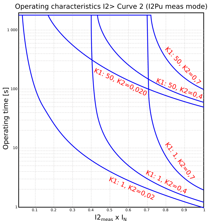
Figure. 5.4.8 - 107. Operation characteristics curve for I2> Curve2.
