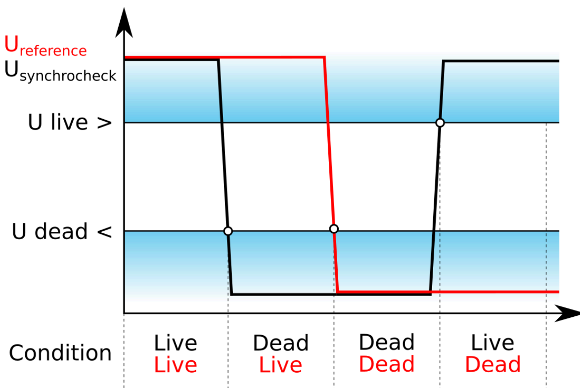
Figure. 5.5.9 - 216. System states.
