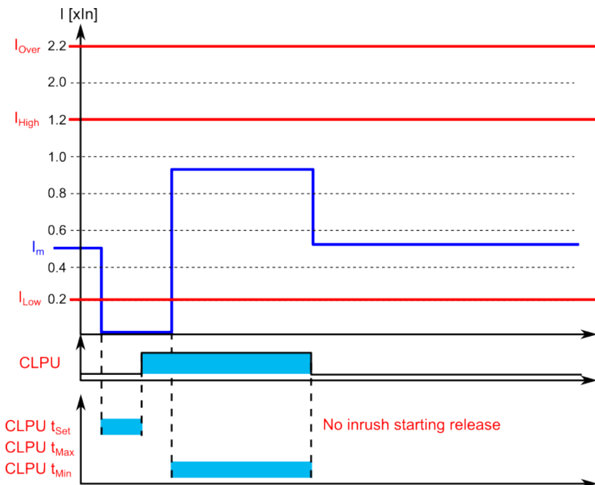
Figure. 5.5.7 - 206. Example of timers and pick-up parameters (no inrush current detected in the starting).
