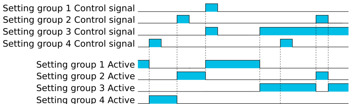
Figure. 5.5.2 - 175. Example sequences of group changing (control with pulse only, or with both pulses and static signals).
