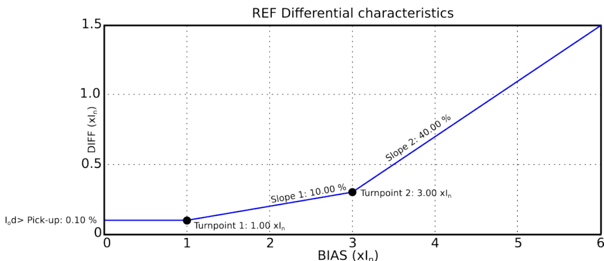
Figure. 5.4.11 - 121. Differential characteristics for the I0d> function with default settings.
