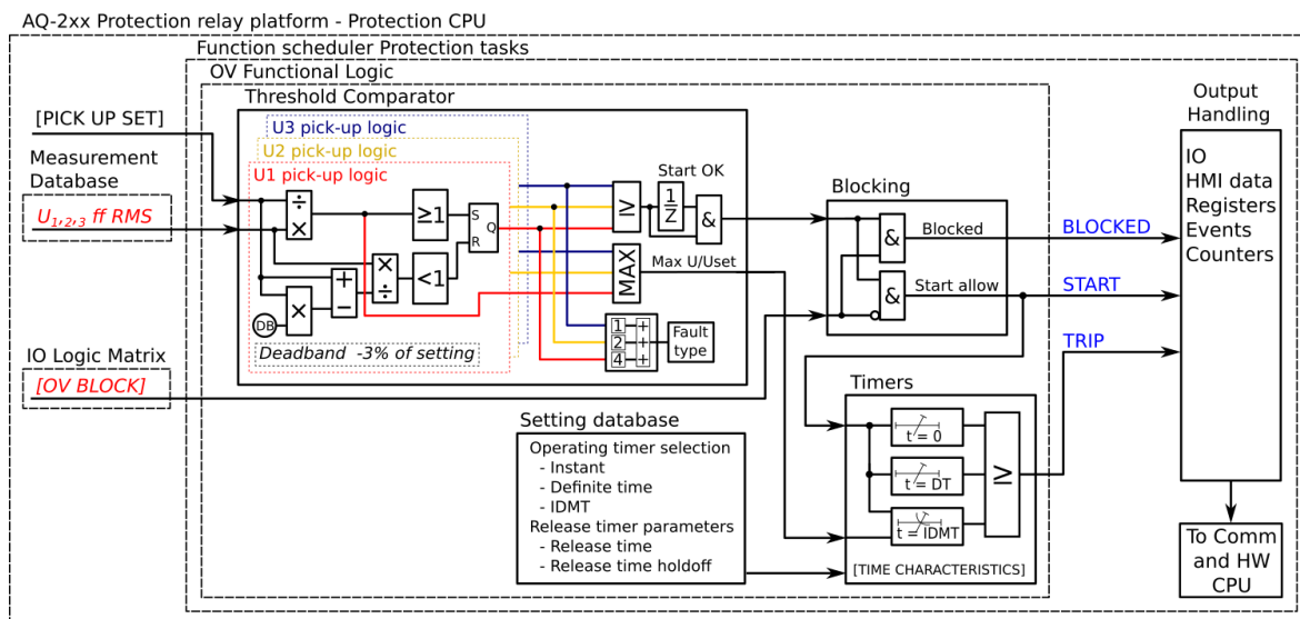
Figure. 5.4.12 - 129. Simplified function block diagram of the U> function.
