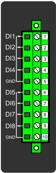
Figure. 8.5 - 252. Digital input module (DI8) with eight add-on digital inputs.
