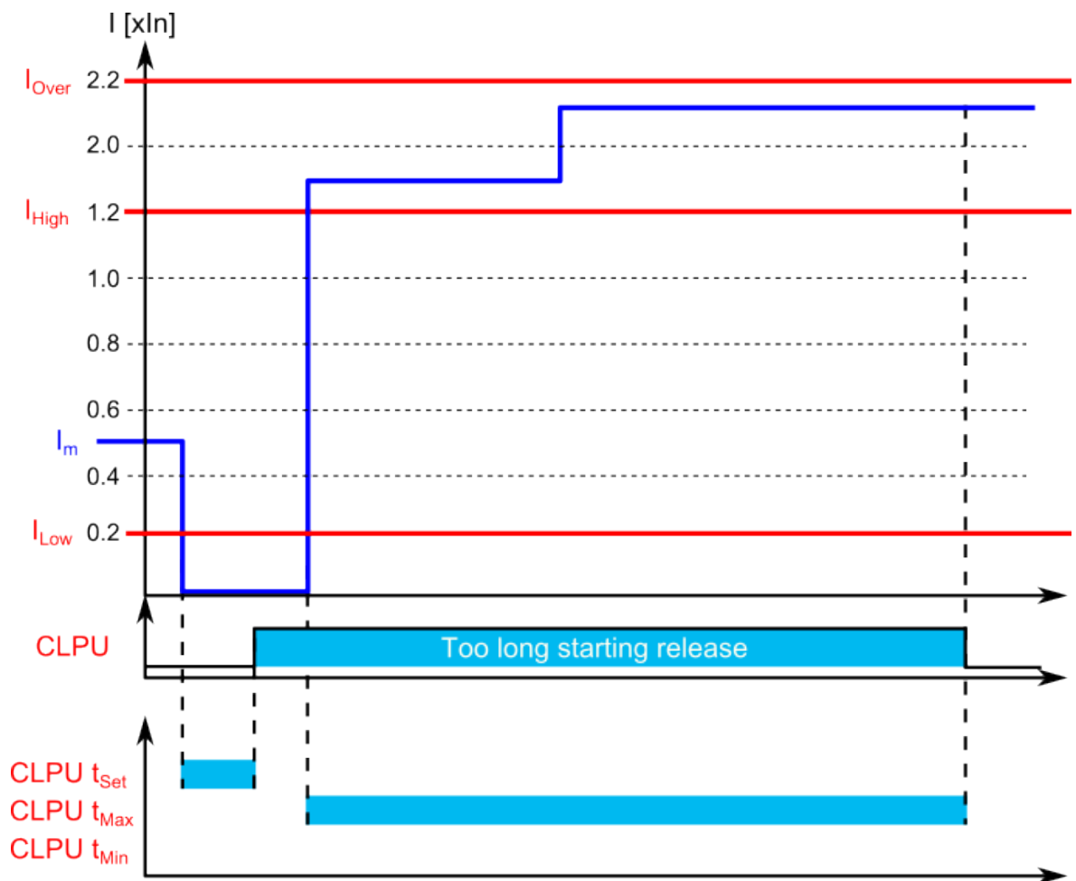
Figure. 5.5.7 - 205. Example of timers and pick-up parameters (activated pick-up and instant release due to too long starting).
