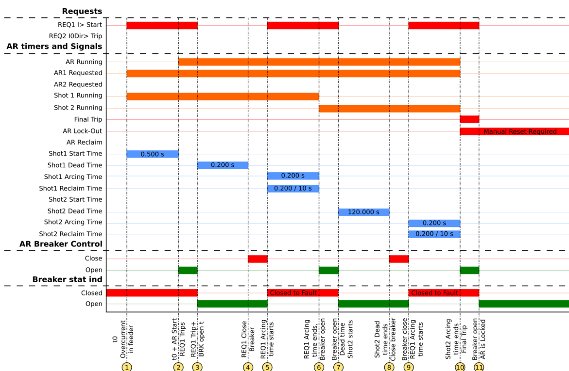
Figure. 5.5.5 - 192. Signal status graph of the permanent overcurrent auto-recloser cycle.
