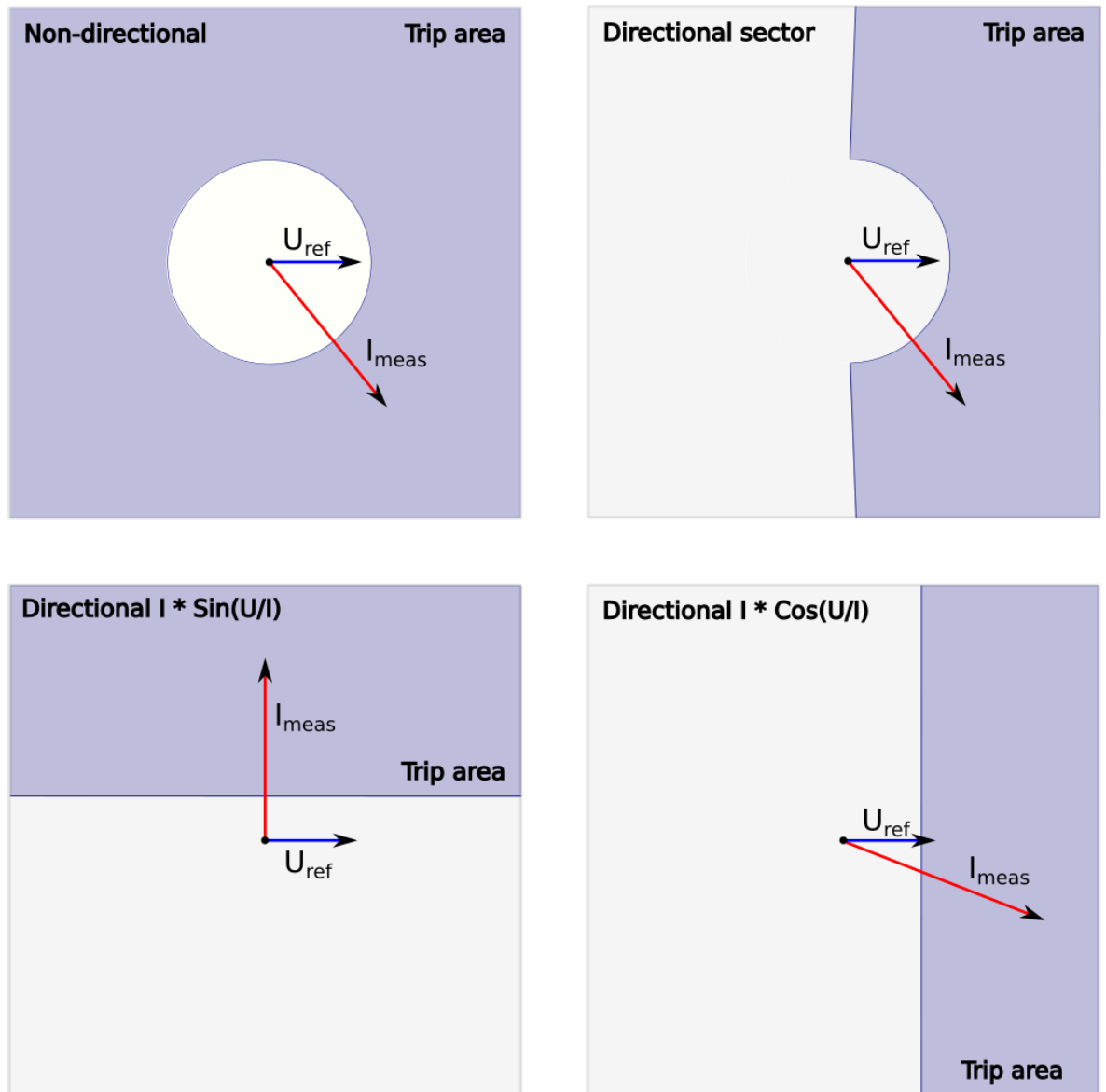
Figure. 5.4.2.2 - 87. Angle tracking of I_{dir} and the four available operating modes. U_{ref} is the chosen channel for reference angle and I_{meas} is the chosen current measurement channel.
