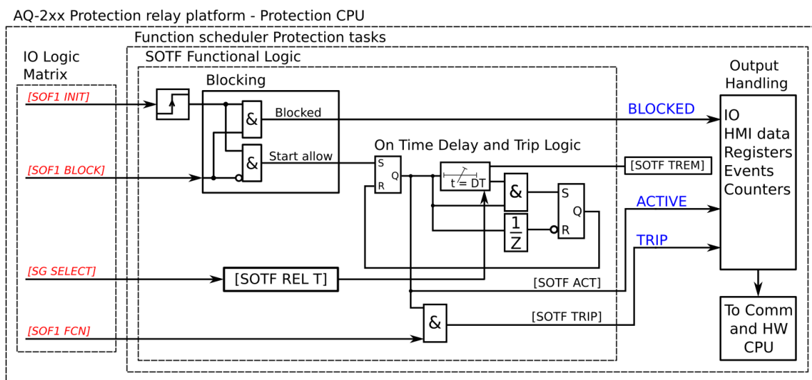
Figure. 5.5.8 - 208. Simplified function block diagram of the switch-on-to-fault function.
