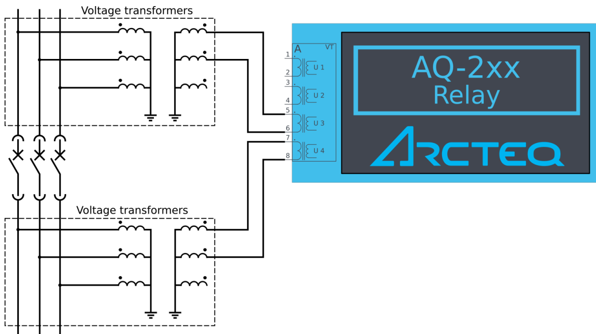
Figure. 5.5.9 - 211. Example connection of the synchrocheck function (2LL+U3+U4 mode, SYN3 in use, UL12 as reference voltage).
