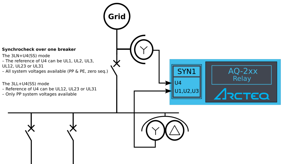
Figure. 5.5.9 - 213. Example application (synchrocheck over one breaker, with 2LL VT connection).
