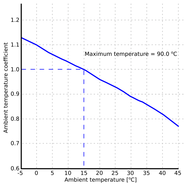
Figure. 5.4.21 - 165. Set correction curve for ambient temperature.
