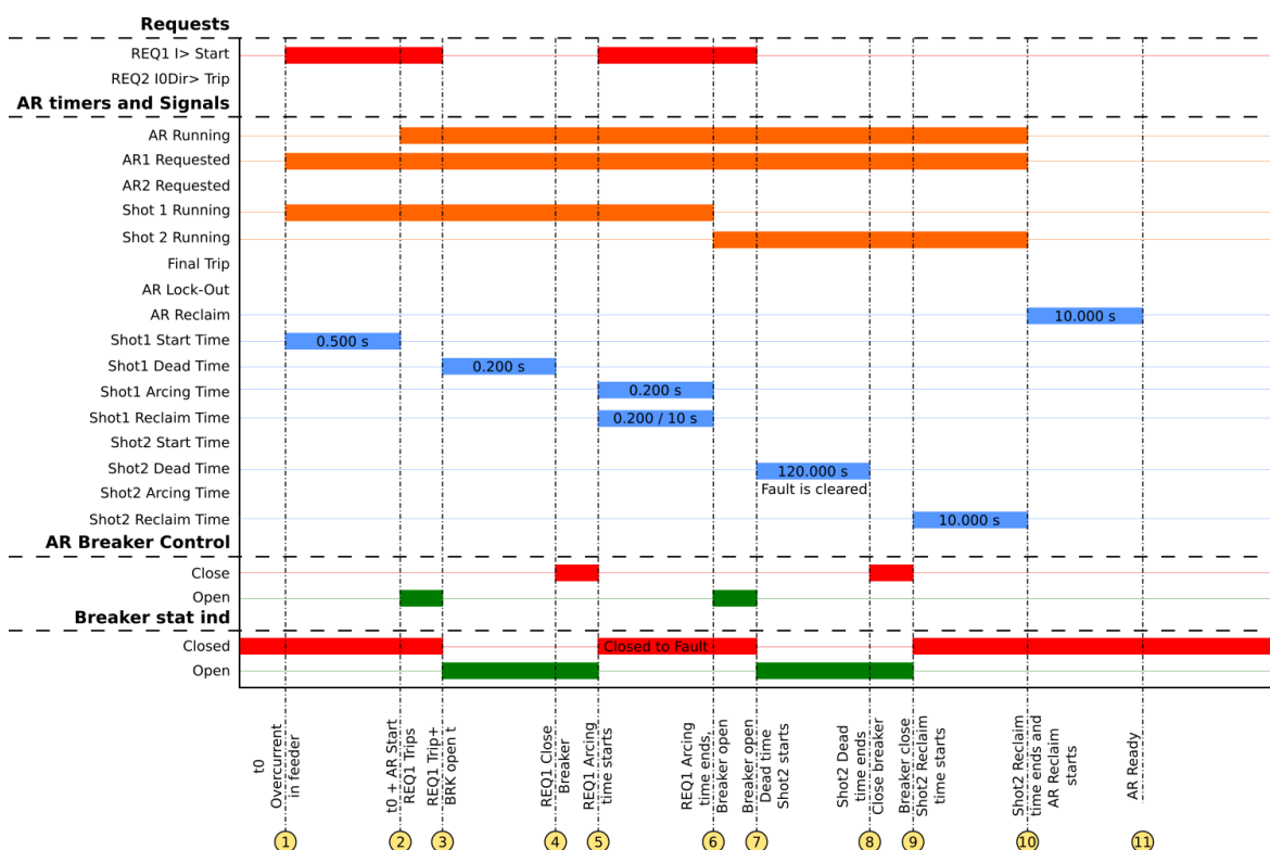
Figure. 5.5.5 - 194. Signal status graph of the semi-permanent overcurrent auto-recloser cycle.
