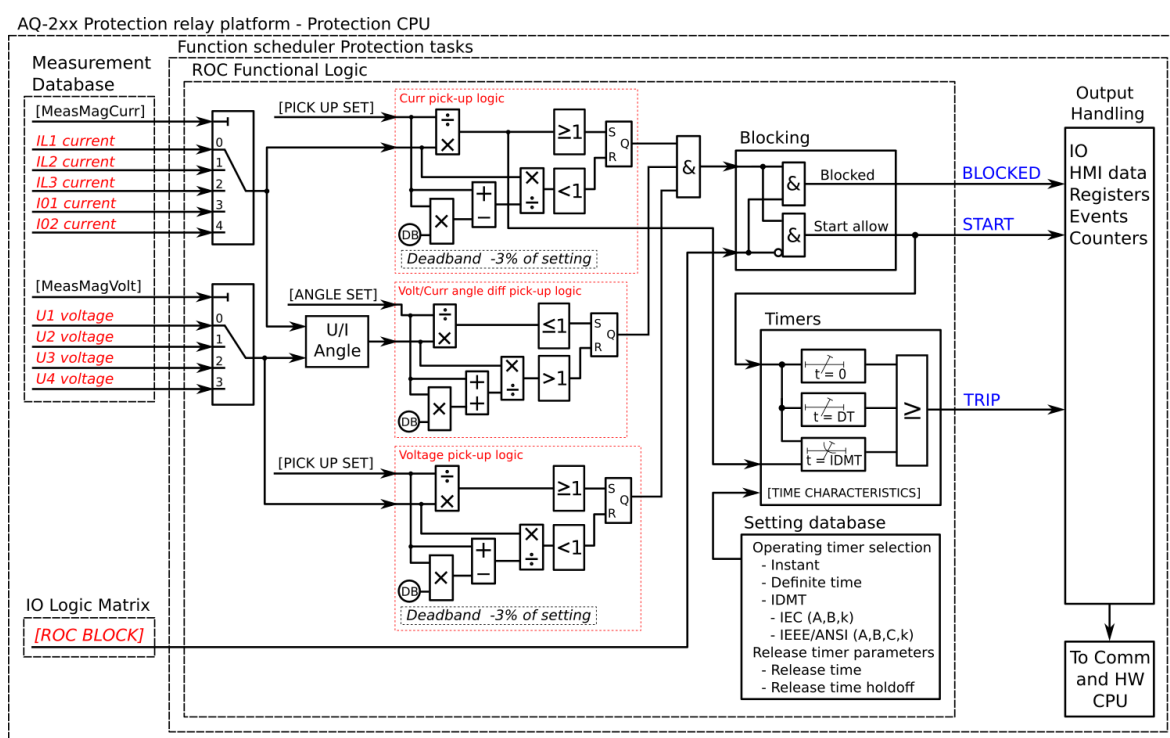
Figure. 5.4.2.2 - 86. Simplified function block diagram of the Idrw> function.
