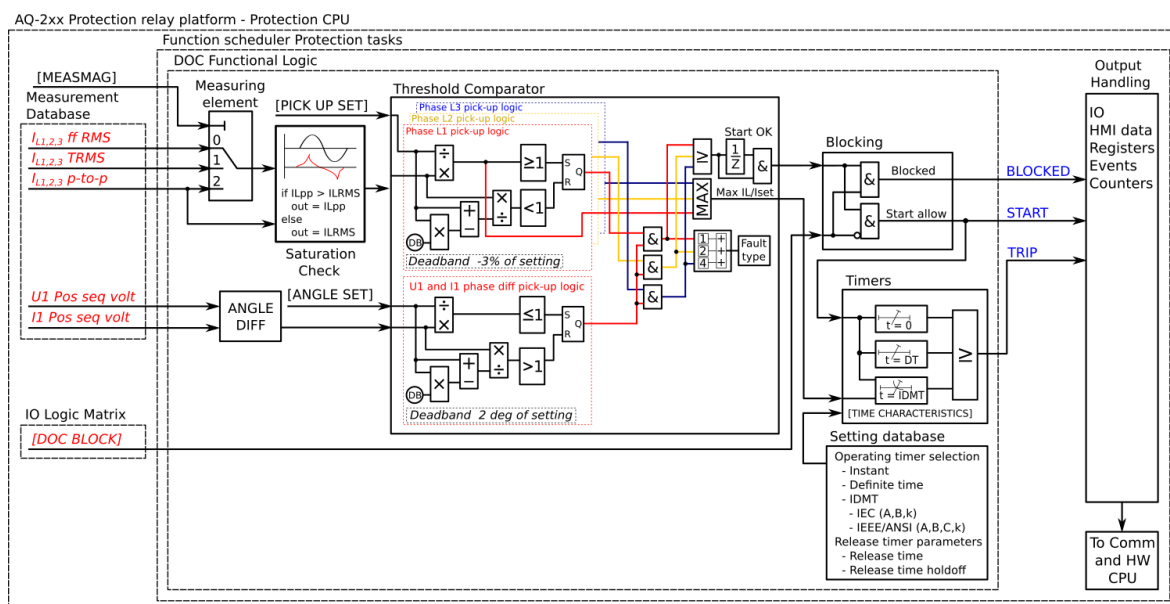
Figure. 5.4.5 - 92. Simplified function block diagram of the Idir> function.
