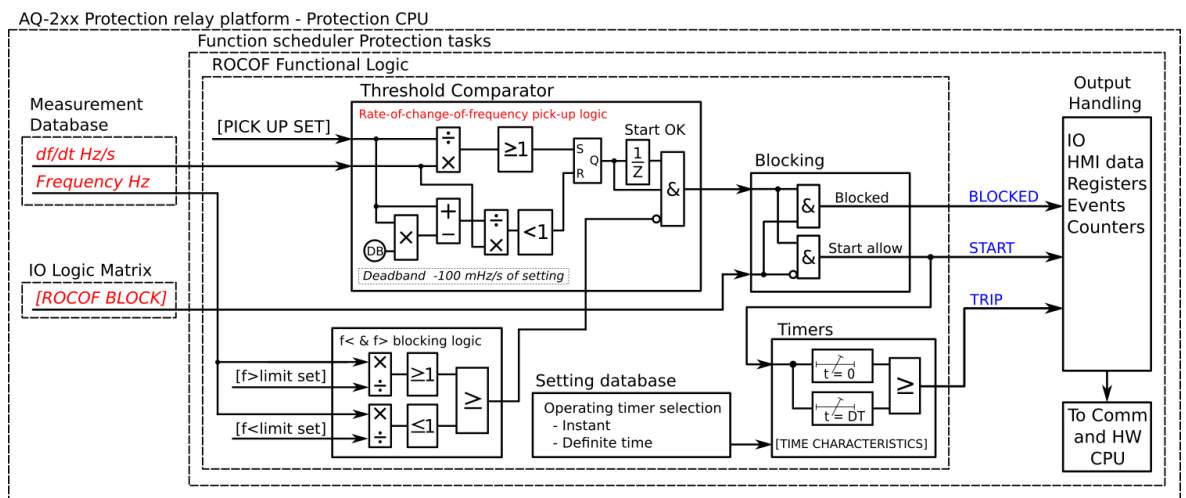
Figure. 5.4.17 - 153. Simplified function block diagram of the df/dt > / < function.
