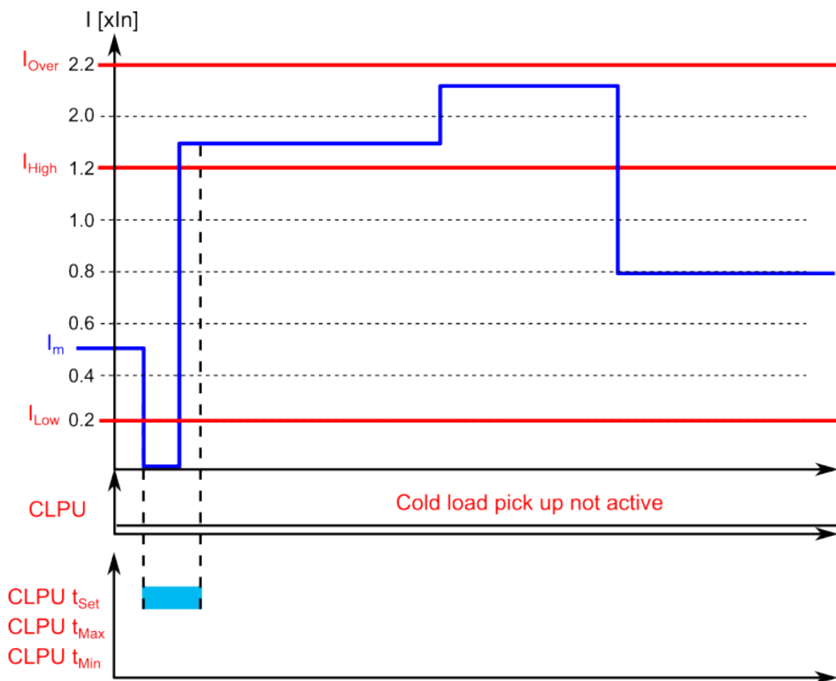
Figure. 5.5.7 - 203. Example of timers and pick-up parameters (no cold load pick-up, I_{low} too short).
