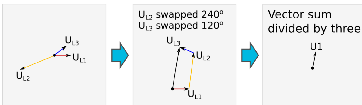
Figure. 5.4.15 - 147. Close-distance short-circuit between phases 1 and 3.
