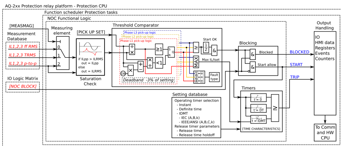
Figure. 5.4.3 - 90. Simplified function block diagram of the I> function.
