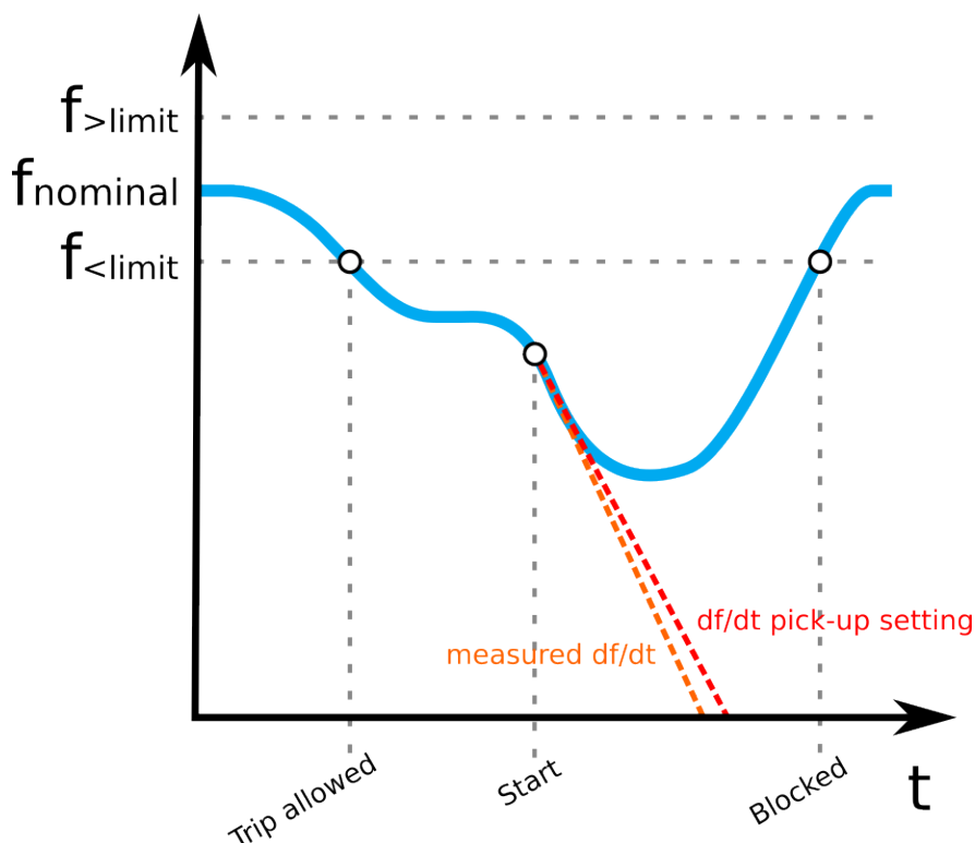
Figure. 5.4.17 - 152. Operation of the df/dt > / < function when the frequency starts but doesn't trip.
