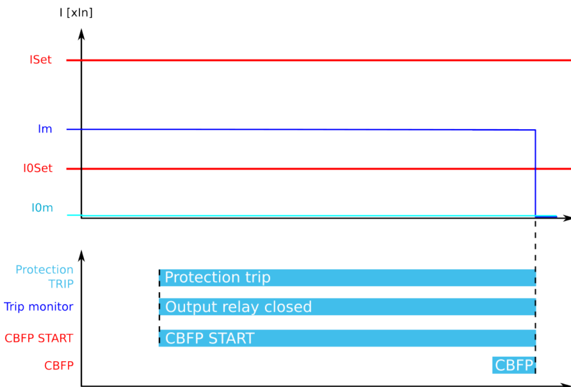
Figure. 5.4.10 - 117. CBFP when "Current or DO" is the selected criterion.
