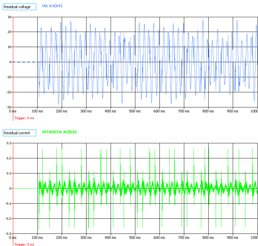
Figure. 5.4.7 - 105. Undercompensated medium size network intermittent earth fault seen by healthy feeder relay.
