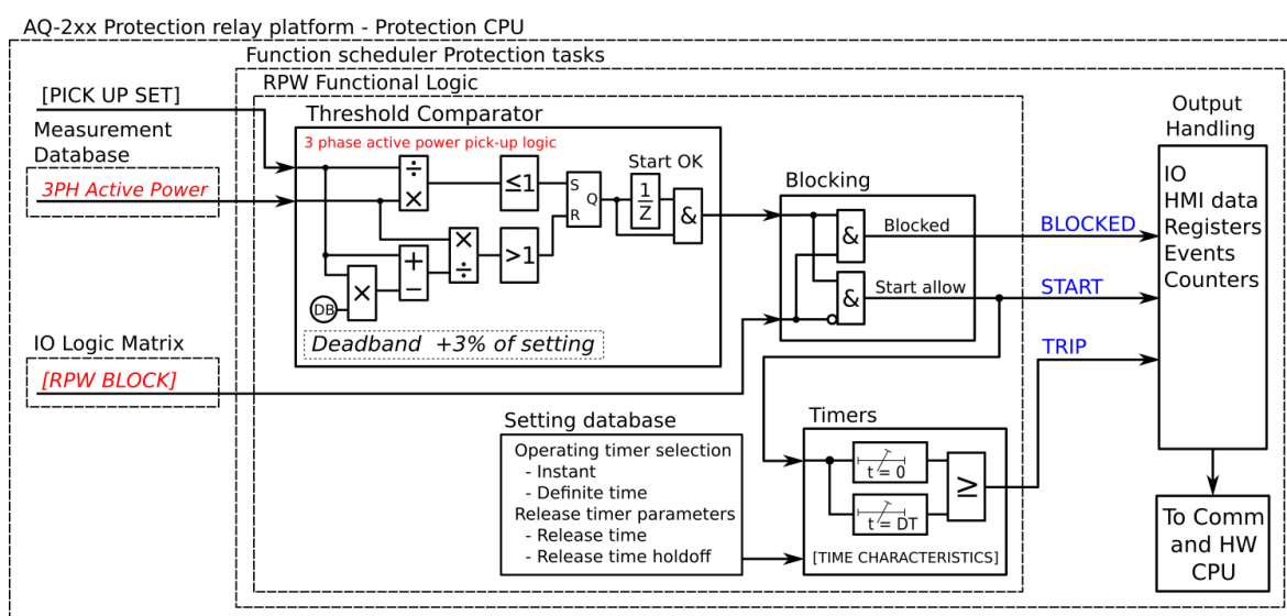
Figure. 5.4.20 - 160. Simplified function block diagram of the Pr function.
