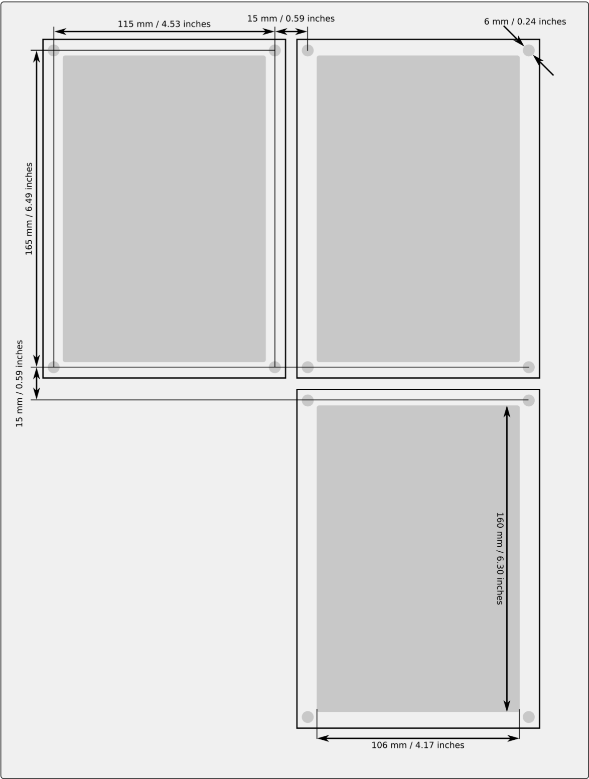
Figure. 8.14 - 268. Panel cutout dimensions and device spacing.
