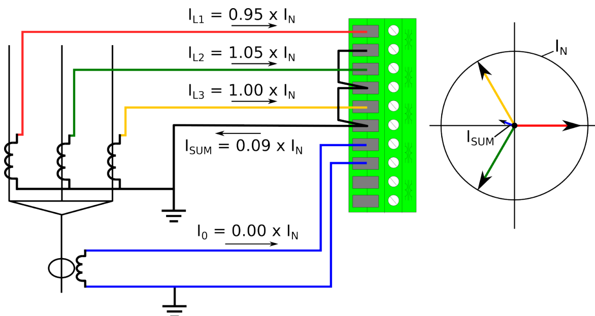
Figure. 5.4.11 - 125. Cable end differential with natural unbalance in the phase current measurement.
