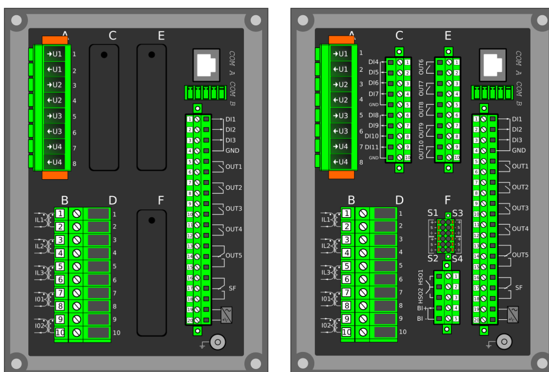
Figure. 8.1 - 247. Modular construction of AQ-X215.
