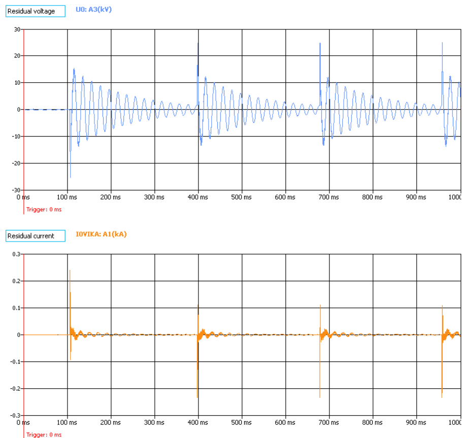
Figure. 5.4.7 - 102. An intermittent earth fault in a medium size network tuned close to resonance, as seen by a faulty feeder relay.
