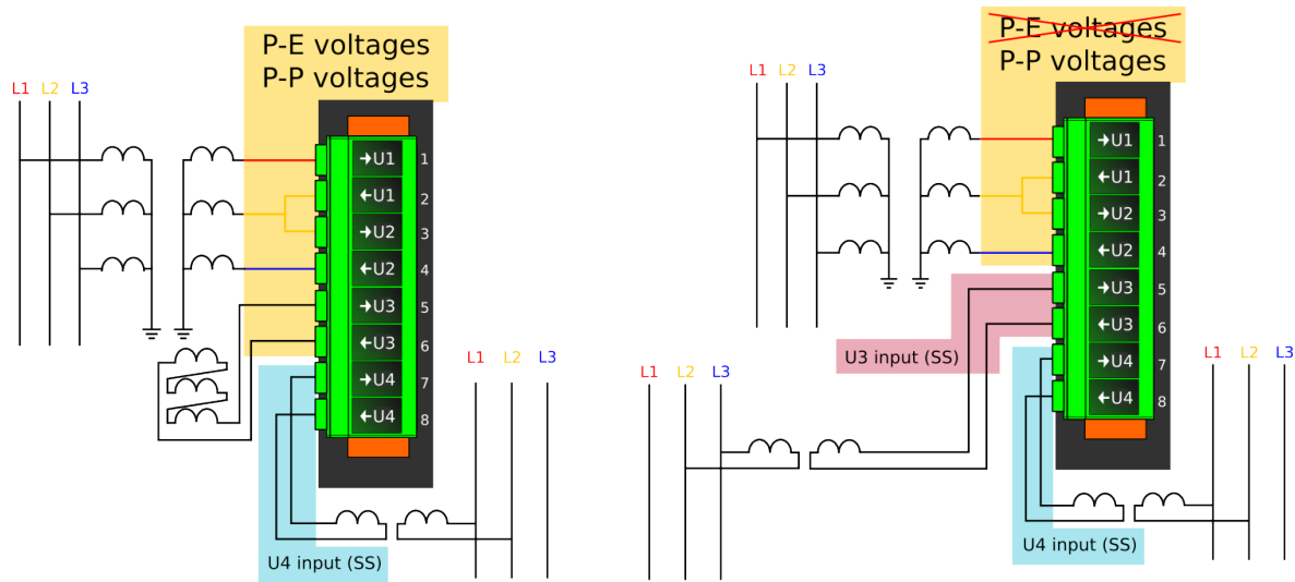
Figure. 5.4.12 - 132. Selectable measurement magnitudes with 2LL+U3+U4 VT connection (P-E voltages not available without residual voltage).
