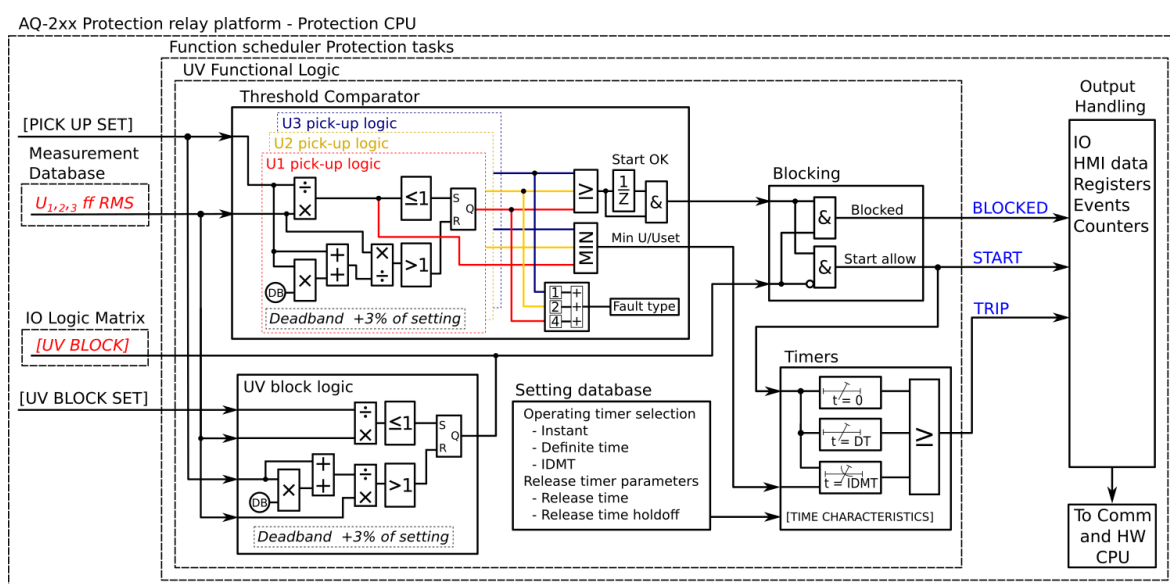
Figure. 5.4.13 - 133. Simplified function block diagram of the U< function.
