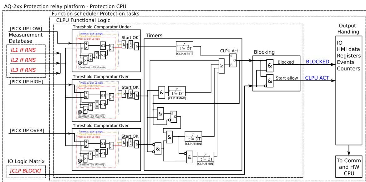
Figure. 5.5.7 - 201. Simplified function block diagram of the cold load pick-up function.
