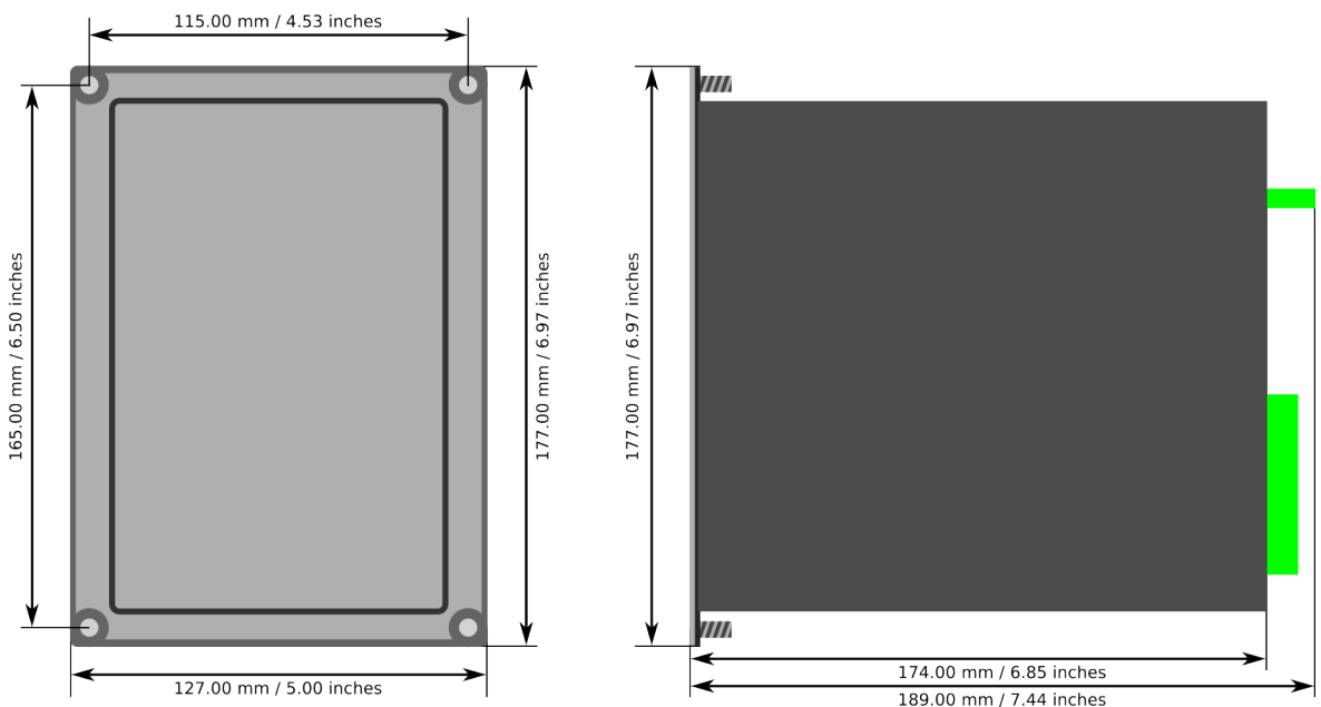
Figure. 8.14 - 266. Device dimensions.
