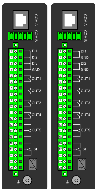
Figure. 8.2 - 249. CPU module.
