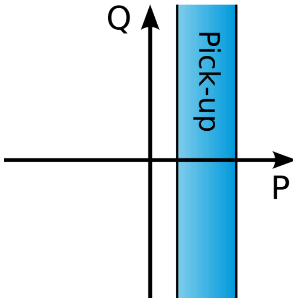
Figure. 5.4.19 - 156. Operating characteristics of underpower protection.
