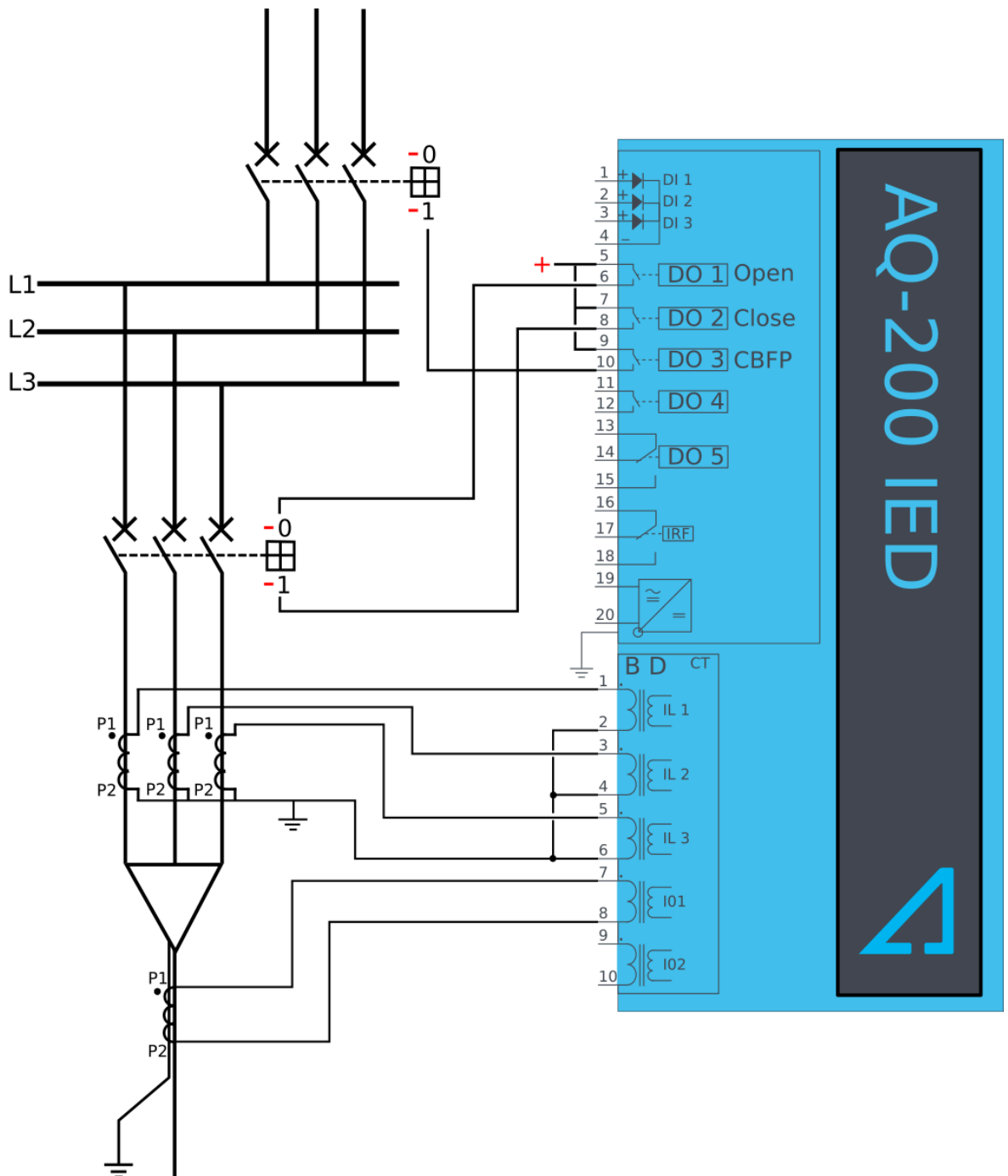
Figure. 5.4.10 - 114. Wiring diagram when Trip and CBFP are configured to the device.
