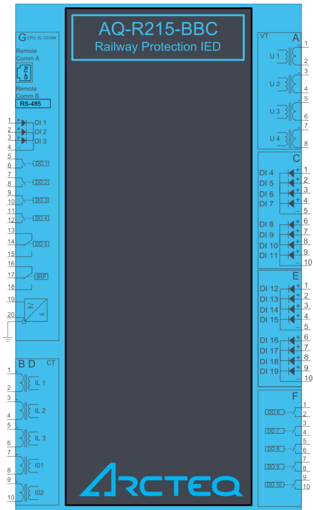
Figure. 7.1 - 244. AQ-R215 variant with digital input and output modules.
