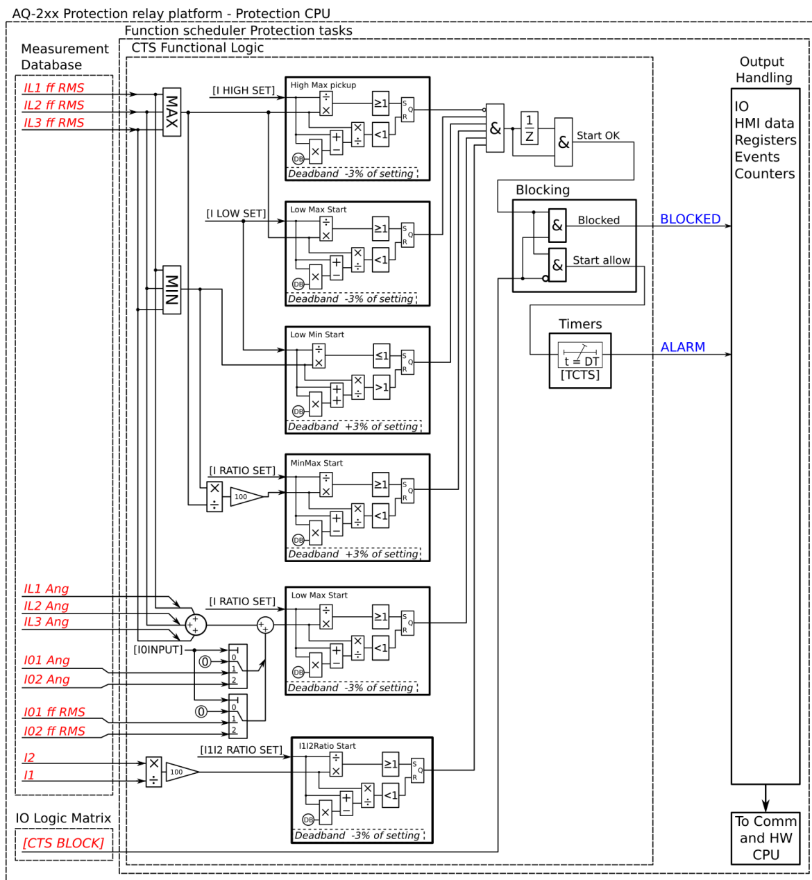
Figure. 5.6.1 - 177. Simplified function block diagram of the CTS function.
