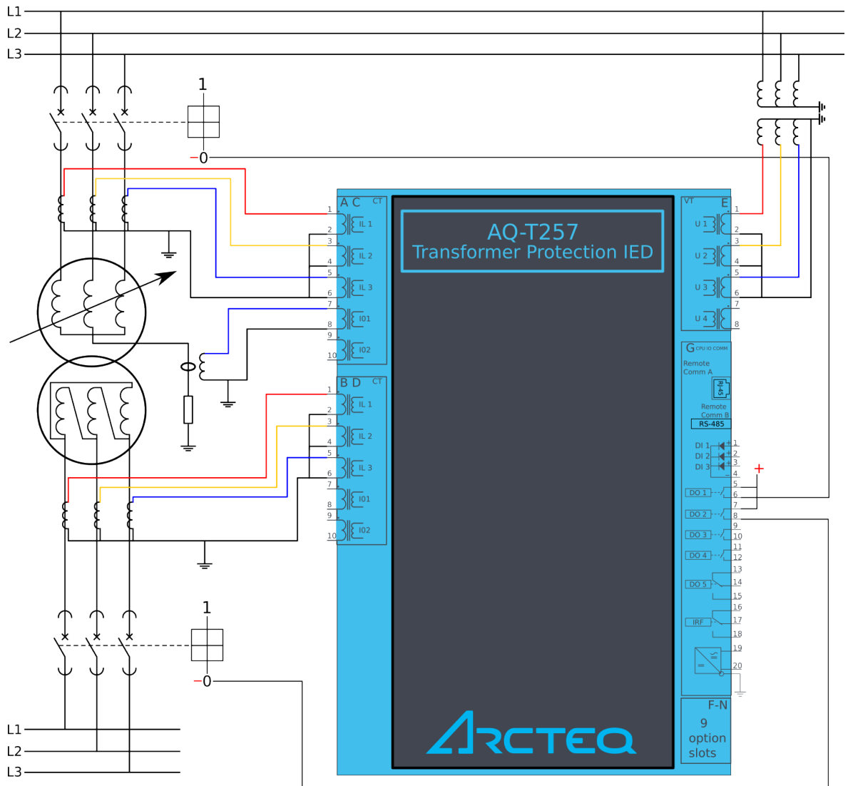
Figure. 7.2 - 202. Application example and its connections.
