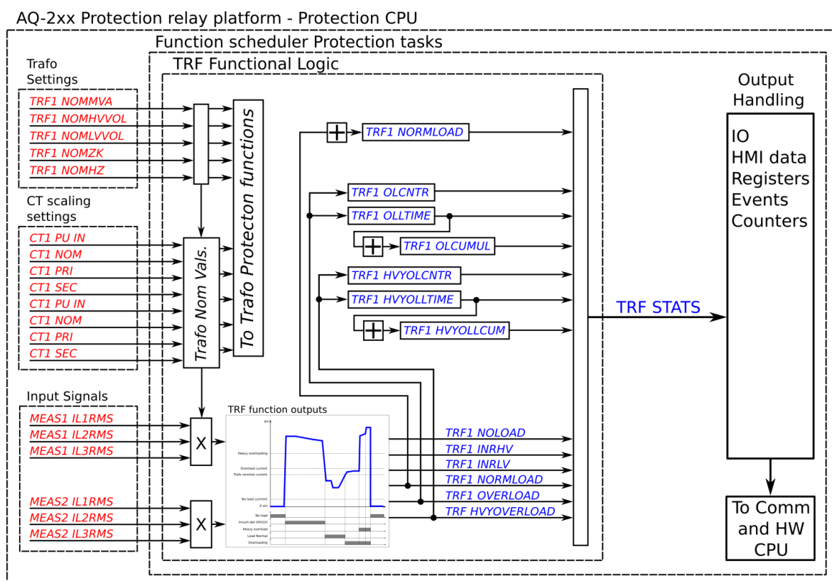
Figure. 5.4.19 - 98. Simplified function block diagram of the transformer status monitoring function.
