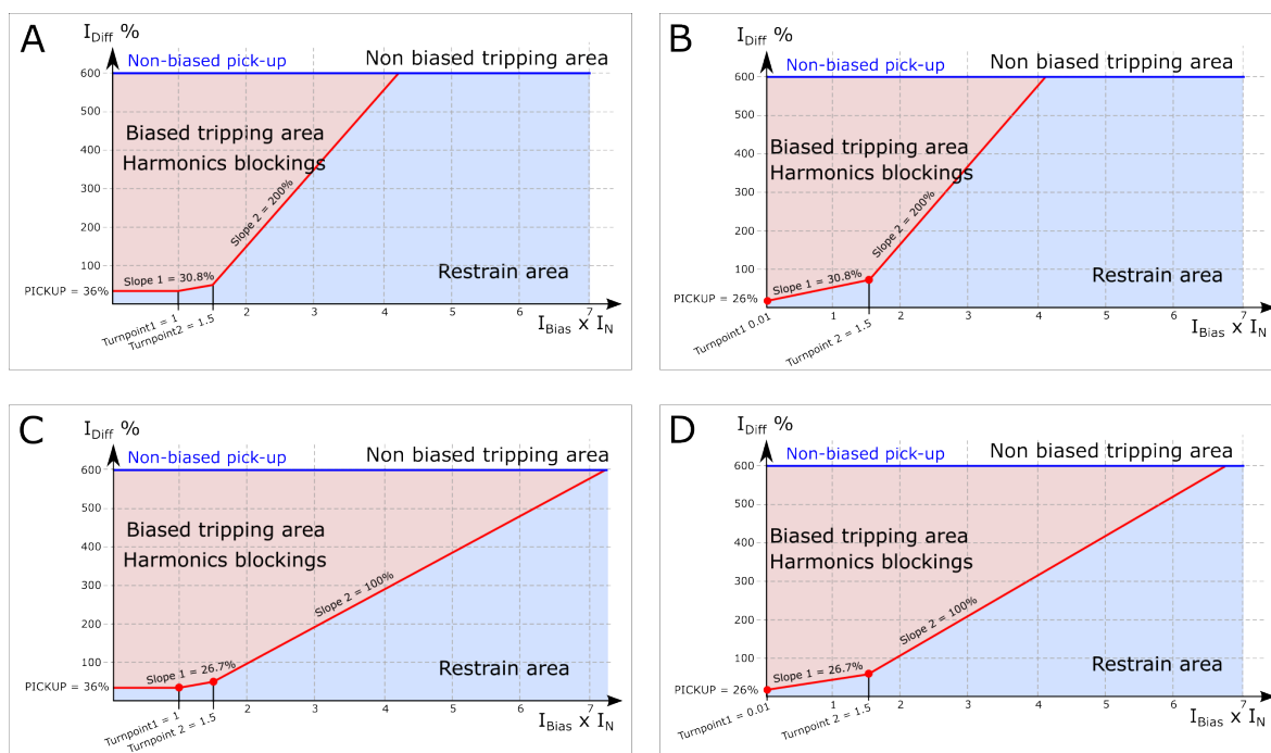
Figure. 5.4.21 - 119. Example differential characteristics
