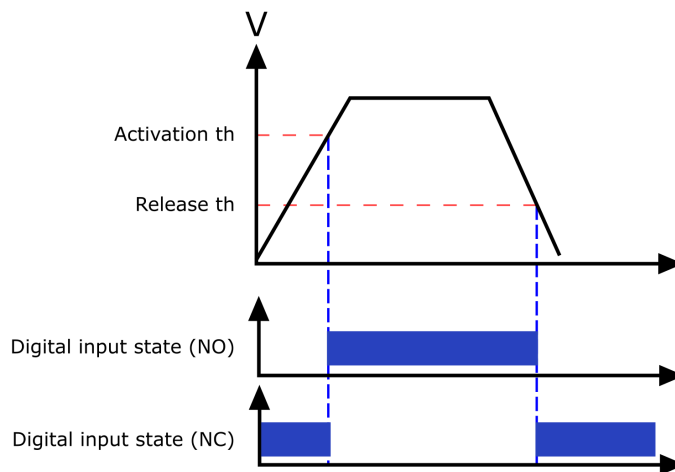
Figure. 8.5 - 215. Digital input state when energizing and de-energizing the digital input channels.
