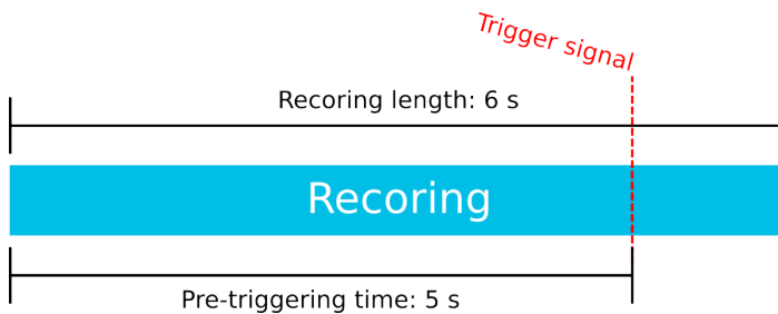
Figure. 5.6.6 - 196. Effects of recording length and pre-triggering time signals. This example is based on the settings shown above.
