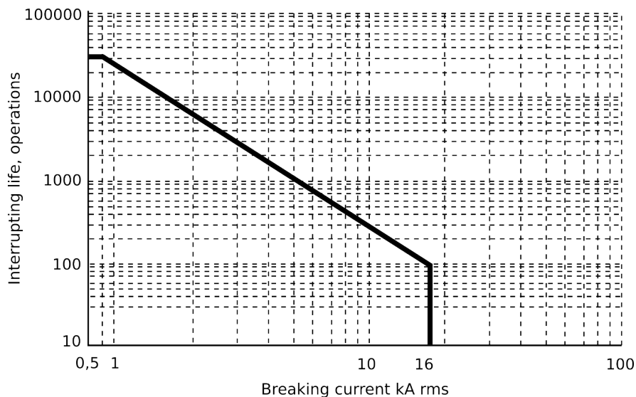
Figure. 5.6.3 - 189. Example of the circuit breaker interrupting life operations.
