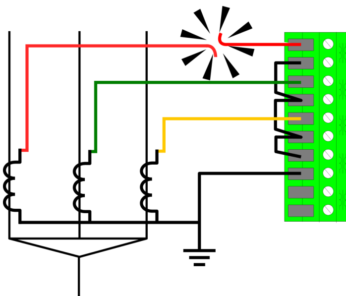
Figure. 5.6.1 - 176. Secondary circuit fault in phase L1 wiring.
