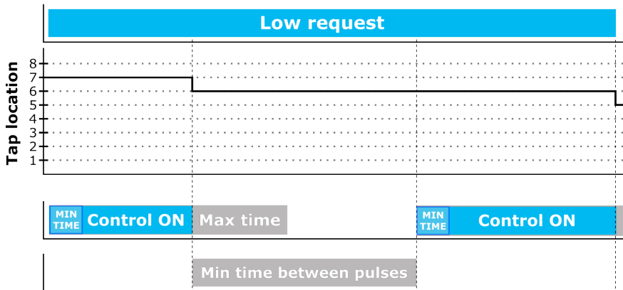
Figure. 5.5.2 - 138. Control pulse timing settings.
