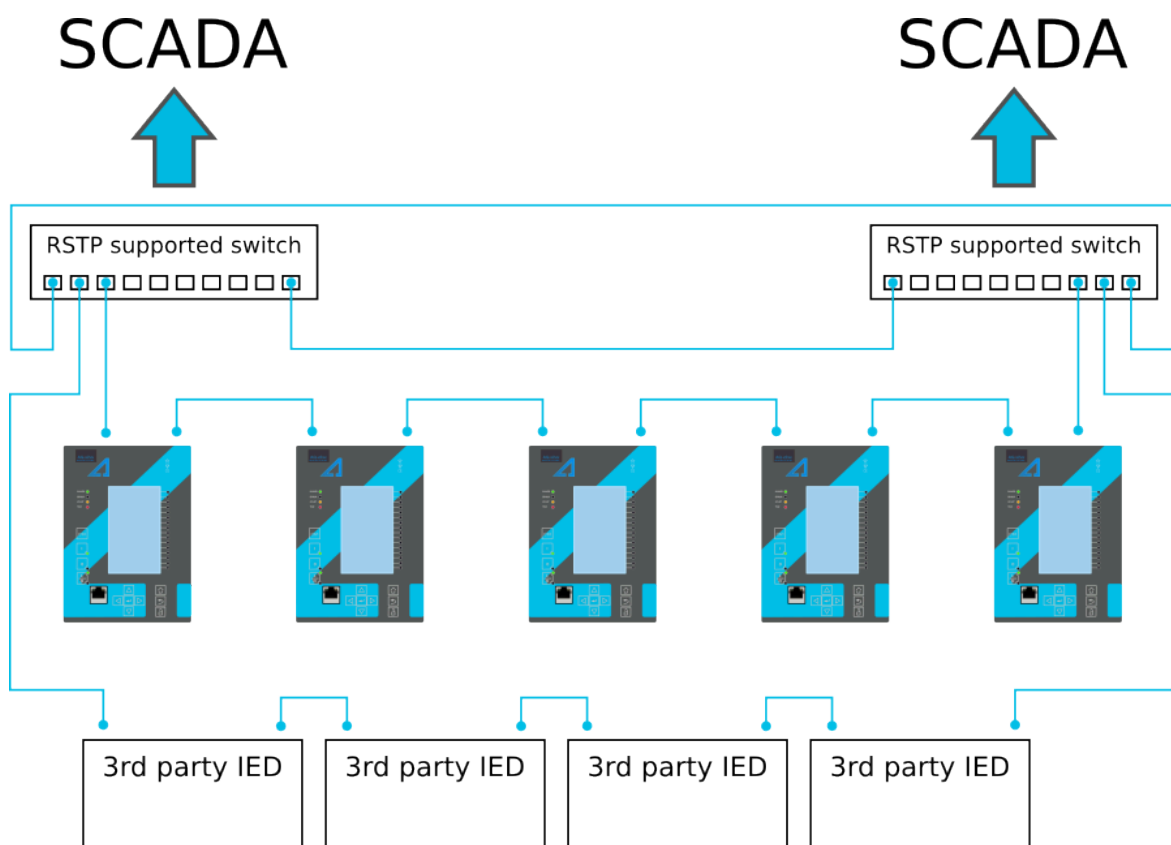
Figure. 8.11 - 223. Example of a ring configuration.
