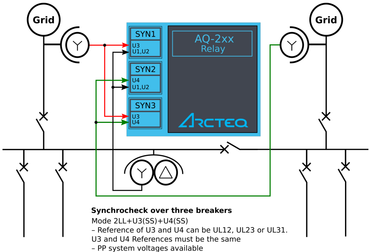
Figure. 5.5.6 - 168. Example application (synchrocheck over three breakers, with 2LL+U3+U4 connection).
