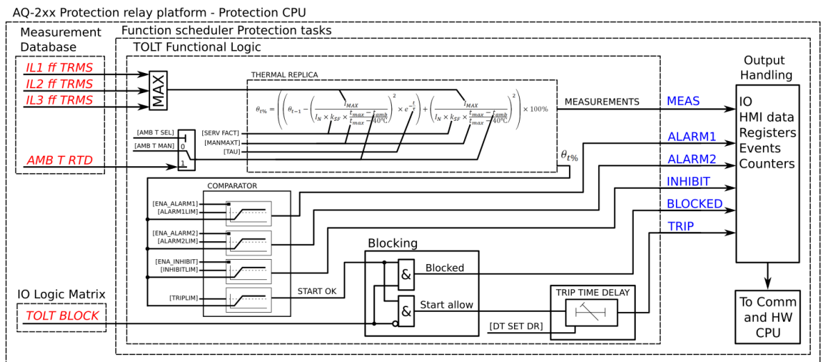
Figure. 5.4.20 - 102. Simplified function block diagram of the TT> function.
