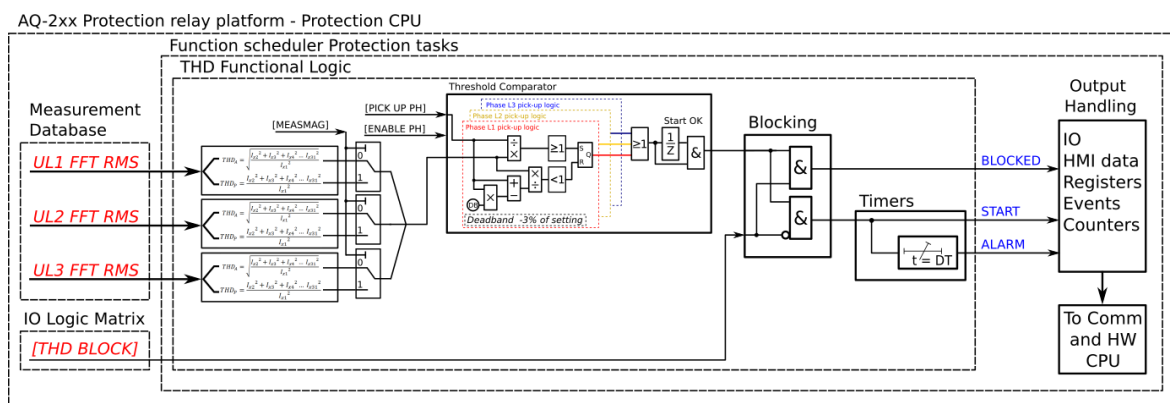
Figure. 5.6.5 - 194. Simplified function block diagram of the total harmonic distortion monitor function.
