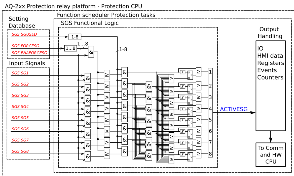
Figure. 5.5.3 - 154. Simplified function block diagram of the setting group selection function.
