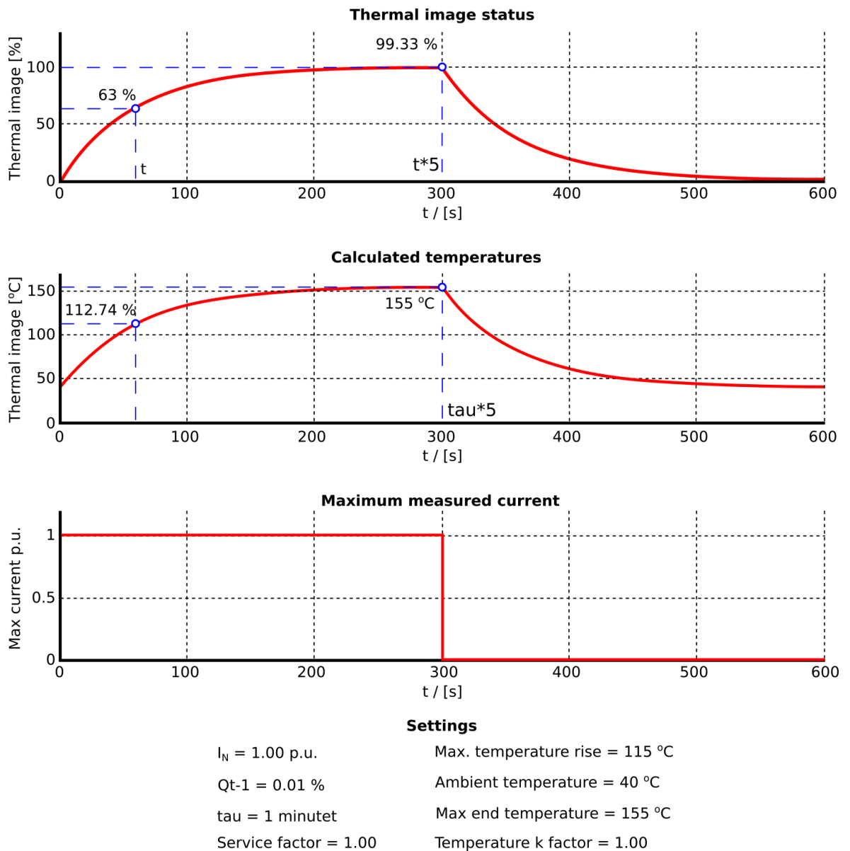
Figure. 5.4.20 - 100. Example of thermal image calculation with nominal conditions.
