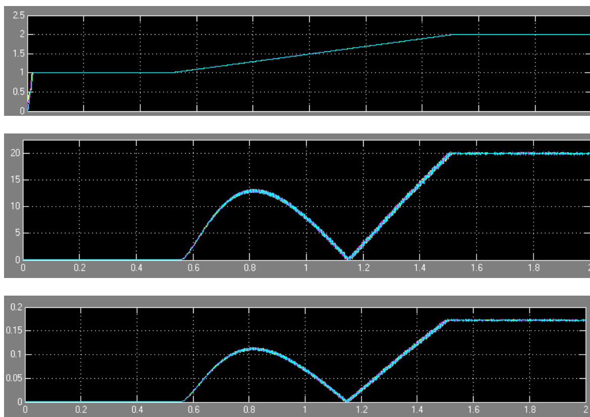
Figure. 5.4.21 - 128. System voltage and magnitude of the 5 th harmonic component.
