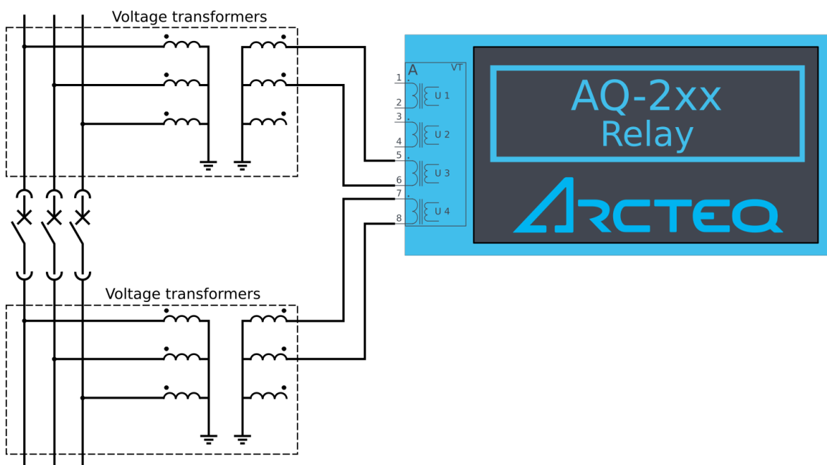
Figure. 5.5.6 - 165. Example application (synchrocheck over one breaker, with 3LL and 3LN VT connections).
