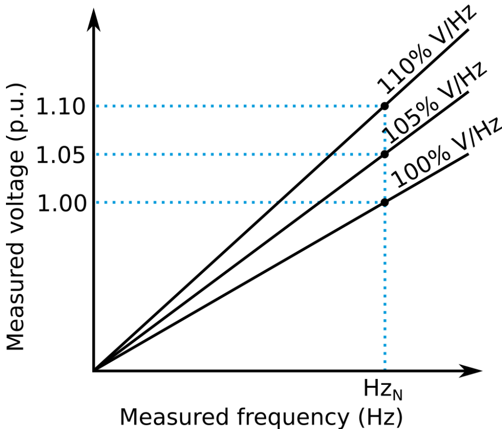
Figure. 5.4.17 - 92. Effect of pick-up settings and the measured frequency to the overvoltage function's pick-up level.
