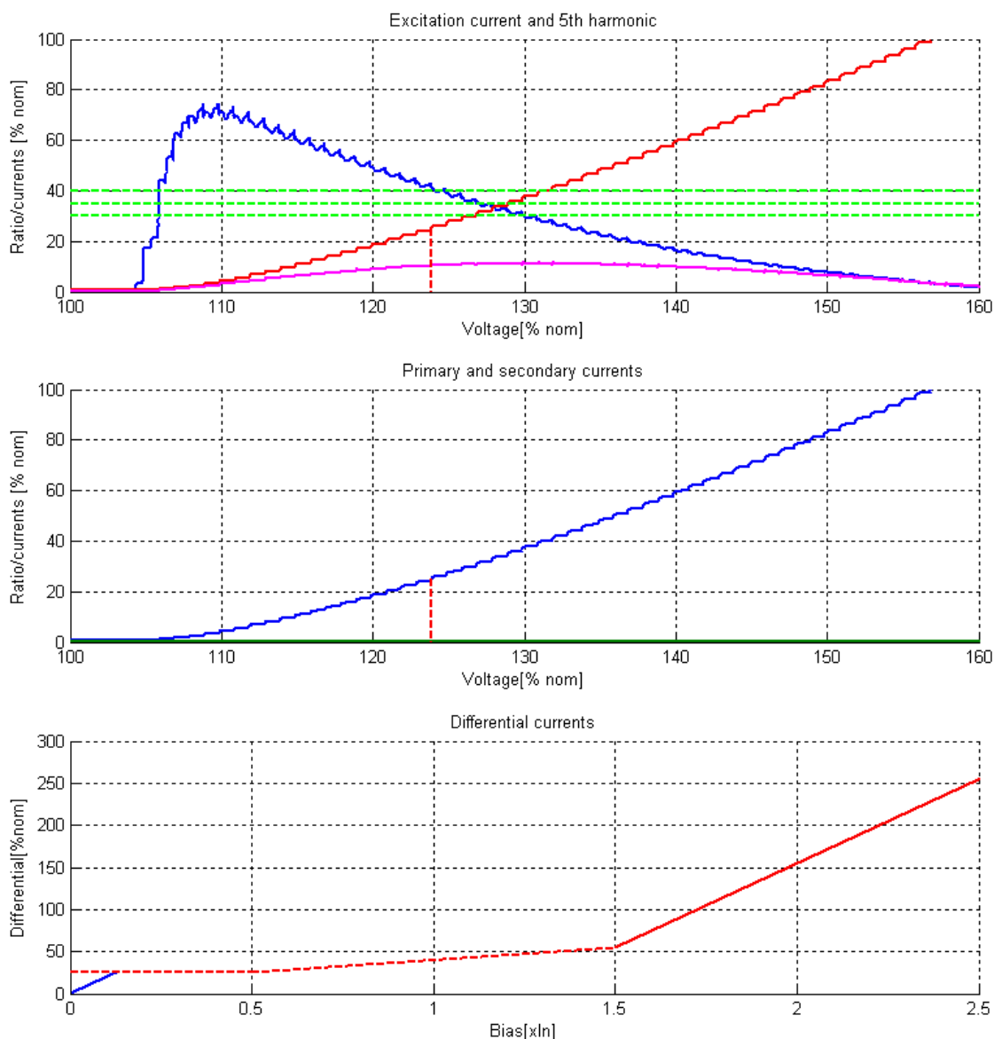
Figure. 5.4.21 - 126. Transformer behavior in case of overvoltage caused by overexcitation.
