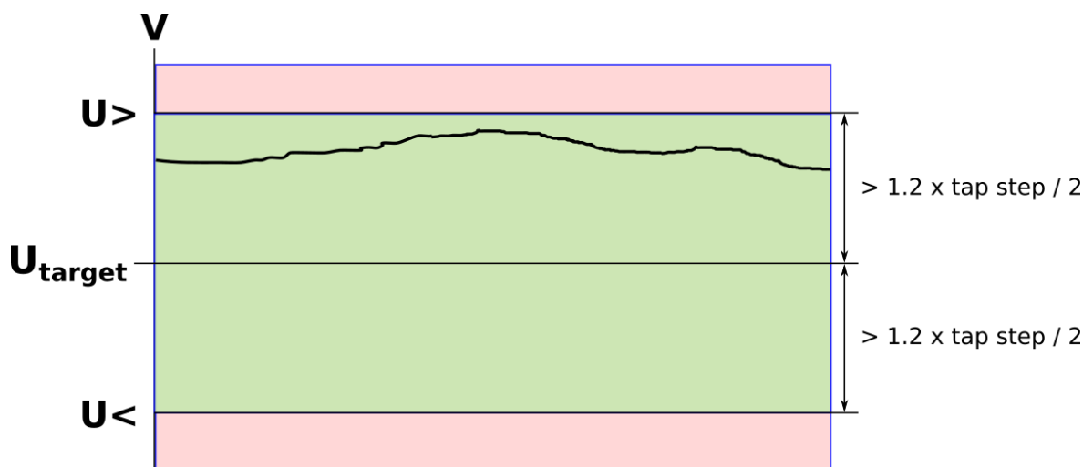
Figure. 5.5.2 - 147. Voltage window according to the recommendation.
