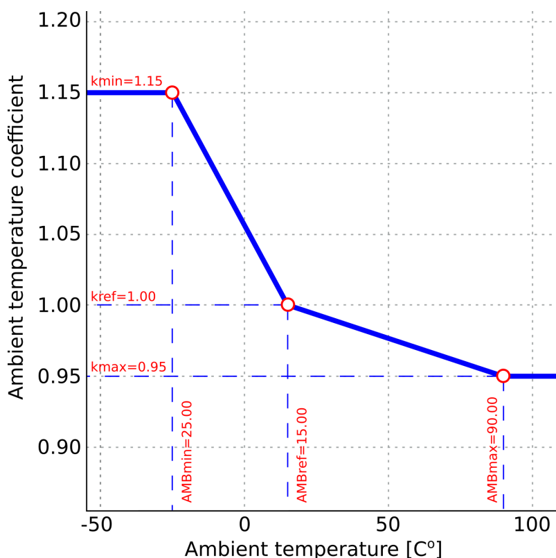
Figure. 5.4.20 - 101. Ambient temperature coefficient calculation (a three-point linear approximation and a settable correction curve).
