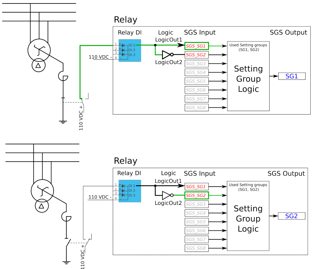
Figure. 5.5.3 - 156. Setting group control – one-wire connection from Petersen coil status.
