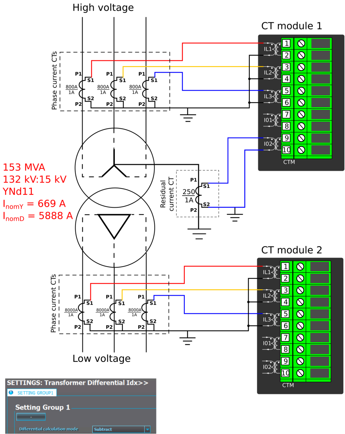
Figure. 5.2.1 - 4. Connections (application 1).
