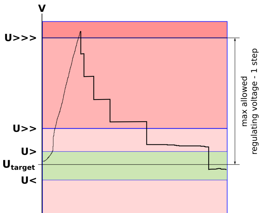
Figure. 5.5.2 - 151. Instant low command with two time-delayed windows.
