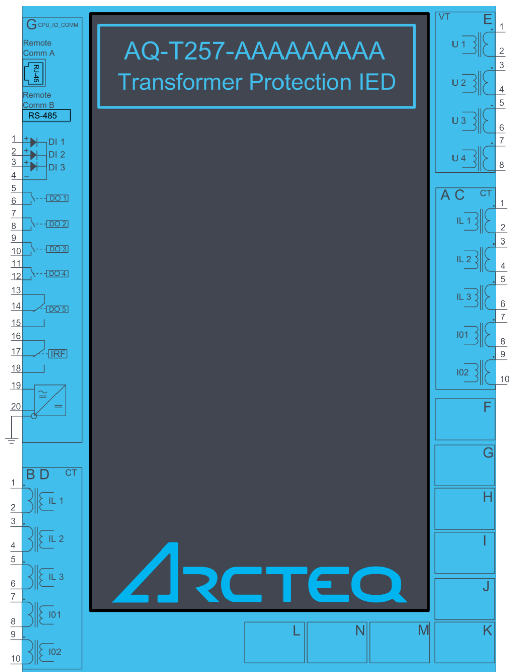
Figure. 7.1 - 199. AQ-T257 variant without add-on modules.
