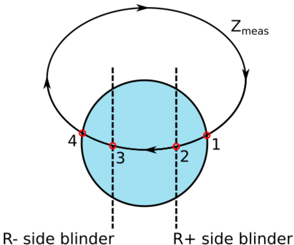
Figure. 5.4.18 - 97. Impedance must enter the circle first then cross the blinders and lastly exit the circle for the function to count a slip. Impedance can enter the circle from either side but it must keep entering the circle from the same side for the function to keep counting the slips.
