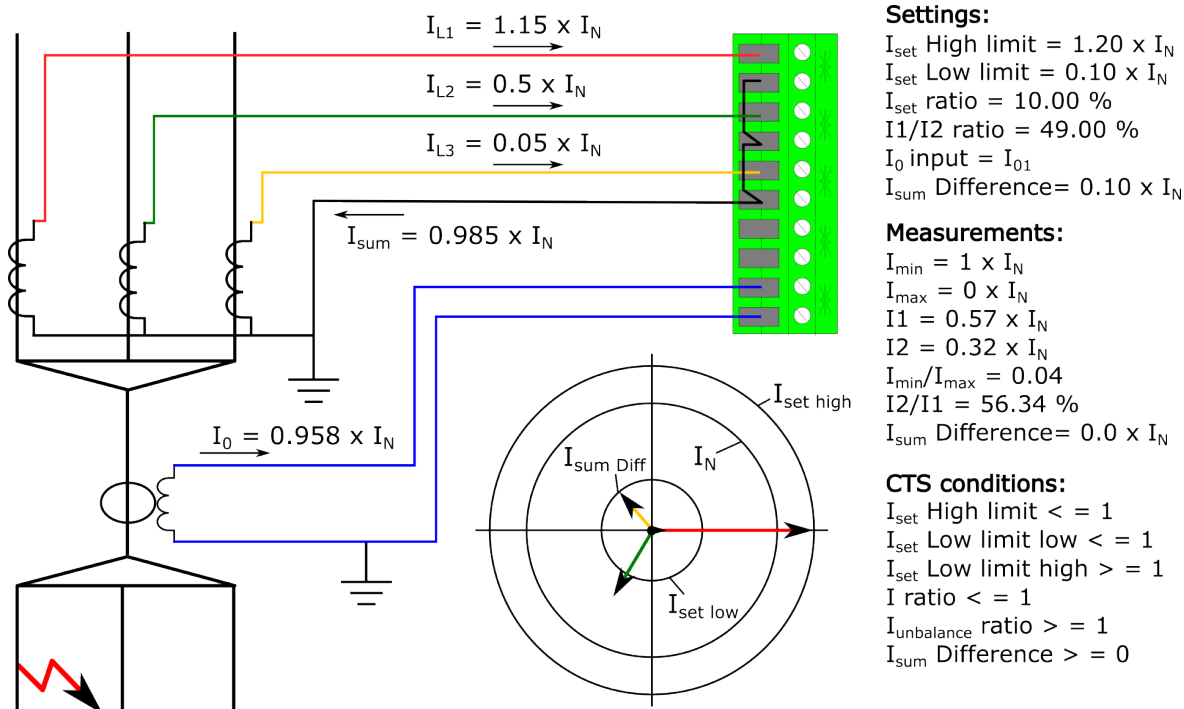
Figure. 5.6.1 - 186. Primary side high-impedance earth fault.
