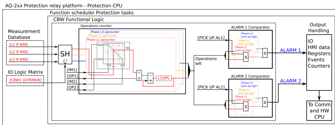
Figure. 5.6.3 - 190. Simplified function block diagram of the circuit breaker wear function.
