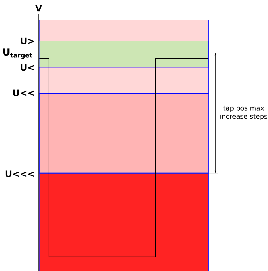
Figure. 5.5.2 - 153. Low voltage blocking.
