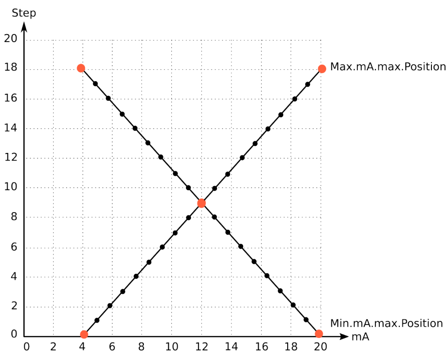
Figure. 5.5.2 - 141. Switching the tap position indication.
