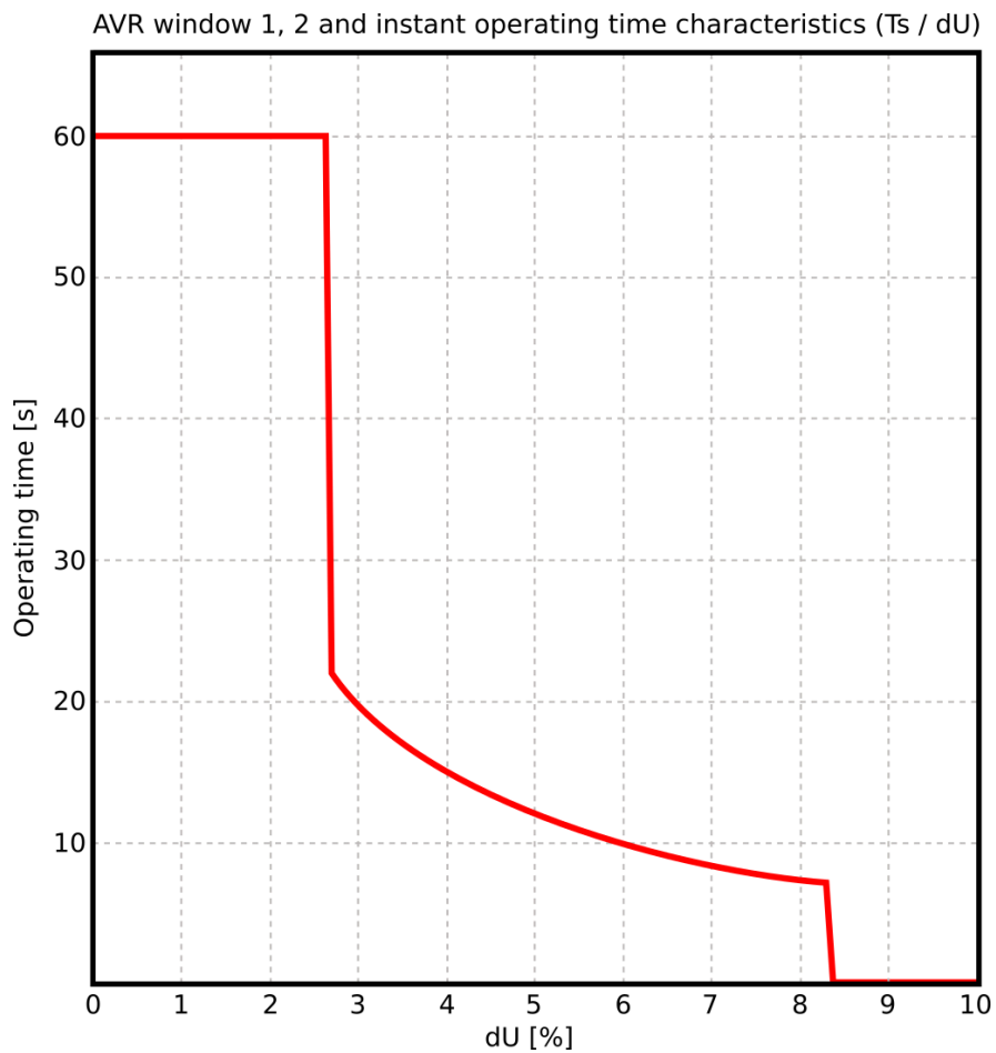
Figure. 5.5.2 - 152. Effect of the Instant low setting on time characteristics.
