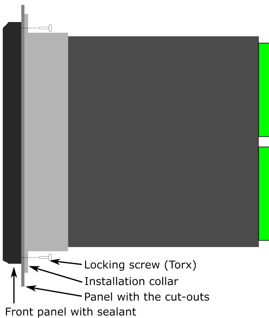
Figure. 8.14 - 229. Device installation.
