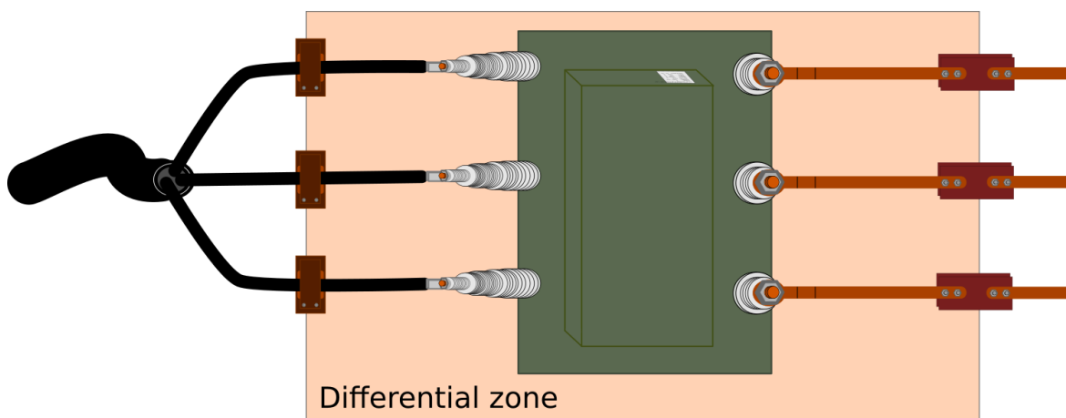
Figure. 5.4.21 - 104. Transformer and its components forming the differential zone.
