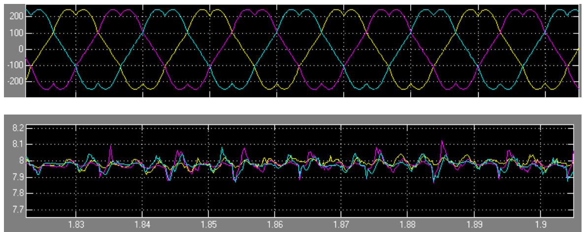
Figure. 5.4.21 - 127. Example waveforms.
