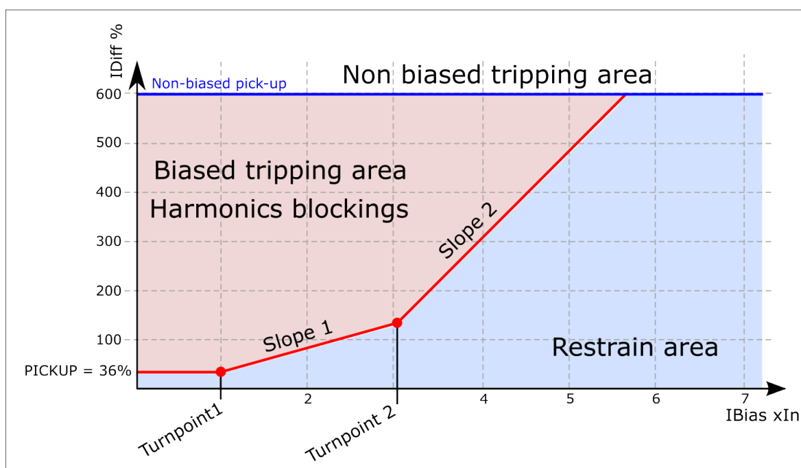
Figure. 5.4.21 - 115. Differential function characteristic, biased and non-biased.
