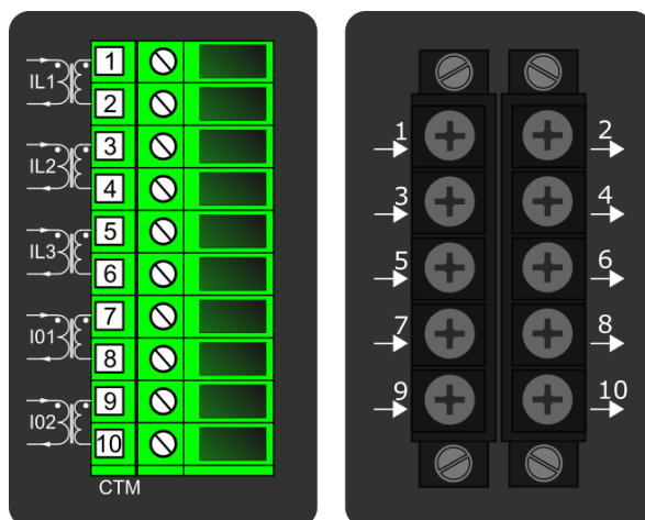
Figure. 8.3 - 212. Module connections with standard and ring lug terminals.
