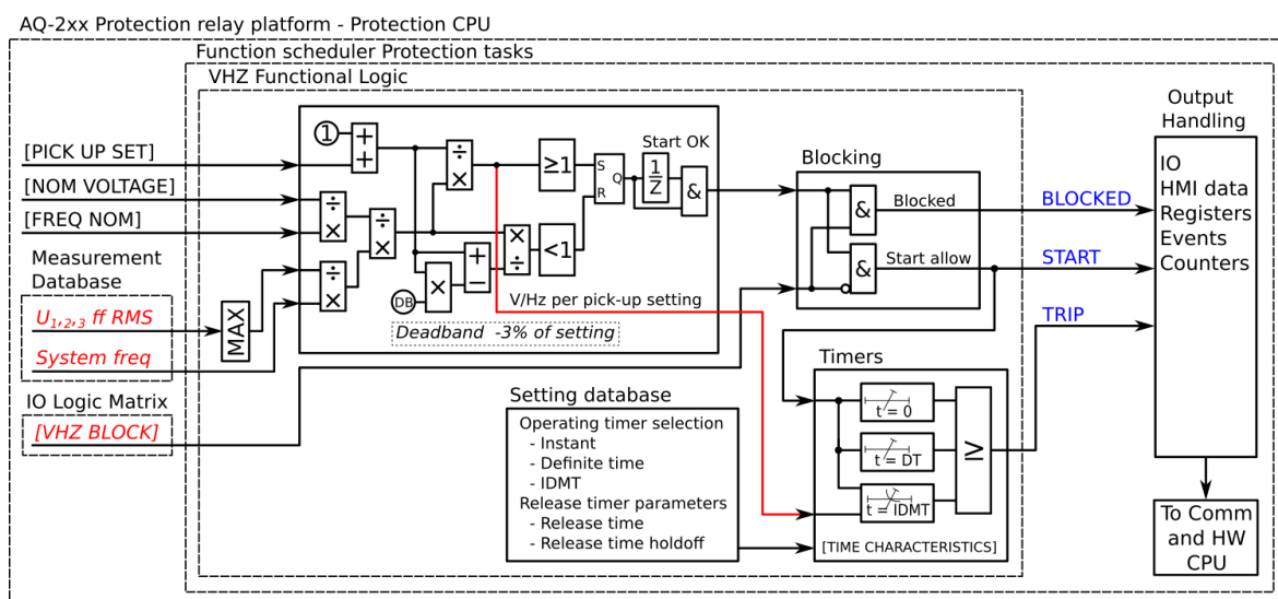
Figure. 5.4.17 - 93. Simplified function block diagram of the V/Hz> function.
