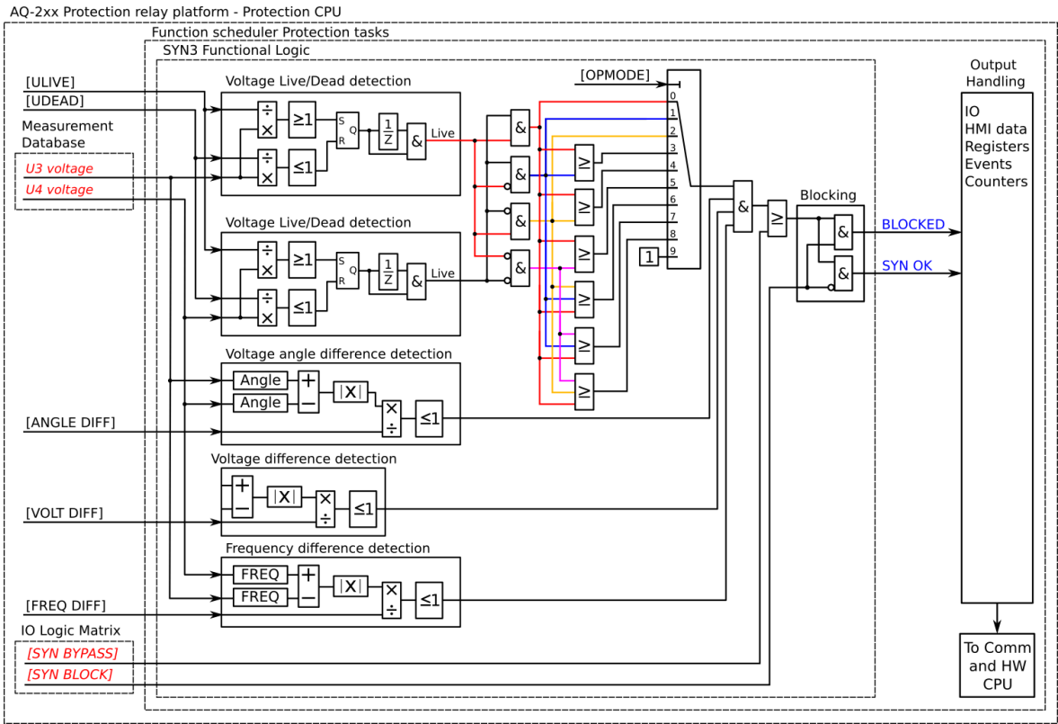
Figure. 5.5.6 - 171. Simplified function block diagram of the SYN3 function.
