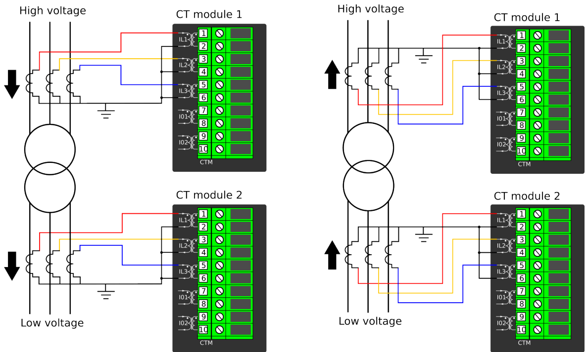
Figure. 5.4.21 - 112. CTs' starpoints requiring the "Subtract" mode.
