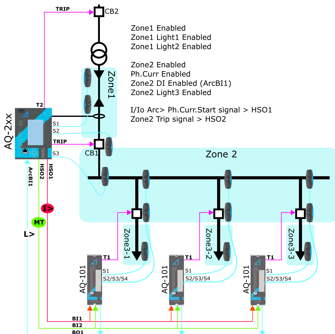
Figure. 5.4.23 - 132. Scheme IA1 (with AQ-101 arc protection relays).
