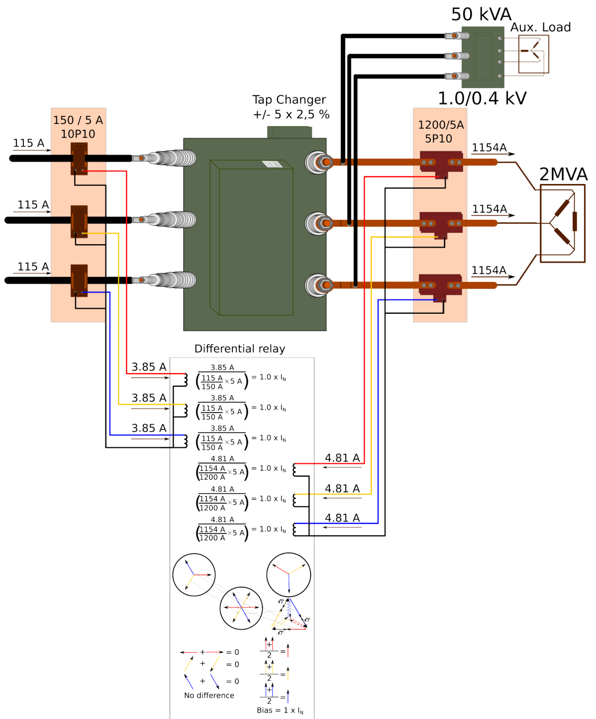
Figure. 5.4.21 - 118. Example configuration for the transformer differential function.
