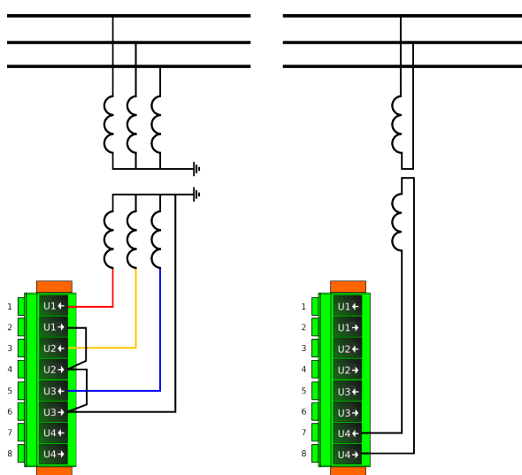
Figure. 5.5.2 - 137. Two connection options for voltage measurement.
