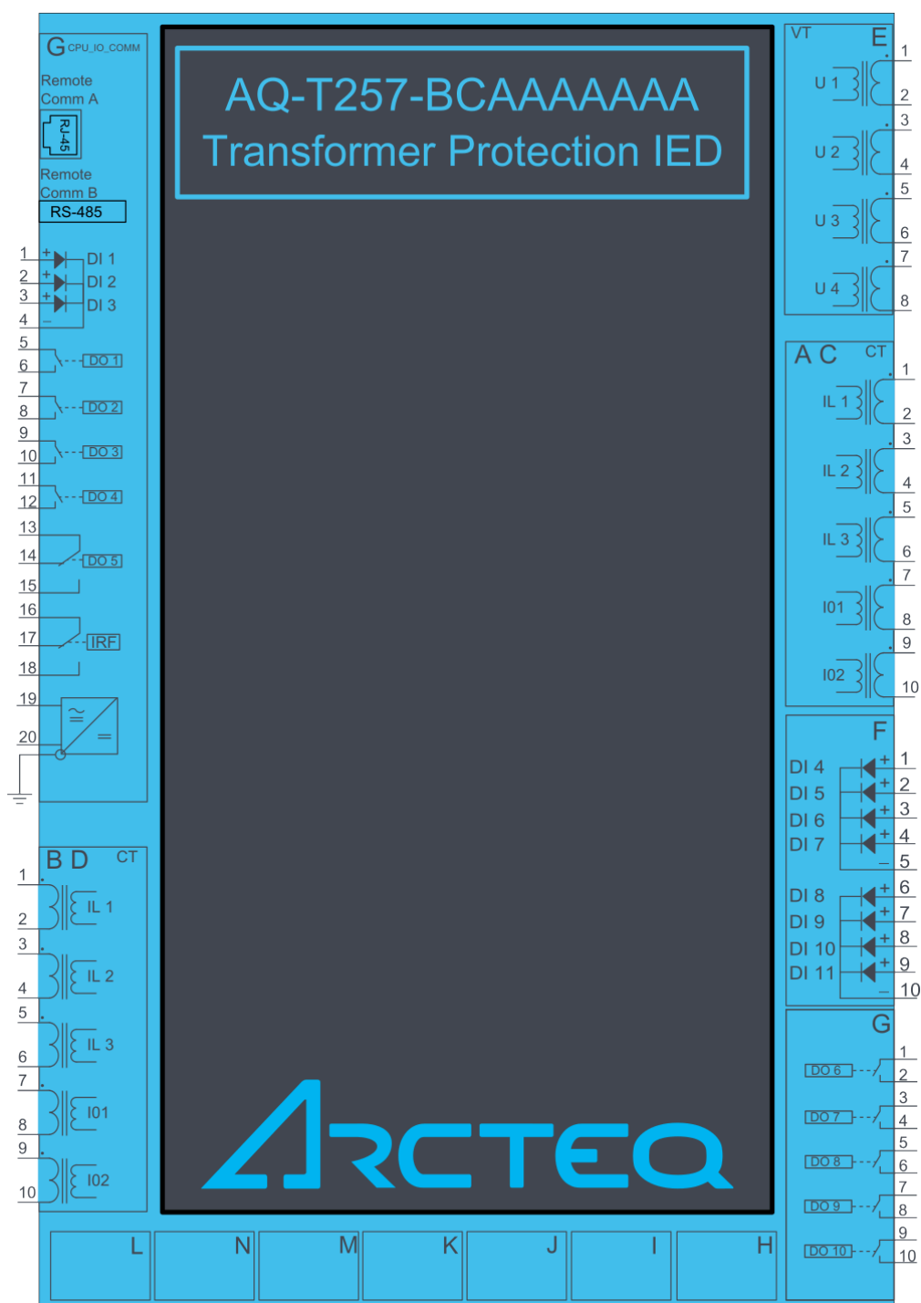
Figure. 7.1 - 200. AQ-T257 variant with digital input and output modules.
