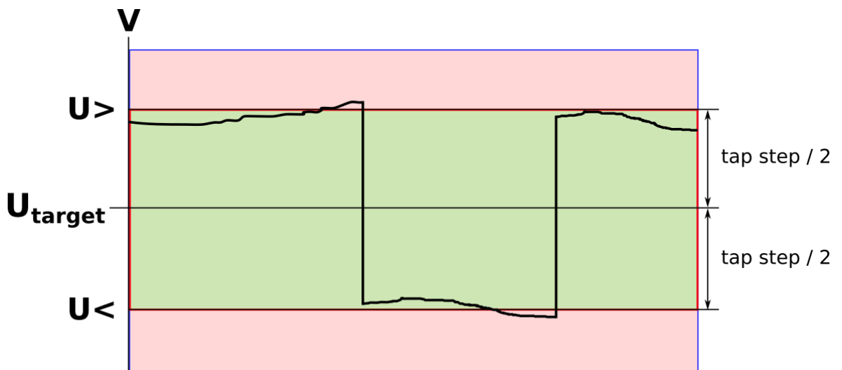
Figure. 5.5.2 - 146. Tight voltage window (window reached but voltage near the limit).
