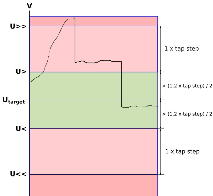
Figure. 5.5.2 - 148. Second voltage window two tap steps from the first voltage window.
