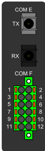
Figure. 8.9 - 220. Serial RS-232 module connectors.
