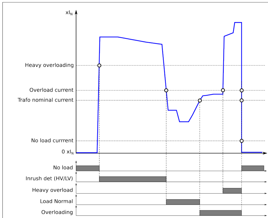
Figure. 5.4.19 - 99. Activation of the function's outputs.
