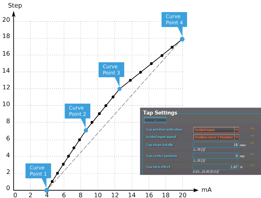
Figure. 5.5.2 - 142. Example of Scaled input setting.
