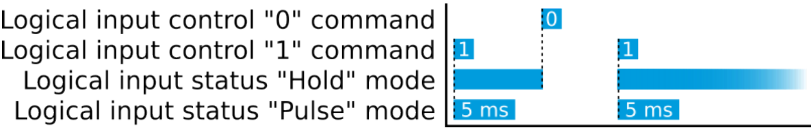
Figure. 5.5.11 - 174. Operation of logical input in "Hold" and "Pulse" modes.
