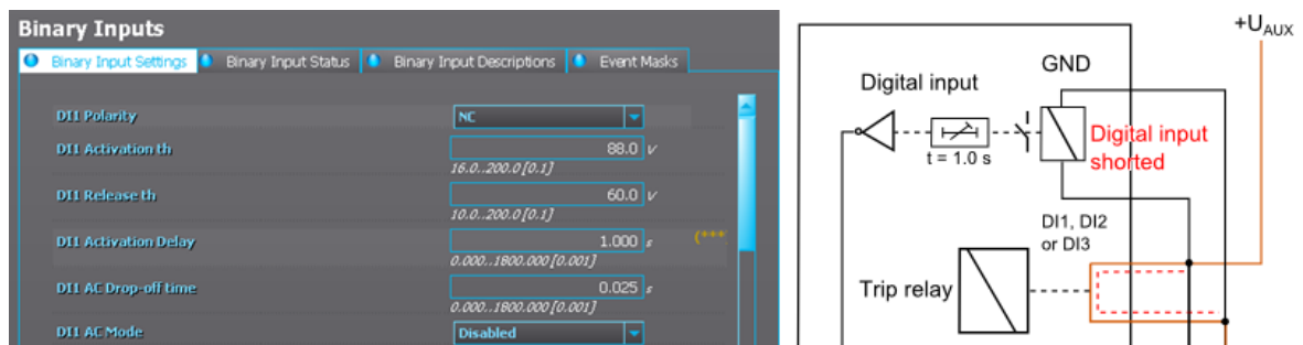
Figure. 7.3 - 204. Settings for a digital input used for trip circuit supervision.
