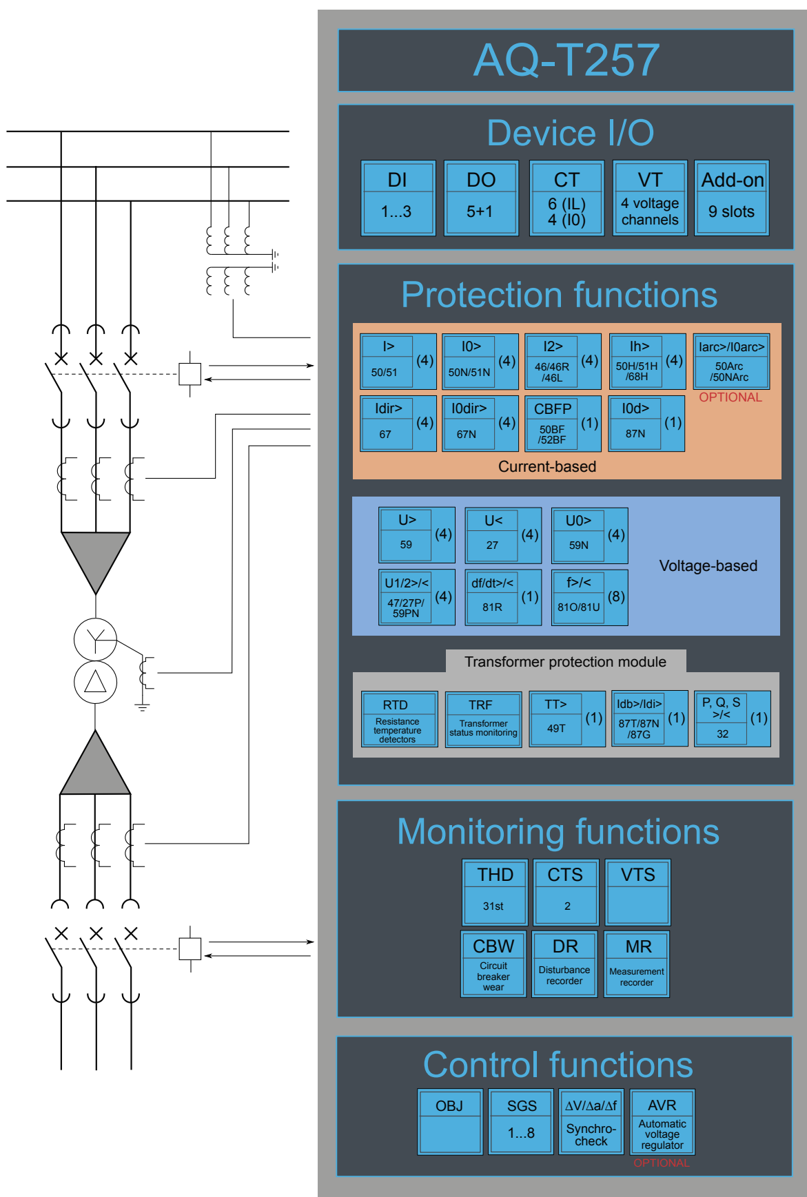
Figure. 7.1 - 201. AQ-T257 application example with function block diagram.
