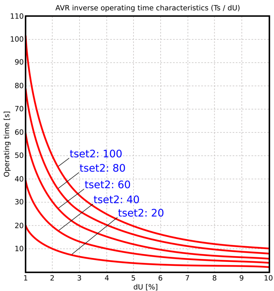
Figure. 5.5.2 - 149. Inverse operating time characteristics for the second voltage window ( U > U_{set2} ).
