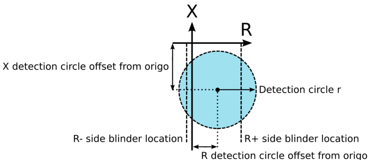
Figure. 5.4.18 - 96. Operating characteristics of pole slip protection.
