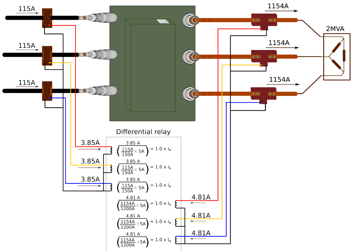
Figure. 5.4.21 - 106. Amplitude scaling to match the nominal currents and CTs in the differential relay.
