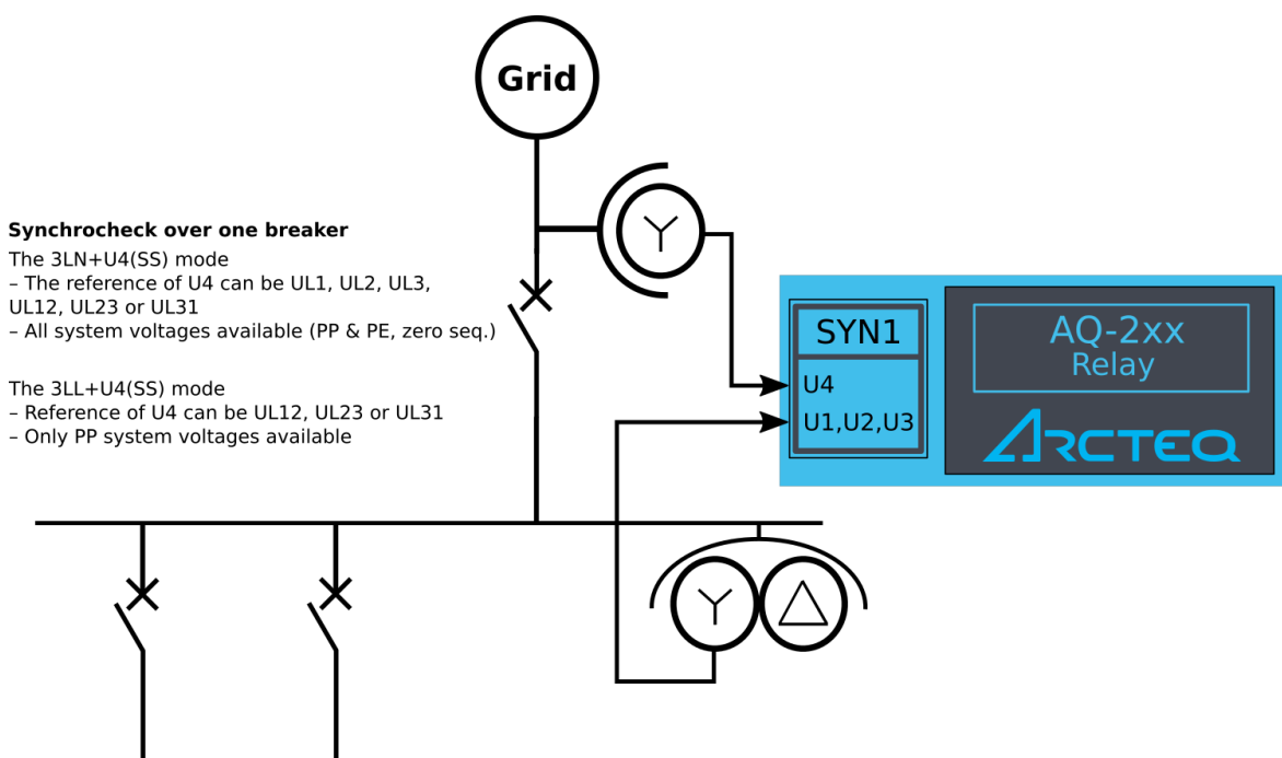
Figure. 5.5.6 - 165. Example application (synchrocheck over one breaker, with 3LL and 3LN VT connections).
