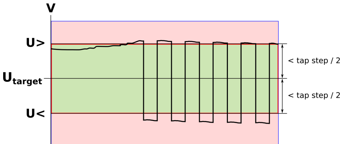
Figure. 5.5.2 - 145. Tight voltage window (window not reached).
