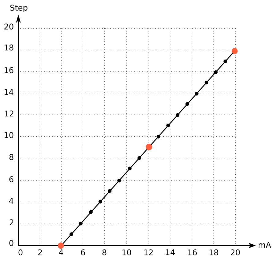
Figure. 5.5.2 - 140. Tap position indication (according to the example settings).
