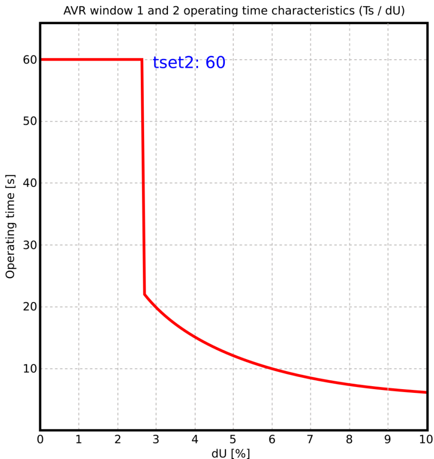
Figure. 5.5.2 - 150. Combined operating time characteristics of both voltage windows.
