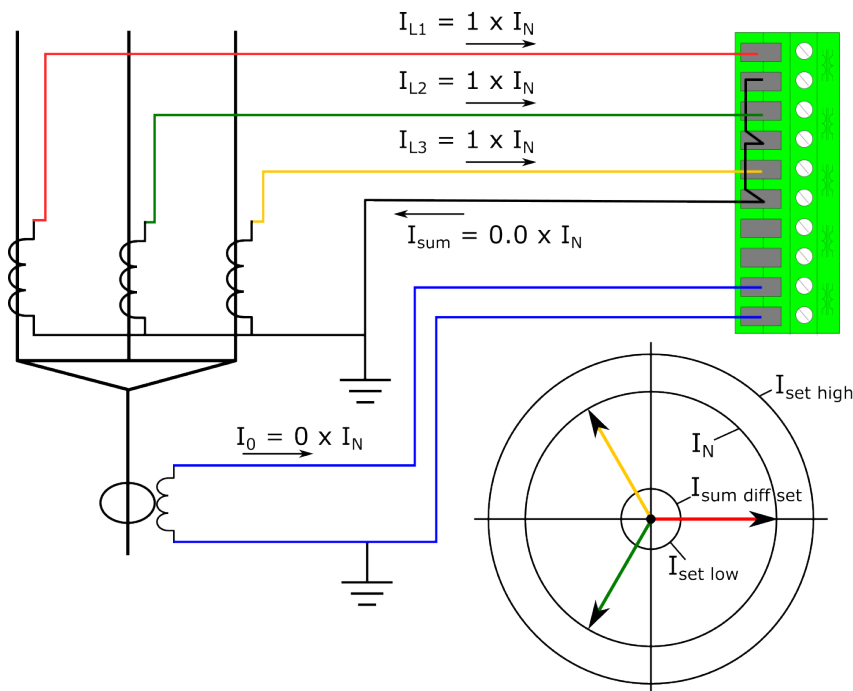
Figure. 5.6.1 - 183. Normal situation, residual current also measured.
