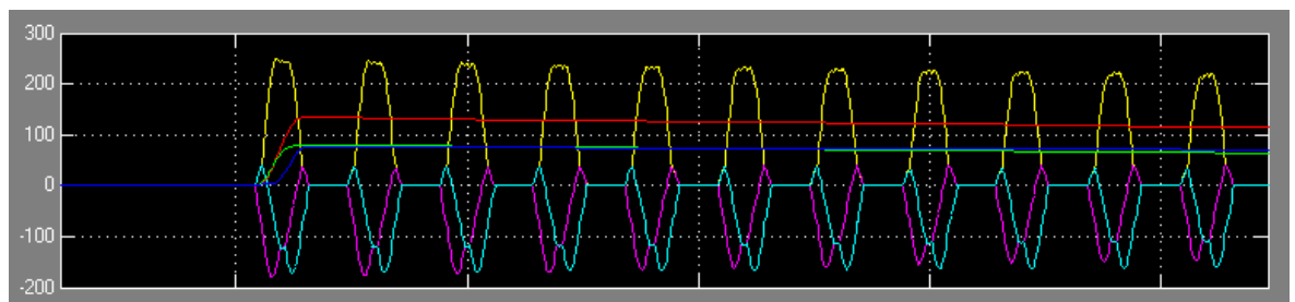
Figure. 5.4.21 - 125. Example of transformer magnetizing inrush currents.
