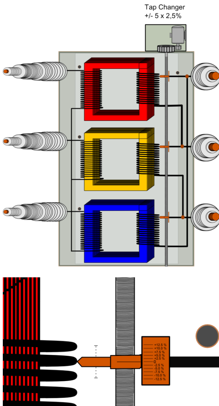
Figure. 5.4.21 - 117. Transformer tap changer.
