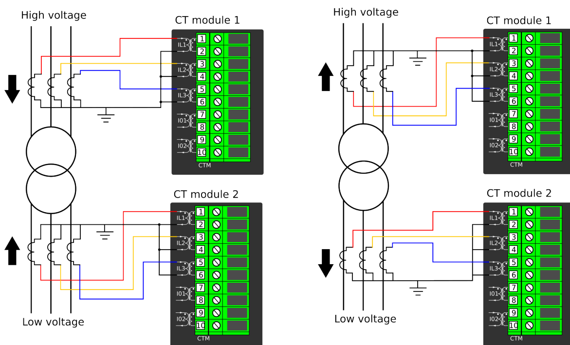
Figure. 5.4.21 - 111. CTs' starpoints requiring the "Add" mode.
