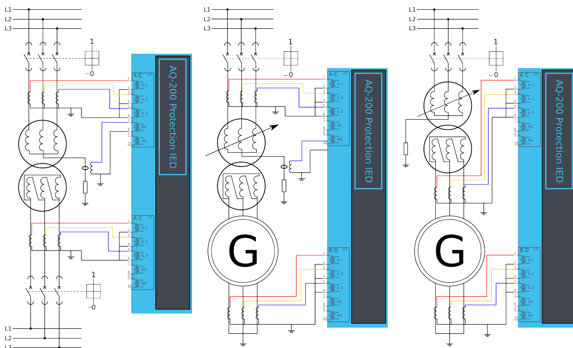
Figure. 5.4.21 - 103. Differential protection function can be used for protecting transformers, generators and both at the same time.
