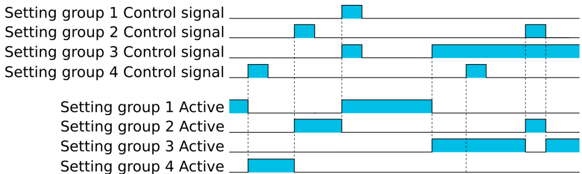
Figure. 5.5.3 - 155. Example sequences of group changing (control with pulse only, or with both pulses and static signals).
