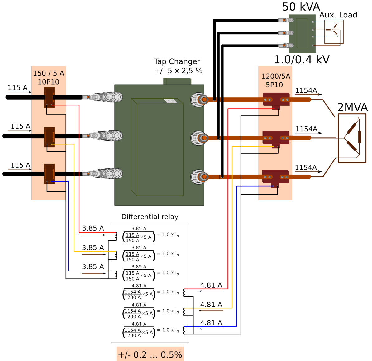
Figure. 5.4.21 - 116. Differential current sources (normal operation).
