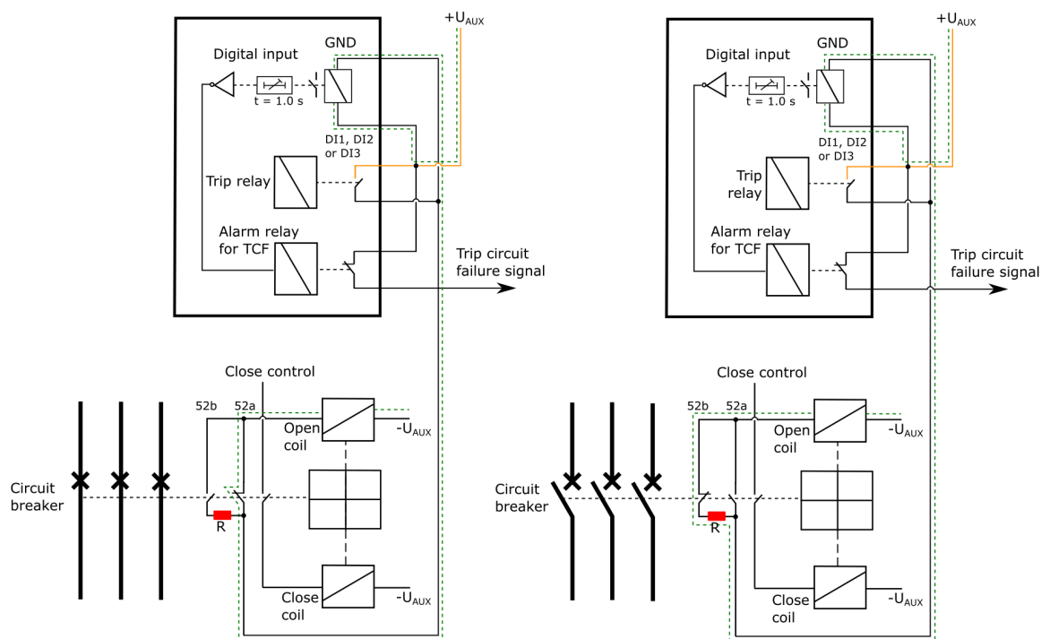
Figure. 7.3 - 203. Trip circuit supervision with one DI and one non-latched trip output.
