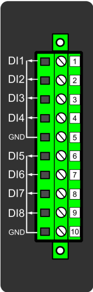
Figure. 8.5 - 214. Digital input module (DI8) with eight add-on digital inputs.
